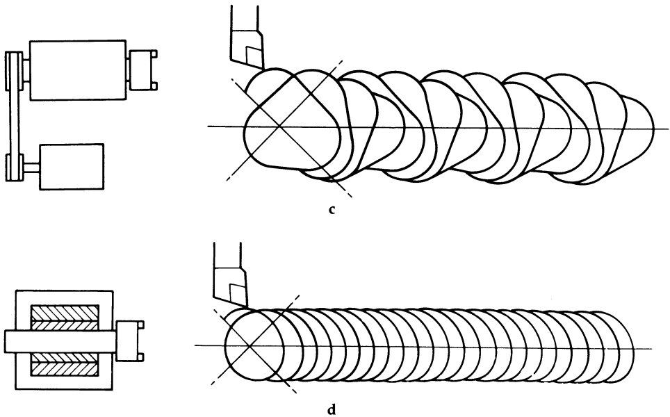
Fig. 2.26. The component quality is improved by using direct-drive spindles, rather than belt-driven headstocks on turning centres. a Direct-drive spindle cartridge for a turning centre. b The sinusoidal influence of component elements on a belt-driven headstock. c The harmonic effect of a belt-driven headstock on a turned component. d The harmonics virtually disappear on the component when direct-drive spindles are utilised. [Courtesy of Yamazaki Mazak Ltd.]
