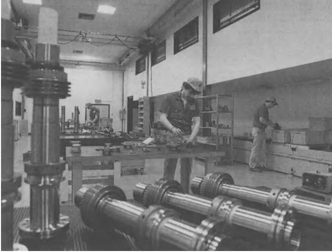
Fig. 2.23. The clean room and sub-assembly area for critical parts, such as spindles and headstocks (turning centres), also spindle cartridges (machining centres) prior to complete machine tool assembly. [Courtesy of Yamazaki Mazak Ltd.]
