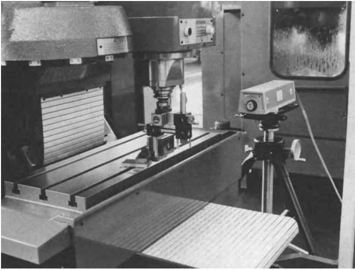
Fig. 1.13. The final test area, prior to alignment testing (laser calibration assessment). Each machine tool is run continuously to check both electrical and mechanical performance before acceptance. [Courtesy of Bridgeport Machine Tools.]
