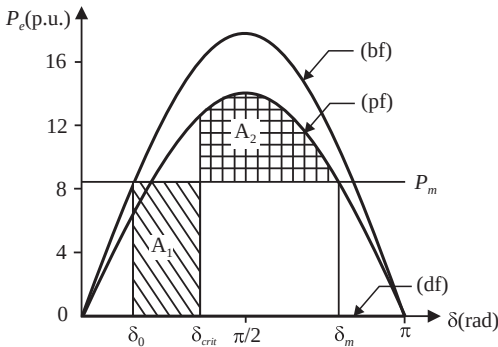
Figure 10.33. Transient characteristic.
