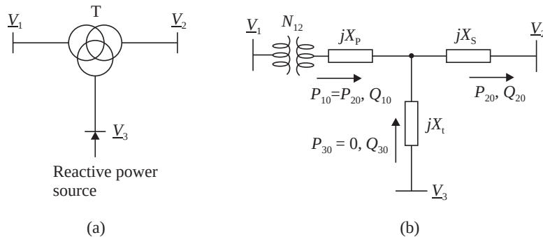
Figure 7.19. Three-winding OLTC transformer with synchronous compensator connected to its tertiary: (a) one-line diagram; (b) equivalent impedance diagram.
