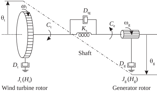
Figure 4.23. Two-mass model of a drive train (Adapted from [8]).
