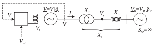
Figure 7.29. Generator connected to an infinite power bus.
