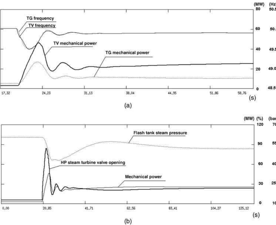
Figure 14.6. GT and SPP both synchronized and 30-MW ballast load connection: (a) GT and SPP comparison; (b) SPP results.
