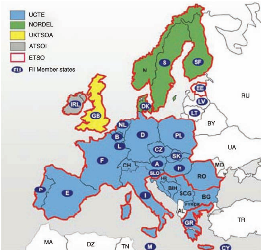
Figure 13.22. The UCTE (ENTSO-E since 2009) system.
