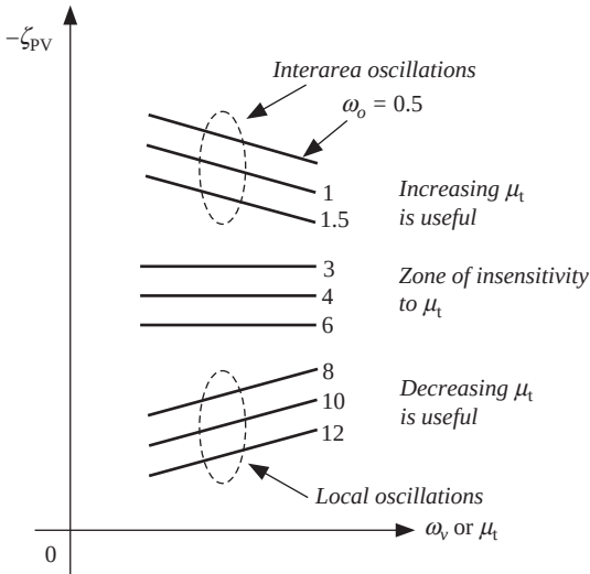
Figure 9.35. Damping contribution of AVR versus its dynamic gain.
