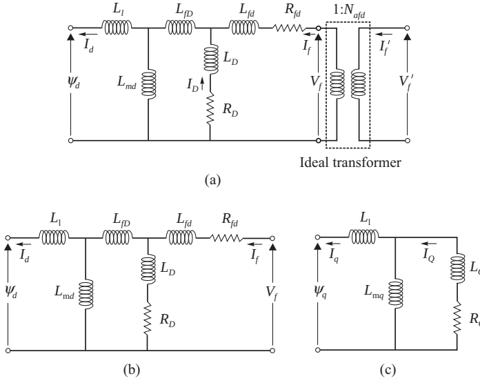
Figure 2.14. d-axis equivalent circuits with a single d -axis damper winding including an ideal transformer (a) and without ideal transformer (b); q -axis equivalent circuit with a single q -axis damper winding (c).
