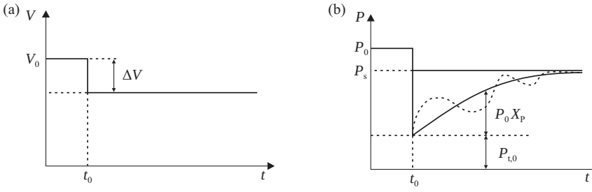
Figure 11.2. The dynamic active power response of a complex load (b) at sudden voltage variation in the connection node (a) [4].
