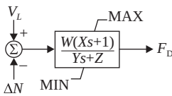
Figure 3.28. Combined-cycle speed-load controls [11].
