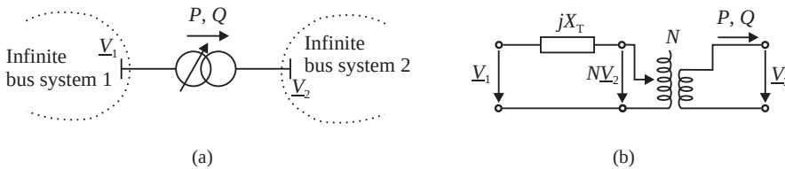
Figure 7.20. Interconnection of two strong networks through an OLTC: (a) one-line diagram; (b) equivalent impedance diagram.
