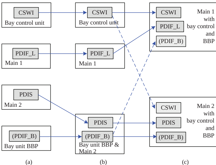
Figure 12.30. Trends to integrate protection functions in multifunctional relays.
