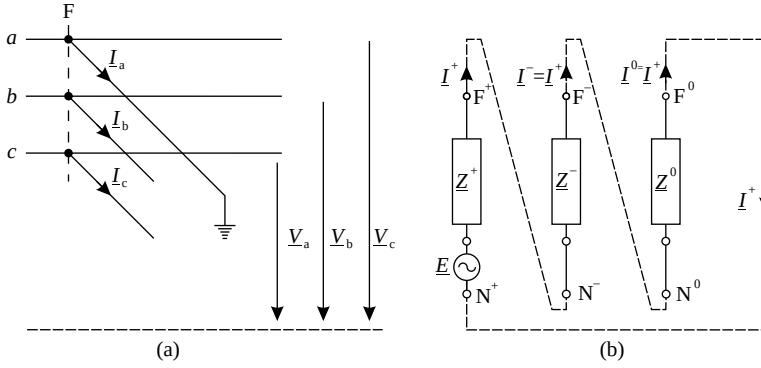
Figure. 5.15 Single phase-to-earth fault at F: (a) definition of fault; (b) equivalent circuit.
