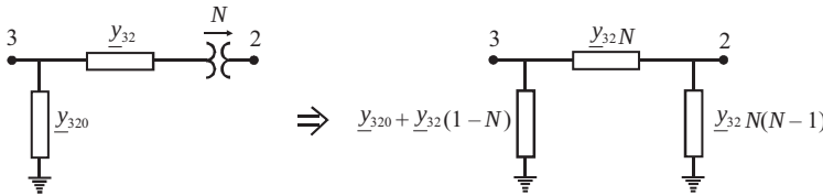
Figure 11.32. Transformation from a \Gamma quadripole into a \Pi (galvanic) quadripole for a transformer equivalent circuit.
