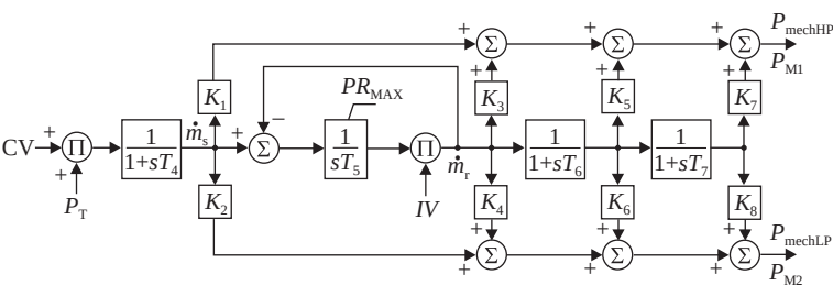
Figure 3.17. Generic turbine model including IV effects. (Reprinted with permission from Ref. 1. © 1991 IEEE.)
