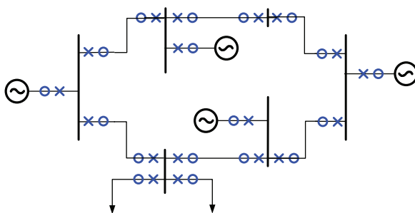
Figure 12.11. Principle structures of transmission power systems.
