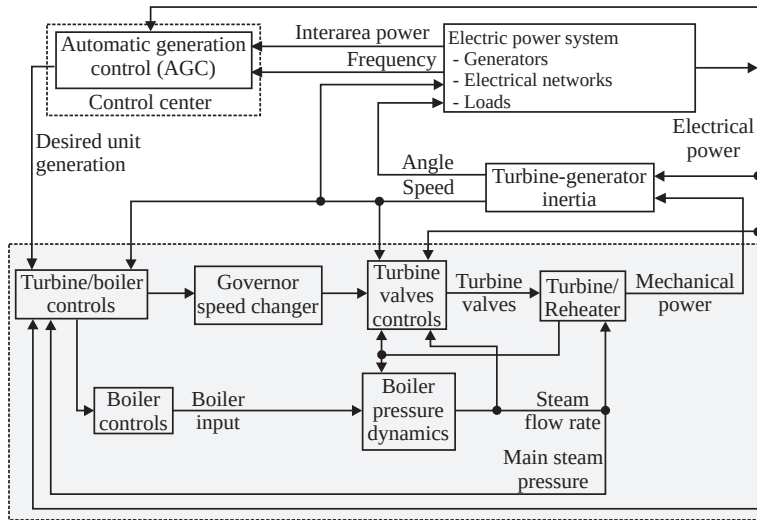
Figure 3.1. Functional block diagram showing relationship of prime mover systems control to complete system [1].
