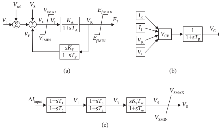
Figure 2.68. ST1-Type exciter with PSS input— V_s (a); terminal voltage control block (b); lead-lag power system stabilizer (c).
