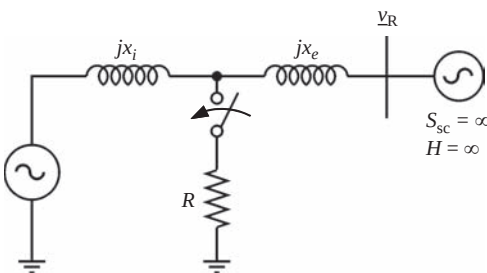
Figure 9.43. Switching-on of braking resistors at generator terminals.
