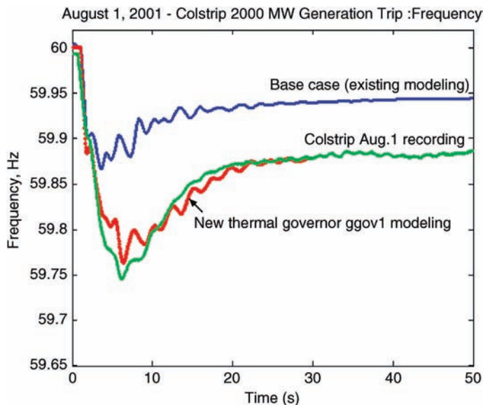
Figure 6.39. Governor model verification, 2000 MW Colstrip trip in Montana on Aug. 1, 2001.
