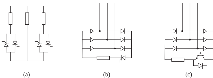
Figure 4.11. Crowbar arrangement [8,9].
