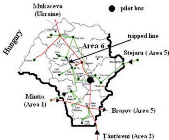
Figure 7.66. Area 6 interconnection lines with the neighboring areas and the tripped line in the test.
