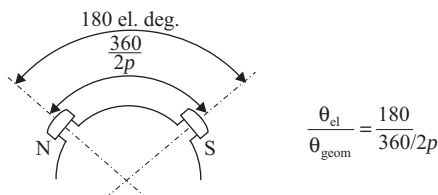
Figure 2.3. The relationship between mechanical and electrical angles.
