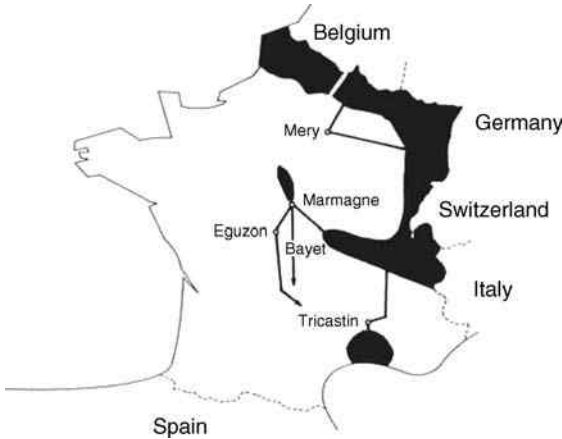
Figure 13.14. Part of the French grid still live at 8.26 a.m. on December 19, 1978 immediately after the first collapse [9].
