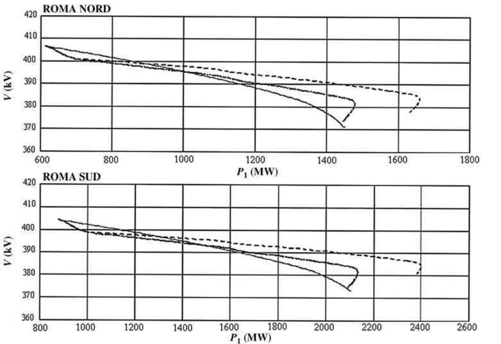
Figure 7.81. Italian grid load ramps stability margins (dynamic evolution): primary voltage regulation (continuous line), secondary voltage regulation (dotted line), secondary+tertiary voltage regulation (dashed line).
