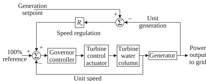
Figure 3.44. Governing system with speed regulation. (Reprinted with permission from Ref. 17. © 2004 IEEE.)
