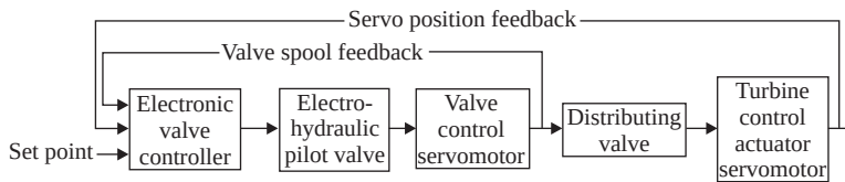
Figure 3.47. Typical electrohydraulic actuator. (Reprinted with permission from Ref. 17. © 2004 IEEE.)
