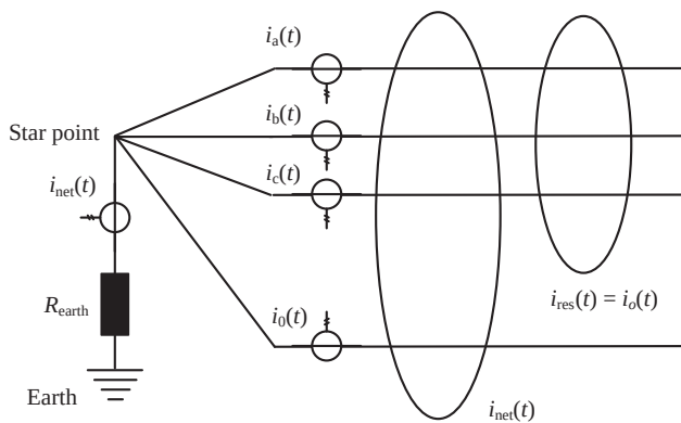
Figure 12.14. Currents caused by unbalance of faults in the three-phase systems.
