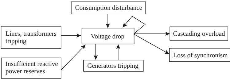
Figure 13.31. The mechanism of voltage collapse.
