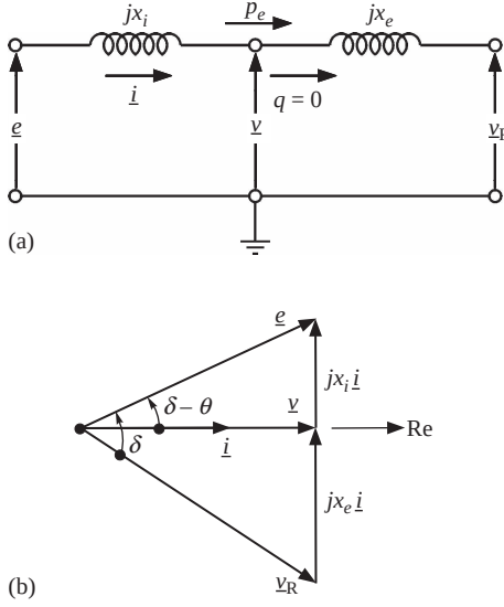
Figure 9.34. Example of evaluation of approximations when computing oscillation frequency.
