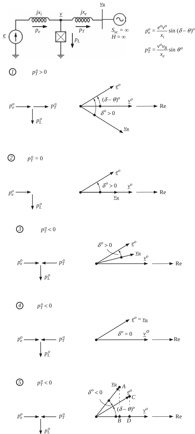
Figure 9.40. Unit in generation mode in the same operating point ( e^o , v^o , (\delta - \theta)^o , p_e^o are const.): effect of the decrease in real transit p_T^o with the increase in real load p_L^o .
