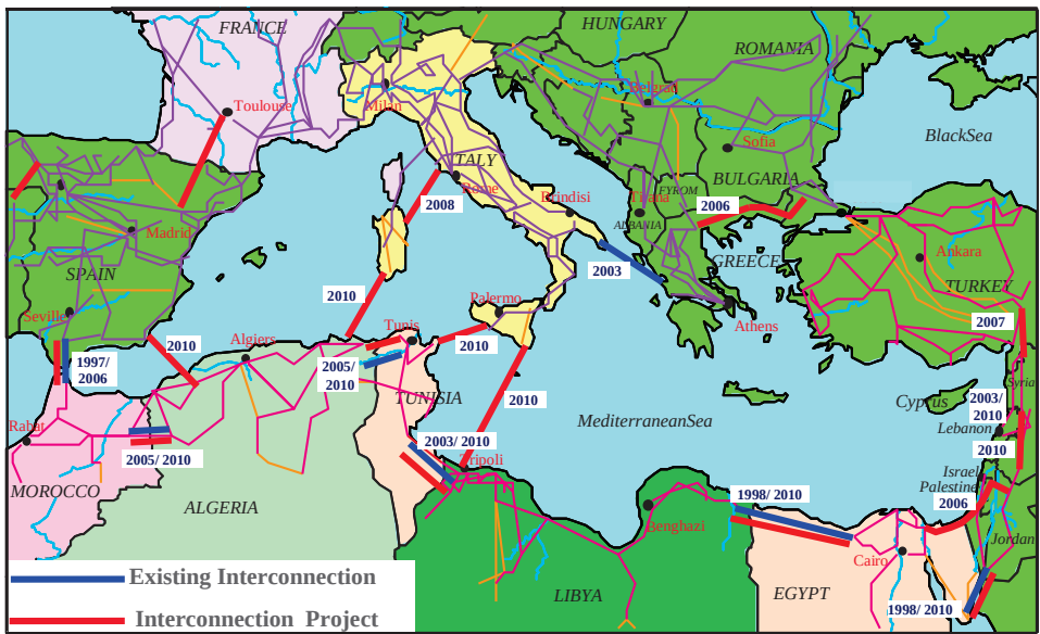
Figure 9.72. The MEDRING Power System.
