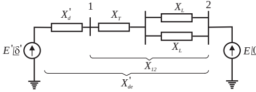
Figure 10.32. Equivalent circuit.
