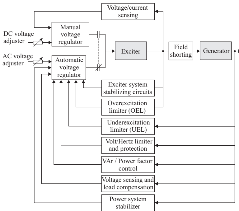
Figure 2.59. Excitation system control and protective circuits. (Adapted from Ref. 1.)
