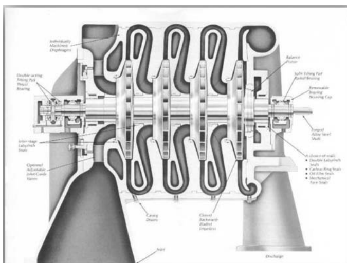
Figure 8-3. Centrifugal Compressor Cross-section Compliments of Dresser Roots, Inc.
