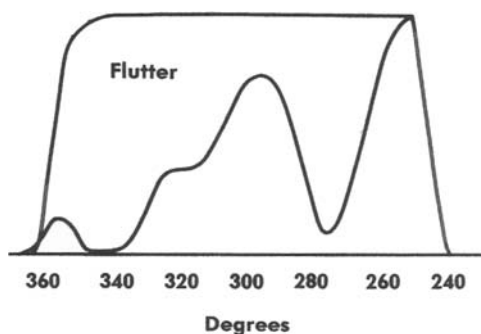
Figure 3-26. Incorrect Valve Operation—Valve Overspringing Courtesy of Roger Vaglia, Product Manager (Retired), White Superior Compressors 1962-2000
