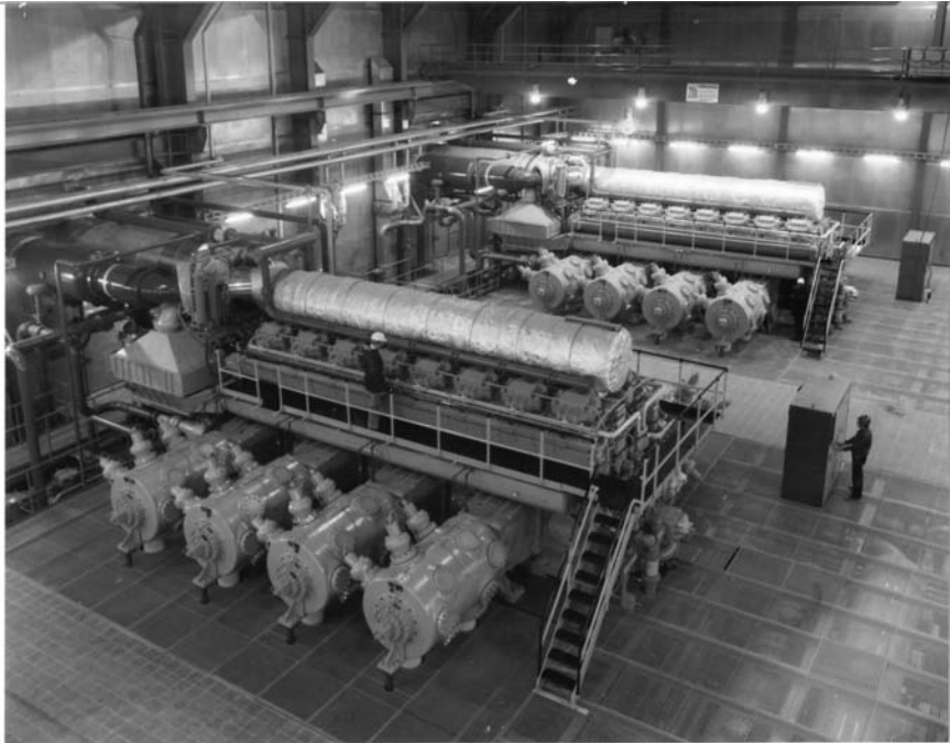
Figure 1-3. Cooper-Bessemer Z-330 Integral Engine Compressors in Krunhörn, Germany. Courtesy of Ben Suurenbroek (Retired Cooper Energy Services)
