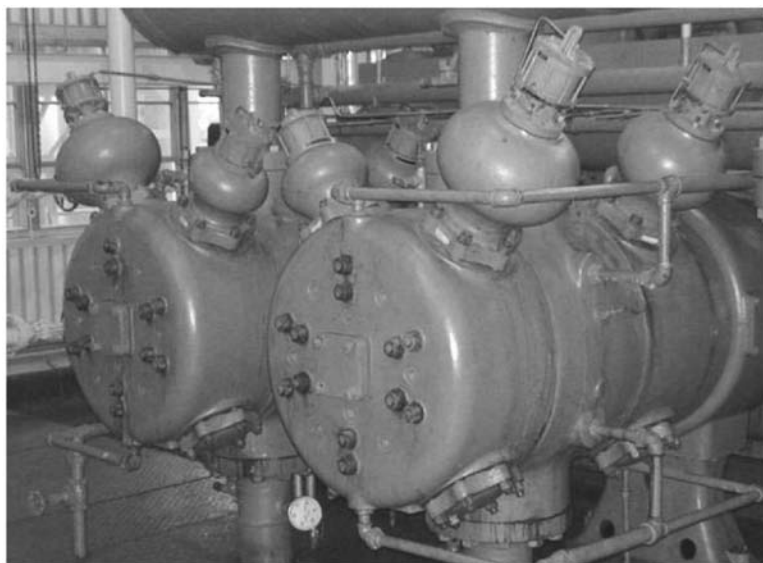
Figure 13-13. Original OEM 1100 psig (75.8 bar) valve-in head type cylinders.
