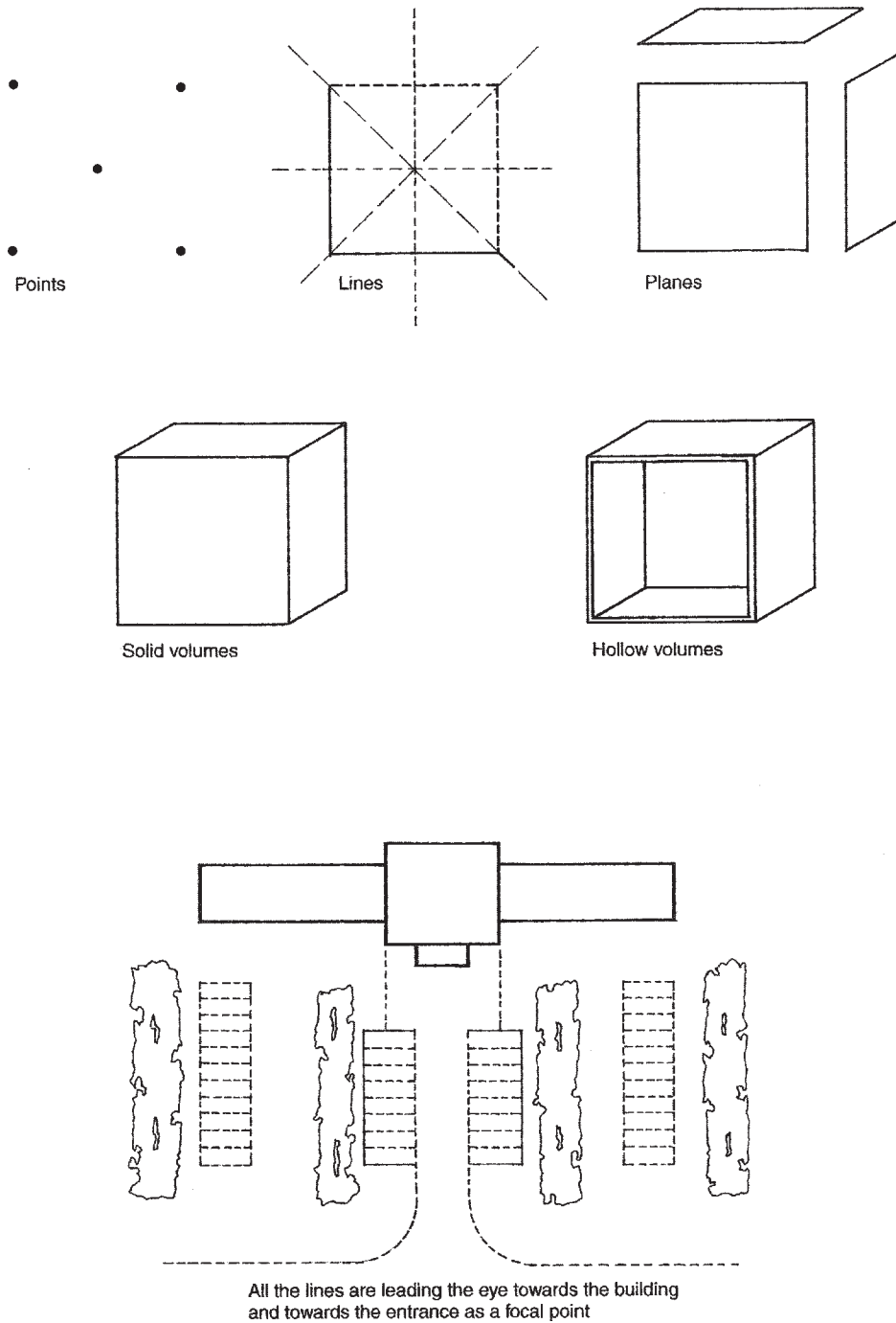
Figure 10.3 Points, lines, planes and volumes.
