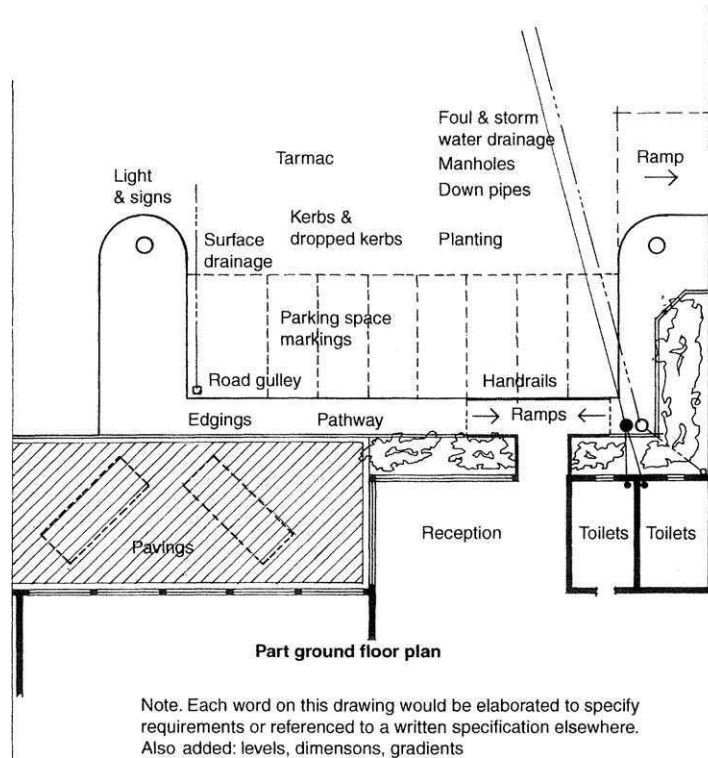
Figure 11.1 A site plan construction detail.
