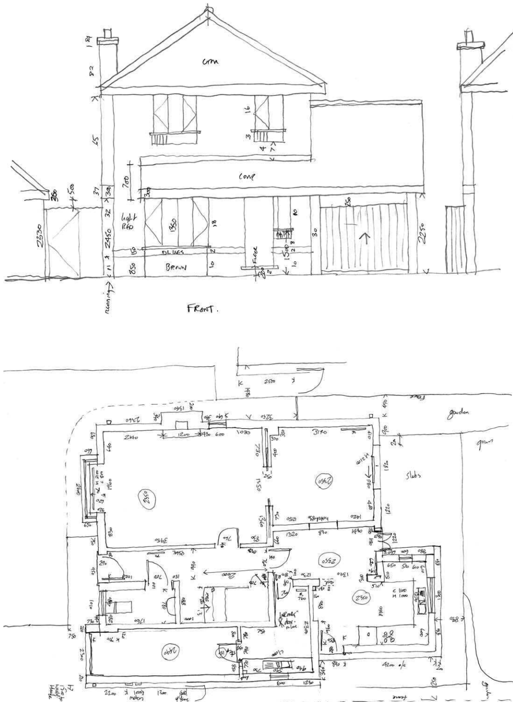
Figure 3.1 Survey drawings.
