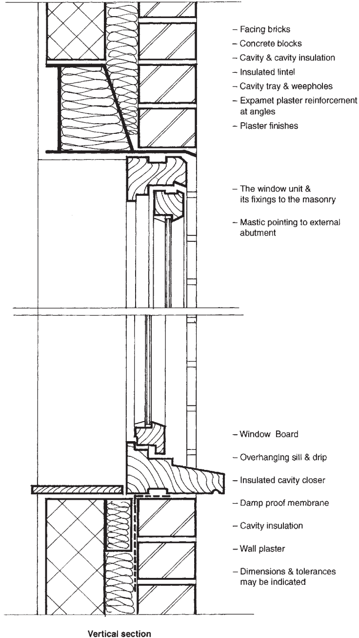
Figure 11.4 An assembly detail.
