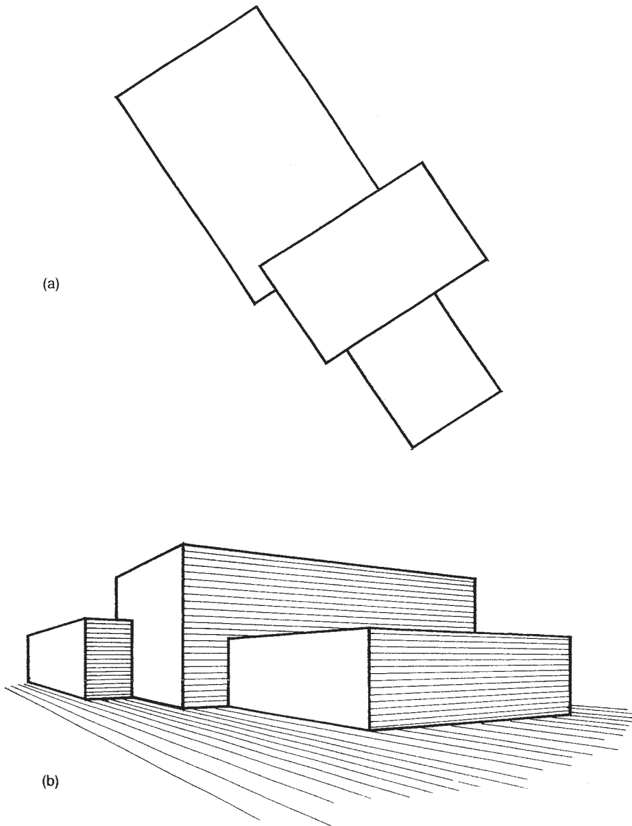
Figure 3.7 A Perspective drawing. (a) The floor plan aligned with the angle of view. (b) The building as it would actually be seen.
