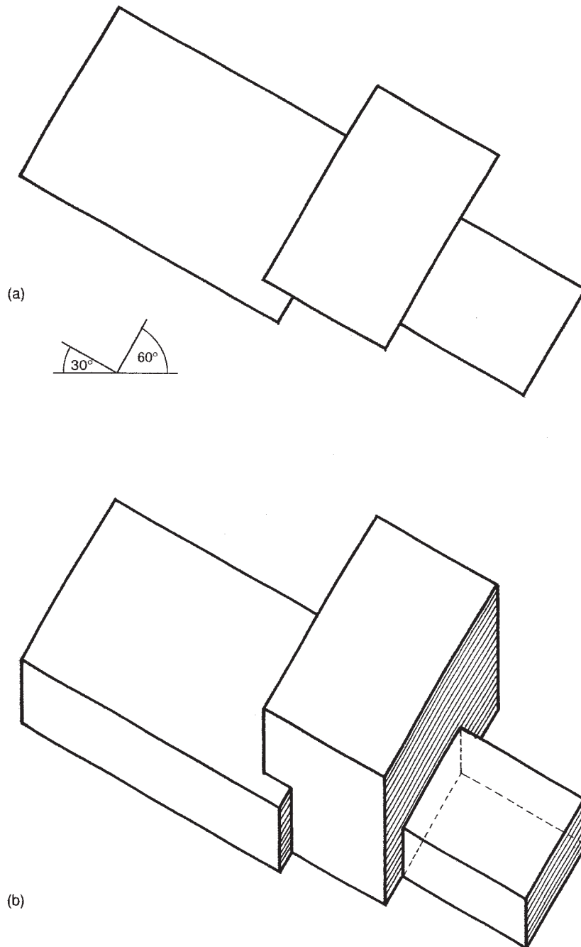
Figure 3.8 An axonometric projection. (a) The floor plan. (b) The 'hidden' construction lines are removed to create a 3D appearance.
