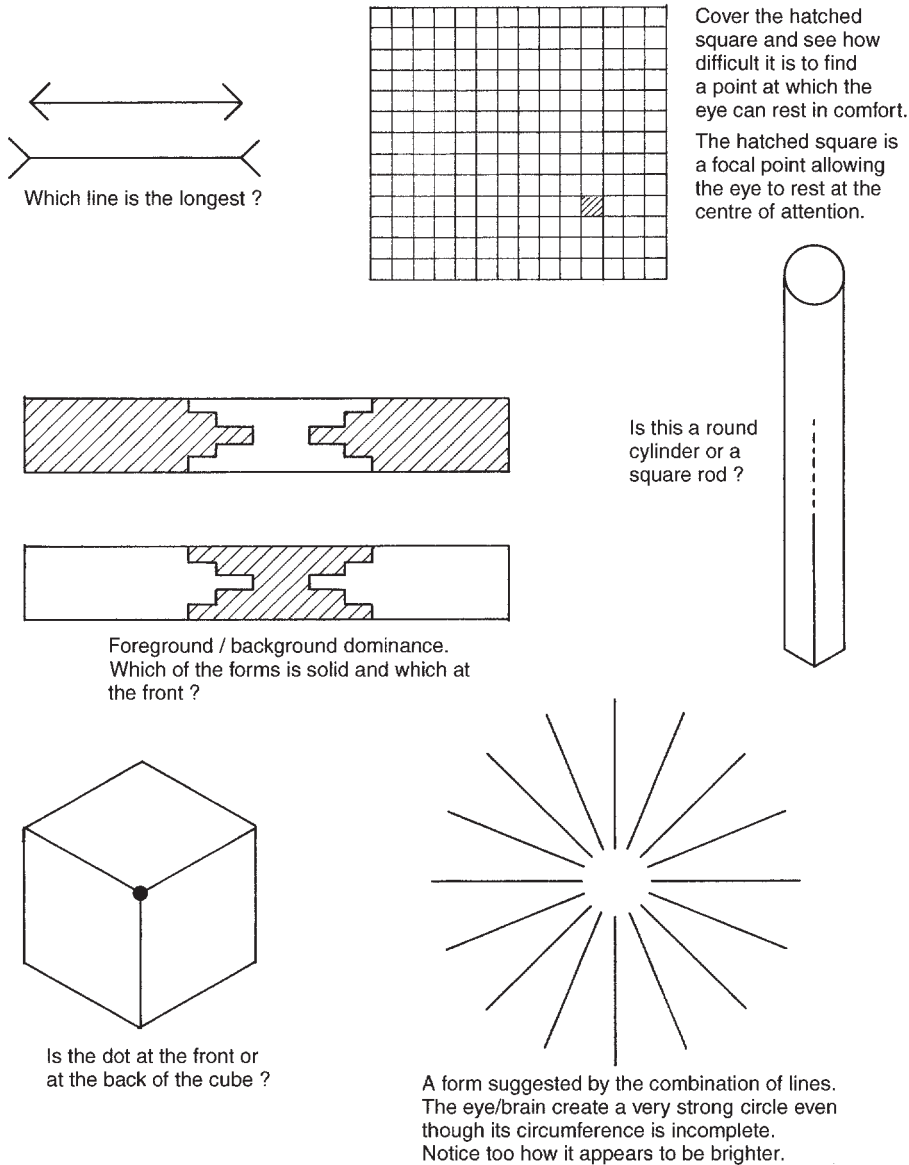
Figure 10.1 Optical effects.
