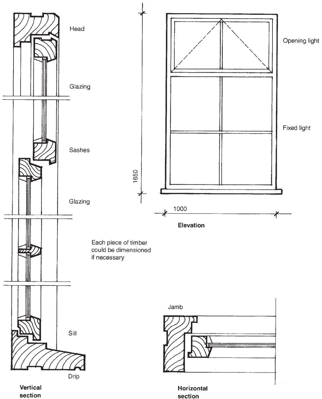
Figure 11.3 A component detail.
