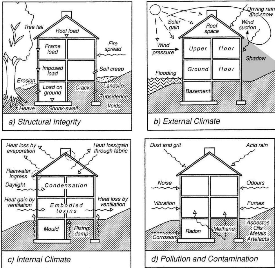
Figure 4.2 Building Control constraints. Diagrams courtesy of Andrew Golland, taken from Housing Development: Theory, process and practice , Edited by Andrew Golland and Ron Blake.
