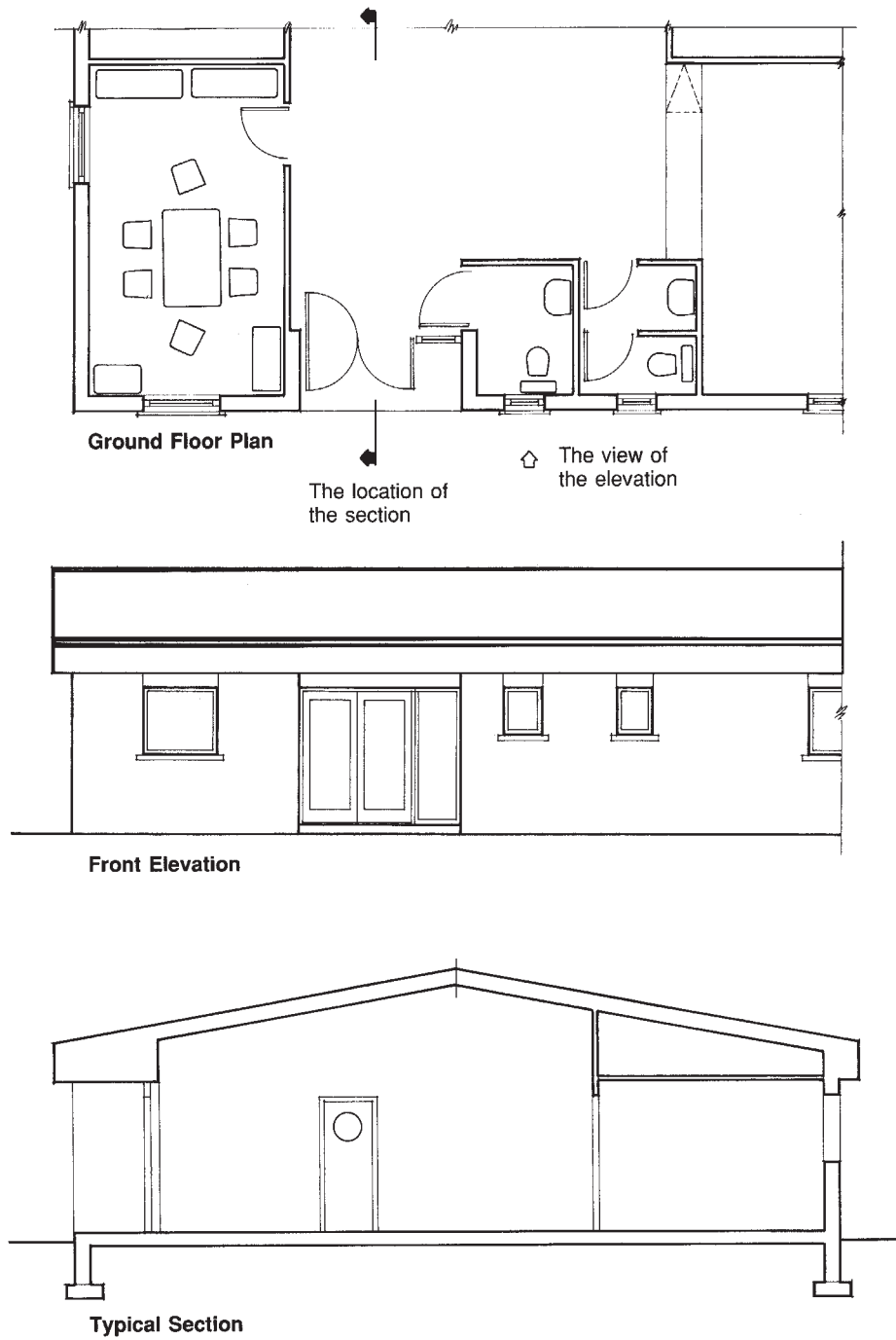
Figure 3.6 Plans, elevations and sections.
