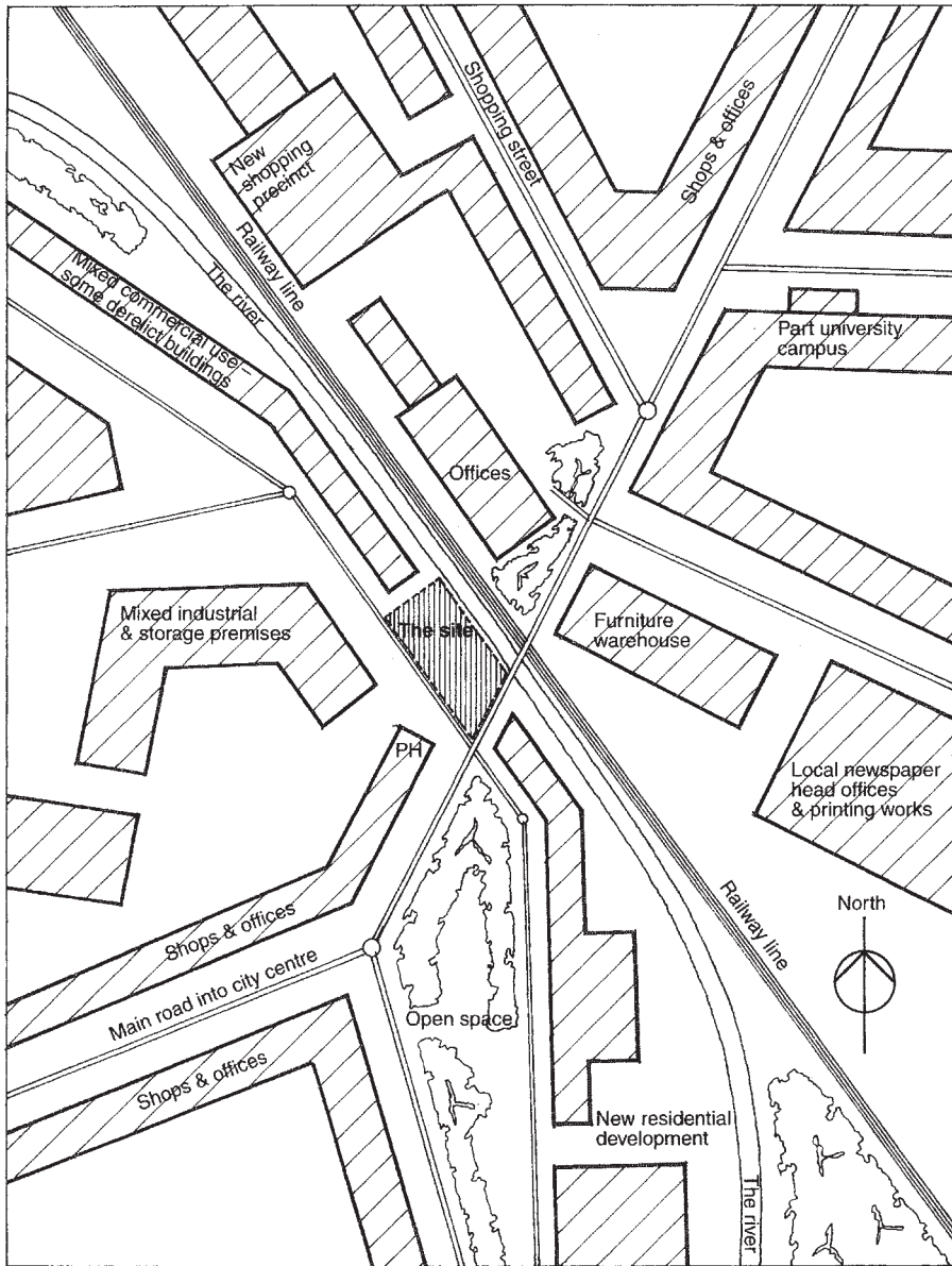
Figure 5.3 The site in the context of its locality.
