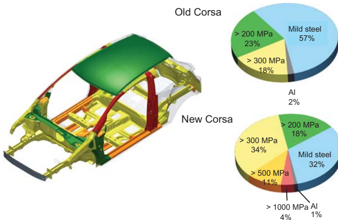
Fig. 2.6 Material distribution of body-in-white – new versus old Opel Corsa.
