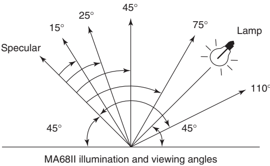
Fig. 6.7 Observation angles in a specific device for effect color measurement (source: X-Rite).
