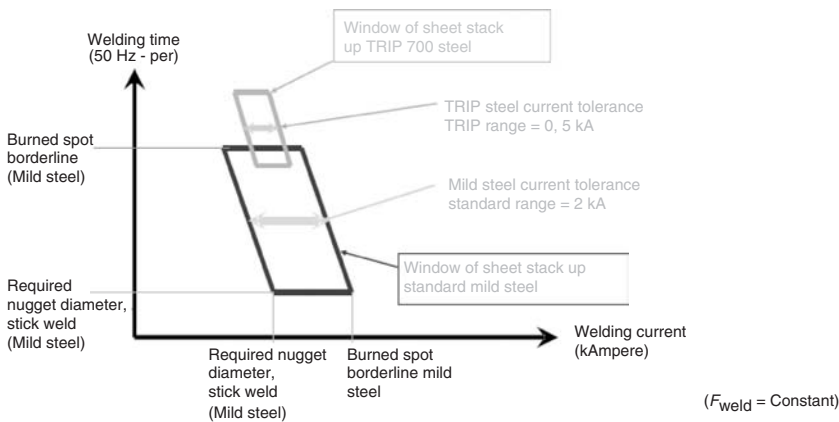
Fig. 2.9 Spot welding resistance of high-strength steel.
