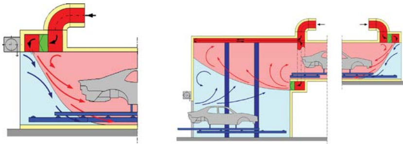
Fig. 8.26 Design of oven air seals: horizontal entry (a), A-type (b).
