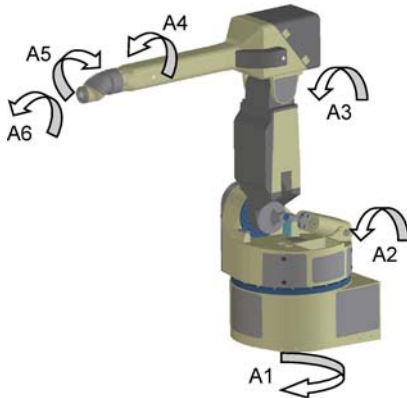
Fig. 8.10 Movement axes of a painting robot.
