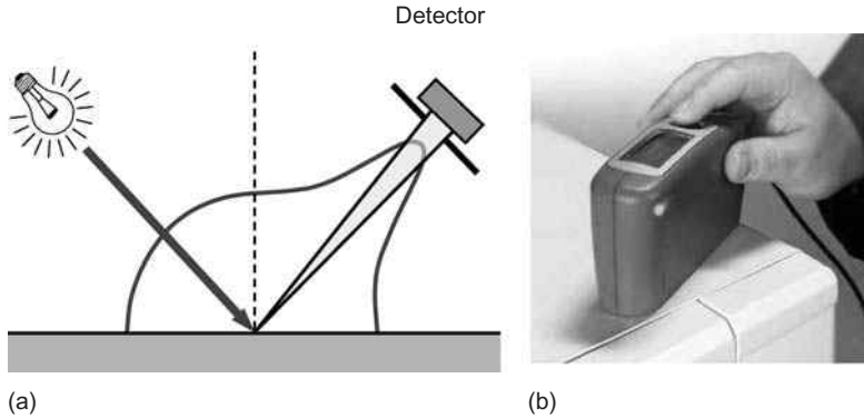
Fig. 12.3 Schematic diagram of a glossmeter (a) and a glossmeter, 'micro-TRI-gloss' (b) (source: Byk-Gardner).
