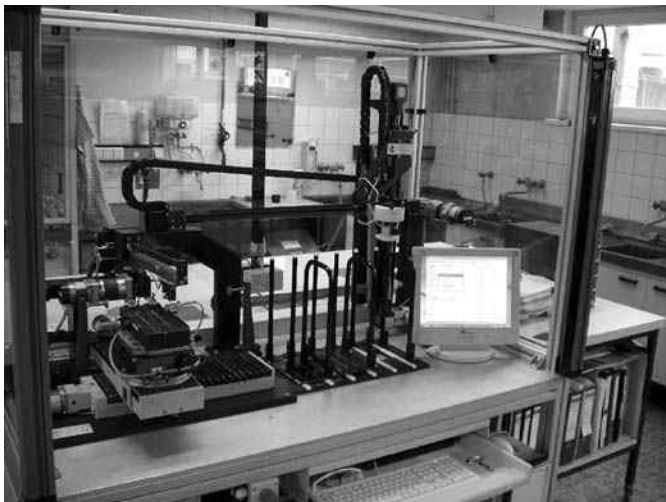
Fig. 12.67 Fully automatic cross-cut equipment (source: DuPont Performance Coatings).
