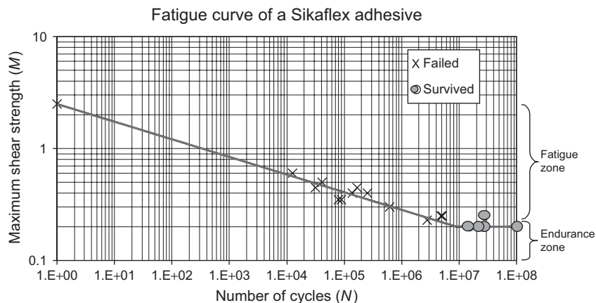
Fig. 10.19 Woehler diagram of an elastic adhesive (Sikaflex, Sika).
