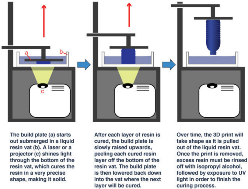
Figure 5-1. The SLA printing process (infographic by Jeff Hansen, HoneyPoint3D™)
