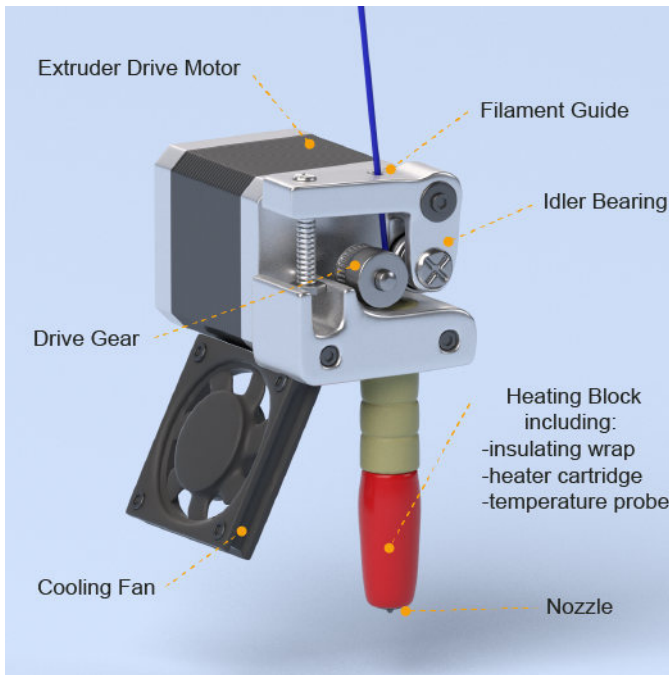
Figure 4-13. Labeled diagram of extruder components (information by Jeff Hansen, HoneyPoint3D™)
