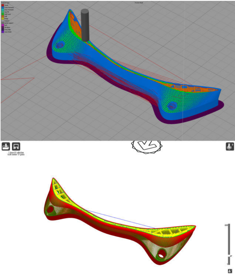
Figure 4-26. Comparison of tool paths between Simplify3D (top) and Cura (bottom)
