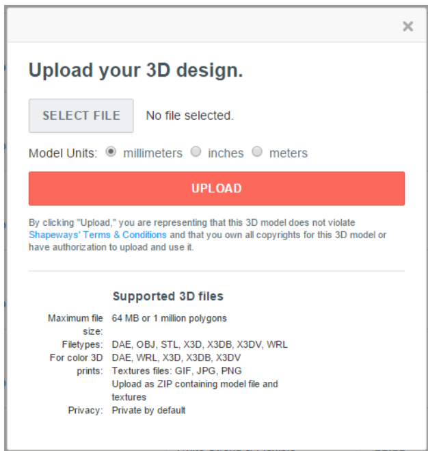
Figure 8-6. File upload dialog from Shapeways.com prompting user to define unit of measurement. Note the maximum file size of 1 million polygons. The bunny had just over 10,000 polygons.
