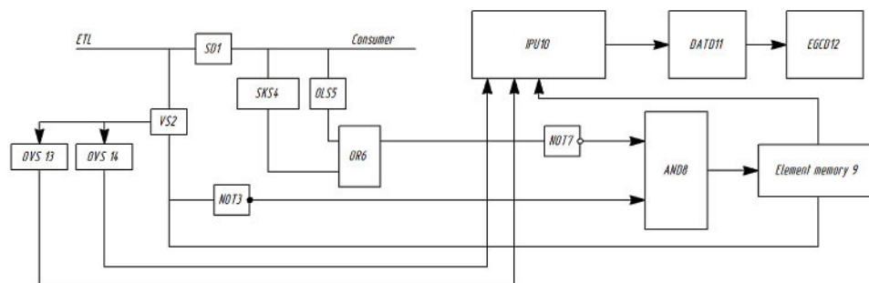
Figure 7. The device for monitoring the number and duration of power supply outages and monitoring the level of voltage deviation at the consumer inputs
