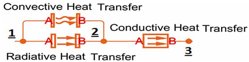
Figure 38. The model diagram. 1 - the source data (ambient temperature, solar radiation), 2 - the point of interaction laws of CvHT and RHT, 3 - heat transfer by conduction through a layer of material (from copper plate to pipe see Figure 34).
