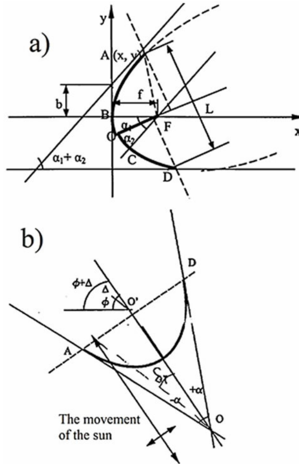
Figure 8. The geometry of the ideal profile of the U-shaped concentrator: a) asymmetric profile; b) symmetrical profile
