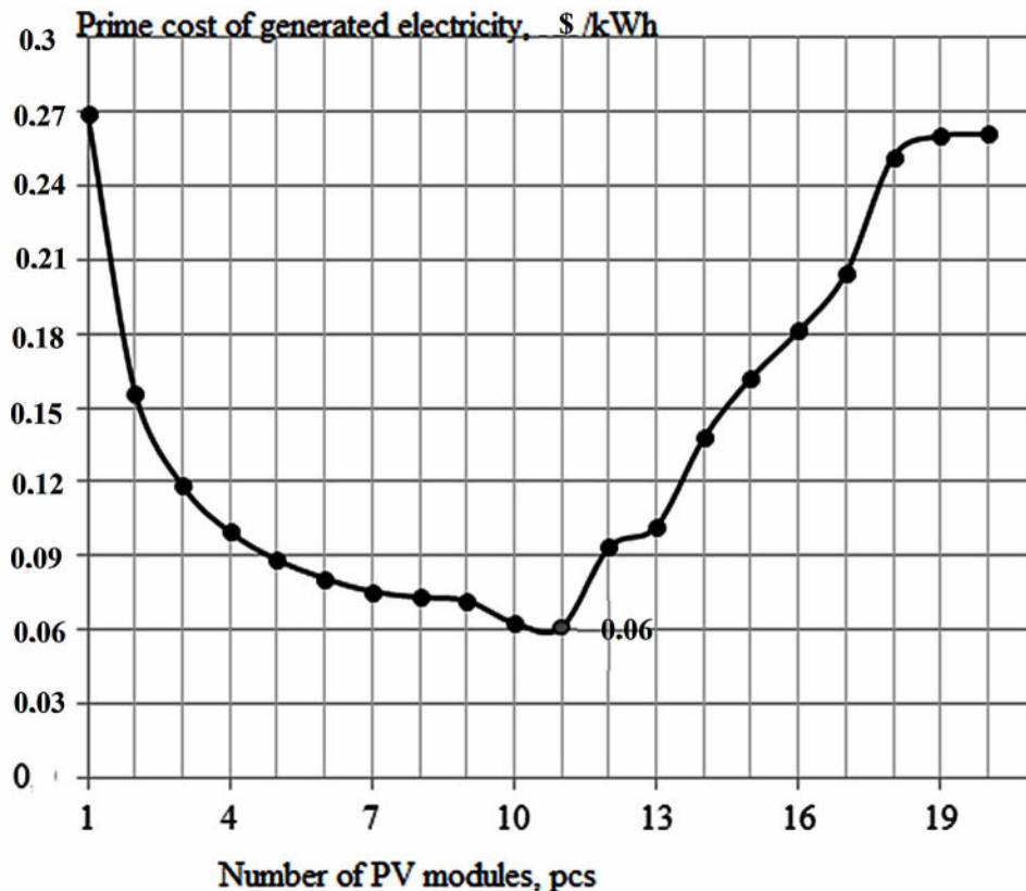
Figure 13. The dependence of the cost of generated electrical energy on the number of photovoltaic modules used in the solar power plant
