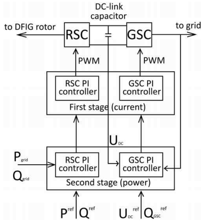
Figure 2. Control signals to RSC and GSC
