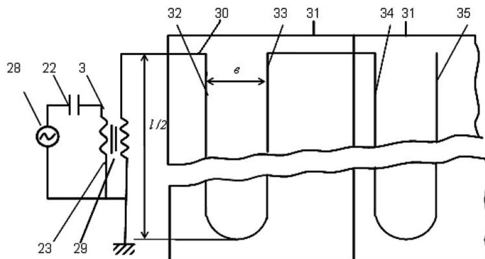
Figure 17. Contactless power supply system with two conductor segments of the same single-conductor line under each traffic row
