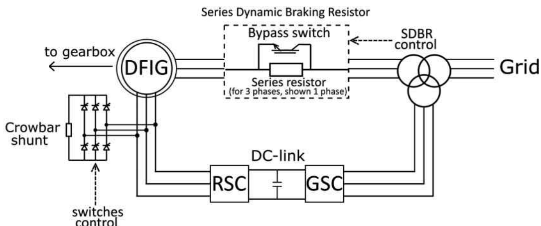
Figure 7. Example of DFIG protection schemes connection: crowbar, DC chopper, SDBR in the stator side
