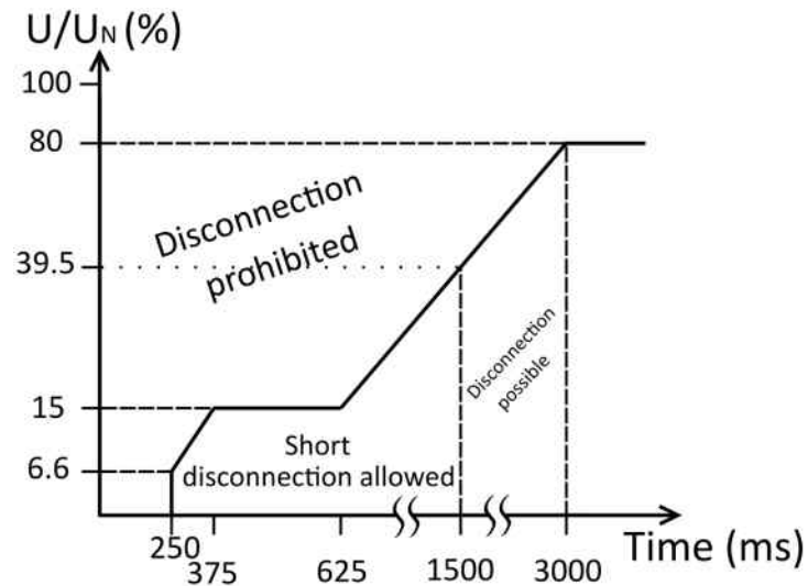
Figure 1. LVRT grid code requirements for wind turbines
