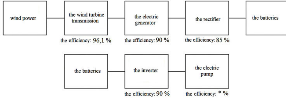
Figure 14. The structural flow chart of a wind electrical station with the electrical pump.
