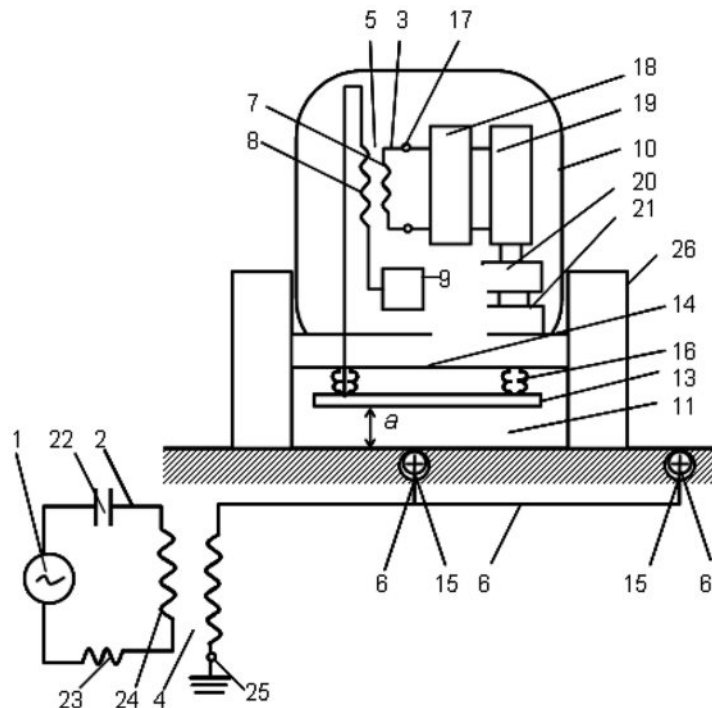
Figure 14. Apparatus for contactless power supply to electric vehicles
