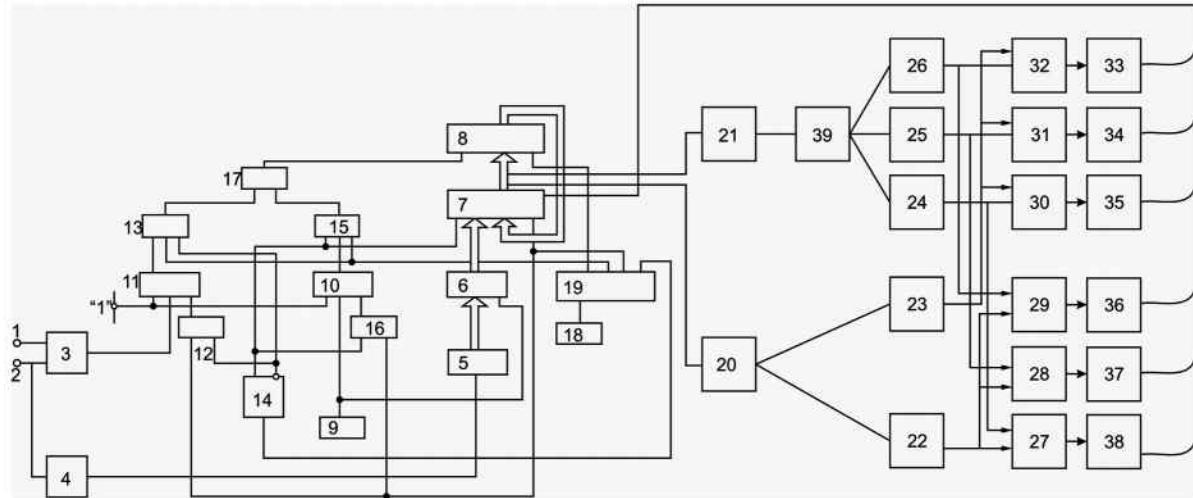
Figure 10. The block diagram of the device for accounting electricity consumption and adjusting the cost of consumed electricity depending on its quality, the source of distortion and the time of power quality indicators distortion
