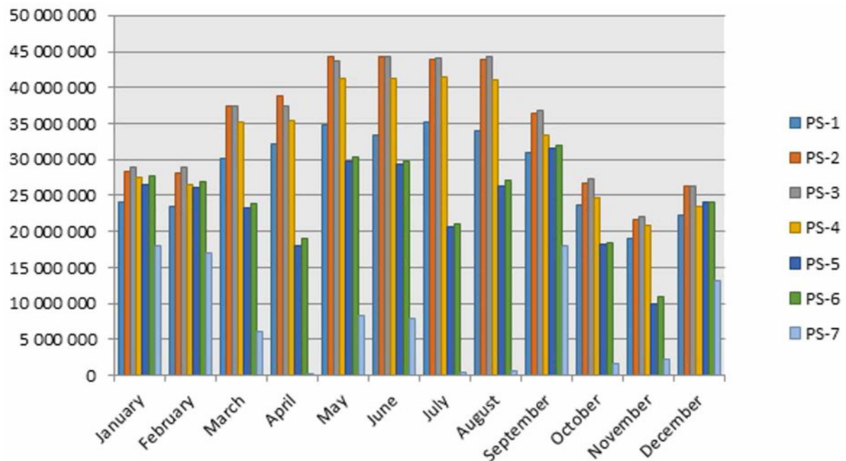
Figure 1. Comparison of the actual energy consumption of pumping stations N°N° 1 ÷ 7 KMK for 2013, kWh
