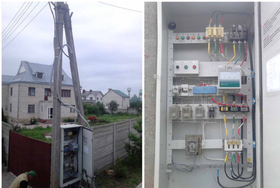
Figure 10. Appearance of SP installed in the Mezenka settlement
