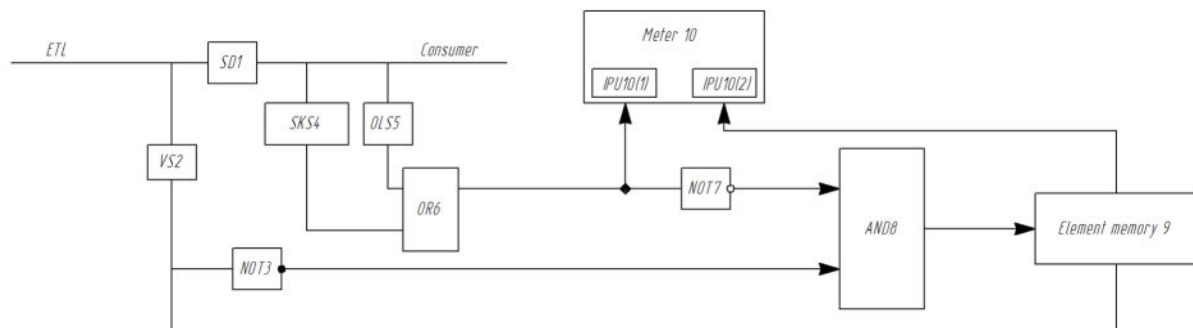
Figure 1. The device for recording the number and duration of outages
