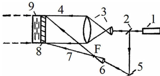
Figure 14. Principle of formation of holographic lenses
