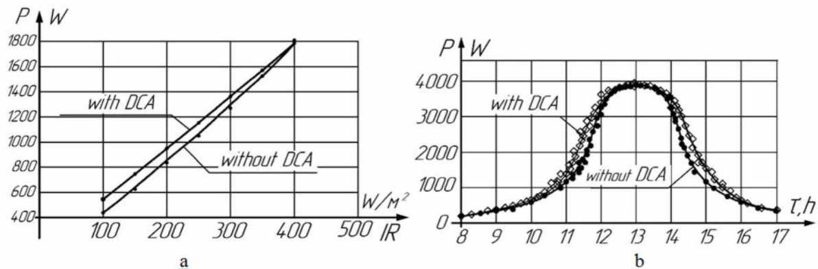
Figure 18. Output power of a uniformly shaded array of modules (a - on the intensity of radiation in the shadow, b - during the light day)
