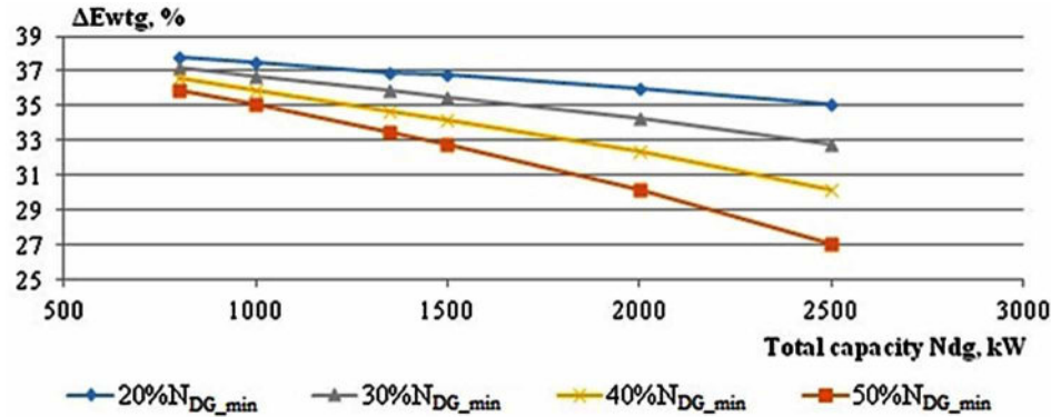
Figure 13. Dependence of the share of WPP penetration on the DG unit installed capacity and the DG minimum load limitation
