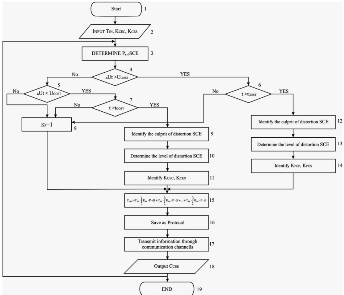
Figure 9. The algorithm of the functional unit, which allows to adjust the cost of consumed electric energy in case of non-compliance with its specified parameters
