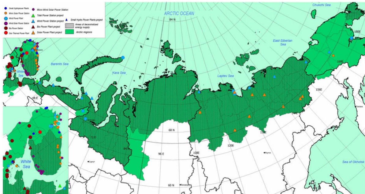
Figure 1. Renewable energy power installations in the Russian Arctic (Morgunova and Solovyev, 2017; GIS, 2018)
