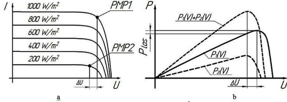
Figure 9. Current-voltage (a) and power (b) characteristics at different illumination PEC
