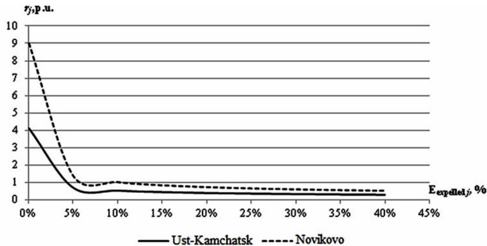
Figure 8. The approximating dependences of r_j on E_{expelled_j} according to the data of WDC of the village of Novikovo and the settlement of Ust-Kamchatsk
