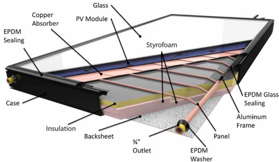
Figure 26. HSP – Power Therm-cross-section (Solimpeks, n.d.)
