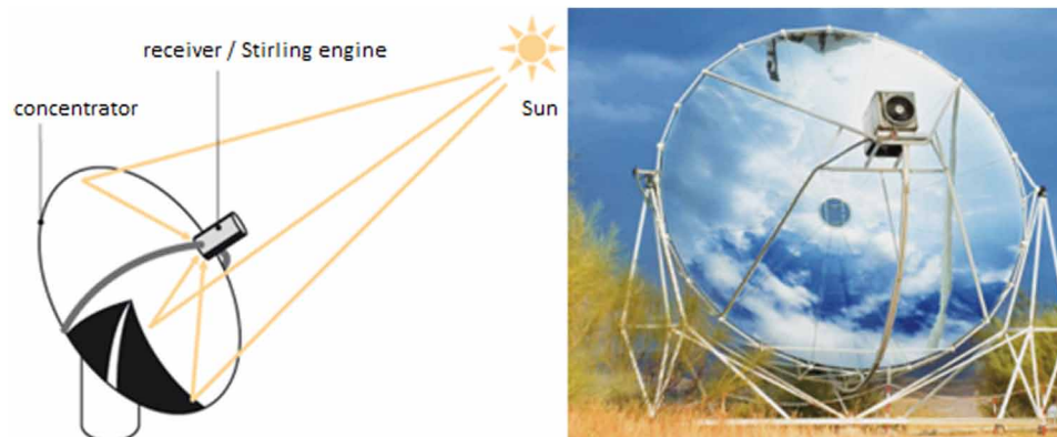
Figure 3. A parabolic solar dish concentrator
