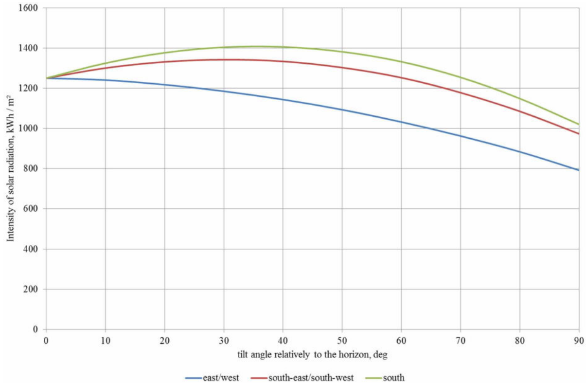
Figure 4. Dependence of the intensity of solar radiation coming on the receiving surface on its inclination angle with respect to the horizon with its different orientations to the sides of the world
