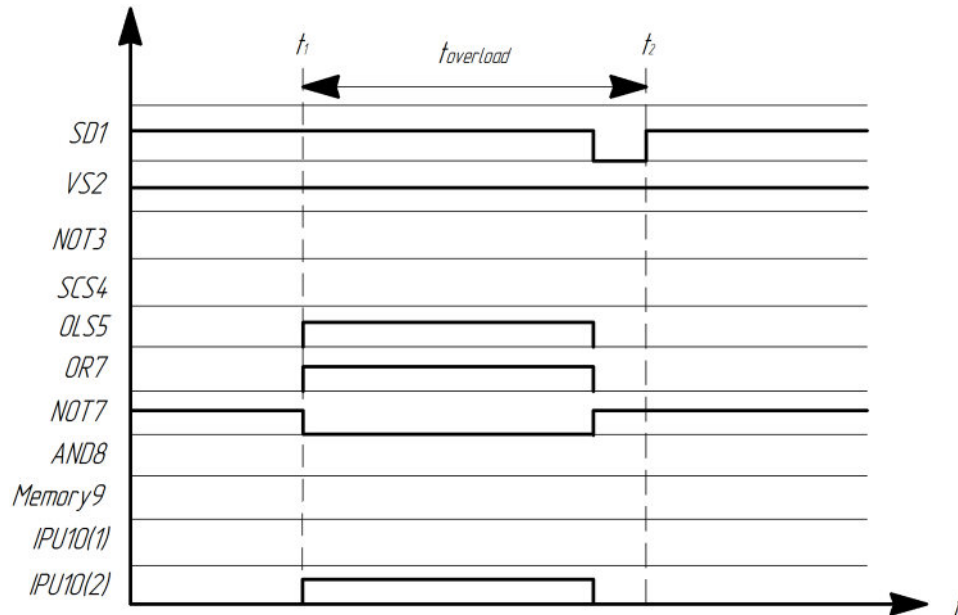
Figure 5. Diagram of signals at the element outputs shown in Figure 1 when the consumer network is overloaded
