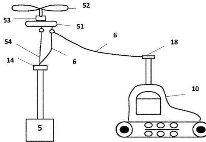
Figure 11. Apparatus for electric power supply using a gas-filled balloon with a propeller driven by a motor
