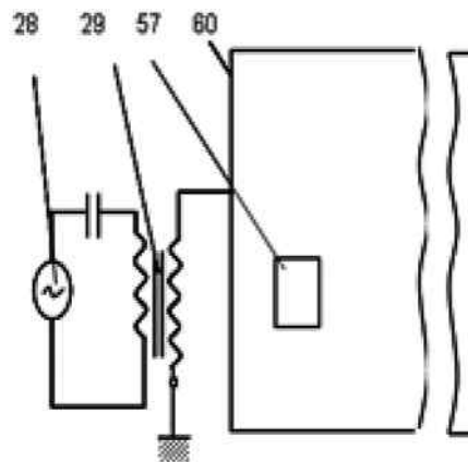
Figure 26. Insulated metal film on the ground surface
