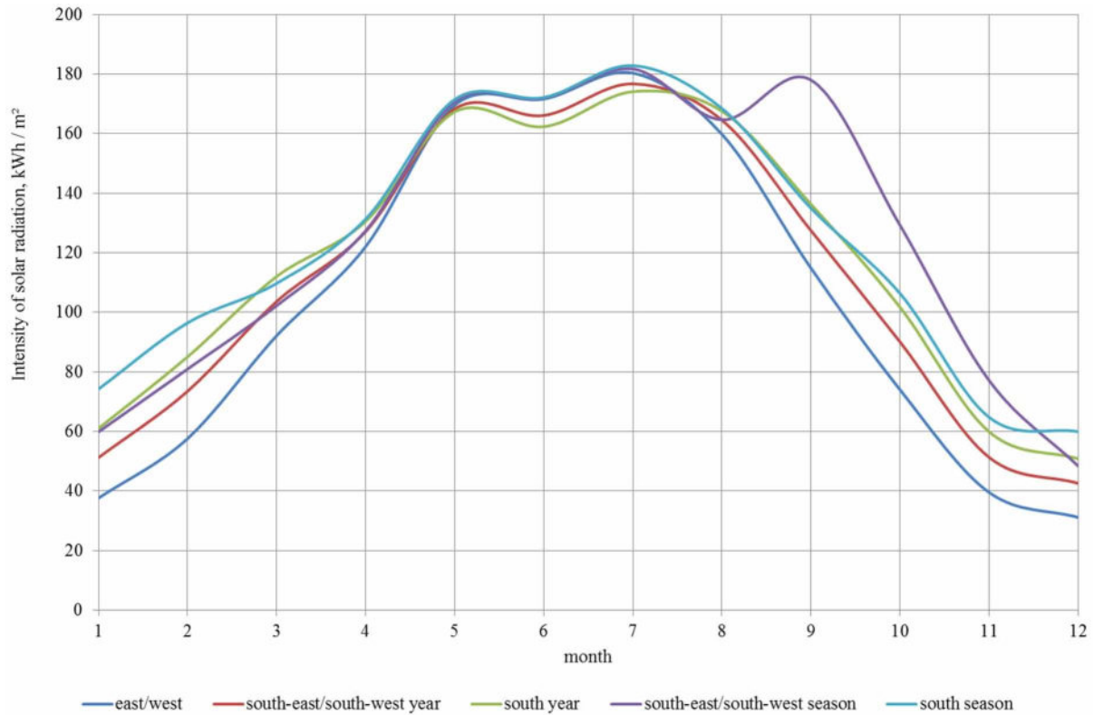
Figure 6. Monthly sums of total solar radiation for the optimal angle of inclination relatively to the horizon receiving surface of different spatial orientation
