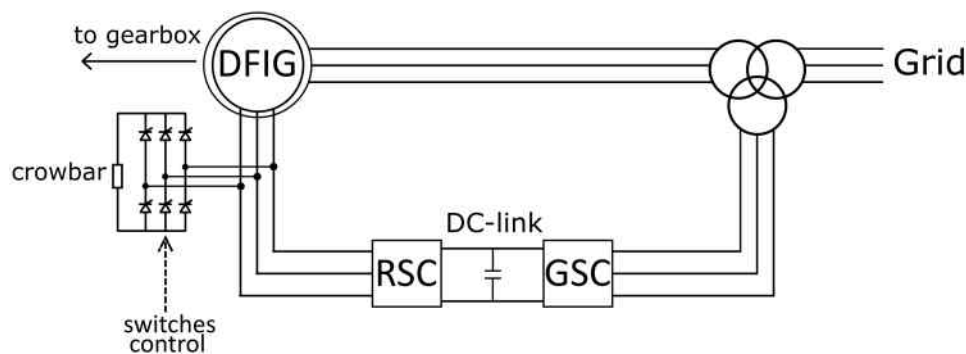
Figure 4. Crowbar in rotor circuit
