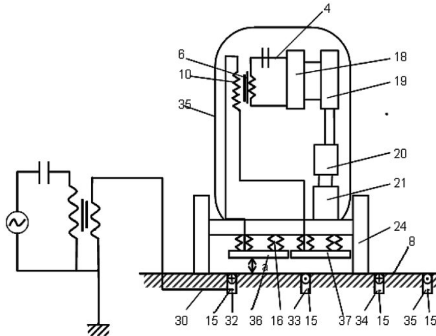
Figure 18. The vehicle with capacitive couplers under the bottom and two line segments
