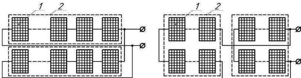
Figure 4. Options for switching photovoltaic modules a - row; b – block; (1 - photoelectric module, 2 - array of modules)
