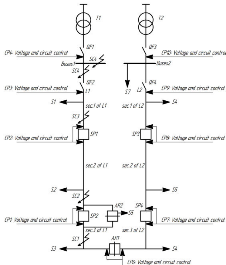
Figure 9. The method of the joint application of sectioning and redundancy means
