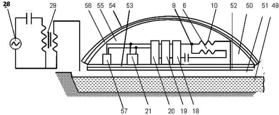
Figure 22. Apparatus for supplying power to an air-cushion vehicle
