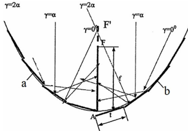
Figure 9. Facet surface of U-shaped parabolic concentrator: a) according to the ideal profile; b) the tangent to the ideal profile (calculated) profile
