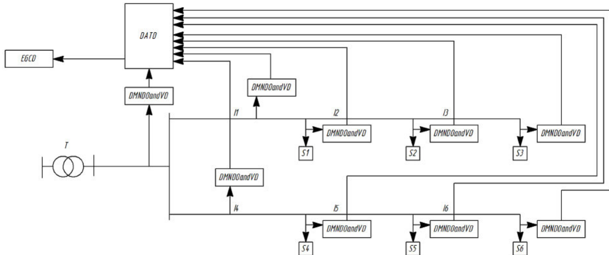
Figure 8. Implementation of a system for monitoring the power quality and power supply reliability on the example of the 0.38 kV outgoing line
