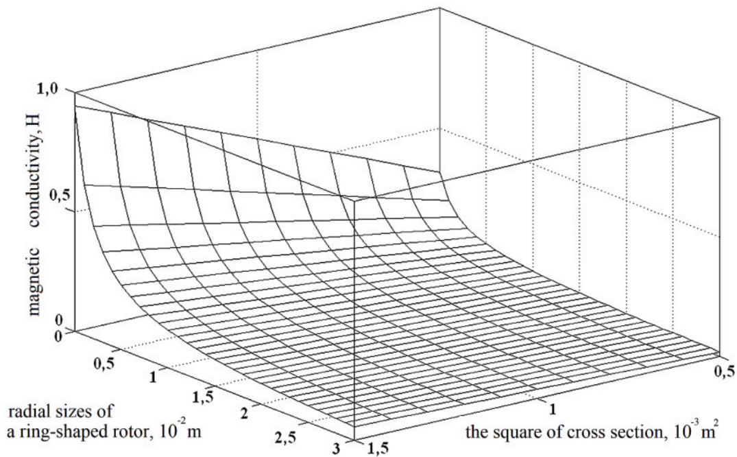
Figure 7. The influence of radial sizes of a ring-shaped rotor and the square of cross section of a ferromagnetic element on the value of magnetic conductivity of a circuit
