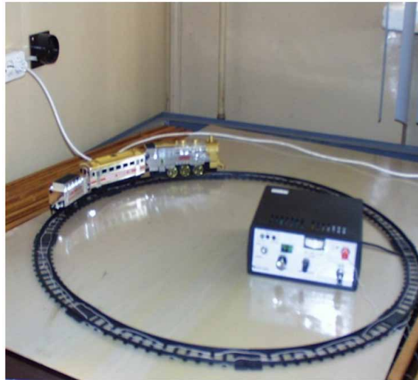
Figure 27. Model of an electrified railroad powered by a resonant single-conductor system
