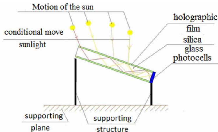
Figure 25. Scheme of operation of the holographic battery
