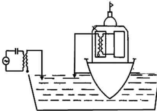
Figure 29. Diagram of the launch model powered through water medium used as a single-conductor circuit
