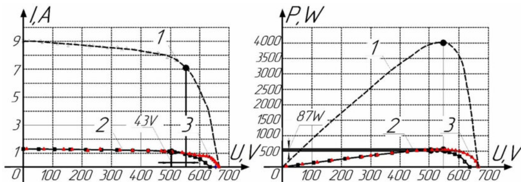
Figure 16. Experimental characteristics of an array of photovoltaic modules (1 - without shading, 1 - with partial shading and in-line vertical switching, 3 - with partial shading, in-line vertical switching with DCA)
