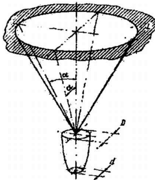
Figure 7. The field of view of focon with a parametric angle \alpha
