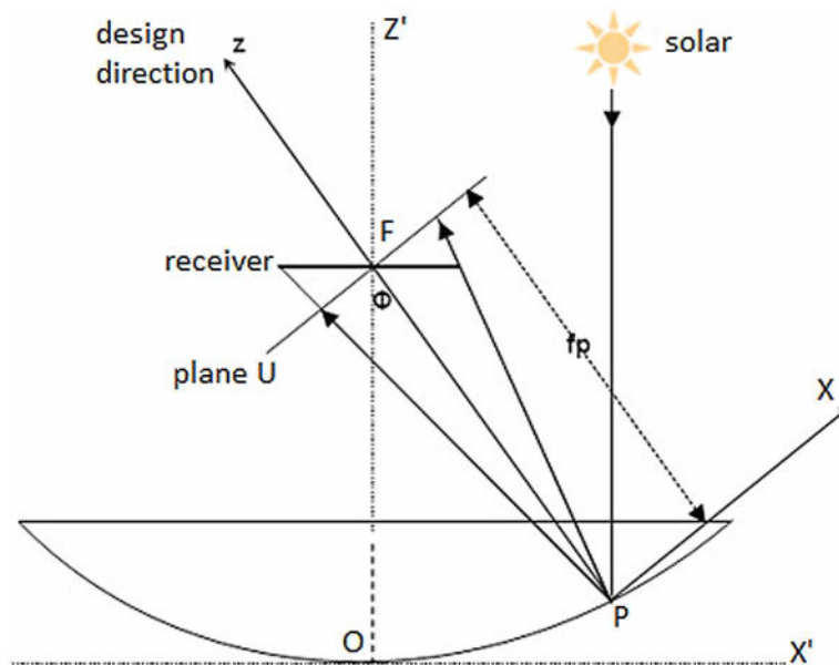
Figure 2. Operational scheme of parabolic concentrator
