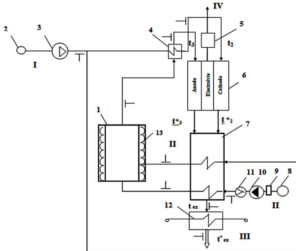
Figure 1. Schematic diagram of mini-CHPP on products of air conversion of motor diesel fuel and electrochemical generator: 1 - catalytic burner; 2 - air pipe; 3 - compressed-air blower; 4 - synthesis gas cooler; 5 – electrical customer; 6 - electrochemical generator based on SOFC; 7 - waste-heat boiler-utilizer; 8 - motor diesel fuel manifold; 9 - fuel filter; 10 - fuel pump; 11 – flow-sensing element; 12 – network heater; 13 - thermal insulation I- air input; II - motor diesel fuel input; III - output of combustion products; IV- electrical power output.
