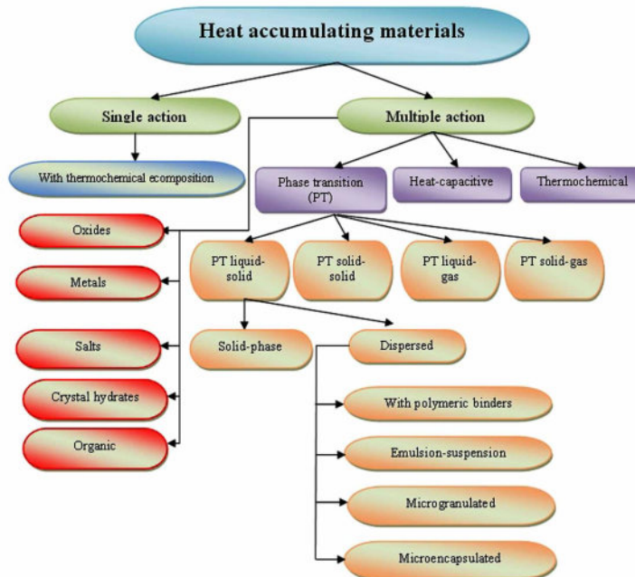
Figure 4. Classification of heat-storage materials
