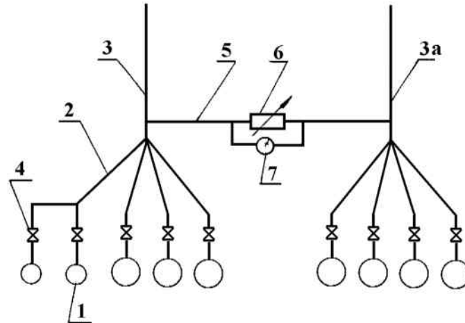
Figure 3. The scheme of connection of pressure pipelines with the bypass device: 1 – pump units; 2 – individual pressure pipelines; 3 and 3-a – the general pressure pipelines; 4 – butterfly valves; 5 – bypass device; 6 – throttle device; 7 – differential manometer
