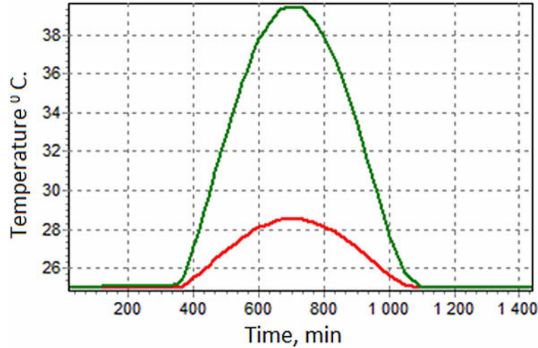
Figure 35. Temperature dynamics of the heated and coldest solar panel modules per day at an input water temperature of 25 °C
