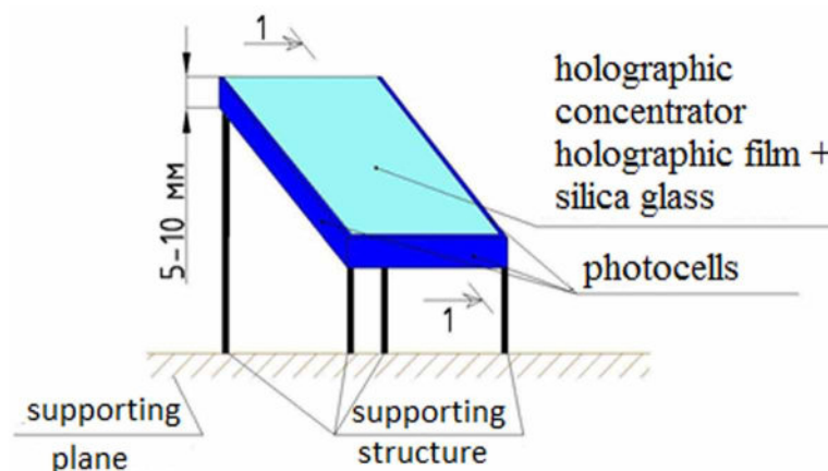
Figure 23. Holographic photovoltaic battery
