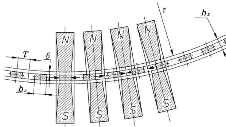
Figure 5. The design of the configuration of the part of a magnetic circle of an arc-shaped wind and electrical generator with a ring-shaped rotor
