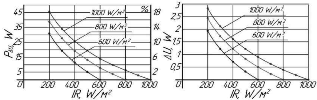
Figure 13. Graphs of the dependence of losses of a photoelectric installation with mixed connection PEC and uniform partial shading on the radiation intensity in the shadow and setting the MPPT to the local maximum point for different illumination: a - loss from inconsistency in voltage, b - mismatch voltage
