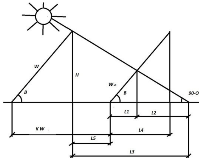
Figure 8. Geometric model for determining the length of the shadow from the photoelectric module
