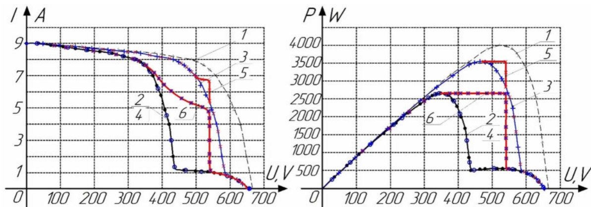
Figure 19. Experimental characteristics of an array of photovoltaic modules (1 - without shading, 2 - with partial shading and block vertical switching, 3 - with partial shading and block horizontal switching, 4 - with partial shading and in-line horizontal switching, 5 - with partial shading, horizontal block switching and DCA, 6 - with partial shading, horizontal in-line, or block vertical switching with DCA)
