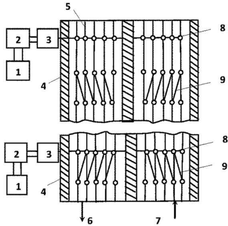
Figure 2. Power supply system for single-trolley electric vehicles
