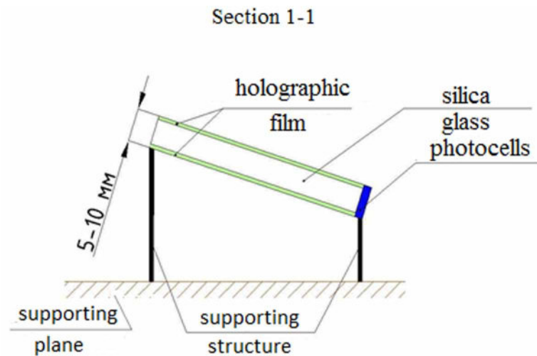
Figure 24. The holographic photovoltaic battery in a section
