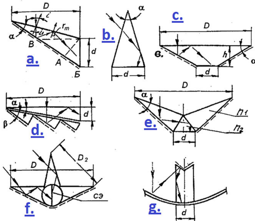
Figure 5. Main types of prismatic concentrators; a) prismatic on the basis of the oblique triangular prism, b) vertical triangular, c) on the basis of a trapezium, d) compound prism, e) with a central deflecting prism, f) for thermal collectors, g) prismatic as a secondary concentrator
