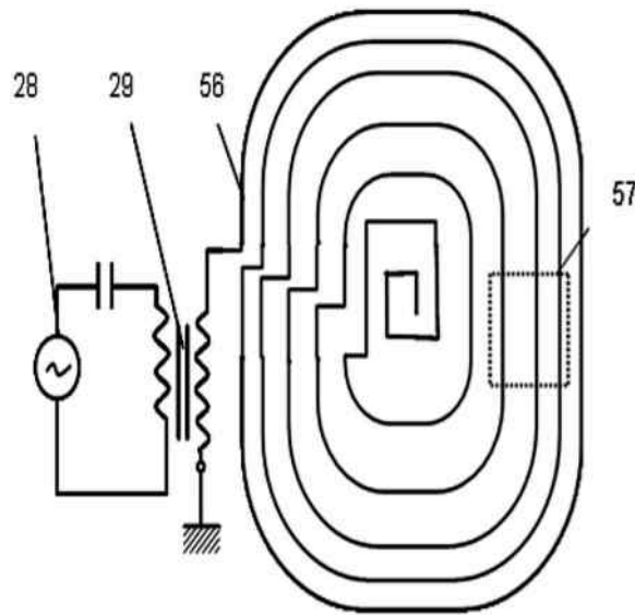
Figure 23. The spiral – shaped insulated conductor connected to Tesla transformer
