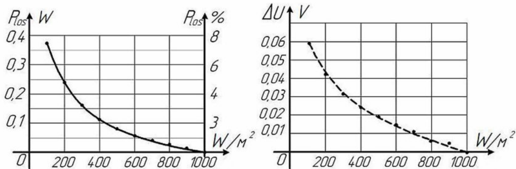
Figure 10. Plots of power loss (a) and voltage difference (b) PEC of radiation intensity
