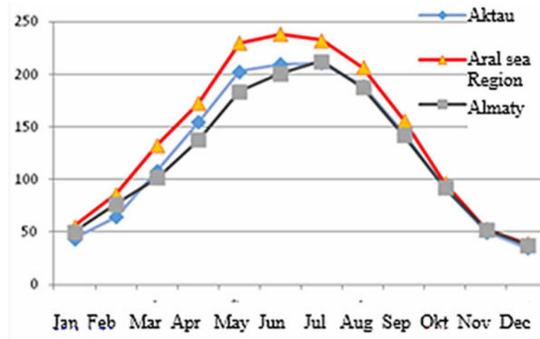
Figure 7. Average monthly daily sum of total solar radiation incident on horizontal plane surface
