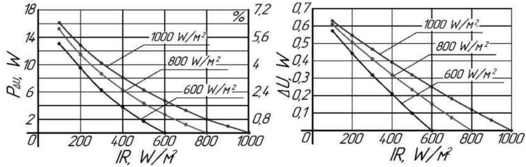
Figure 12. Graphs of the dependence of losses of a photoelectric installation with mixed connection PEC and uniform partial shading on the radiation intensity in the shadow and setting the MPPT to the absolute maximum point for different illumination: a - loss from inconsistency in voltage, b - mismatch voltage
