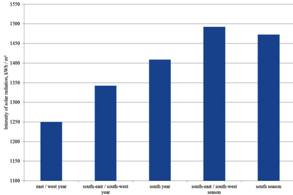
Figure 7. The annual sums of total solar radiation for the optimal angle of inclination relatively to the horizon of the receiving surface of different spatial orientations
