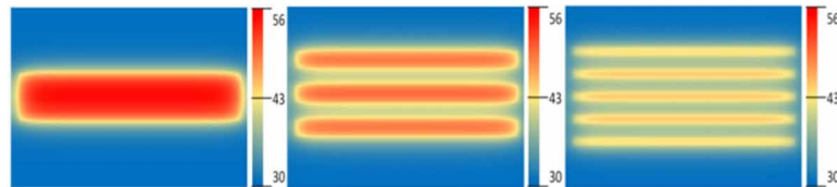
Figure 21. Model derived heat maps at the solar cell layer for an EPV of 800 \text{ Wm}^{-2} and a heat transfer of 15 \text{ Wm}^{-2} for the glass surfaces for the test coupon configurations. The color scales varies from 30C (light blue) to 56C (bright red).
