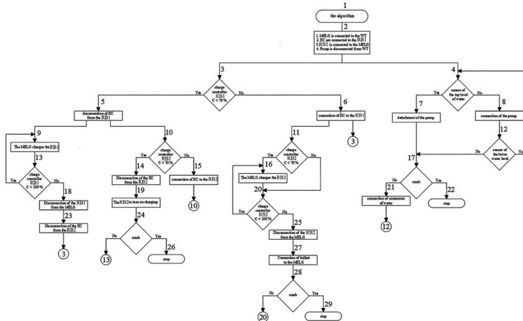
Figure 11. The algorithm of autonomous functioning of an electrical and technical system of a combined electrical and water supplying wind turbine
