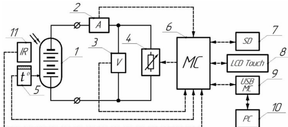
Figure 15. Structure of the IMC (1 - photovoltaic system; 2 - current sensor; 3 - voltage sensor; 4 - special adjustable load; 5 - solar cell temperature sensor and OS; 6 - microcontroller; 7 - electronic storage device; 8 - LCD TFT Touch Screen; 9 - interface microcontroller; 10 - personal computer; 11 - light sensor)
