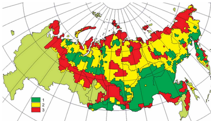
Figure 4. Risk map for buildings and structures in the permafrost zone: 1 - weak, 2 - medium, 3 - high risk (Anisimov and Reneva, 2006)
