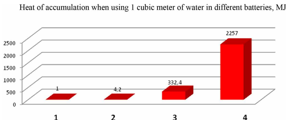
Figure 7. Comparison of the amount of heat accumulated by water in different types of HA (1. Hydro accumulating electric power station, V = 1 \text{ m}^3 ; 2. Capacitive battery, V = 1 \text{ m}^3 , \Delta t = 1.0 \text{ }^\circ\text{C} ; 3. Phase-transfer battery of heat (solid - liquid), V = 1,0 \text{ m}^3 ; 4. Phase-transfer battery of heat (liquid-gaseous, at t = 100 \text{ }^\circ\text{C} ), V = 1,0 \text{ m}^3 ).
