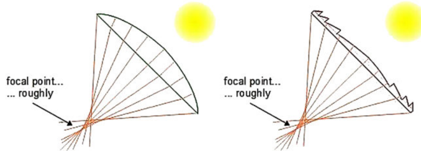
Figure 4. Principles of formation of the working profile of Fresnel lenses to obtain the necessary irradiation in the focal point
