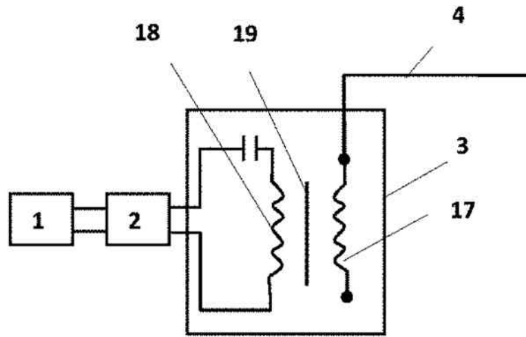
Figure 4. Block diagram of a power substation delivering electric energy to the contact system
