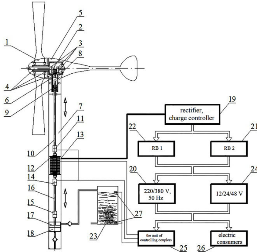
Figure 10. A basic functional-and-kinematic design of a combined electrical and water supplying wind station.
