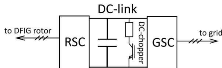
Figure 5. DC chopper in DC-link circuit
