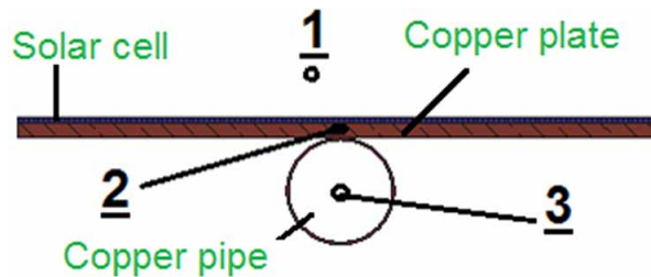
Figure 39. The cut view of the HSP section, which include solar cell, copper plate and pipe
