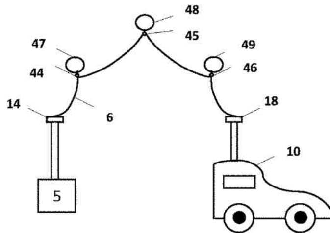
Figure 9. Apparatus for electric power supply with a flexible conductor suspended on three gas-filled balloons
