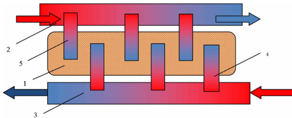
Figure 5. Construction of a thermal battery with heat pipes: 1 – HA with a granular matrix; 2 – collector with heated medium; 3 – collector-flue with heating medium; 4, 5 – respectively, heat supply and heat removal heat pipes
