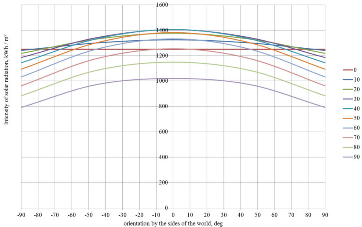
Figure 3. Dependence of the intensity of solar radiation coming on the receiving surface on its orientation to the sides of the world at different angles of inclination relatively to the horizon
