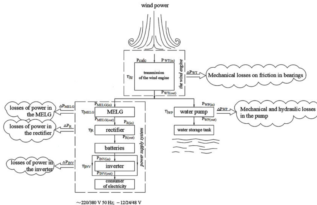
Figure 12. A structural and functional scheme of the balance of capacity of CEWWS
