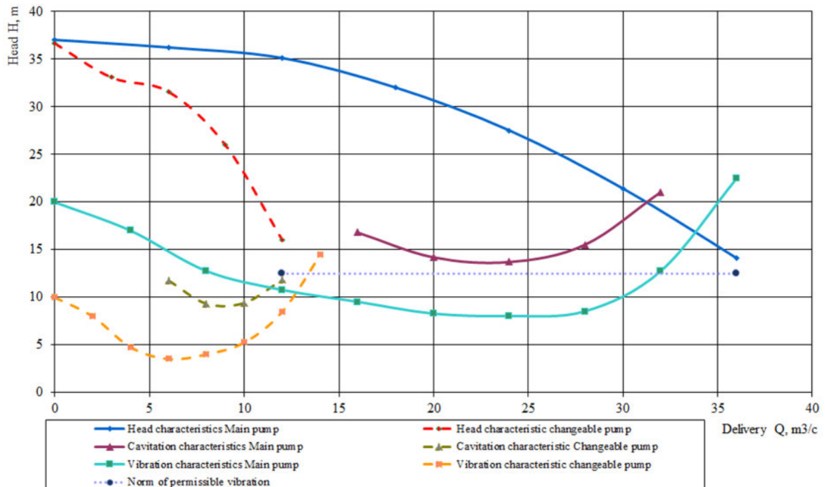
Figure 8. Pressure, cavitation and vibration characteristics of the main units 2400VR-25/25 and changeable units 1600V-10-40 NS No. 7 KMC according to test results
