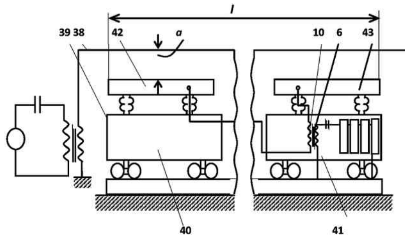
Figure 19. Contactless single-conductor power supply system for rail vehicles
