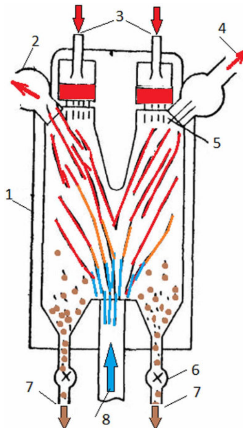
Figure 6. High-temperature heat exchanger with direct contact: 1 – heat-insulated wall; 2 – hot gas channel; 3 – supply of melt under pressure; 4 – hot gas outlet; 5 – partition with injectors; 6 – the throttle of pressure; 7 – exit of solid balls into an additional container; 8 – inlet of cold gas
