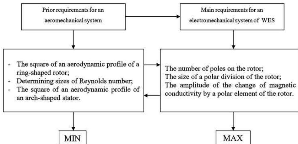
Figure 3. The chart of mutual dependency of different requirements for an aeromechanical and an electromechanical system
