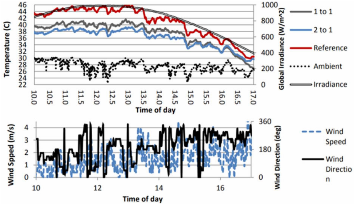
Figure 20. Experimental temperature data for the HPC coupon modules for a day in late May, 2010. (Upper) temperature for the three tested coupons. (Lower) wind data for the experiment site (N=0, E=90)
