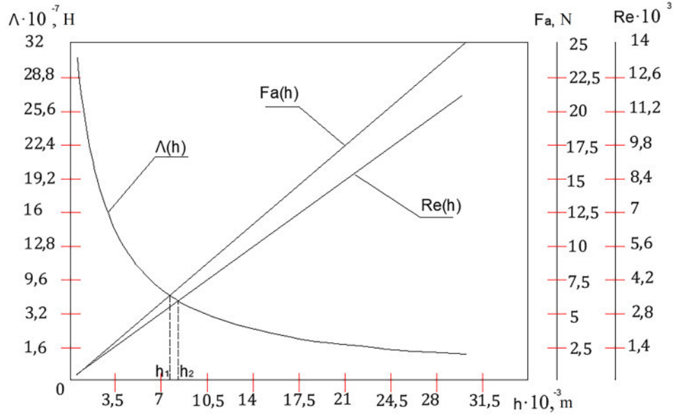
Figure 8. The dependence of magnetic conductivity \Lambda and the force of aerodynamic resistance F_a and Reynolds number Re on the size h of non-magnetic area of the ring-shaped rotor which is between poles when the velocity of the wind is 8 m/s and fixed sizes b , \ell and \delta which are 0.02, 0.05 and 0,001 m.
