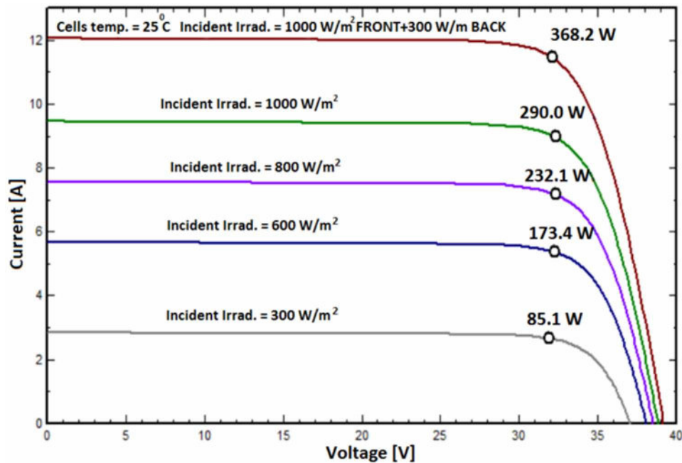
Figure 16. Irradiance dependence Bi60-368BSTC (Prism Solar Technologies Company, n.d.)
