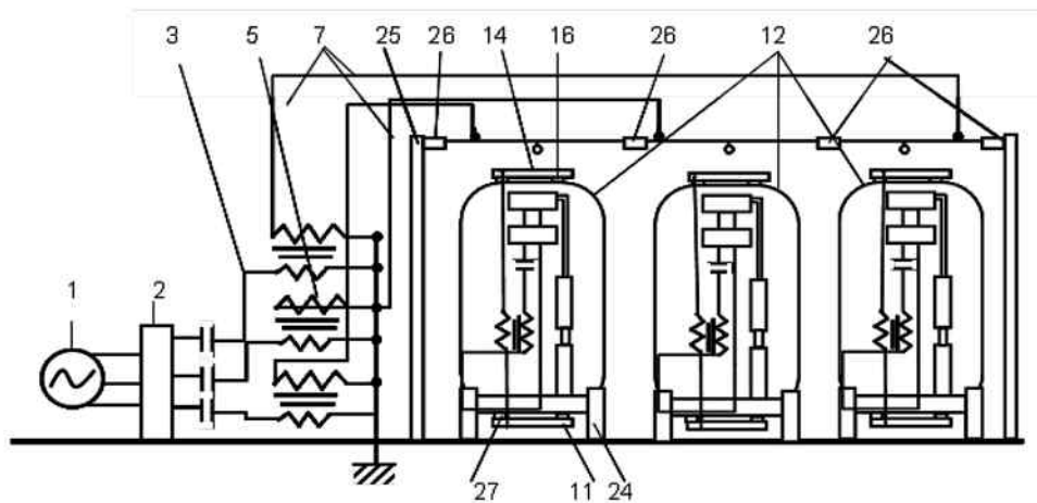
Figure 16. Block diagram of a contactless power supply system using overhead lines
