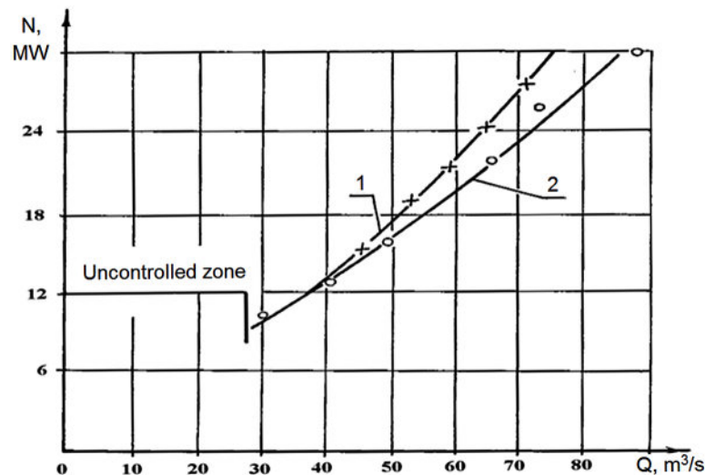
Figure 5. Comparison of methods for controlling the water supply of the pumping station: 1 - the characteristic of the power consumption of the pumping station with the guide device at the inlet, 2 - the same when using the bypass device
