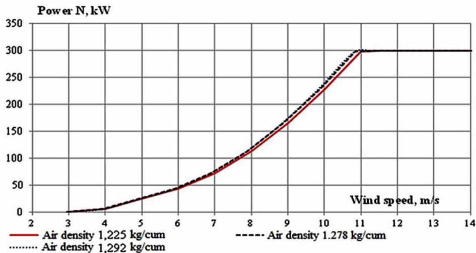
Figure 3. Passport and adjusted for air density power curves of WTG
