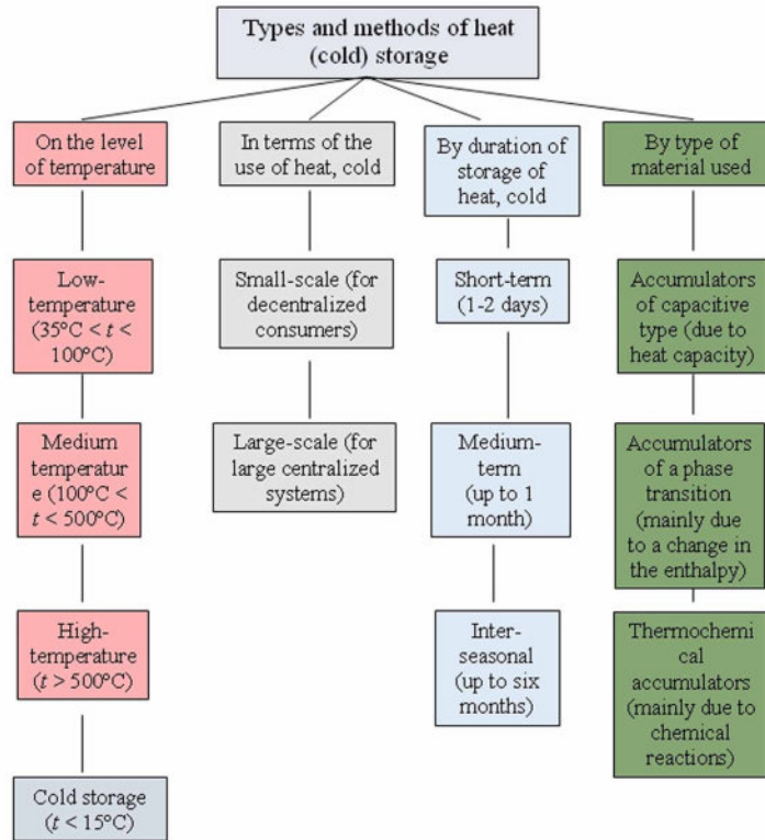
Figure 3. Types and methods of heat (cold) storage
