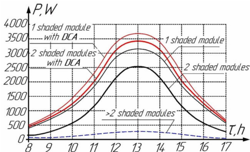
Figure 21. Graphs of the daytime power generation of the array of modules
