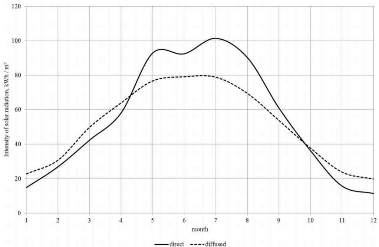
Figure 1. Monthly sums of direct and diffused components of total solar radiation on the horizontal receiving surface
