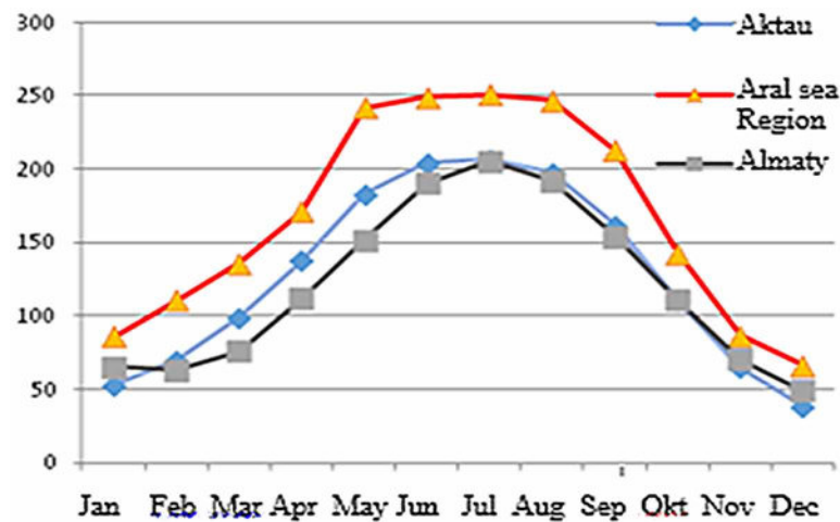
Figure 8. Average monthly daily sum of direct solar radiation on the surface normal to the beam of surface, kWh / m 2 (European Bank for Reconstruction and Development. 2016)
