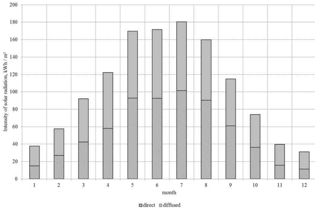
Figure 2. Monthly sums of total solar radiation on the horizontal receiving surface
