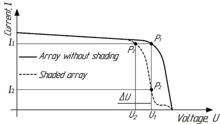
Figure 6. Volt-ampere characteristics of arrays of photovoltaic modules with greater and lesser-rated voltage
