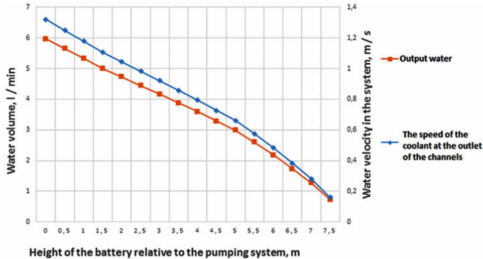
Figure 34. Graph reduction of the coolant flow rate in the system with the increase in the height of the solar panel lift relative to the pump obtained in the simulation
