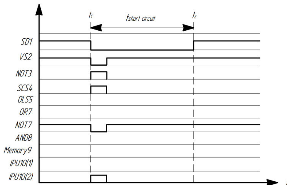
Figure 3. The diagram of signals at the element outputs shown in Figure 1 with a short circuit in the internal network of the consumer
