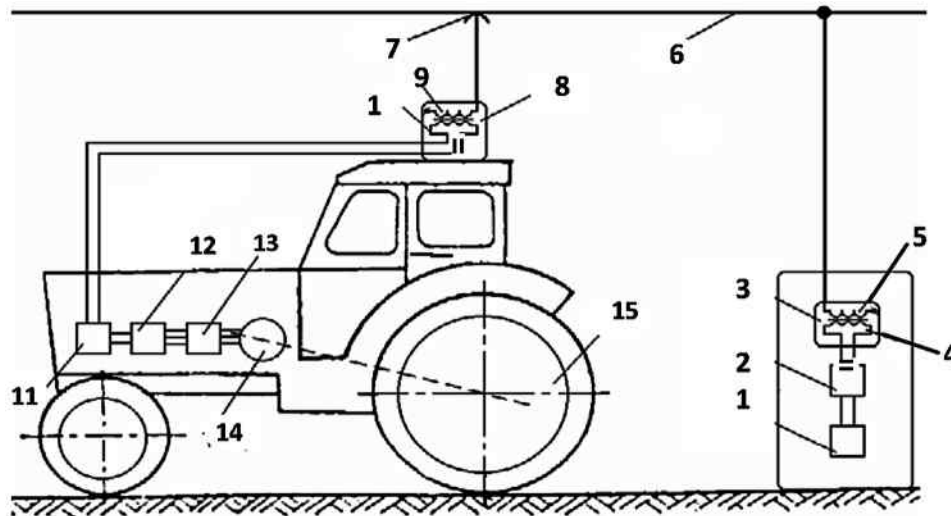
Figure 1. Scheme of the resonant system used to power a mobile mechanism
