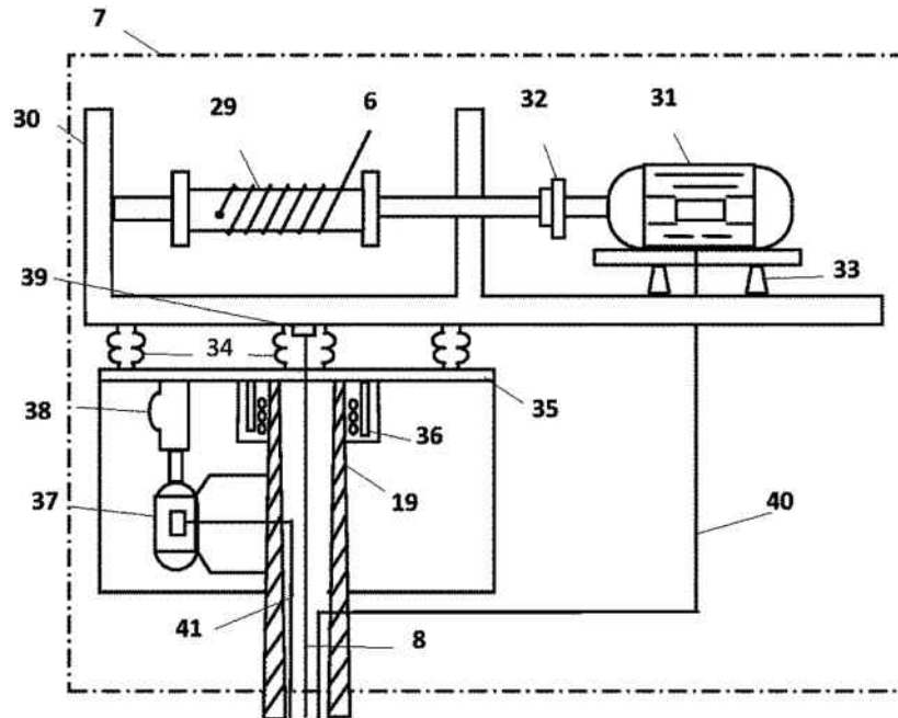
Figure 7. Rotating unit with two motors
