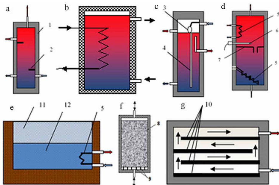
Figure 8. Tanks-batteries and types of HA capacitive type: a – a tank with cold water supply from below and internal partitions; b – a tank with heat input through the heat exchanger; c – a tank with a float valve and a pipe for supplying cold water to the bottom of the tank; d – sectionalized tank with electric heater; e – solar pond; f – a tank with a solid HSM; g – channel; 1 – heat-insulated housing; 2 – partition; 3 – float valve; 4 – standpipe; 5 – heat exchangers; 6 – electric heater; 7 – sectional partition; 8 – solid HSM (gravel, crushed stone, etc.); 9 – supports; 10 – HSM; 11 – water with increasing downward concentration; 12 – a layer of hot solution
