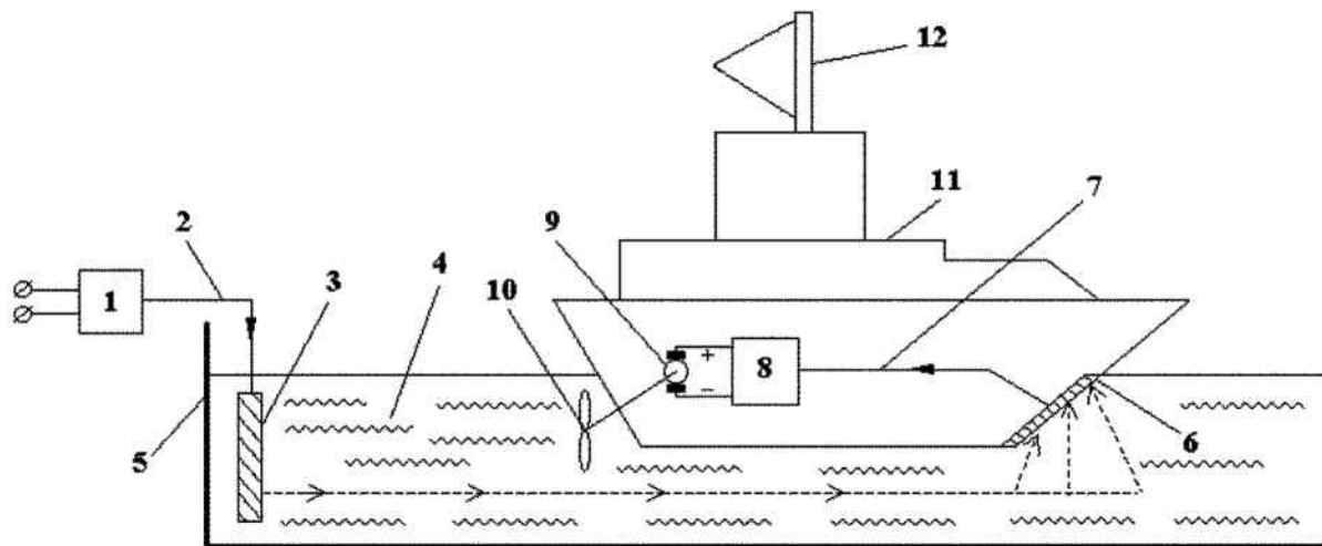
Figure 32. Diagram of the launch power supply circuit, using water medium as a single-wire line 1 – resonant generator; 2, 7 – single –conductor lines; 3 – transmitter electrode; 4 – water; 5 – basin; 6 – receiver electrode; 8 – matching unit; 9 – motor; 10 – propeller; 11 – launch; 12 – natural capacitor.
