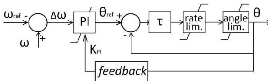
Figure 3. Pitch angle control
