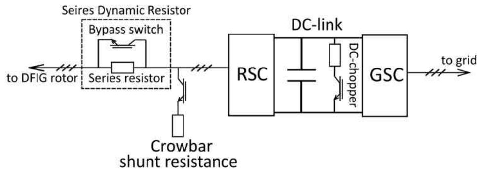
Figure 6. DFIG rotor equivalent circuit with crowbar, DC chopper and series dynamic resistor
