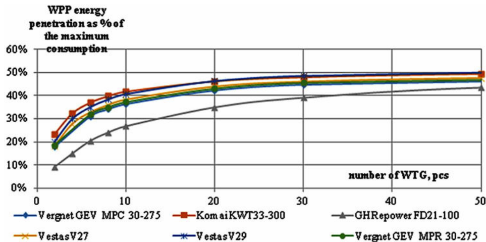
Figure 4. WPP energy penetration, % of annual consumption
