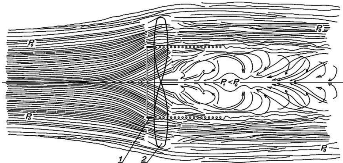
Figure 2. A scheme of the possible motion of a wind flow through the plane of blades rotation with a ring-shaped rotor of an electric generator: 1 – a profile of a coaxial ring-shaped cylinder of the rotor of an electric generator, 2 – blades of a wind turbine.
