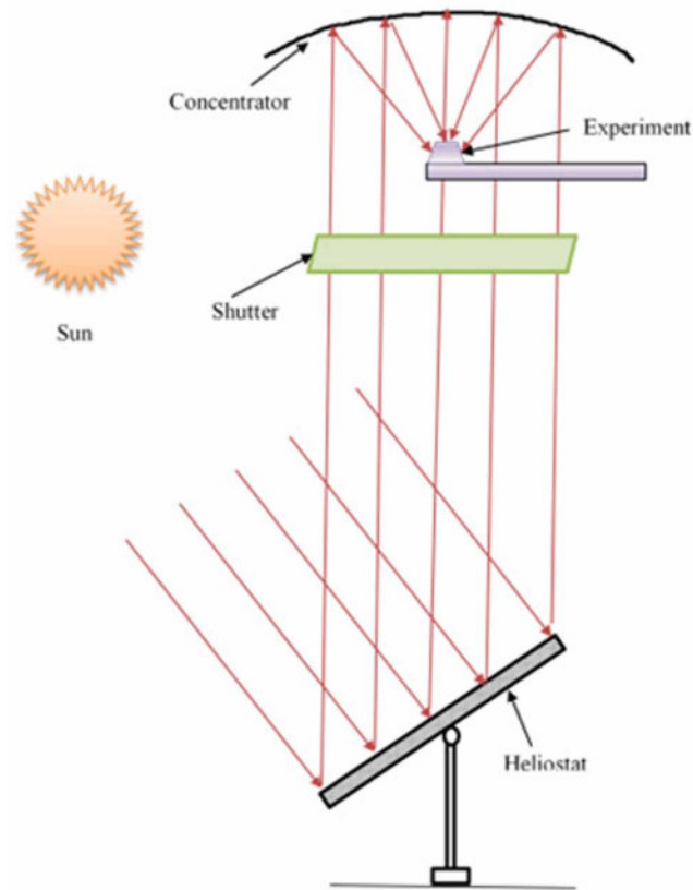
Figure 13. Example 2: method of using heliostats
