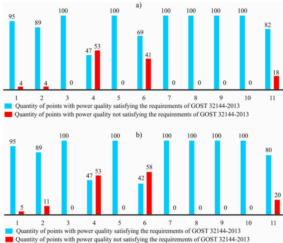
Figure 2. The results of power quality measurements in the Orel region: a - at points of balance delineation between a consumer and a power supplying organization; b – at points of common connection
