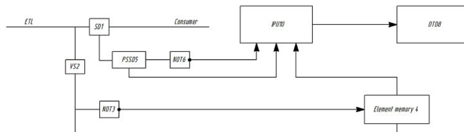
Figure 6. The device for recording the number and duration of power supply outages using the position sensor of the switching device
