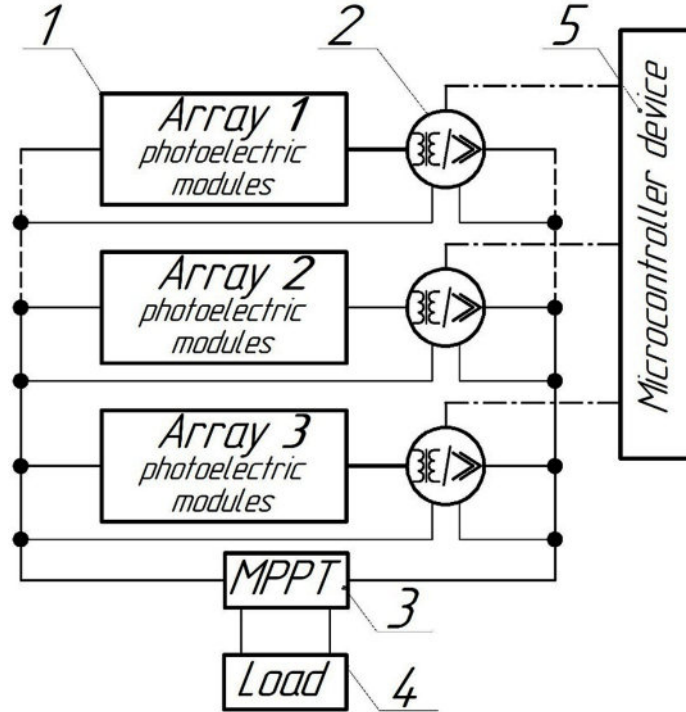
Figure 5. Structural diagram of the method for selecting maximum power from arrays of photovoltaic modules
