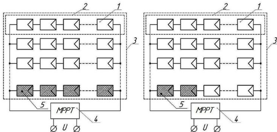
Figure 11. Photovoltaic installation mixed switched PEC: a - uniform shading; b - non-uniform shading (1 - normally illuminated PEC; 2 - array of PEC; 3 - solar installation; 4 - MPPT; 5 - shaded PEC)
