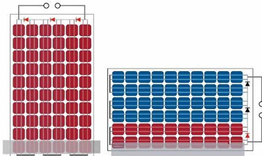
Figure 3. Disconnection of photovoltaic module solar cells by shunt diodes a - for block switching, b - for line switching
