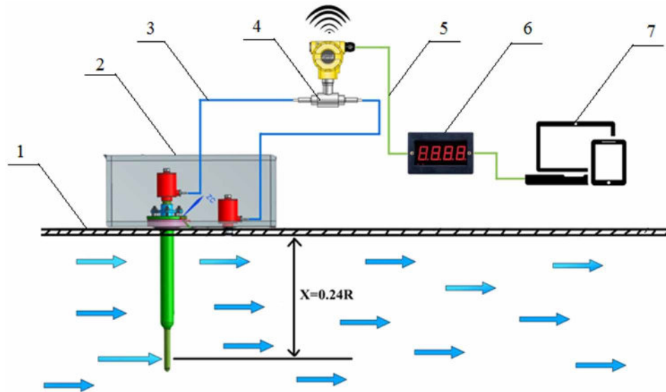
Figure 7. Flowmeter assembly for pump stations with large pipeline diameters: 1 - large diameter pipeline, 2 - flowmeter primary transducer, 3 - hydraulic signal, 4 - pressure difference converter of hydrodynamic heads into a unified current signal, 5 - electrical signal, 6 - microelectronic flow measuring device, 7 - computer
