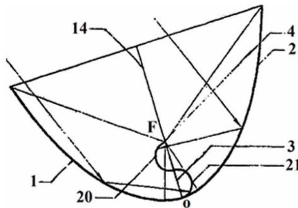
Figure 10. Solar module with a symmetric parabolic concentrators and S - shaped secondary reflectors. 1, 2 - semi parabolic cylindrical reflectors; 20, 21 – additional semi parabolic cylindrical reflectors; 3- radiation receiver with double-sided working surface; 4 - focal axis
