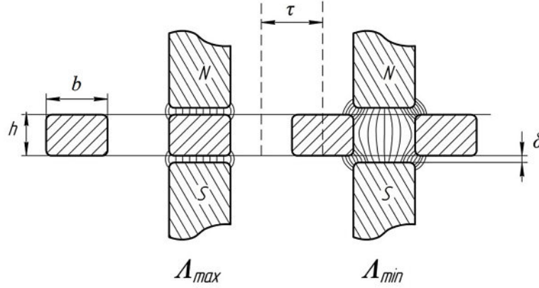
Figure 6. The line drawing presentation of force lines of magnetic field without loading for end positions of ferromagnetic elements of the rotor within one polar division
