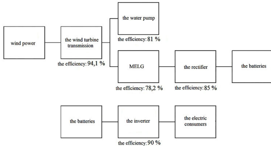
Figure 15. The structural flow chart of a combined electrical and water supplying wind station
