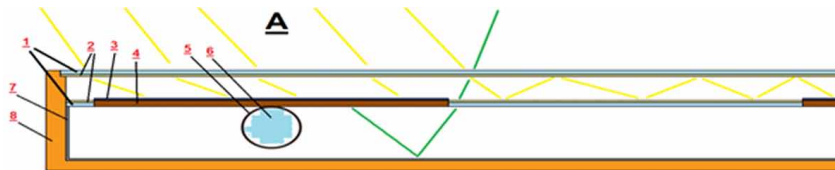
Figure 29. The cut view of the HSP section A (see Figure 3). Where 1 - a glass with total internal reflection, 2 – HOE, 3 – solar cell, 4 - copper plate, 5 - copper pipe, 6 - heat-transport fluid (for example, water), 7 - reflective film, 8 – frame.
