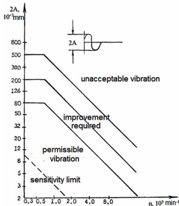
Figure 6. Norms V, D, J on the vibration of pumps of large pumping units of type V
