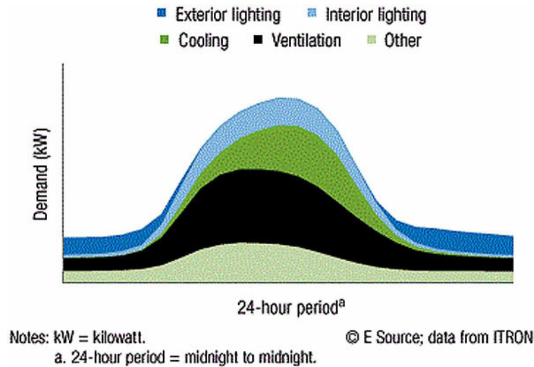
Figure 31. Diagram of a hypothetical daily load shape of school
