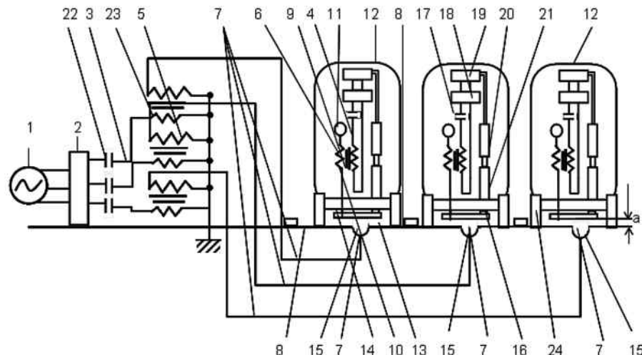
Figure 15. Apparatus for contactless power supply to vehicles, using a three-phase power source
