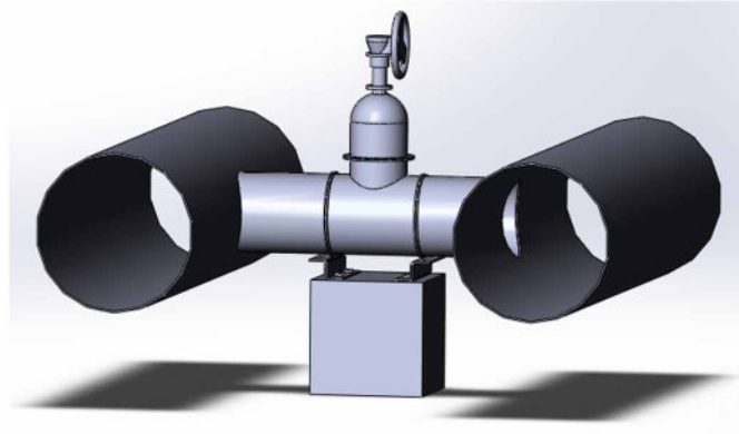
Figure 2. Three-dimensional model of a bypass device with a throttle device
