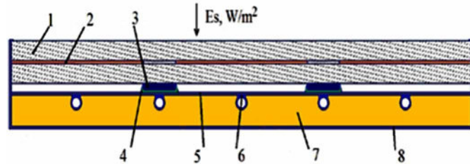
Figure 27. Hybrid solar system 1. Polycarbonate monolith, 2. concentrator of solar radiation – holographic film, 3. Photovoltaic cells, 4. heat conducting grease, 5. absorber, 6. heat transfer fluid, 7. insulation, 8. body.
