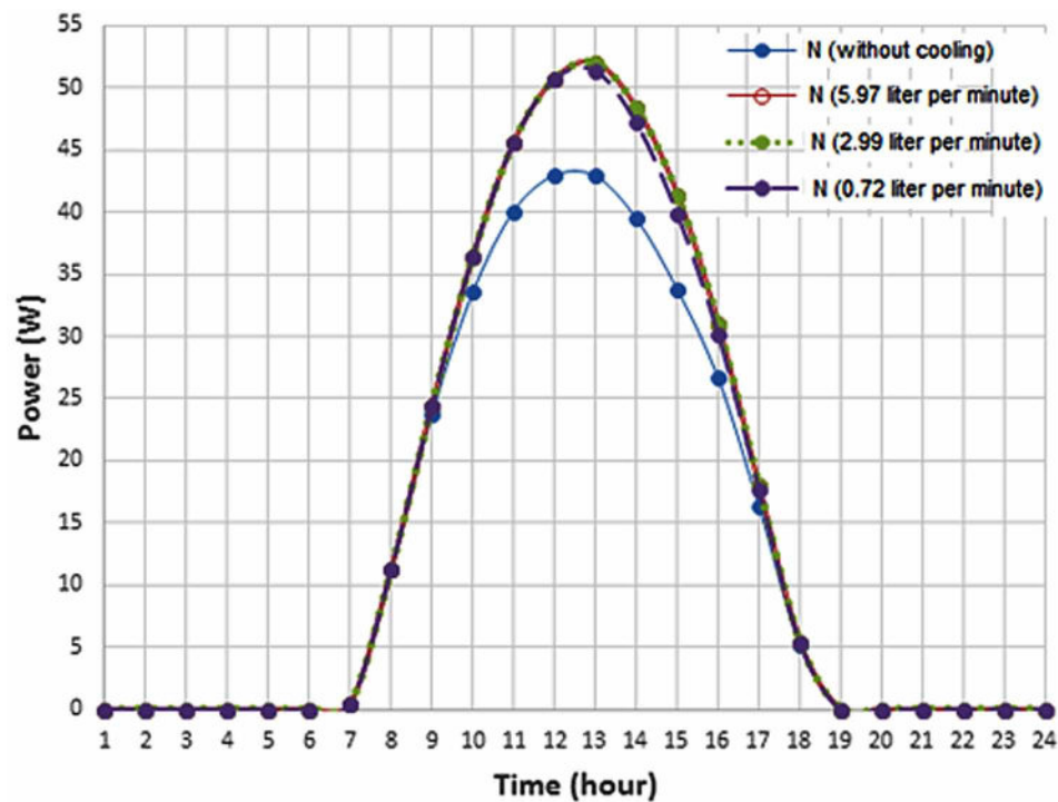
Figure 37. The variation of PV output power by temperature
