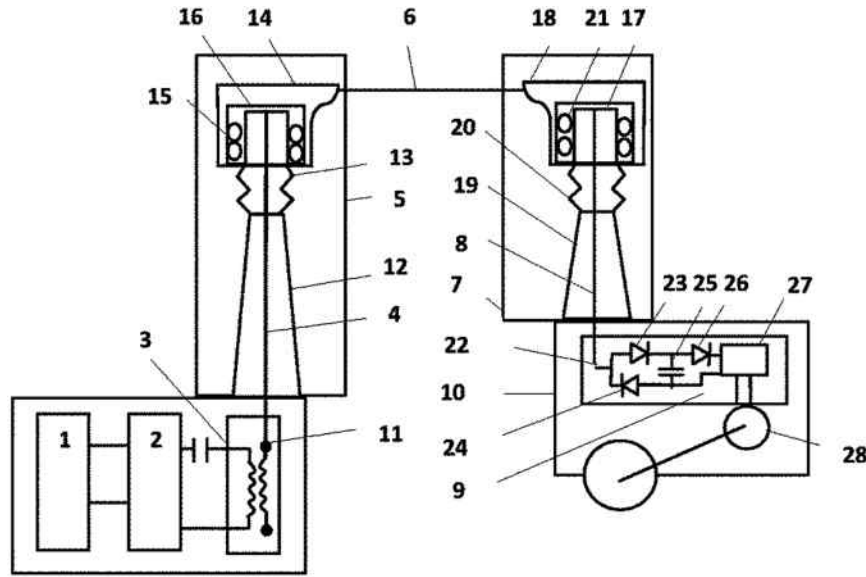
Figure 6. Structure of a transmitter and a receiver with rotating units
