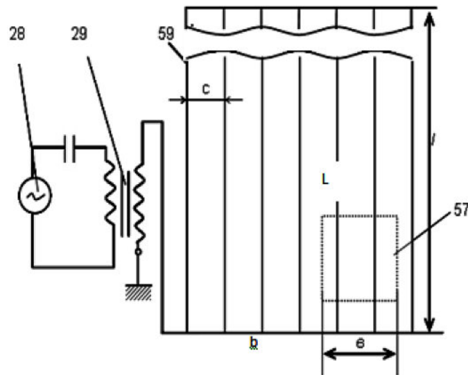
Figure 25. Parallel connection of single wire conductive fines
