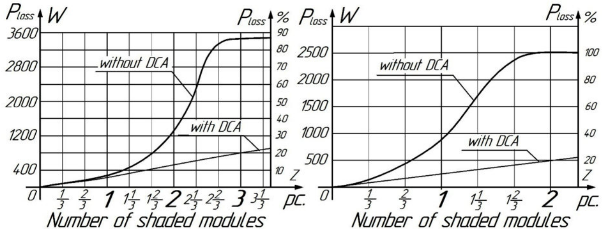
Figure 20. Graphs of power loss of the array of modules from partial shading of modules (a - at the “Sevastopol” solar power plant, b - at the station LLC “NPF” Energospetsproekt)
