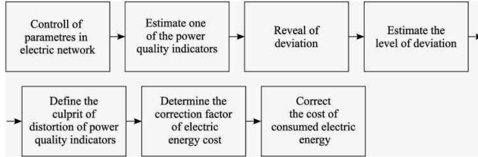
Figure 3. Block diagram of the functional unit for determining the cost of consumed electricity depending on its quality
