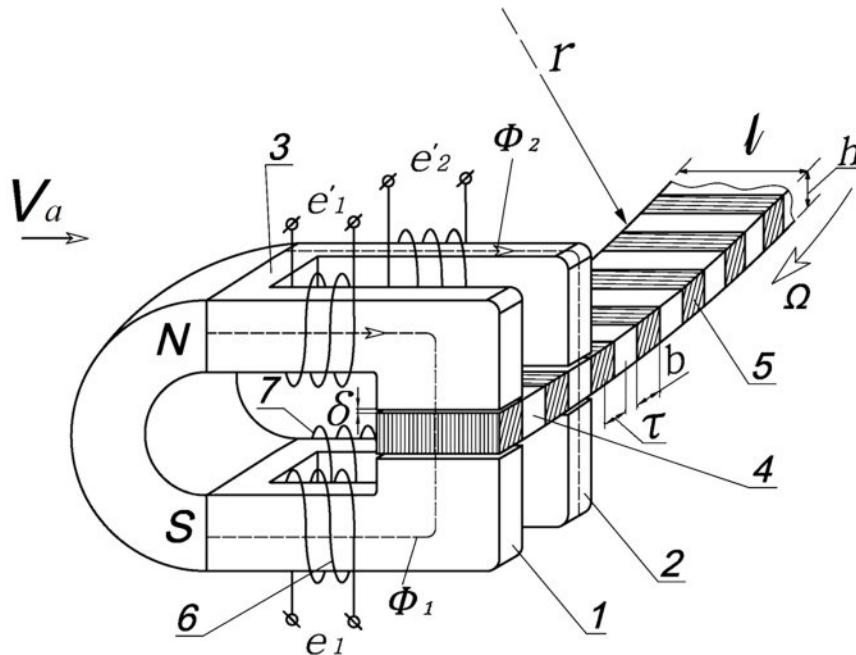
Figure 4. The design of a radial and ring-shaped configuration of the system of a two-packet magneto electrical module of an arc-shaped stator of an inductor-type generator: 1 – the right, on the side of a north pole of the magnet, packet of the magnetic core of a sector of the stator; 2 – the left packet of the magnetic core of a sector of the stator; 3 – a uniform area of the magnetic core between packets; 4 – magnetically non-conductive part of the rotor; 5 – ferromagnetic element of the rotor; 6 and 7 – anchor windings of the right and the left packet of magnetic cores; \Phi_1 and \Phi_2 – the path of magnetic excitation fluxes in packets; \delta – a working airy gap; r – a radius of a ring-shaped rotor; b , \ell , h – overall sizes of ferromagnetic elements of the rotor; \tau – a polar division of the rotor, \tau = b ; V_a – an approximate wind direction, e_1 , e_2 – an electric driving force in the windings of the corresponding packets.
