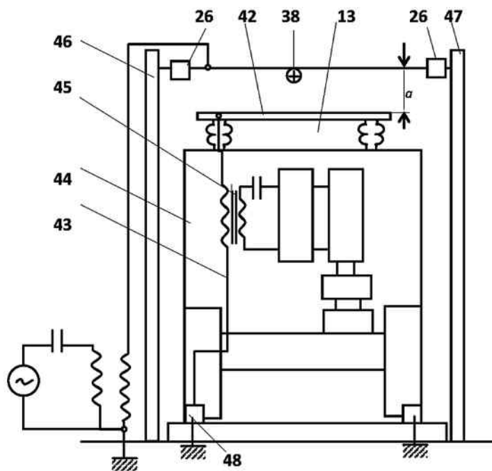
Figure 20. Power supply for rail way vehicle
