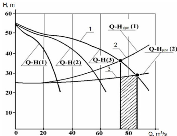
Figure 4. Method of regulation of operating modes by means of bypass device
