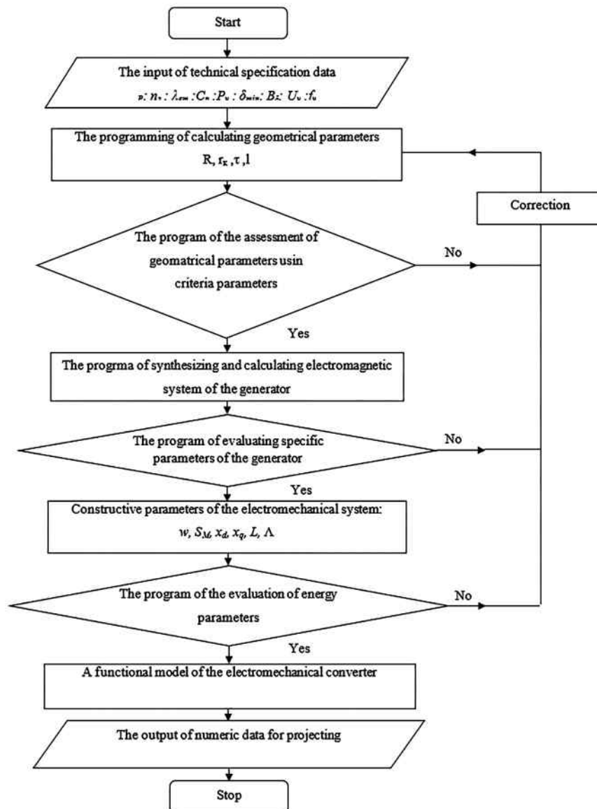
Figure 9. The algorithm of projecting an integral non-transmission electromechanical converter with a ring-shaped rotor
