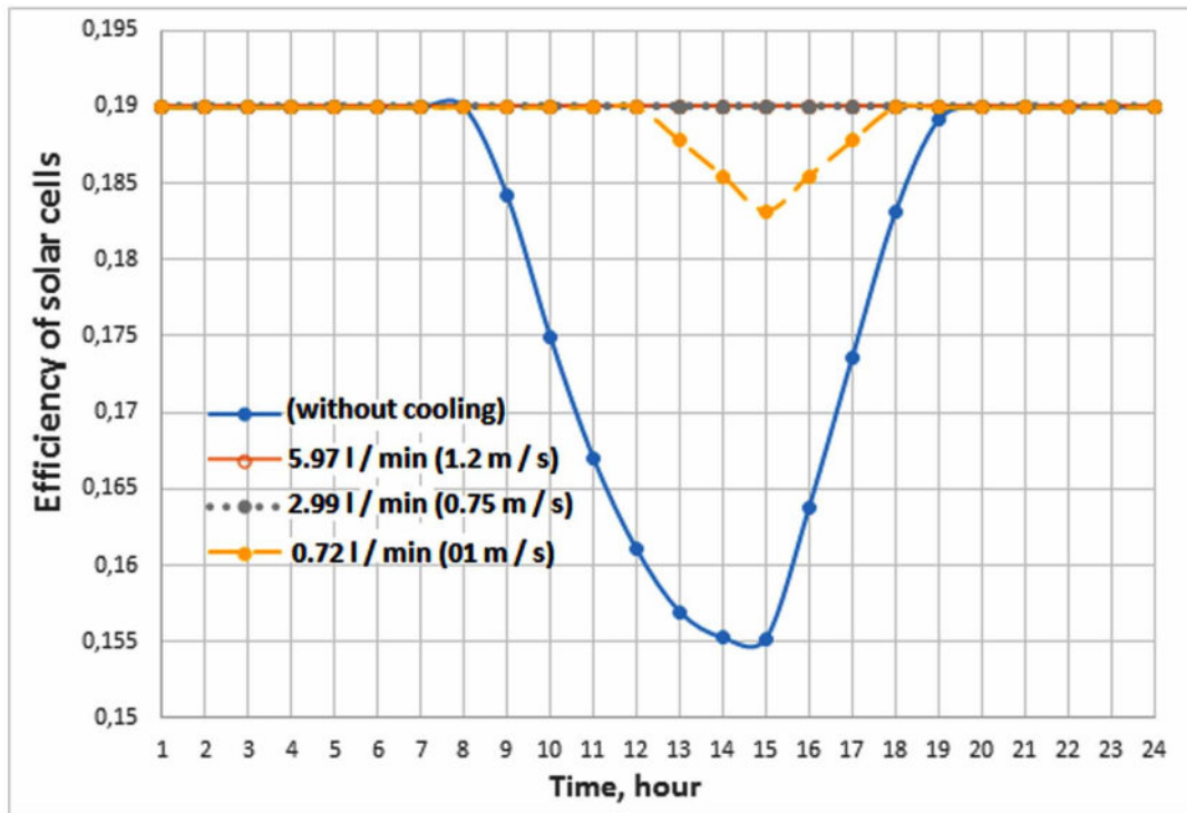
Figure 36. Changing the efficiency of the solar module with and without cooling
