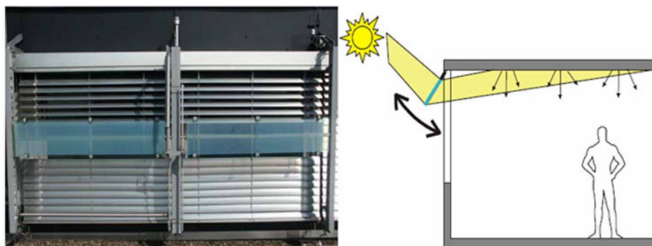
Figure 15. Light directing system with conventional shading device (Wagner, 2004)
