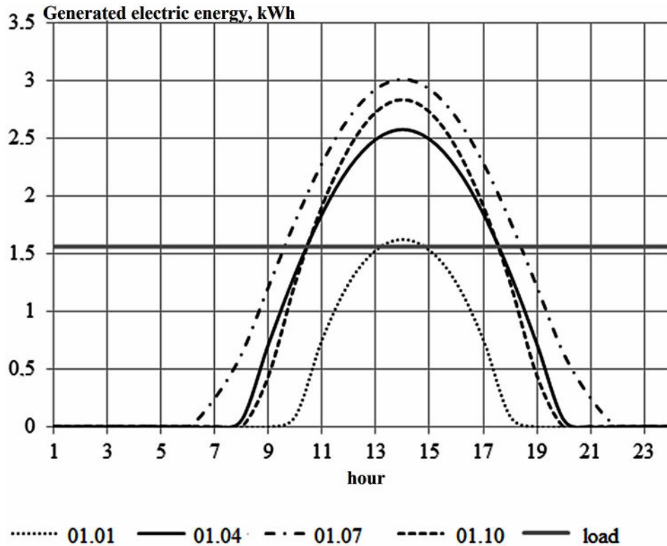
Figure 9. Daily schedule of generation and consumption of electrical energy for 1 option of its layout by photoelectric modules
