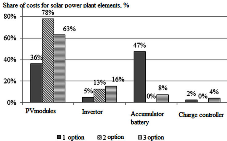
Figure 12. The share of the initial costs of acquired components of the solar power plant
