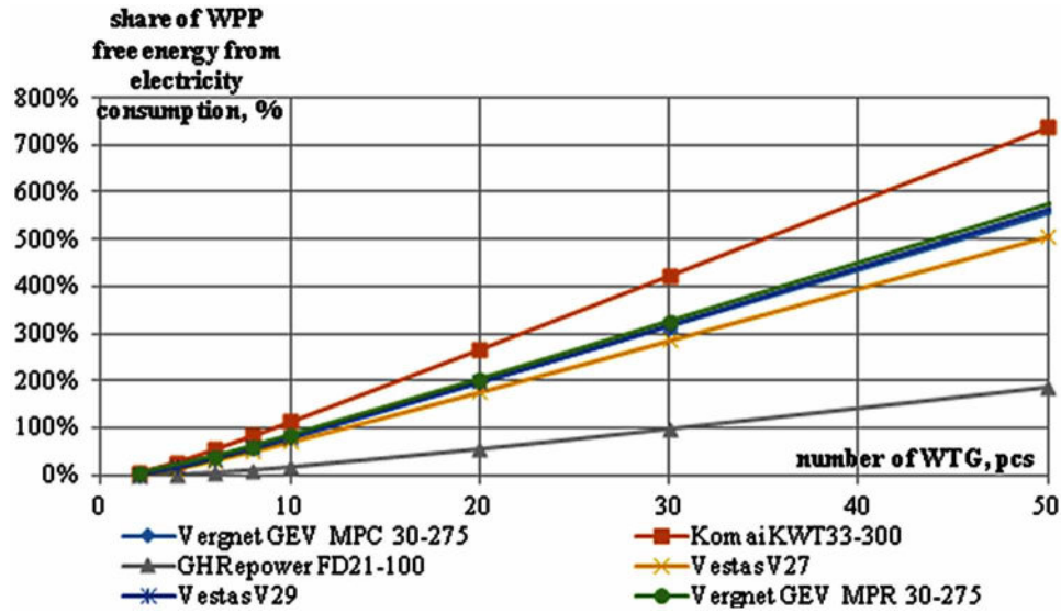
Figure 5. Free energy of WPP, % of annual consumption
