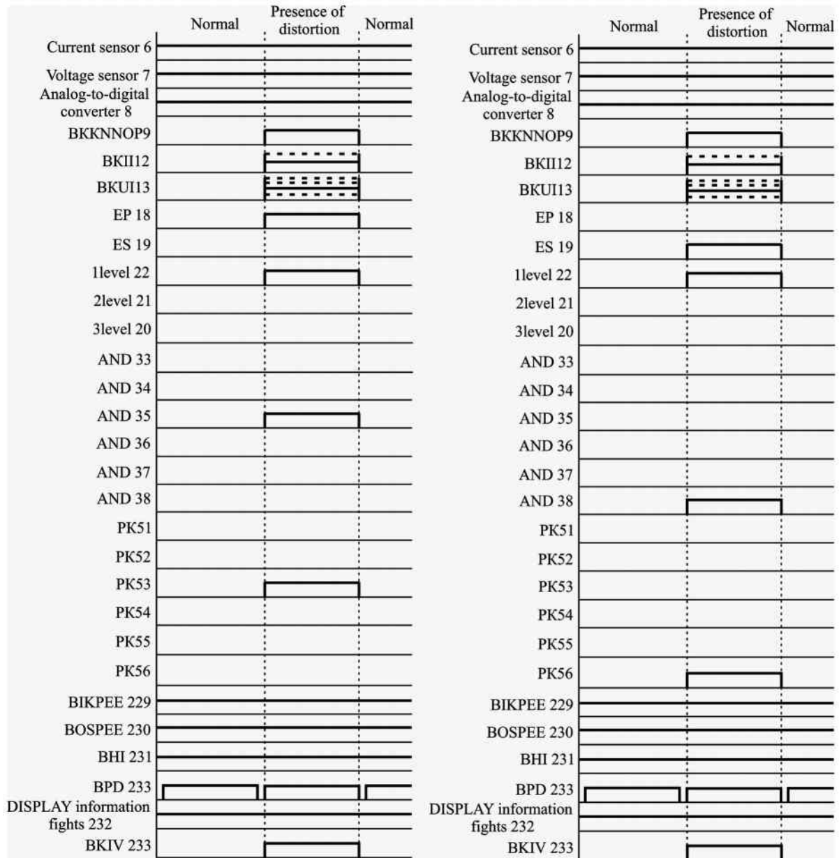
Figure 8. Diagram of output signals when: A - Energy supply system is the source of distortion; B - Consumer is the source of distortion
