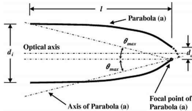
Figure 6. Compound cone concentrator; l - the height of the reflector; D, d - hole of entry and exit
