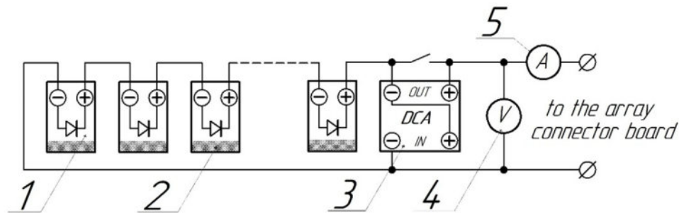
Figure 17. Structural diagram of the inclusion of the DCA (1 - solar module, 2 - shadow, 3 - DCA, 4 - voltmeter, 5 - ammeter)
