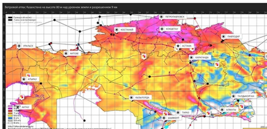
Figure 3. Wind speed distribution over the territory of Kazakhstan (height of measurements – 80 m) (The Kazakhstan an Electricity Association Committee on Renewable Energy Sources)
