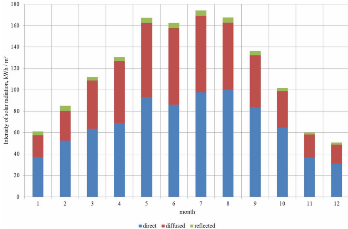
Figure 5. Monthly sums of all components of solar radiation for the optimal angle of inclination relatively to the horizon of the receiving surface of southern orientation
