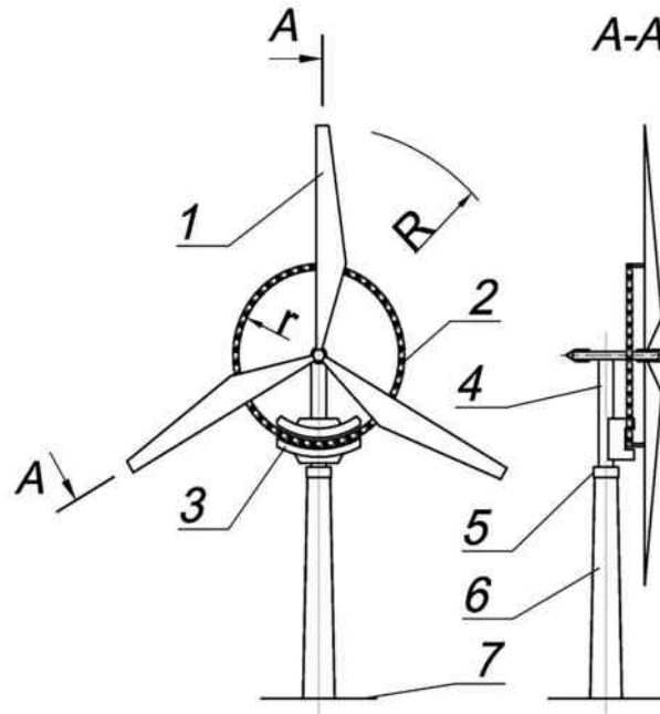
Figure 1. A general construction scheme of a non-transmission wind energy station with an electric generator with the ring-shaped rotor and the arc-shaped stator: 1 – a blade, 2 – a ring-shaped rotor, 3 – an arc-shaped stator, 4 – a swinging spar, 5 – a spider of the swinging spar, 6 – a bearing pier, 7 – pedestal, R – a radius of a circle of the rotation of blades ends, r – a radius of a circular rotor.
