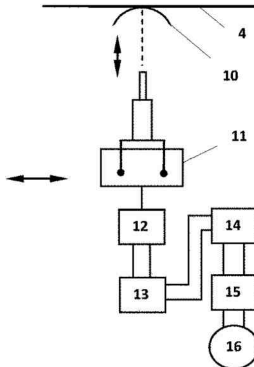
Figure 3. Block diagram of vehicle equipment powered from a single-conductor contact system
