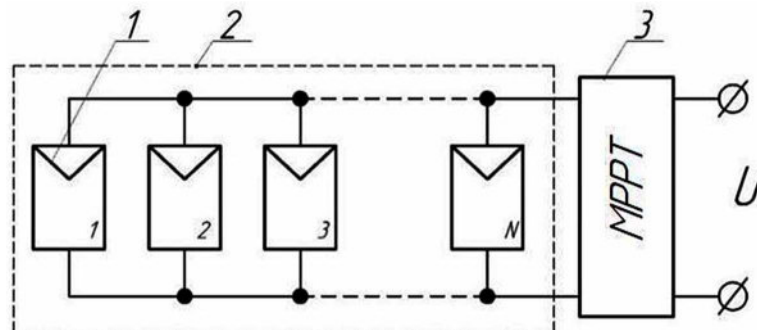
Figure 8. Installation with parallel solar cells in the battery (1 - PEC; 2 - solar photovoltaic installation; 3 - the device for finding the maximum power point and optimizing the output power (MPPT))
