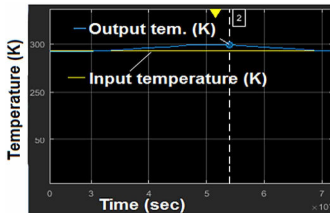
Figure 42. The variation of the output and input temperature result from Simulink (the length of the copper tube 1 meter)
