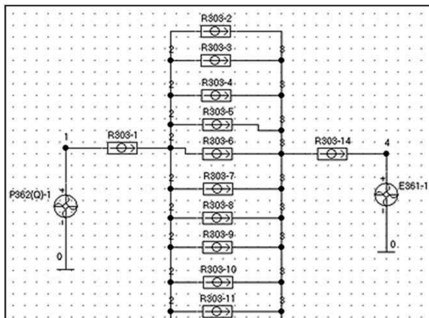
Figure 33. An example of a graphical representation of the model of hydrodynamic processes in the program ASONIKA-P
