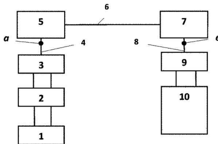
Figure 5. Block diagram of the apparatus for electric power supply to a mobile electric mechanism
