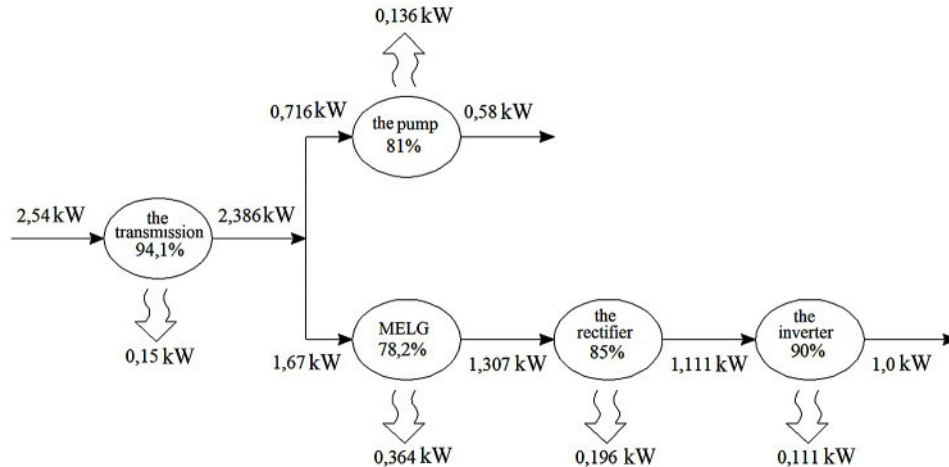
Figure 13. The structural flow chart of the balance of powers of CEWWS for electricity consumers, the value of the power being 1.0 kW, with the valid water flow 2 \cdot 10^{-3} \text{ m}^3/\text{s} , and the pressure 0.29 \cdot 10^6 \text{ Pa}
