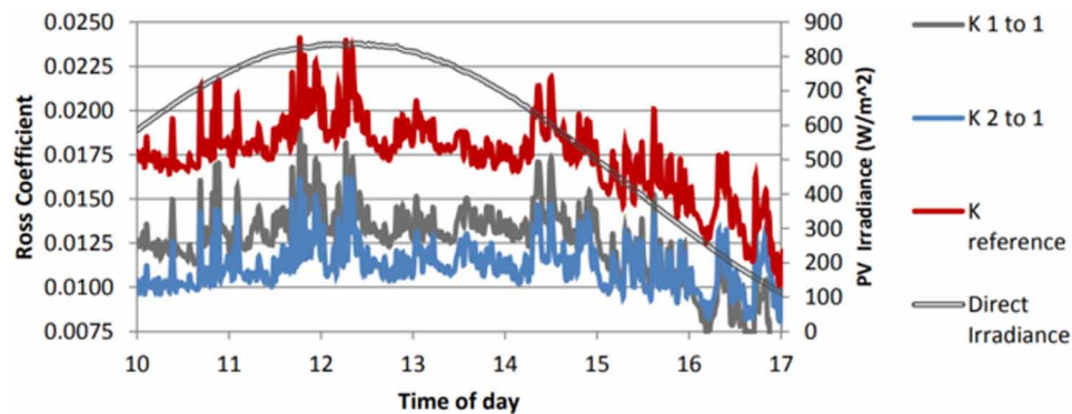
Figure 19. Ross coefficient [ \text{Km}^2\text{W}^{-1} ] for the measured data from the test coupons
