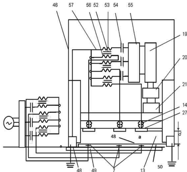
Figure 21. Apparatus for non-contact supplying power to a rail vehicle using the three-phase lines
