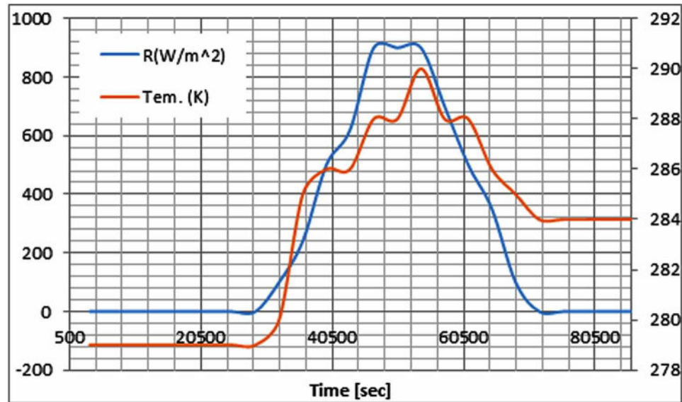
Figure 41. The variation of the solar radiation ( \text{W/m}^2 ) and ambient temperature (K) for a typical day on January in Tajikistan (Li et al., 2013).
