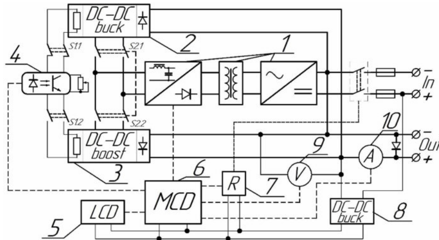
Figure 7. Functional diagram of the DCA; 1 - high-frequency converter with galvanic isolation; 2 - DC/DC buck (power); 3 - DC/DC boost (power); 4 - control device for DC/DC converters; 5 - display; 6 - microcontroller device; 7 - relay; 8 - DC/DC buck (low-current); 9 - voltage sensor 10 - current sensor.
