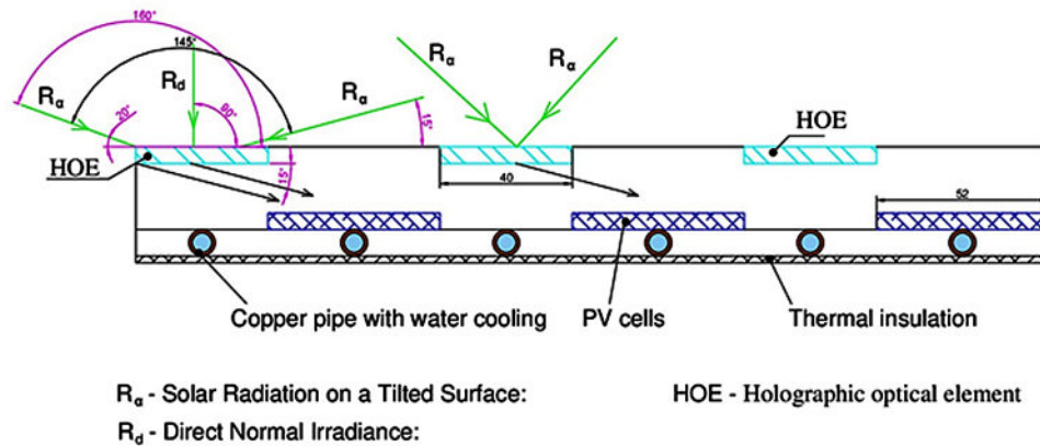
Figure 30. Design of hybrid solar panel without the use of the law of total internal reflection
