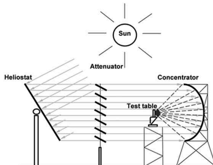
Figure 12. Example 1: method of using heliostats
