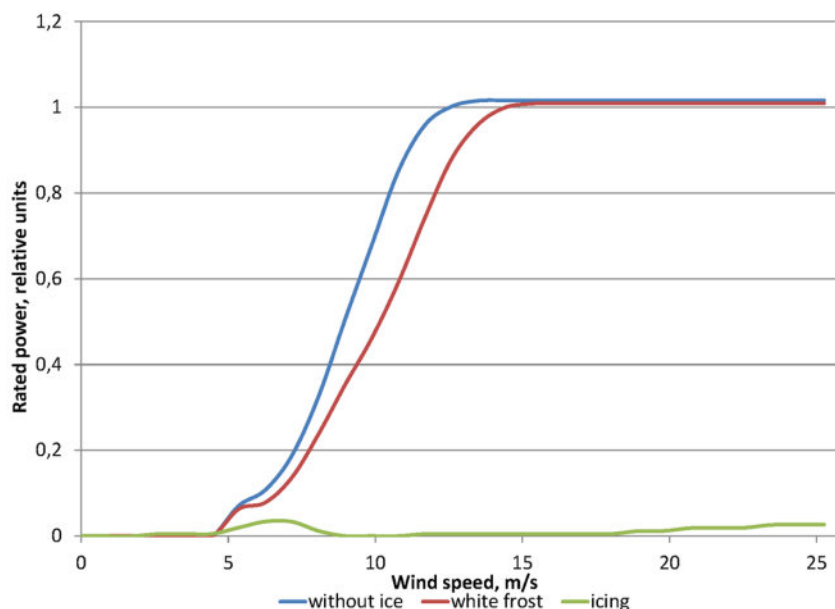
Figure 3. Dependence of the rated power of wind turbines on wind speed under different conditions of icing of blades and equipment (Elistratov, 2017)
