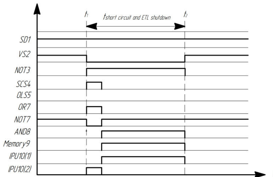
Figure 4. Diagram of signals at the element outputs shown in Figure 1 with a short circuit in the customer network and the subsequent non-selective tripping of the switching device in the power line
