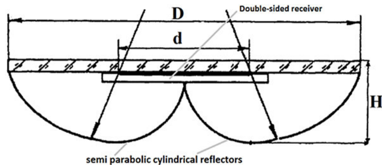
Figure 11. A photovoltaic module based on w shaped concentrator
