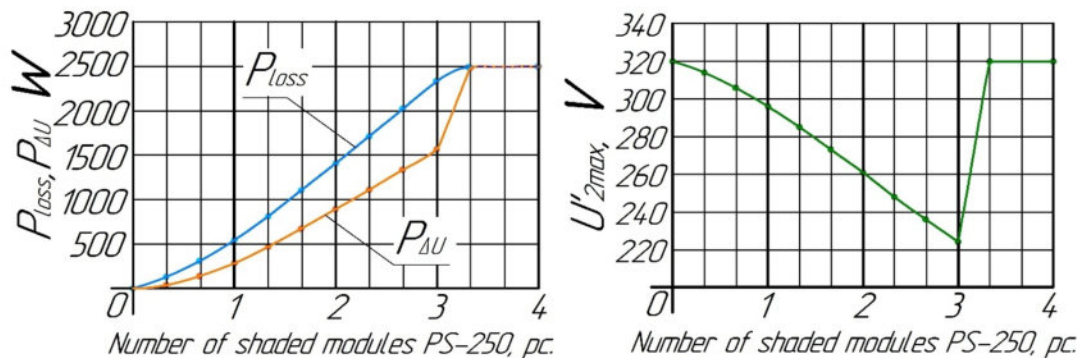
Figure 14. Graphs of the dependence of power losses and output voltage of SFU with a power of 30 kW from partial shading of photoelectric modules of one of the arrays
