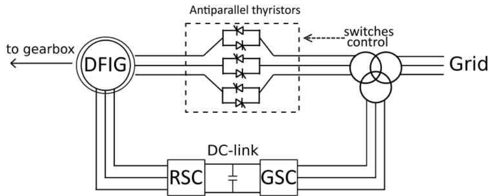
Figure 8. Antiparallel thyristors in the stator side
