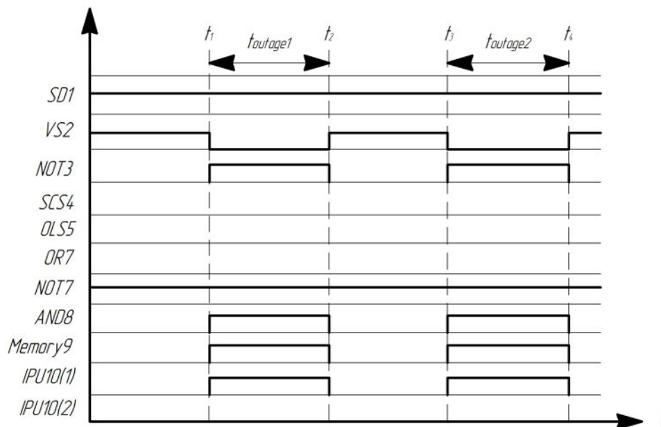
Figure 2. The diagram of signals at the element outputs shown in Figure 1 when the voltage at the consumer input is disconnected
