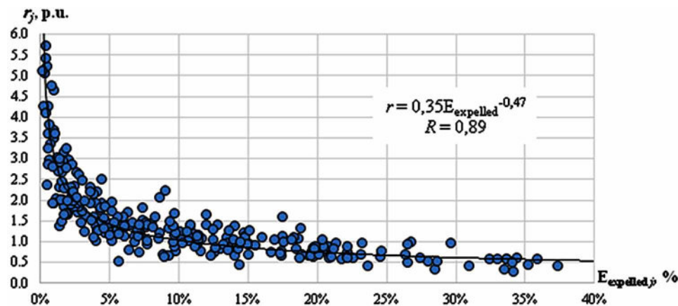
Figure 7. The empirical and approximating dependence of r_j on E_{\text{expelled}_j} according to the data of WDC of the village of Novikovo, Sakhalin Region
