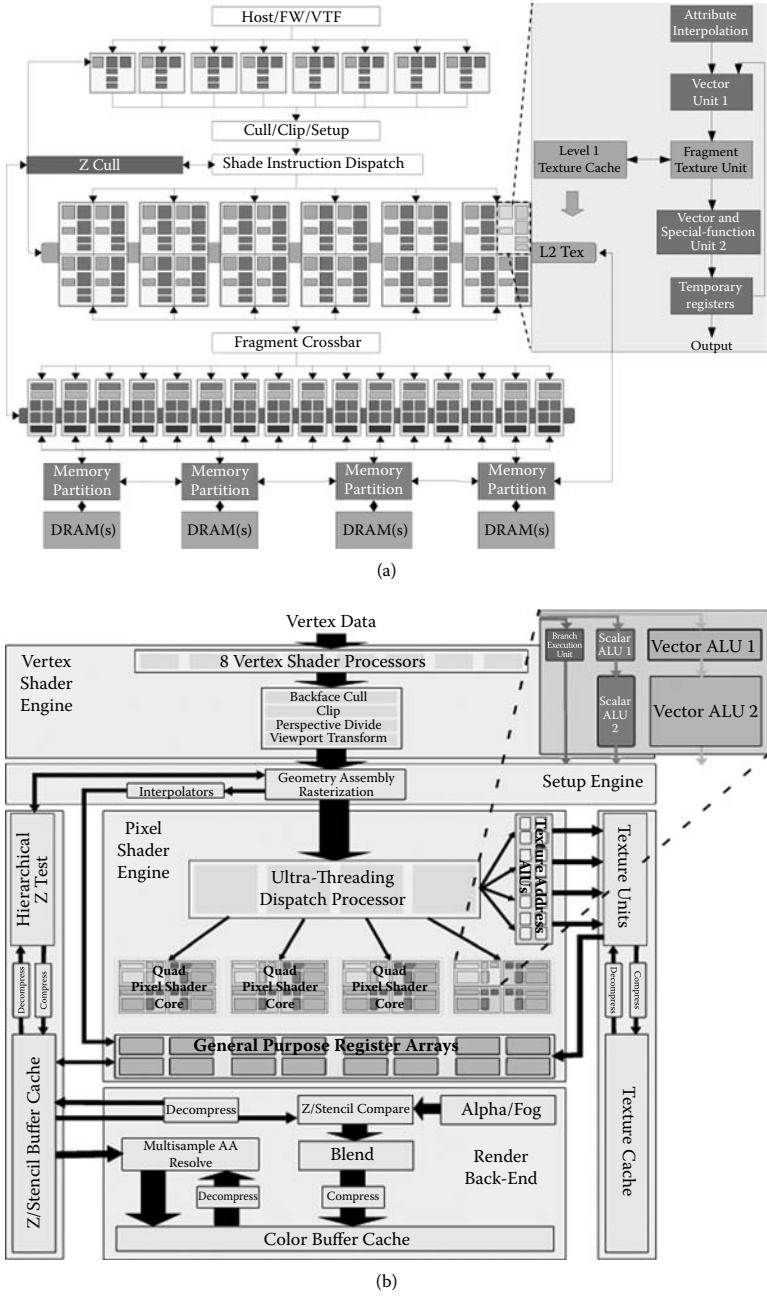
Figure 18.4 NVIDIA G70 (a) and ATI-RADEON R520 (b) block diagrams.
