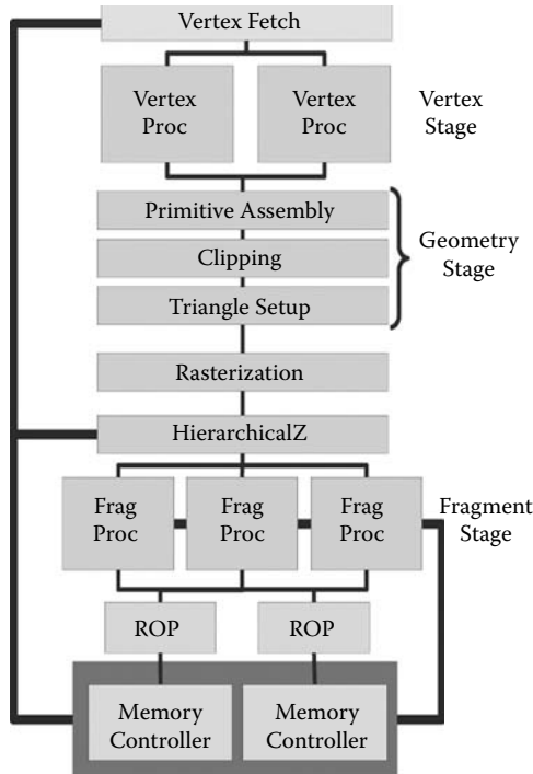
Figure 18.3 Fourth generation of GPUs block diagram. These GPUs incorporate fully programmable vertexes and fragment processors.
