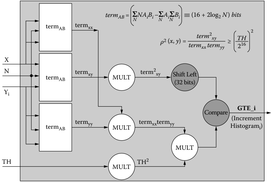
Figure 15.9 Correlator module.
