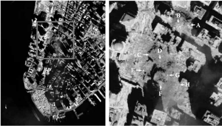
Figure 2.6 AVIRIS hyperspectral image collected by NASA’s Jet Propulsion Laboratory over lower Manhattan on Sept. 16, 2001 (left), and location of thermal hot spots in the fires observed in the World Trade Center area (right).
