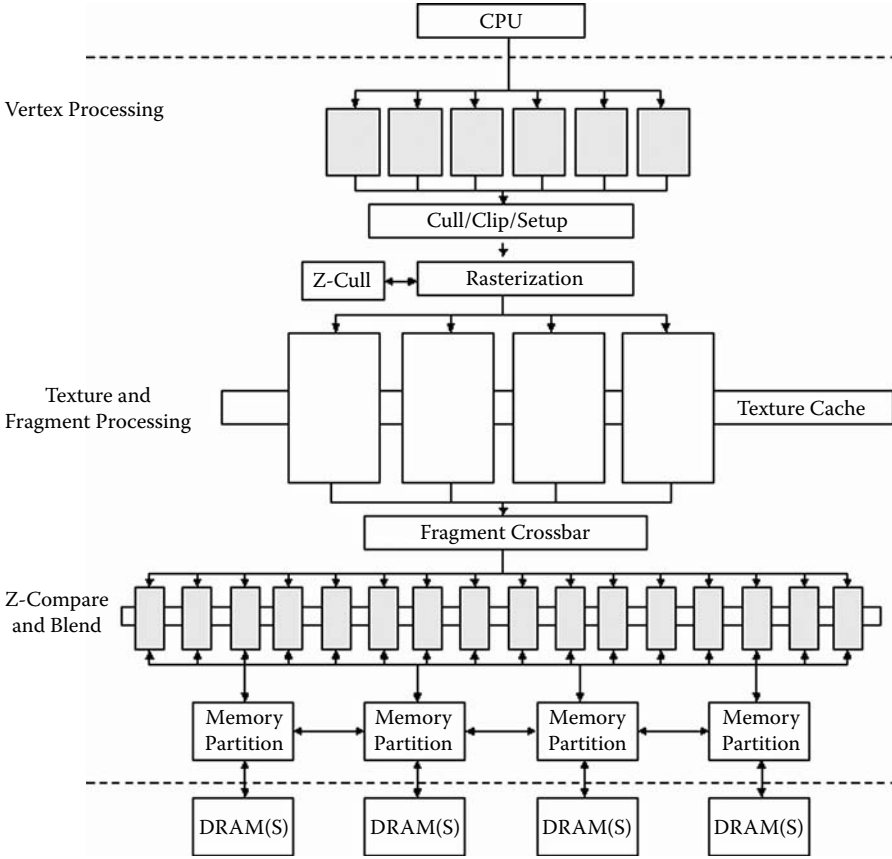
Figure 3.2 GPU pipeline.
