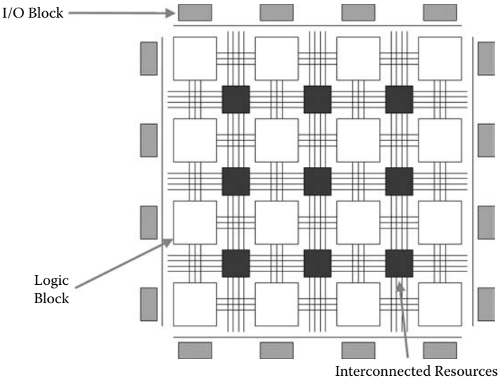
Figure 15.3 FPGA structure.
