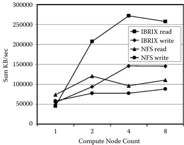
Figure 6.9 Performance comparison of multiple computer node access to a data storage system using the traditional NFS or newer IBRIX parallel file system.
