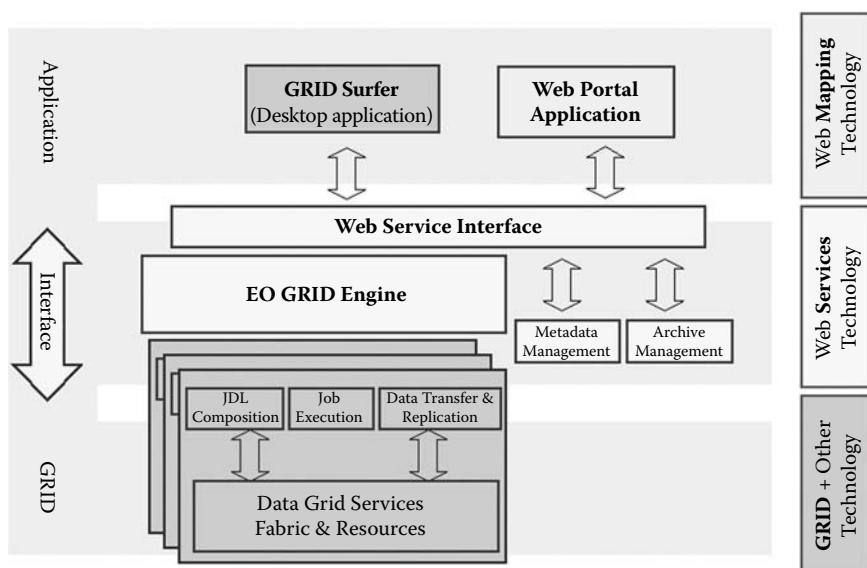
Figure 11.4 The architecture model for EO Grid on-Demand Services.
