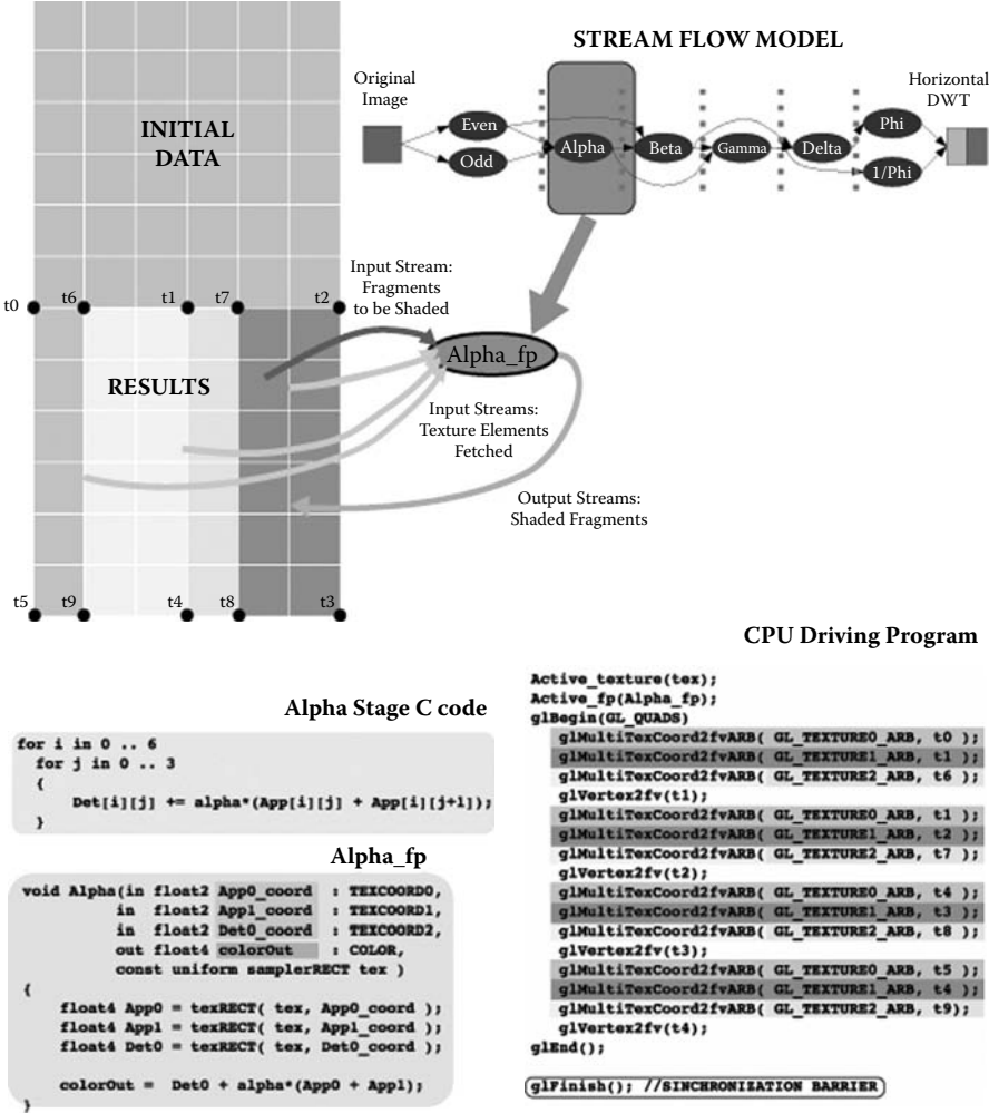
Figure 18.8 Mapping one lifting step onto the GPU.
