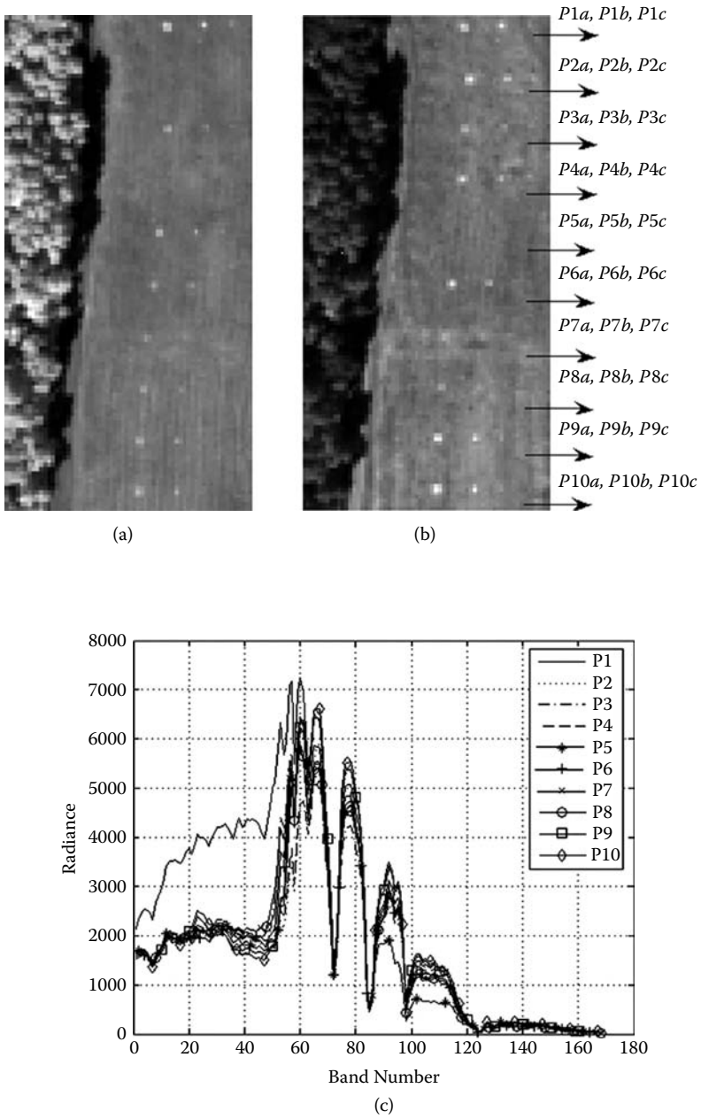
Figure 17.1 (a) A HYDICE image scene that contains 30 panels. (b) Spatial locations of 30 panels provided by ground truth. (c) Spectra from P1 to P10.
