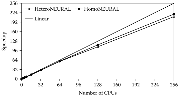
Figure 7.5 Scalability of parallel neural classifier on Thunderhead.
