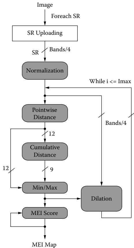
Figure 18.15 Flowchart of the proposed stream-based GPU implementation of the AMEE algorithm using SID as pointwise distance.
