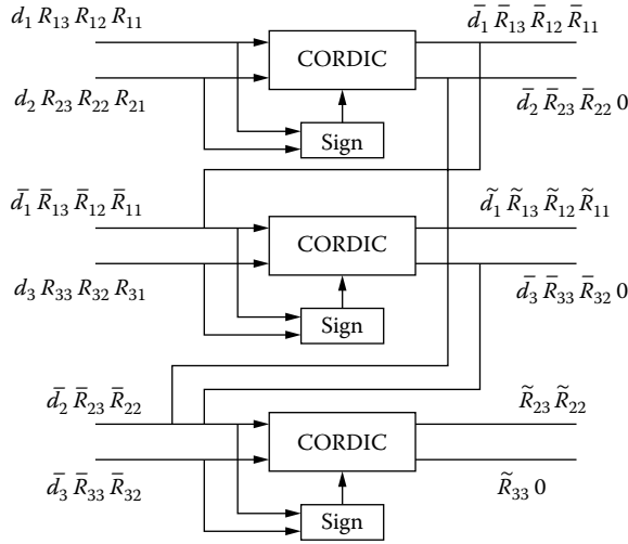
Figure 16.8 QR-decomposition by CORDIC circuit.
