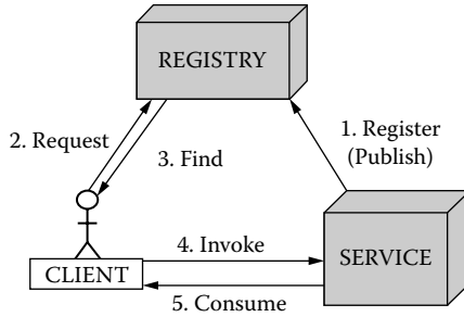
Figure 9.1 The service architecture concept.
