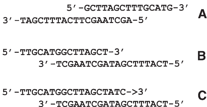
Fig. 2. Dimer structures.
