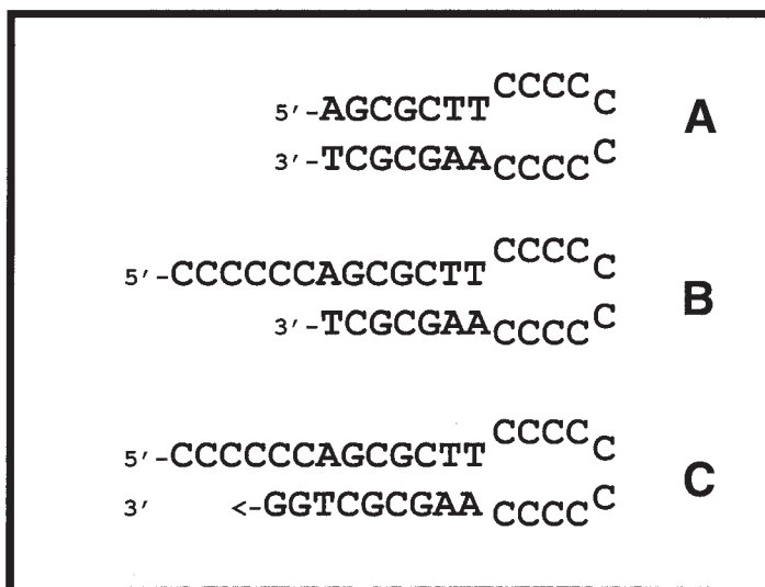
Fig. 1. Hairpin structures.
