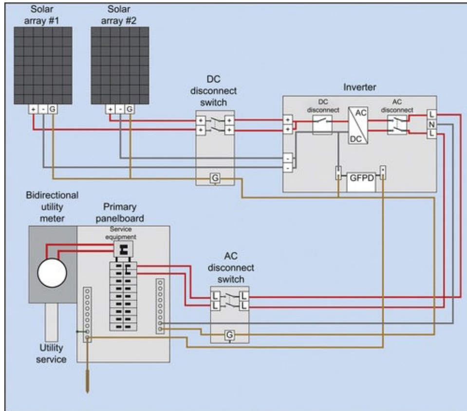
FIGURE 5.2 Grid-tied photovoltaic system with single inverter. Courtesy of www.DreamHomeConsultants.com . (For color version of this figure, the reader is referred to the online version of this book.)
