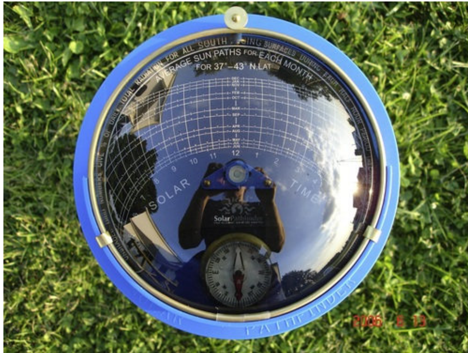
FIGURE 2.15 Solar Pathfinder. Photo courtesy of The Solar Pathfinder Company. (For color version of this figure, the reader is referred to the online version of this book.)
