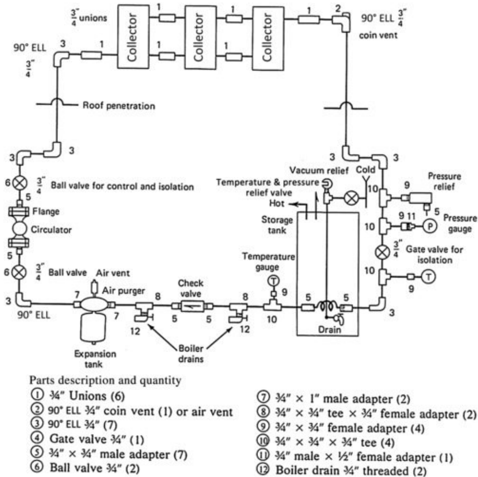
FIGURE 4.2 Miscellaneous plumbing hardware (closed-loop freeze-resistant system).
