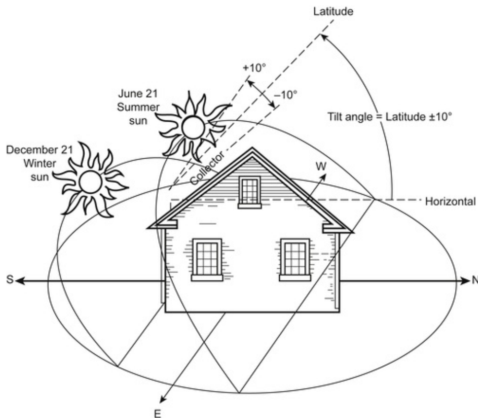
FIGURE 2.13 Collector tilt.
