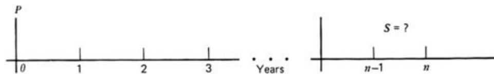
FIGURE 6.1 Time scales.
