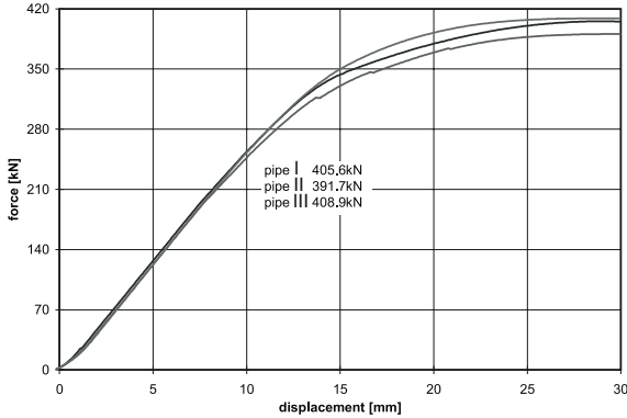
Fig. 17. Load-displacement curves.
