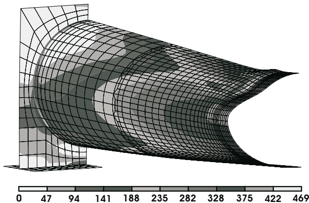
Fig. 22. Contour plot of the v. Mises equivalent stress for the pipe segment.
