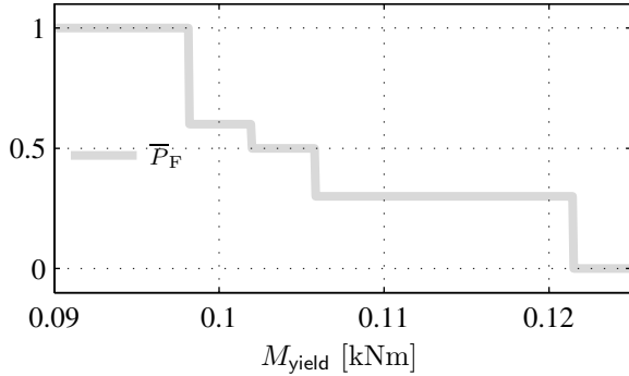
Fig. 12. Upper probability \bar{P}_F(y \geq M_{yield}) of failure.
