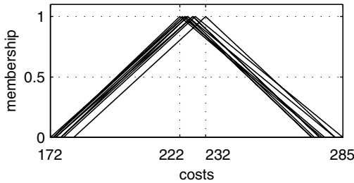
Fig. 23. Fuzzy cost variations at duration T = 29 .
