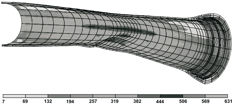
Fig. 4. Contour plot of the v. Mises equivalent stress [N/mm^2] of the pipe in the vicinity of the support on the pile.
