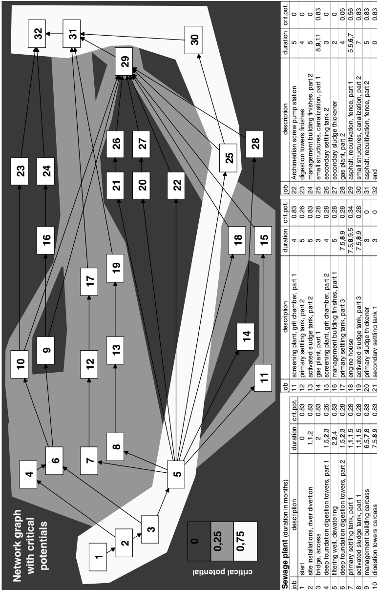
Fig. 19. Fuzzy network.
