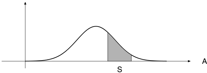
Fig. 3. Probability distribution
