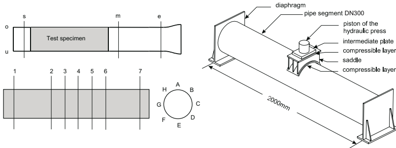
Fig. 6. Pipe segments and test set-up.
