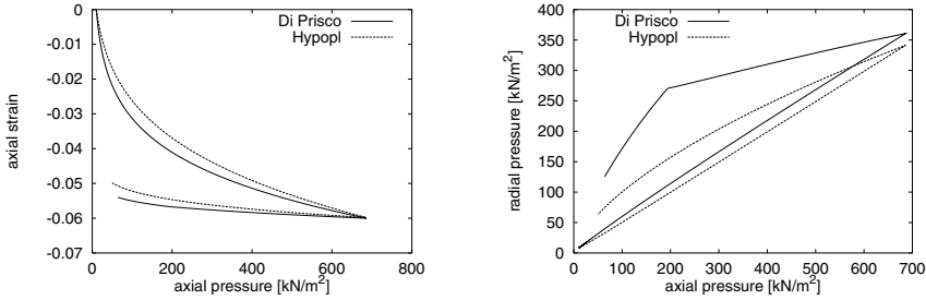
Figure 1. Elastic range of di Prisco model yields an unrealistic oedometer stress path during unloading (right)
