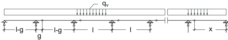
Fig. 1. Structural system and loading of a pile-supported pipeline.
