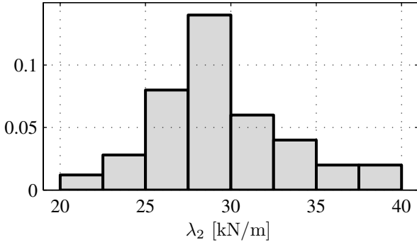
Fig. 7. Example 4: Uncertainty of \lambda_2 .
