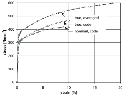
Fig. 38. Stress-strain diagrams.
