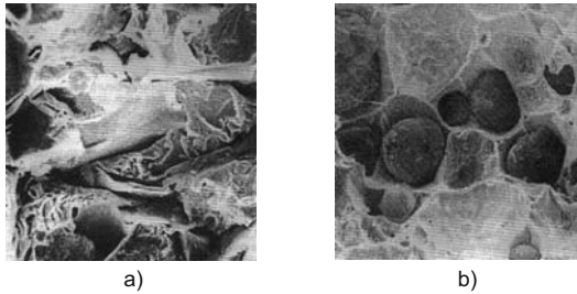
Fig. 7. Microstructure of a) grey cast iron and b) spheroidal graphite cast iron; (REMx700).
