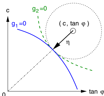
Fig. 11. Two situations with equal \eta (14) and different limit state functions g_1 and g_2 : more combinations of c and \varphi exist with failure conditions in the case of g_2 (area below the limit state g_2 = 0 is larger than the area below g_1 = 0 ).
