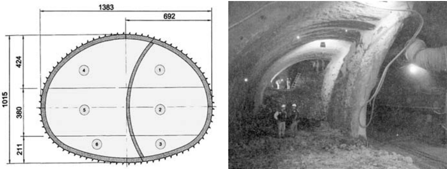
Fig. 9. Experiment – Compressed-air tunnel driving in the shotcrete construction method, 1979 Line5/9 Munich Odeonsplatz [1]
