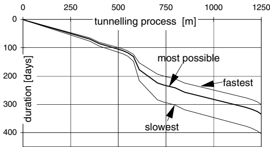
Fig. 18. Time/velocity diagram.
