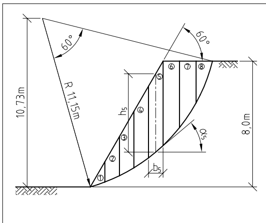
Fig. 2. Stability of slope.
