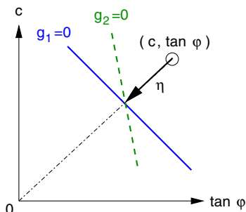
Fig. 10. Two situations with equal \eta (14) and different limit state functions g_1 and g_2 : The distance to g_2 is shorter.
