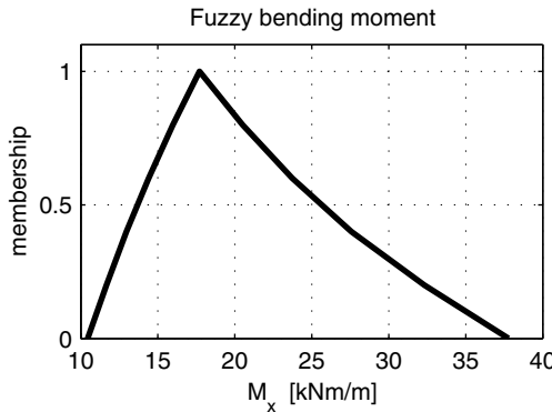
Fig. 6. Membership function of \tilde{M}_x .
