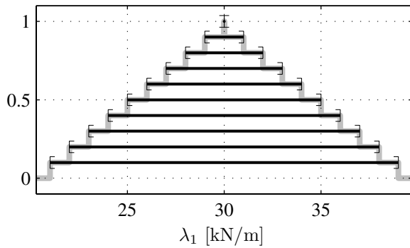
Fig. 6. Example 3: Uncertainty of \lambda_1 and \lambda_2 .
