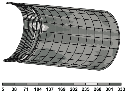
Fig. 5. Contour plot of the v. Mises equivalent stress [N/mm^2] of the pipe in the vicinity of the sleeve
