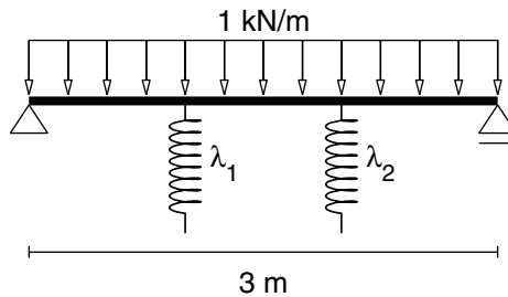
Fig. 1. Beam bedded on two springs.
