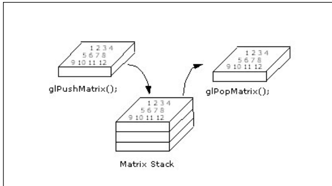
Figure 4.13 Pushing and popping on the matrix stack.
