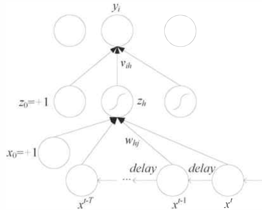
Figure 11.20 A time delay neural network. Inputs in a time window of length T are delayed in time until we can feed all T inputs as the input vector to the MLP.
