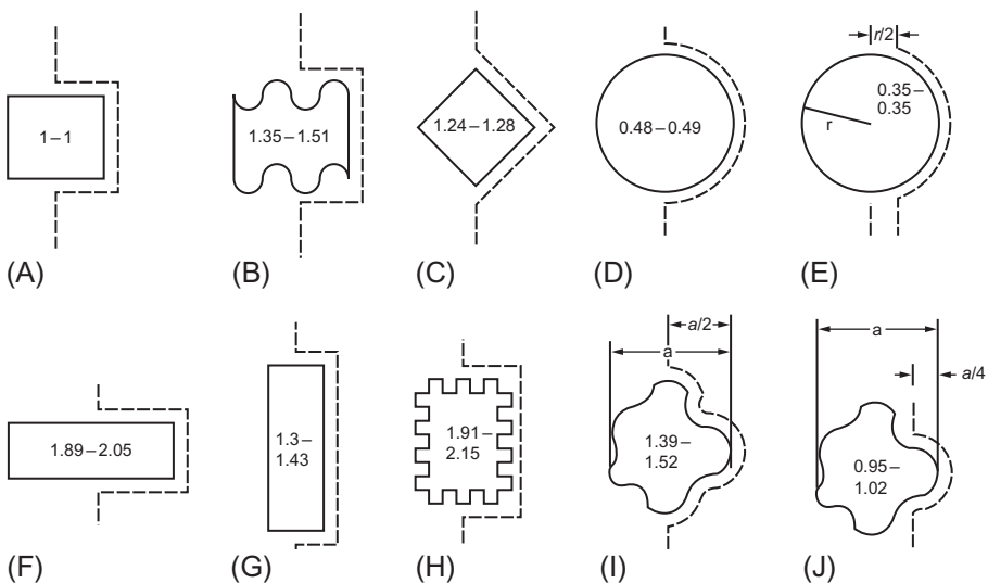
Fig. 11.1 The effects of aggregate shape, surface texture, and disrupt position on concrete. (A) Cubical, with three sides of smooth surface. (B) Cubical, with two sides of rough texture. (C) Cubical, with two sides of smooth surface. (D) Spherical, half of the smooth surface. (E) Spherical, covered the surface of 1/4 of the diameter. (F) Rectangular, horizontal position, with three sides of smooth surface. (G) Rectangular, vertical position, with three sides of smooth surface. (H) Cubical rough surface, covered half of the surface. (I) Angular surface, covered half of the surface. (J) Angular surface, covered the surface of 1/4 of the diameter.
