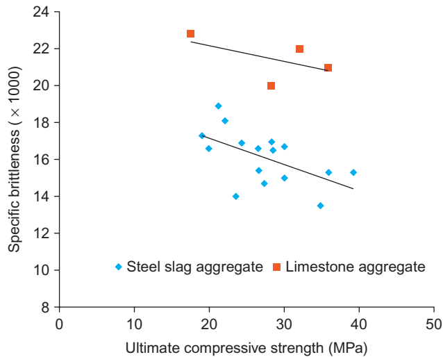
Fig. 11.9 Relationship between specific brittleness and compressive strength.
