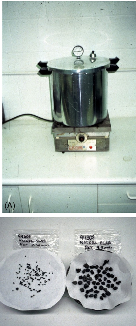
Fig. 14.12 (A) Autoclave test nickel slag aggregate and (B) aggregate after testing.
