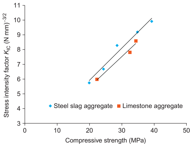
Fig. 11.10 Relationship between stress intensity factor and compressive strength.
