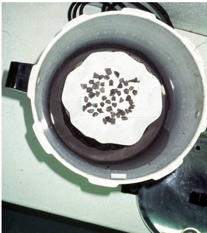
Fig. 12.10 View of slag particles following the autoclave disruption test.
