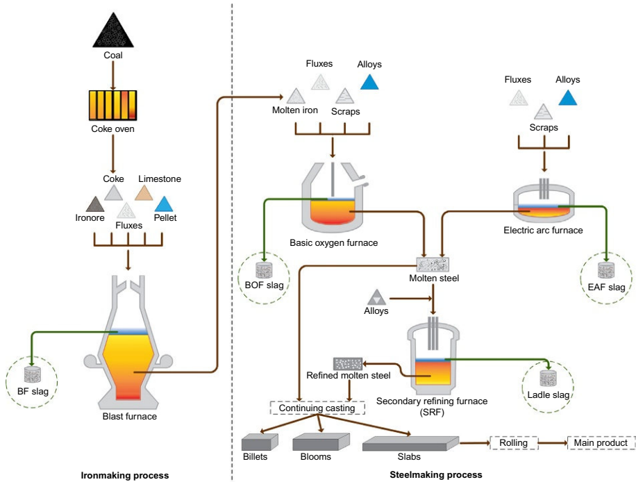
Fig. 2.1 The integrated iron- and steelmaking process and ferrous slag generation.
