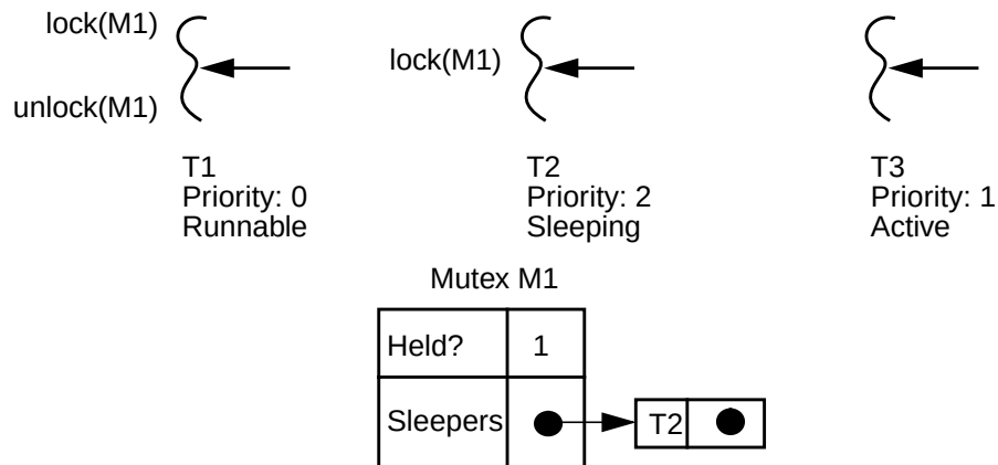
Figure 7-3 Priority Inversion
