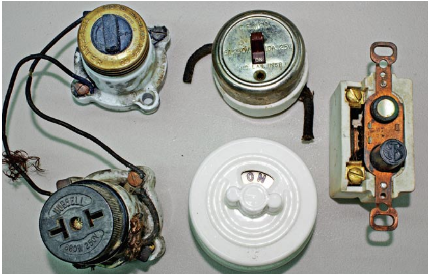
Switch evolution. On left, a screw-in switch and receptacle (very early Hubble configuration). Then came the early snap switches (middle) and then the ever-popular push button (right).
