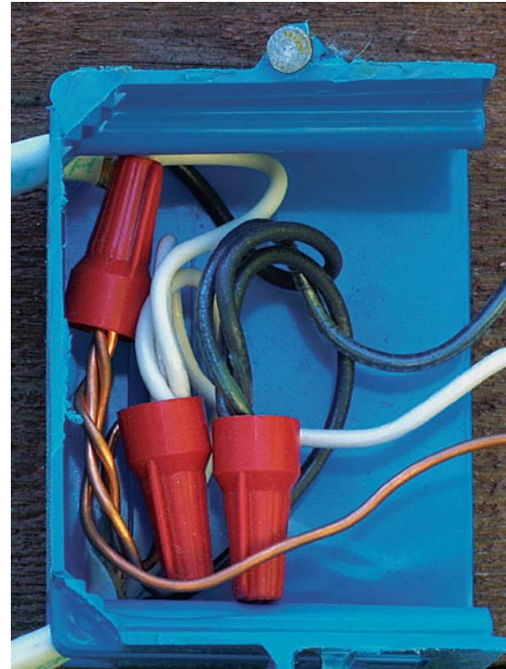
This cutaway view shows the order in which to fold wires back into a box: first the grounds, then the neutrals, then the hot wires. The pigtails to the receptacle are prebent so that they fold neatly into the box.
