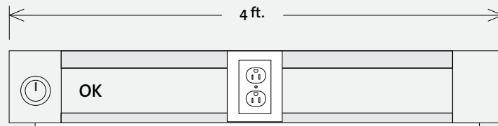
Receptacle-mounted heater
