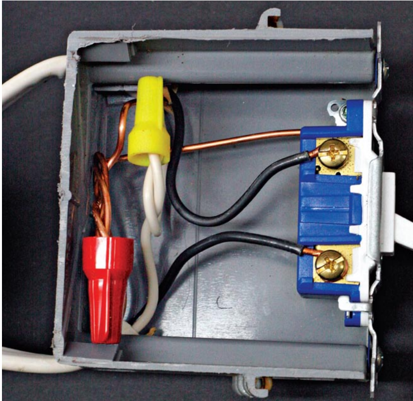
Cutaway view of a switch in the outlet box. Fold the grounds first (pigtail the ground wire over to the switch), the neutrals second, and accordion the hot switch wires back last.
