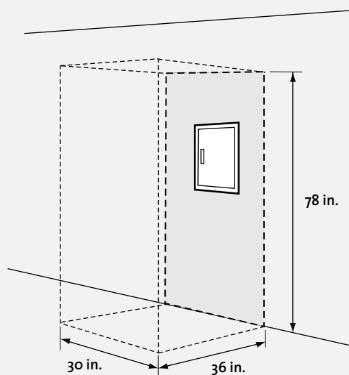
Clearances at the Panel
