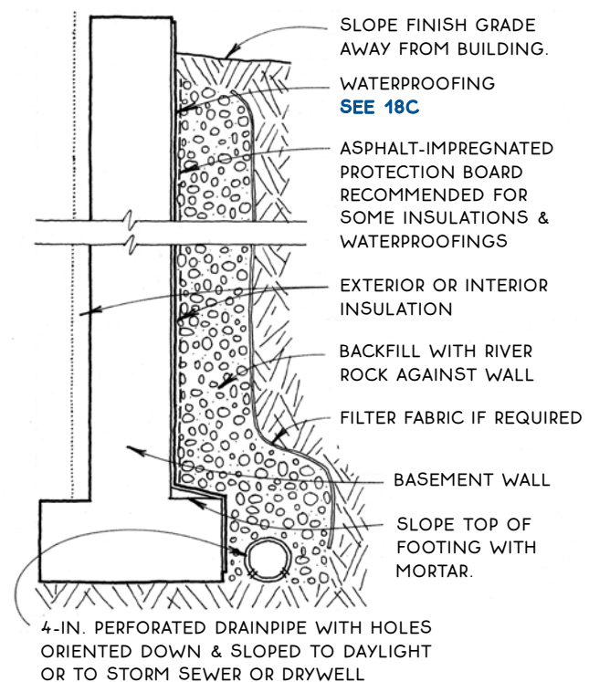
B BASEMENT DRAINAGE
