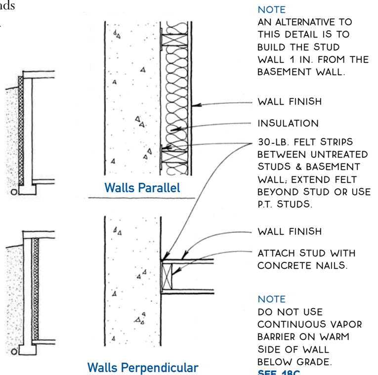
D BASEMENT WALL/STUD WALL Plan Views
