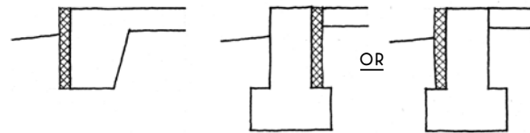
TURNED-DOWN FOOTINGS SEE 22C & D, 23C
