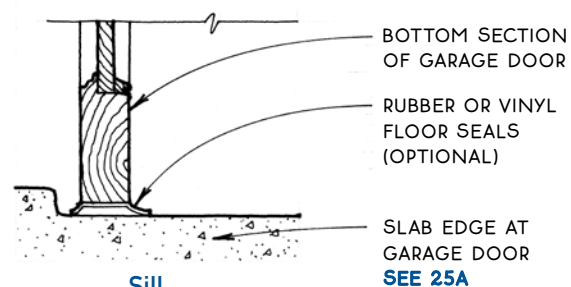
Sill
