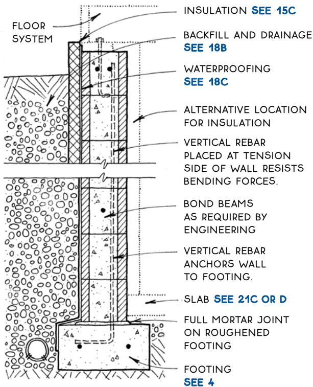
A BASEMENT WALL Concrete Block
