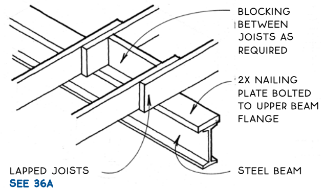
Joists on Nailing Plate
