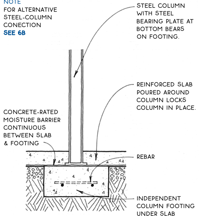
Steel Column
