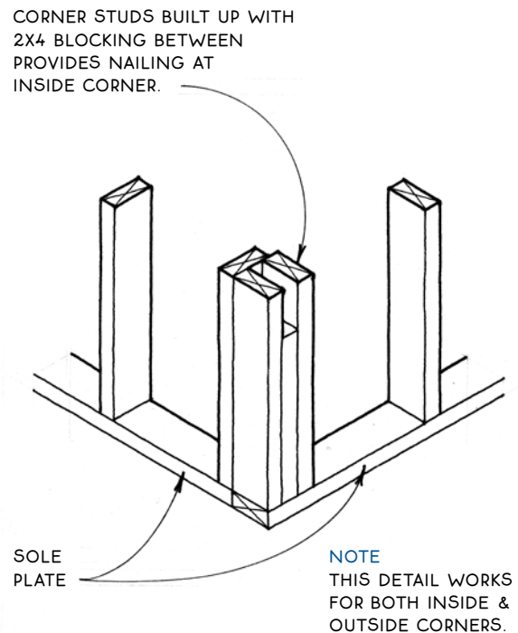
D 2X4 CORNER At Sole Plate
