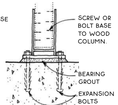
Drilled Base
