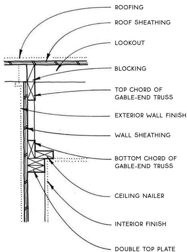
Truss/Gable-End Wall
