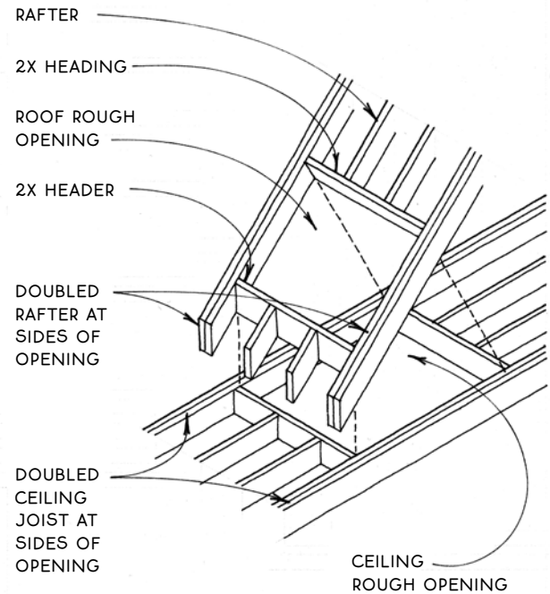
Framing Isometric
