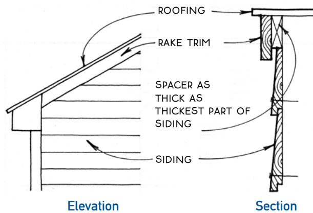
Rake Details
