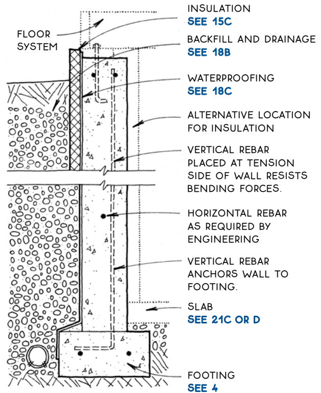
B BASEMENT WALL Concrete
