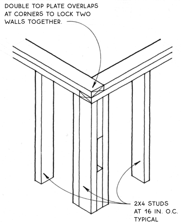
B 2X4 CORNER At Double Top Plate
