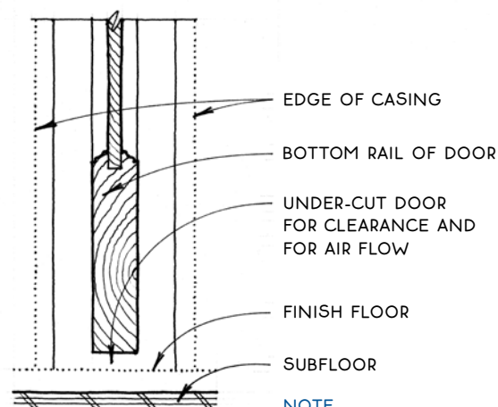
Sill
