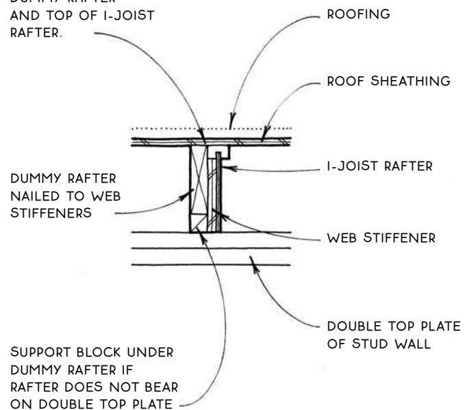
Section Parallel to Eave
