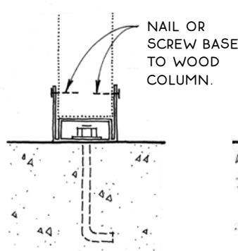
Adjustable Base
