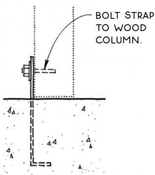
Single Strap
