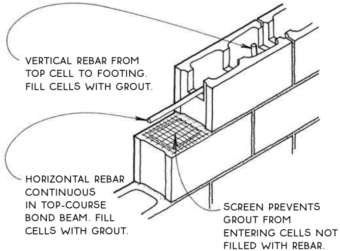
A CONCRETE-BLOCK FOUNDATION Rebar Placement
