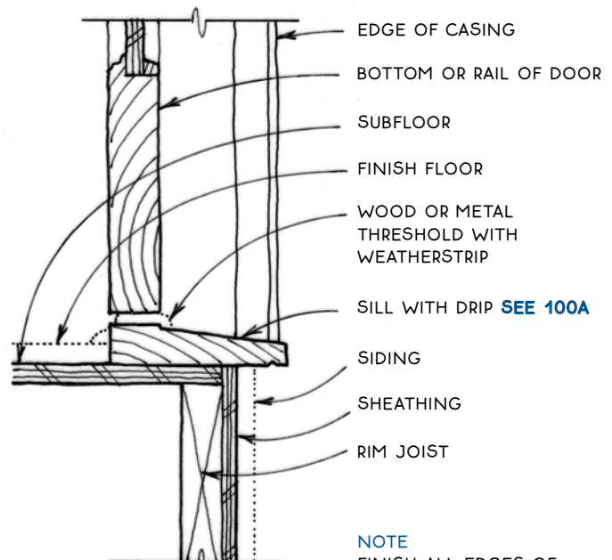
Sill
