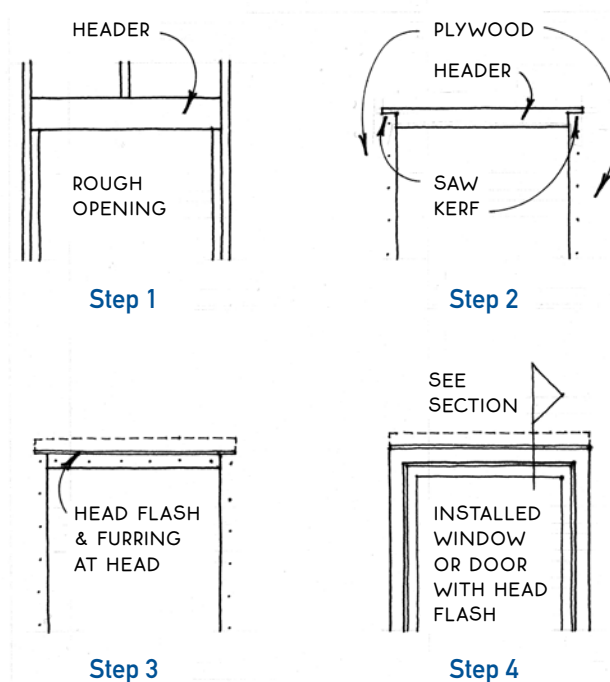
Flashing a Header
