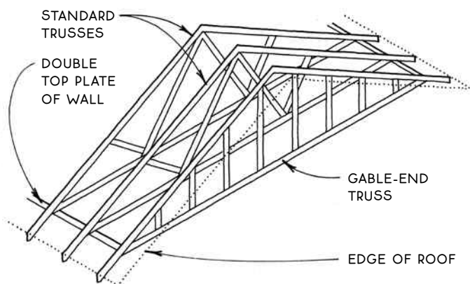
Truss/Gable-End Wall
