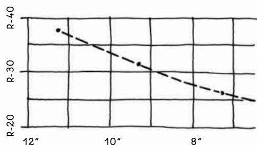
REDUCTION OF R-VALUE IN BATT INSULATION DUE TO COMPRESSION
