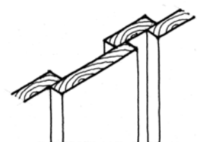
REVERSE BOARD AND BATTEN
