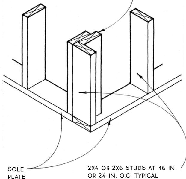
C 2X4 OR 2X6 CORNER At Sole Plate
