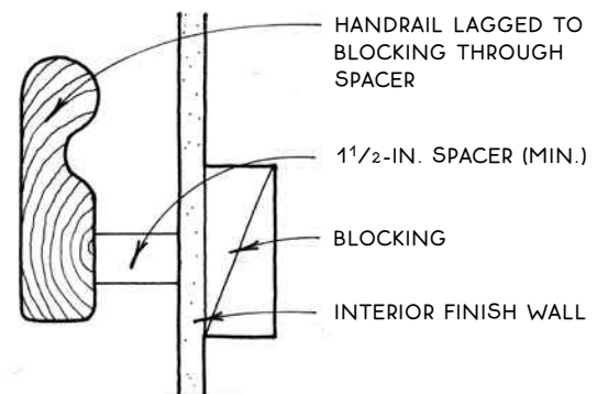
Handrail Screwed to Wall through Spacer
