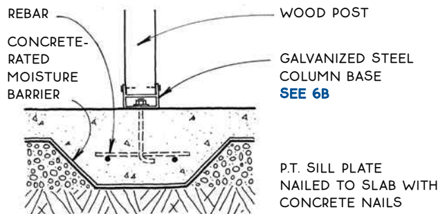
Wood Post
