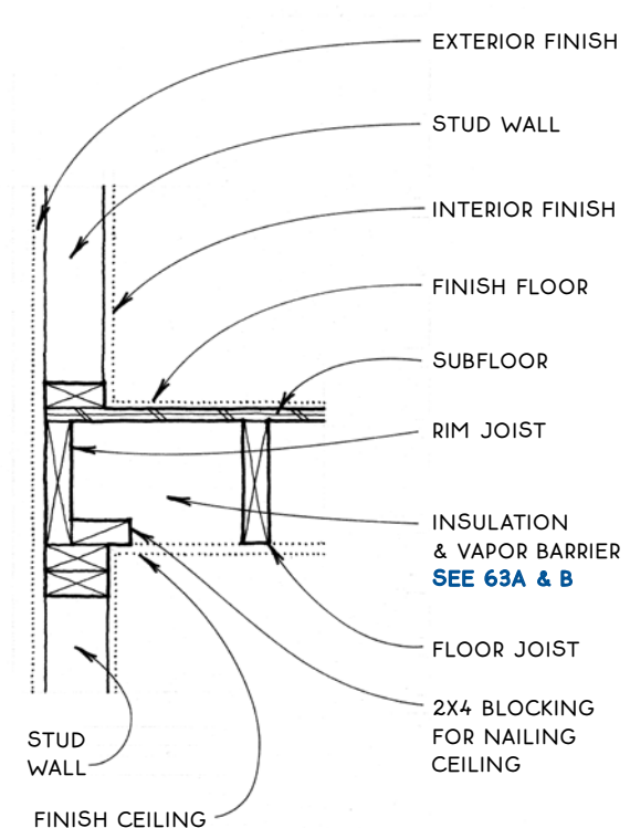
B JOISTS AT EXTERIOR WALL Joist Parallel to Wall
