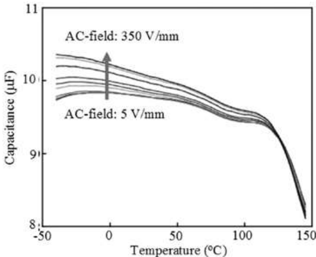
Figure 7. Variation of a nominal capacitance of 10 µF with temperature.
