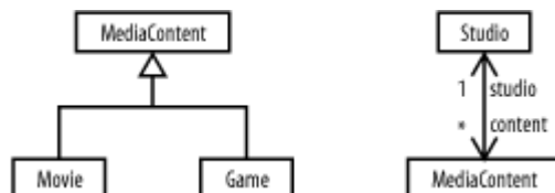
Figure 4-2. Studio and MediaContent classes in com.mediamania.content package
