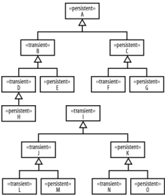
Figure 4-1. Persistence within an inheritance hierarchy
