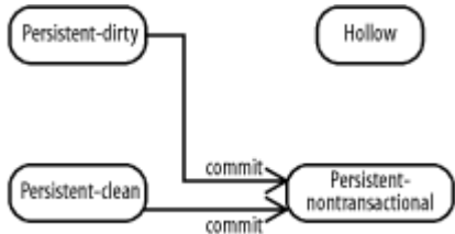
Figure 15-2. State transitions during optimistic transactions
