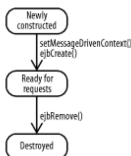
Figure 17-3. The lifecycle of a message-driven bean
