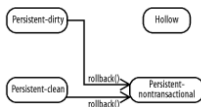
Figure 14-3. Rollback with RestoreValues true
