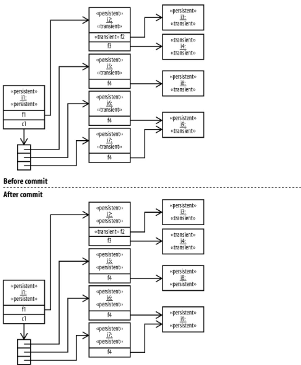
Figure 8-1. Persistence-by-reachability
