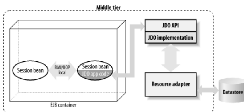
Figure 3-12. EJB session beans using session bean delegates
