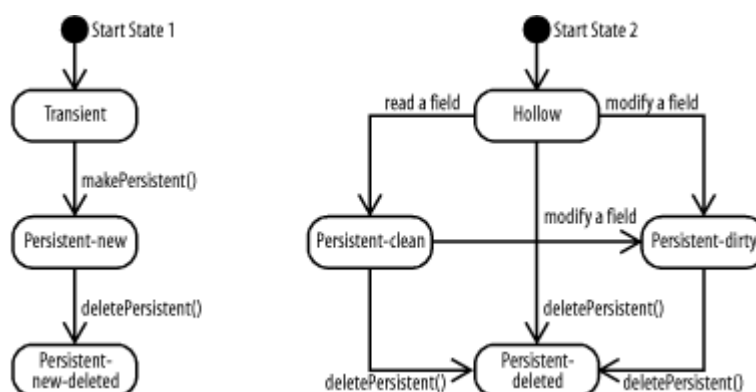
Figure 11-1. Lifecycle-state transitions
