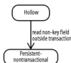
Figure 14-1. State transitions outside a transaction
