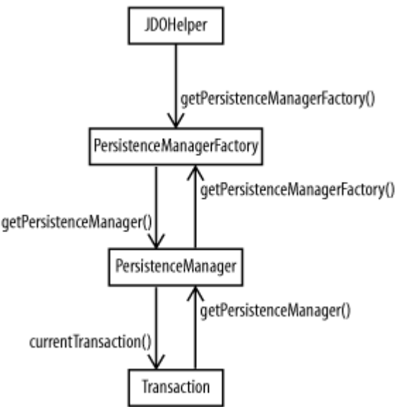
Figure 7-1. Interfaces used to configure and control the JDO runtime environment
