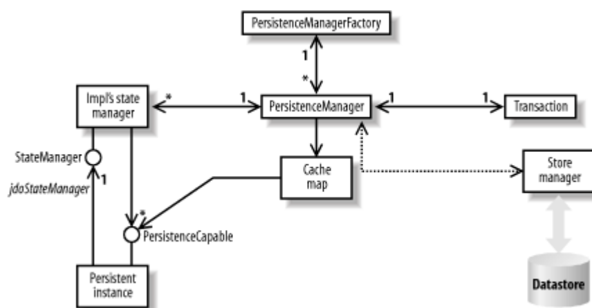
Figure 3-2. UML diagram of persistent instance cache
