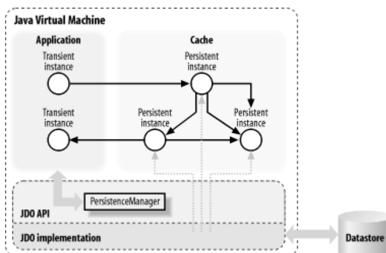
Figure 3-1. Application using a single PersistenceManager to access a datastore
