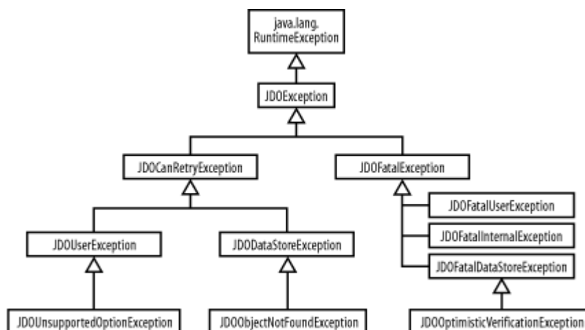
Figure 2-2. JDOException inheritance hierarchy
