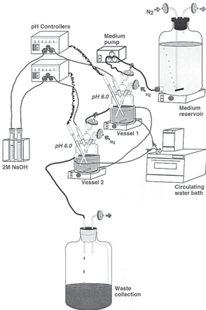
Fig. 3. Schematic diagram showing a simple single-stage continuous culture system.
