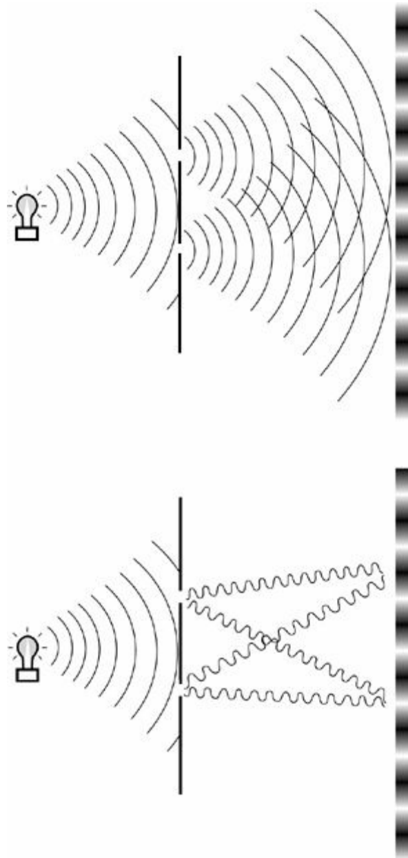
Figure 71 Young's slits experiment viewed from above. Diagram (a) shows light fanning out from the two slits in the partition, interacting and creating a striped pattern on the screen. Diagram (b) shows how individual waves interact. If a trough meets a peak at the screen, the result is a dark stripe. If two troughs (or two peaks) meet at the screen, the result is a bright stripe.
