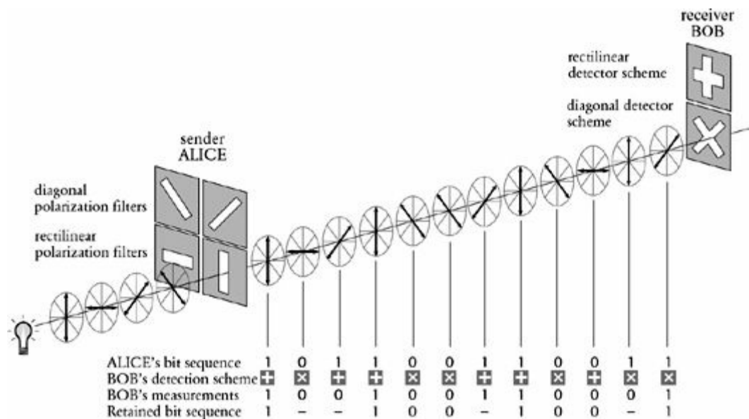
Figure 76 Alice transmits a series of 1's and 0's to Bob. Each 1 and each 0 is represented by a polarized photon, according to either the rectilinear (horizontal/vertical) or diagonal polarization scheme. Bob measures each photon using either his rectilinear or his diagonal detector. He chooses the correct detector for the leftmost photon and correctly interprets it as 1. However, he chooses the incorrect detector for the next photon. He happens to interpret it correctly as 0, but this bit is nevertheless later discarded because Bob cannot be sure that he has measured it correctly.
