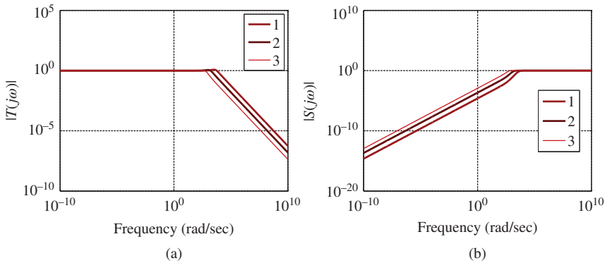
Figure 5.15 Complementary and sensitivity functions for inner-loop current control (PMSM) using PI controller ( \xi = 0.707 , R_s = 2.98 \Omega , and L_q = 7 \times 10^{-3} \text{ H} ) Key: line (1) \gamma = 0.9 , line (2) \gamma = 0.7 , line (3) \gamma = 0.3 . (a) Complementary sensitivity function, and (b) Sensitivity function.
