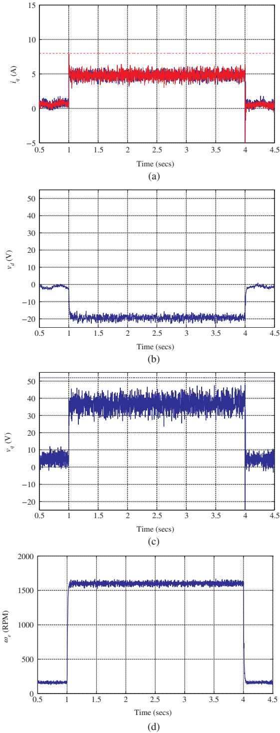
Figure 5.20 Case B. w_n = \frac{1}{1-\gamma} \frac{R_s}{L_q} rad/s, R_s = 2.98 \, \Omega , and L_q = 7 \times 10^{-3} H, \gamma = 0.5 . (a) Current i_q and i_q^* , (b) Voltage v_d , (c) Voltage v_q , and Velocity \omega_e .
