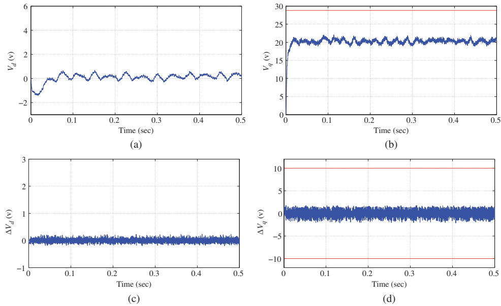
Figure 8.4 Control signal when q_\omega = 0.01 . (a) Control signal v_d , (b) Control signal v_q , (c) Difference of the control signal \Delta v_d , and (d) Difference of the control signal \Delta v_q .
