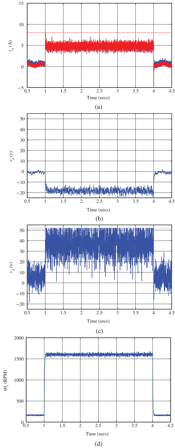
Figure 5.19 Case A. w_n = \frac{1}{1-\gamma} \frac{R_s}{L_q} rad/s, R_s = 2.98 \, \Omega , and L_q = 7 \times 10^{-3} \, \text{H} , \gamma = 0.8 . (a) Current i_q and i_q^* , (b) Voltage v_d , (c) Voltage v_q , and (d) Velocity \omega_e .
