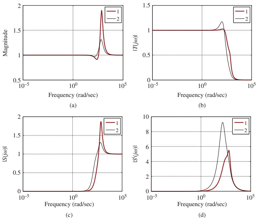
Figure 5.39 Sensitivity functions for outer-loop voltage control (power converter) where PI current controllers are used. Inner-loop current control system has bandwidth 634.9. Key: line (1) w_n = 300 rad/s, line (2) w_n = 150 rad/s. (a) Weighting function, (b) Actual complementary sensitivity function, (c) Actual sensitivity function, and (d) Actual input sensitivity function.
