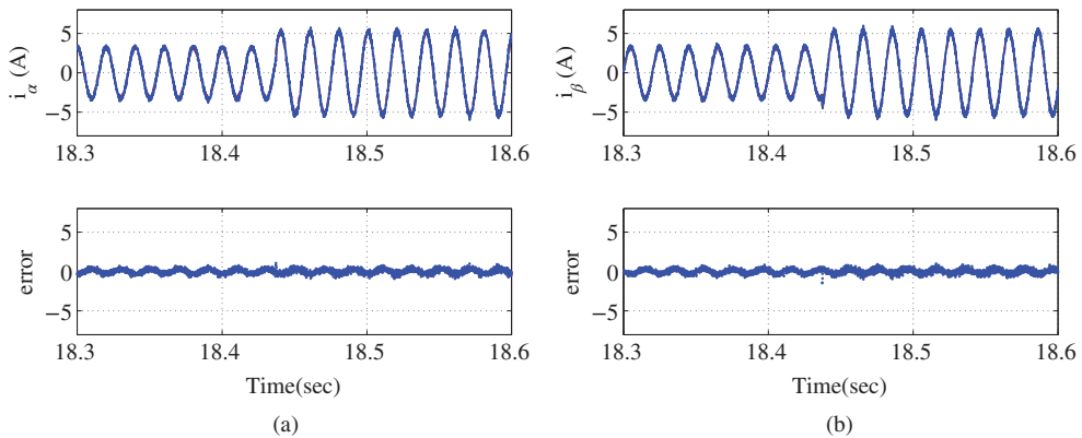
Figure 7.11 Experimental results of current control of power converter using the original FCS scheme in \alpha - \beta reference frame. \Delta t = 80 \mu s . Key: line (1) Actual feedback; line (2) set-point signal. (a) i_\alpha and i_\alpha current error and (b) i_\beta and i_\beta current error.
