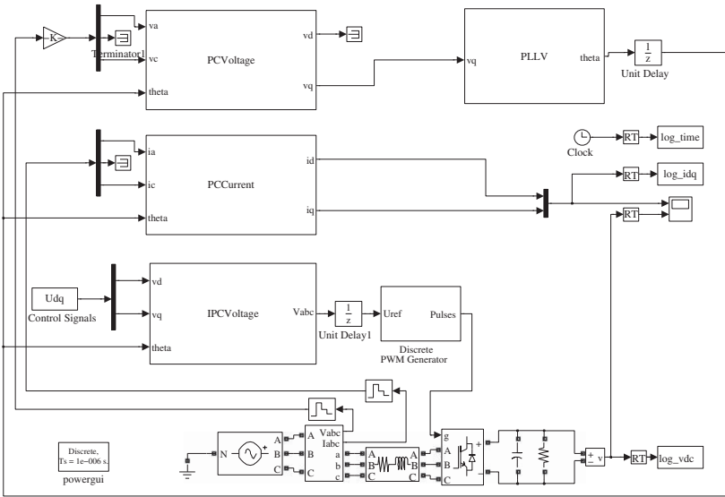
Figure 10.5 Simulink diagram for simulation of grid connected power converter.
