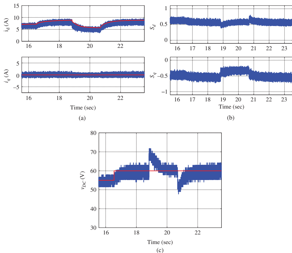
Figure 5.46 Power converter. PI control of q -axis current and P control of d -axis current, \alpha, \gamma = 0.90 , \xi = 0.707 . Outer-loop voltage control system specification: w_n = 80 rad/s and \xi = 0.707 . (a) Current and reference, (b) S_d and S_q , and (c) Output voltage and reference.
