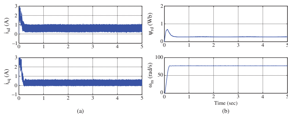
Figure 1.8 Experimental results. (a) i_{sd} and i_{sq} currents and (b) Flux and velocity.
