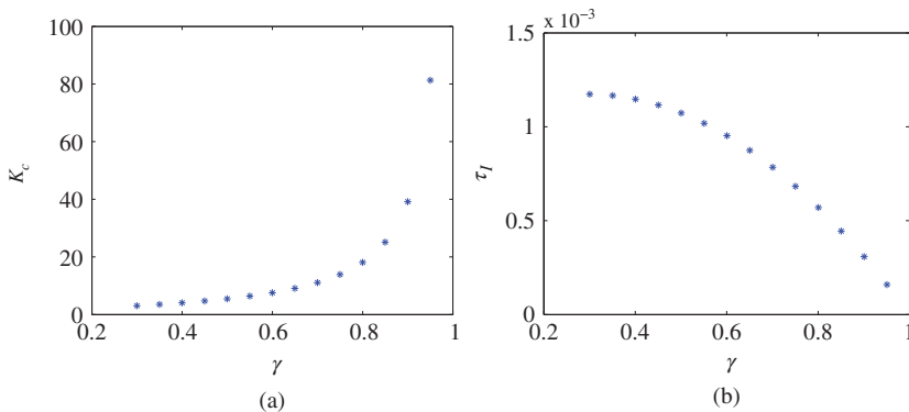
Figure 5.14 Variation of proportional gain and integral time constant for inner-loop current control (PMSM) using PI controller ( \xi = 0.707 , R_s = 2.98 \, \Omega , and L_q = 7 \times 10^{-3} \, \text{H} ). (a) Proportional gain, and (b) Integral time constant.
