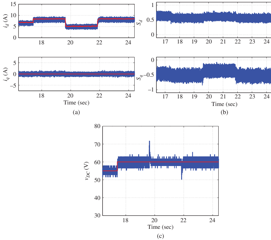
Figure 5.49 Power converter. PI control of q -axis current and P control of d -axis current, \alpha, \gamma = 0.95 , \xi = 0.707 . Outer-loop voltage control system specification: w_n = 300 rad/s and \xi = 0.707 . (a) Current (solid) and reference (dashed), (b) S_d and S_q , and (c) Output voltage (solid) and reference (dashed).
