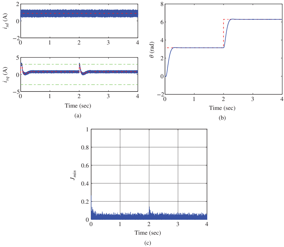
Figure 6.32 Induction motor position control, Case A. Sampling interval \Delta t = 80 \times 10^{-6} sec, k_d = k_q = 0.1 . Bandwidth for the position control system is w_n = 22 rad/s. (a) i_{sd} and i_{sq} currents, (b) Angular position (rad), and (c) Minimum of the objective function.
