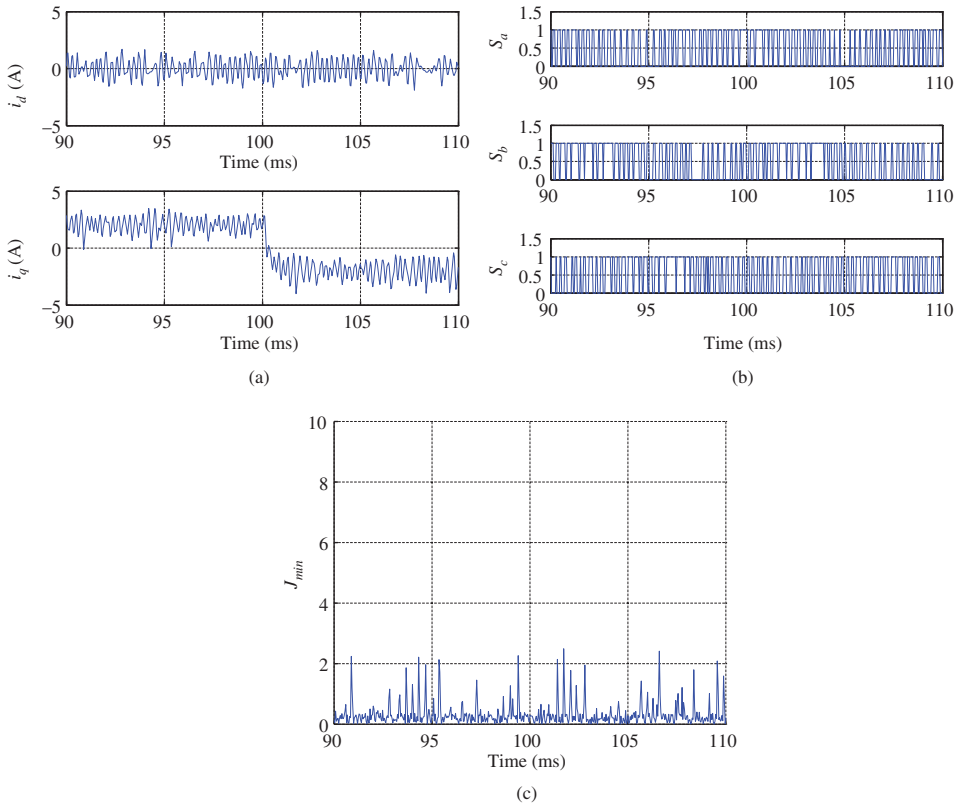
Figure 6.10 Simulation results for I-FCS-MPC of PMSM. Case C. Sampling interval \Delta t = 40 \times 10^{-6} sec, k_d = k_q = 0.1 . (a) i_d and i_q currents, (b) The normalized control signals, and (c) Minimum of the objective function.
