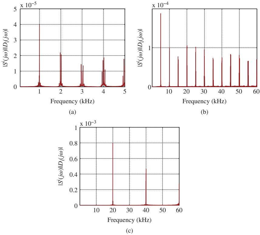
Figure 5.18 |Y_d(j\omega)| = |S^i(j\omega)||D_i(j\omega)| , effect of PWM noise on the current output using PI current control system with varying carrier frequency. The bandwidth w_n = \frac{1}{1-\gamma} \frac{R_s}{L_q} rad/s, R_s = 2.98 \, \Omega , and L_q = 7e-3 \, \text{H} , \gamma = 0.7 . (a) Carrier frequency: 1 kHz, (b) Carrier frequency: 5 kHz, and (c) Carrier frequency: 20 kHz.
