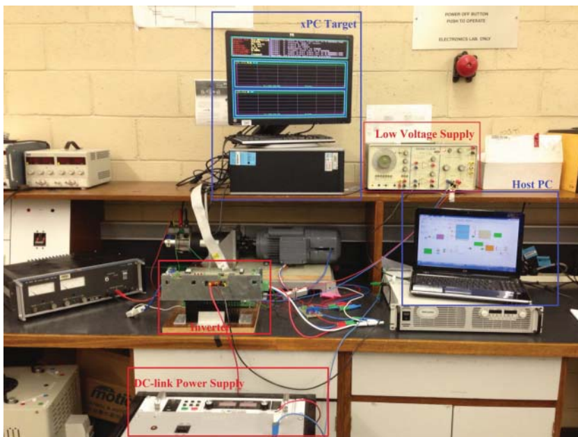
Figure 10.8 Test-bed of the induction motor control experiment.
