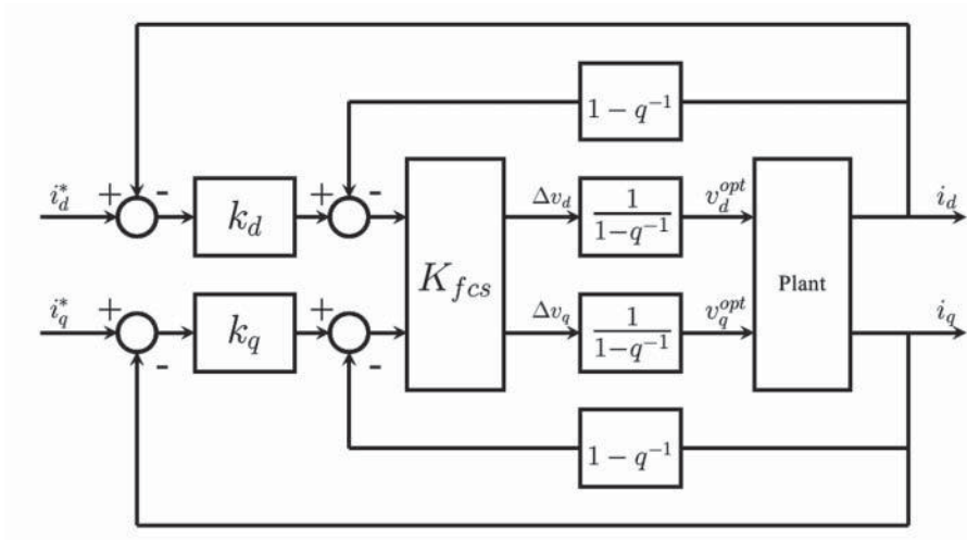
Figure 6.7 I-FCS feedback current control using incremental variables.
