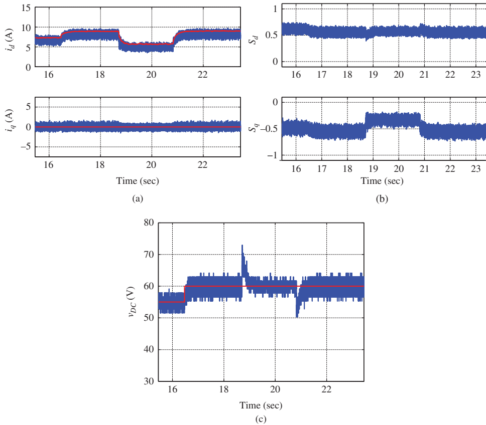
Figure 5.47 Power converter. PI control of q -axis current and P control of d -axis current, \alpha, \gamma = 0.90 , \xi = 0.707 . Outer-loop voltage control system specification: w_n = 150 rad/s and \xi = 0.707 . (a) Current and reference, (b) S_d and S_q , and (c) Output voltage and reference.
