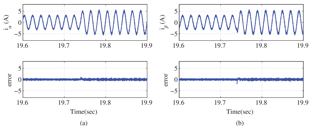
Figure 7.12 Experimental results of current control of power converter using the resonant FCS scheme in \alpha - \beta reference frame. \Delta t = 80 \mu s . Key: line (1) Actual feedback; line (2) set-point signal. (a) i_\alpha and i_\alpha current error and (b) i_\beta and i_\beta current error.
