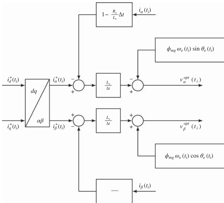
Figure 7.1 FCS-MPC in \alpha - \beta frame.
