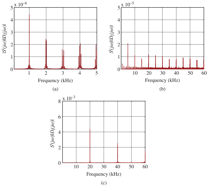
Figure 5.17 |Y_d(j\omega)| = |S'(j\omega)||D_i(j\omega)| , effect of PWM noise on the current output using PI current control system with varying carrier frequency. The bandwidth w_n = \frac{1}{1-\gamma} \frac{R_s}{L_q} rad/s, R_s = 2.98 \, \Omega , and L_q = 7 \times 10^{-3} \, \text{H} , \gamma = 0.9 . (a) Carrier frequency: 1 kHz, (b) Carrier frequency: 5 kHz, and (c) Carrier frequency: 20 kHz.
