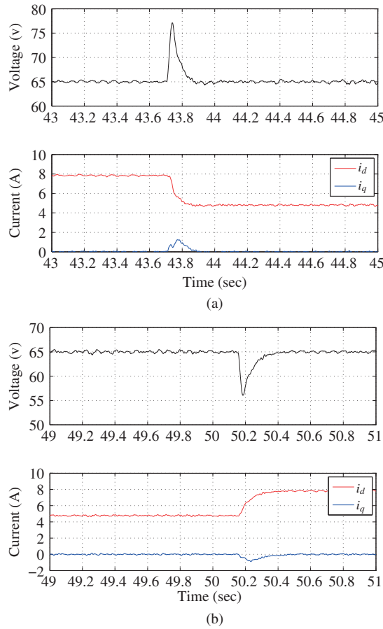
Figure 9.12 Experimental results of CMPC of power converter in disturbance rejection mode though load change. (a) DC bus voltage v_{dc} , i_d and i_q response to a step load change of R_{dc} from 20\ \Omega to 40\ \Omega . (b) DC bus voltage v_{dc} , i_d and i_q response to a step load change of R_{dc} from 40\ \Omega to 20\ \Omega .
