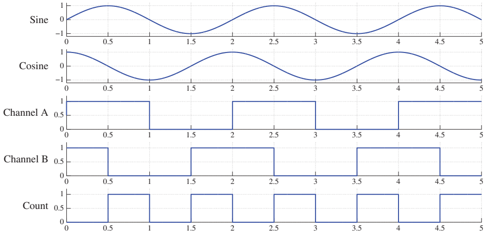
Figure 10.7 Encoder signal.
