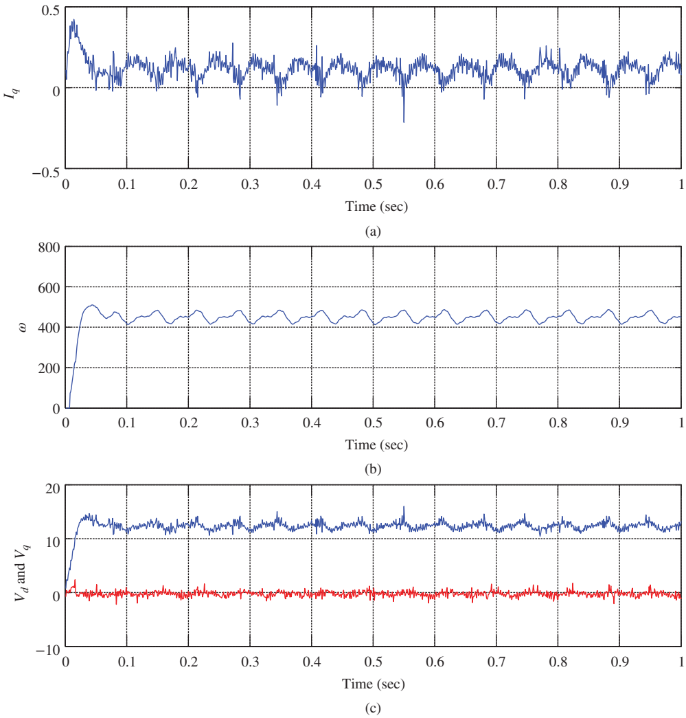
Figure 5.11 Case B. Current control with \alpha = 0.8 , outer-loop velocity control with closed-loop bandwidth: w_n = \frac{1}{1-\gamma}a rad/s, \gamma = 0.98 , a = 2.3404 . Top plot: i_q current; middle plot: output velocity; bottom plot: control variables.
