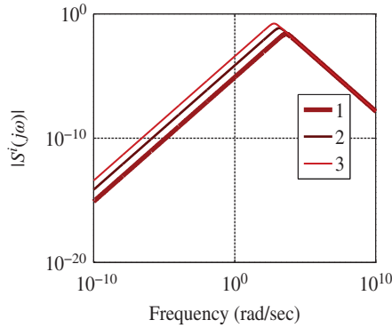
Figure 5.16 Input sensitivity function for inner-loop current control (PMSM) using PI controller ( \xi = 0.707 , R_s = 2.98 \, \Omega , and L_q = 7 \times 10^{-3} \, \text{H} ) Key: line (1) \gamma = 0.9 , line (2) \gamma = 0.7 , line (3) \gamma = 0.3 .
