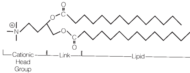
Fig. 1A. Structure of cationic lipids.
