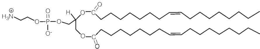
Fig. 1B. DOPE (dioleoylphosphatidylethanolamine).
