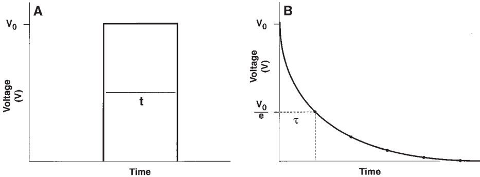
Fig. 1. (A) Square wave pulse. (B) Exponential decay pulse. In the case of square waves, the pulse length t describes the length of time the cell is subjected to the field strength of V_0 . In the case of exponential decay waves, the time constant \tau describes the length of time required to reduce the field strength to 1/e of the initial value.
