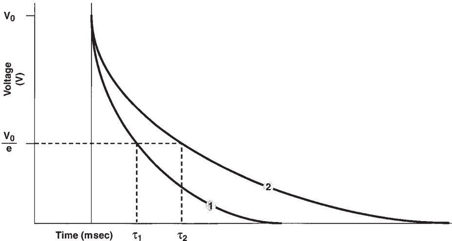
Fig. 2. Voltage decay from a capacitance discharge system according to the equation V = V_0 e^{-t/RC} . In discharge 1 the voltage decreases from V_0 to V_0/e at t = \tau_1 = RC . In discharge 2 the voltage decreases from V_0 to V_0/e at t = \tau_2 = RC , such that \tau_2 = 2\tau_1 . For discharge 2, the longer time constant can be produced by using a capacitor with twice the capacitance as in discharge 1, or by using electroporation media with twice the resistance as in discharge 1 (neglecting ionization effects in the media). Alternatively, by decreasing the sample volume of cuvet 1 by one-half, the resistance of the circuit will increase by approx twofold (see text for details).
