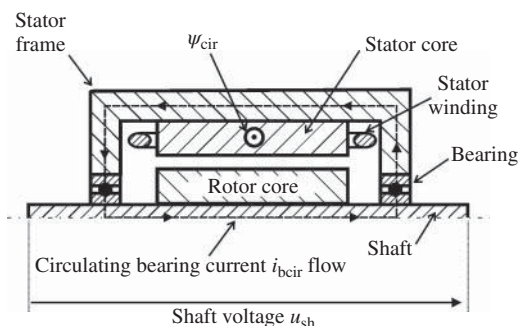
Figure 21.7 The flow path of the circulating bearing current i_{\text{bcir}} [9]
