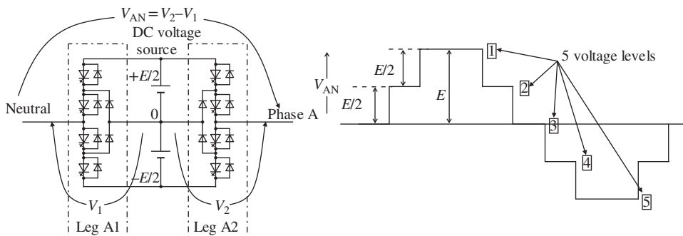
Figure 22.27 Operation principle of star-connected five-level inverter
