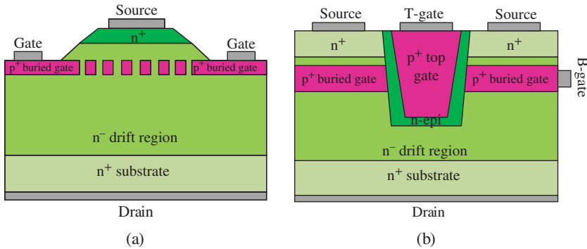
Figure 4.10 (a) Cross-section of the BGJFET and (b) cross-section of the SiC DGTJFET [1]
