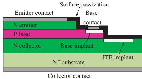
Figure 4.11 Cross-section of the SiC BJT [1]
