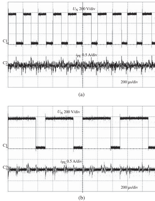
Figure 21.16 Reduction of CM current by decreasing the inverter switching frequency: (a) f_{\text{imp}} = 5 \text{ kHz} and (b) f_{\text{imp}} = 2 \text{ kHz}
