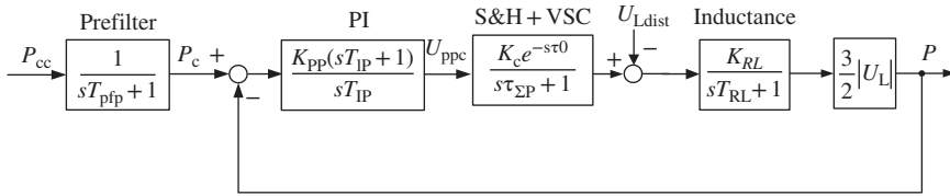
Figure 11.38 Power control loop with prefilter, where P_{cc} is the referenced active power before prefilter, T_{pfp} is the prefilter time constant, which equals the integral time constant of the power PI controller, and U_{Ldist} is the distortion of the grid voltage, for example, caused by higher harmonics
