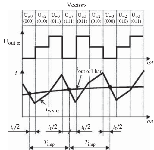
Figure 21.42 The relationship between current sampling instant and inverter output vectors in classical SVM
