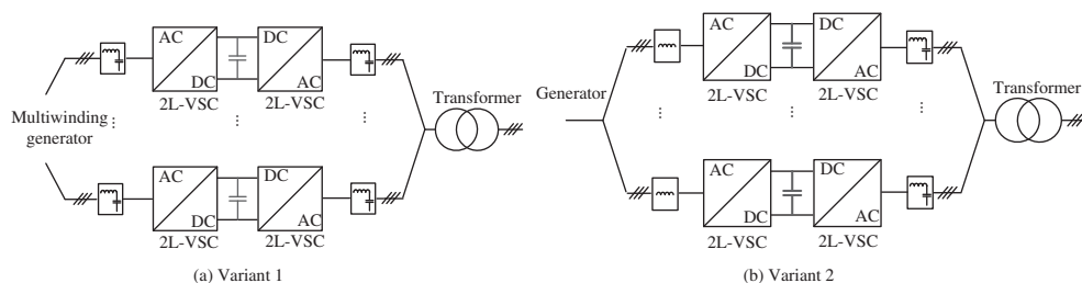
Figure 6.16 Multicell converter with paralleled converter cells (MC-PCC)
