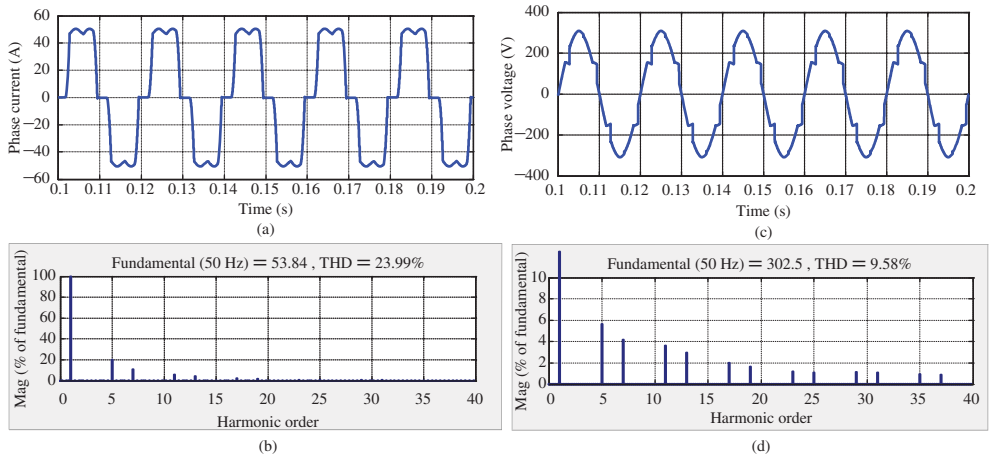
Figure 17.2 Harmonic current source: (a) and (b) source current and its spectrum and (c) and (d) supply voltage and its spectrum (supply impedance 1 mH and 0.1 \Omega )
