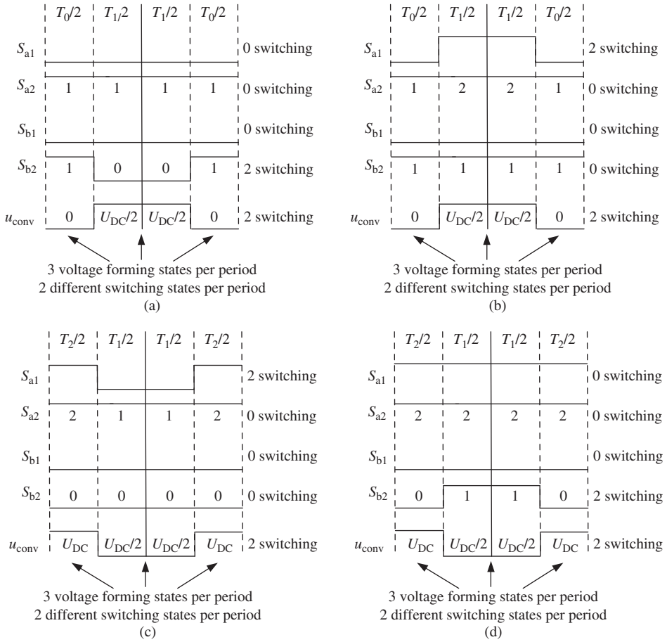
Figure 23.5 Duty cycles for H-DCC with 1D-N2V modulation generating u_{CONV} output voltage level: (a) and (b) positive lower 0 \leq 1/2 U_{DC} \leftrightarrow 0 , (c) and (d) positive upper 1/2 U_{DC} \leftrightarrow U_{DC} \leftrightarrow 1/2 U_{DC} for 10 and 21 redundant switching state selections, respectively
