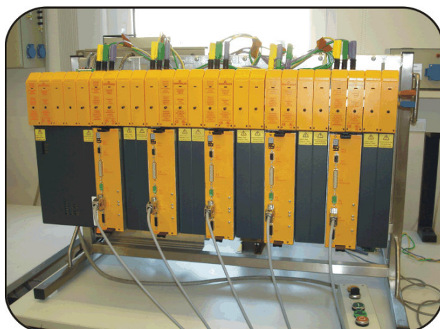
Figure 18A.16 Virtual machine – five inverters in parallel [1]
