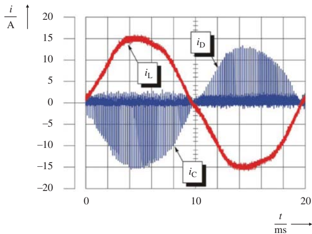
Figure 18A.20 “Load” current and inverter branch current [1]
