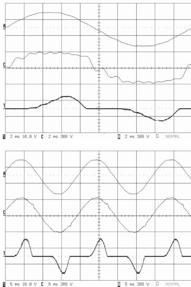
Figure 9.31 Experimental results obtained for the case of distorting load: (a) without shunt converter: A grid voltage (300 V/div), C load voltage (300 V/div), 1 load current (10 V/div); (b) with a shunt converter connected to the grid: A grid voltage (300 V/div), C load voltage (300 V/div), 1 load current (10 V/div) [13]
