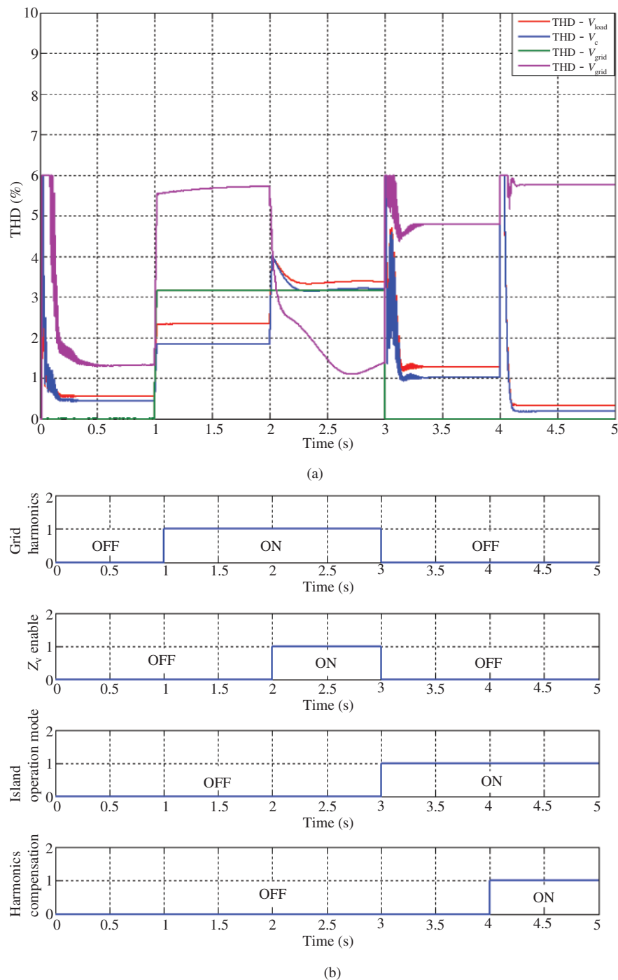
Figure 9.26 (a) PCC voltage and DPGS output current THDs, (b) time slot of different operation modes [35]
