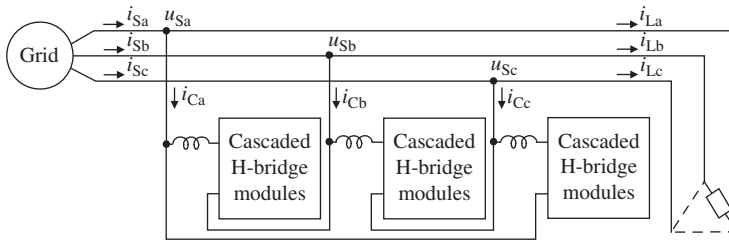
Figure 14.31 Δ-connected CMI-based STATCOM with imbalanced load
