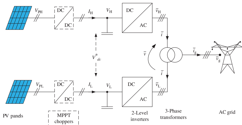
Figure 1.10 Typical configuration of photovoltaic system
