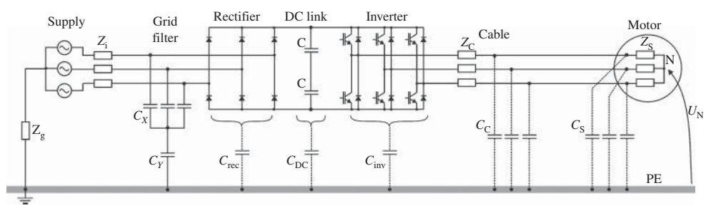
Figure 21.1 The structure of the IM drive for common-mode current flow analysis [4]
