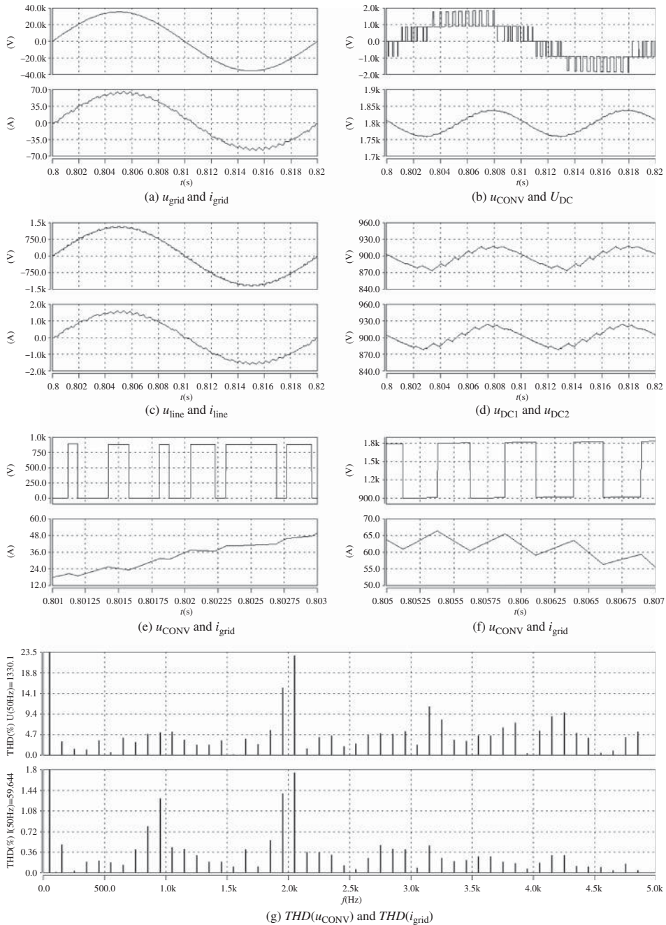
Figure 23.14 Operation of H-DCC with 1D-N3V: (a) grid voltage u_{\text{grid}} and current i_{\text{grid}} , (b) converter voltage u_{\text{CONV}} and DC-link voltage U_{\text{DC}} , (c) line voltage u_{\text{line}} and current i_{\text{line}} , (d) upper and lower DC-link capacitor voltage U_{\text{DC1}} and U_{\text{DC2}} , (e) and (f) two periods zoom for lower and upper u_{\text{CONV}} converter voltage level and grid current i_{\text{grid}} , (g) grid current and converter voltage harmonics spectrum \text{THD}(u_{\text{CONV}}) and \text{THD}(i_{\text{grid}}) .
