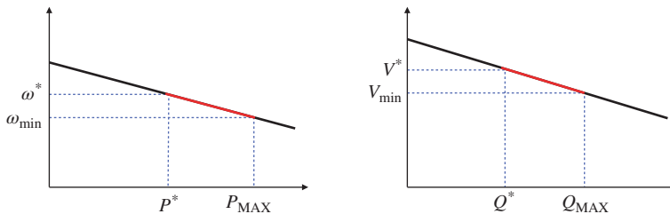
Figure 9.11 Frequency and voltage droop characteristics
