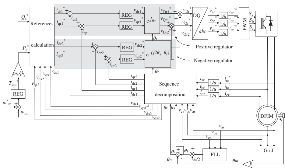
Figure 10.21 Dual-vector control block diagram of a DFIM
