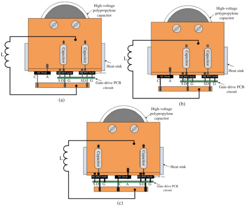
Figure 4.30 Graphical schematics of the various circuit layouts (a) circuit layout L1, (b) circuit layout L2 and (c) circuit layout L3 [45]
