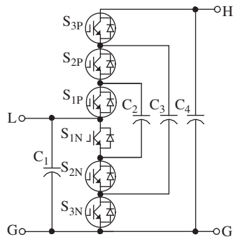
Figure 14.46 1X converter
