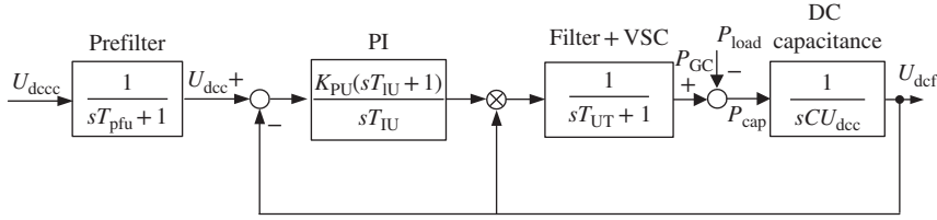
Figure 11.39 Block diagram for a simplified DC-link voltage control loop, where U_{dccc} is the referenced DC voltage before prefilter, T_{pfu} is the DC voltage prefilter time constant, and P_{GC} is the grid-side converter active power
