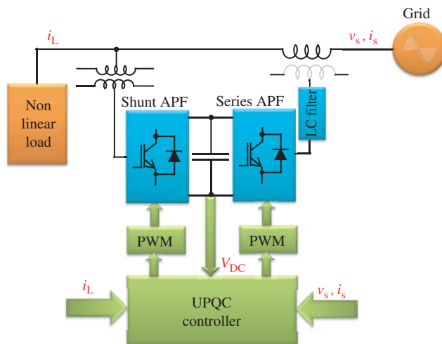
Figure 17.29 UPQC
