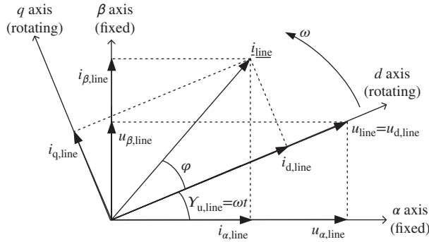
Figure 23.19 Coordinate transformation of line current vector \underline{i}_{\text{line}} and line voltage vector \underline{u}_{\text{line}} from stationary \alpha\beta to synchronous rotating dq reference frame coordinates
