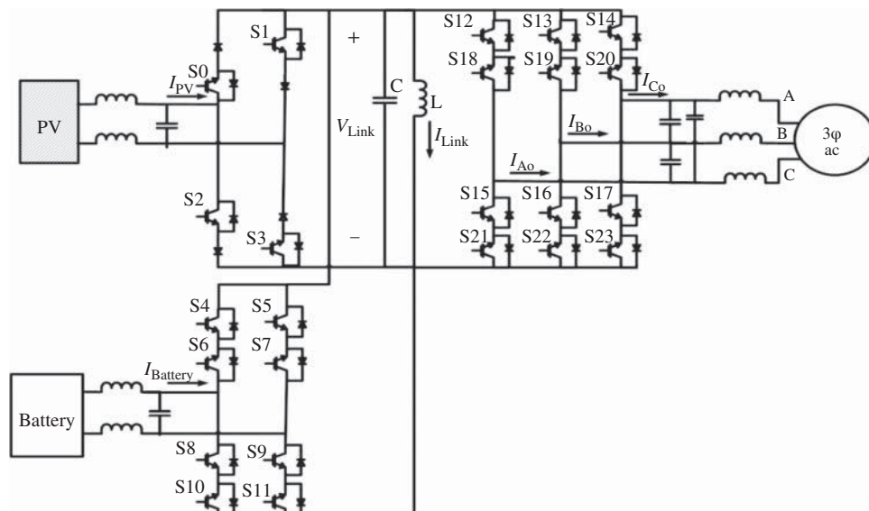
Figure 5.20 Multipoint ac-link universal converter [11]
