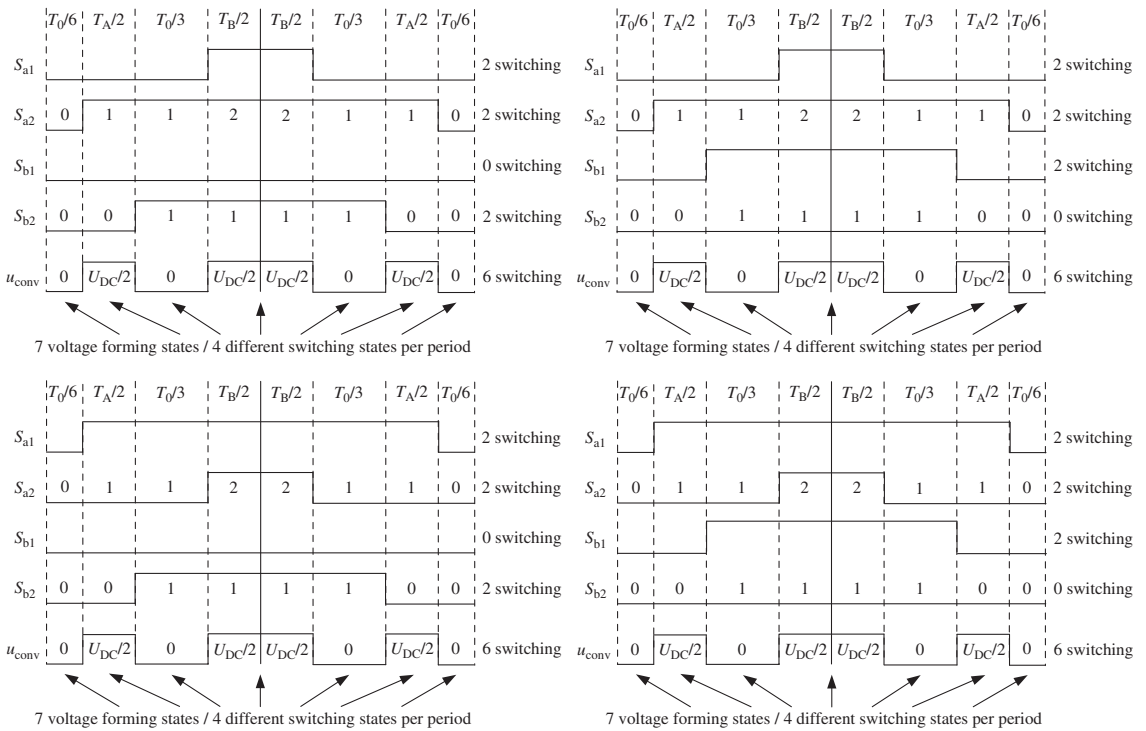
Figure 23.9 Duty cycles for the H-FCC with 1D-N3V modulation generating u_{conv} lower positive output voltage level 0 \leftrightarrow \frac{1}{2}U_{DC} \leftrightarrow 0 with different redundant switching states
