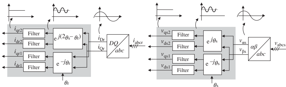
Figure 10.22 Sequence decomposition
