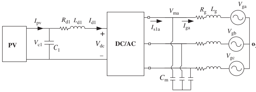
Figure 8.13 A PV generator system with a current source inverter connected through LCL filter to the grid
