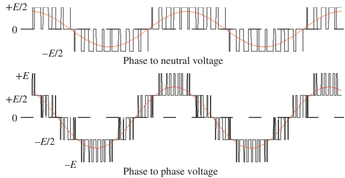
Figure 22.25 Voltage waveforms of NPC three-level inverter
