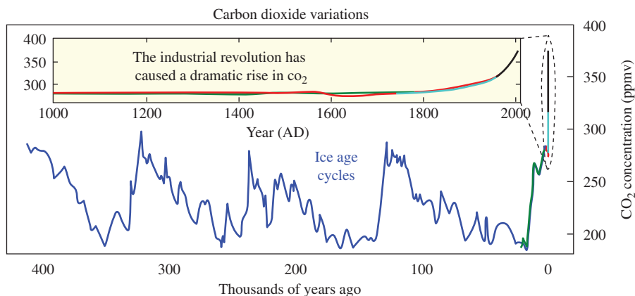
Figure 1.4 \text{CO}_2 variation in atmosphere thousands of years ago [4]
