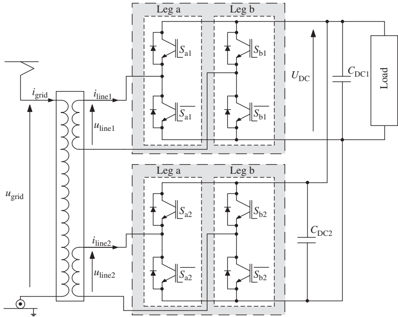
Figure 23.1 Single-phase five-level parallel-connected H-bridge converter
