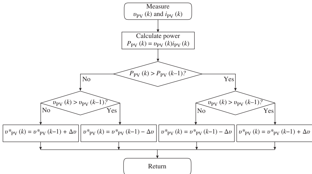
Figure 7.21 P&O algorithm
