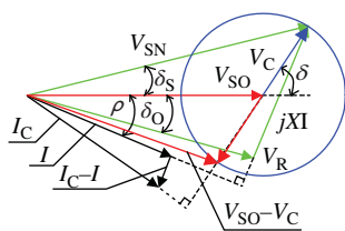
Figure 14.35 Phasor diagram
