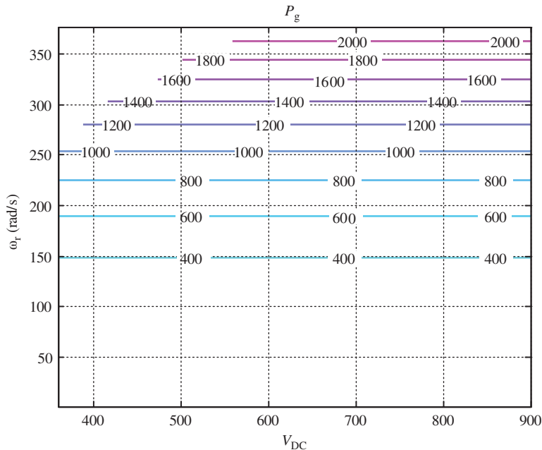
Figure 8.11 Active power flowing into the grid
