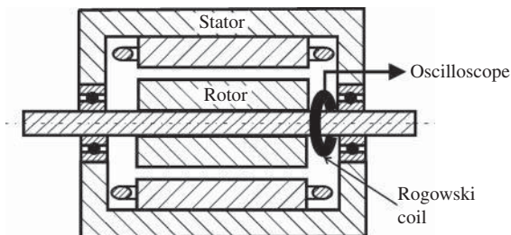
Figure 21.8 The use of a Rogowski coil for circulating current i_{\text{bcir}} measurement [10]
