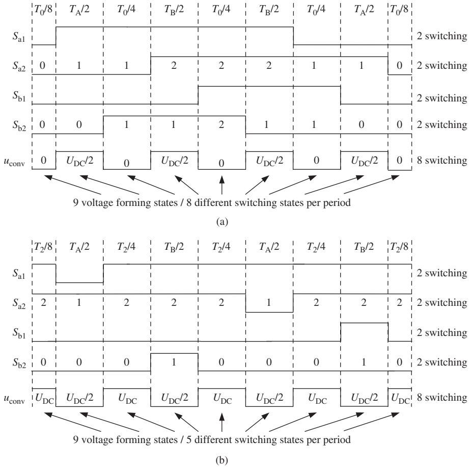
Figure 23.11 Duty cycles for the H-FCC with 1D-N(3+2R)V modulation generating u_{\text{CONV}} output voltage level: (a) positive lower 0 \leftrightarrow \frac{1}{2}U_{\text{DC}} \leftrightarrow 0 and (b) positive upper \frac{1}{2}U_{\text{DC}} \leftrightarrow U_{\text{DC}} \leftrightarrow \frac{1}{2}U_{\text{DC}}
