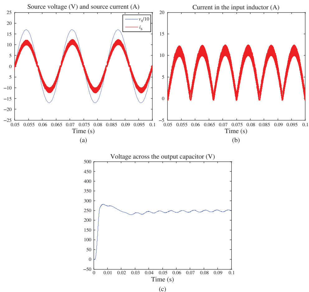
Figure 16.15 Simulation results given by the hysteresis-based control system at a rated load: steady-state waveforms of (a) the source voltage ( v_s ) and the source current ( i_s ), (b) the current in the input inductor ( i_{in} ) and (c) transient waveform of the voltage across the output capacitor ( v_{out} ) following a start-up [97]
