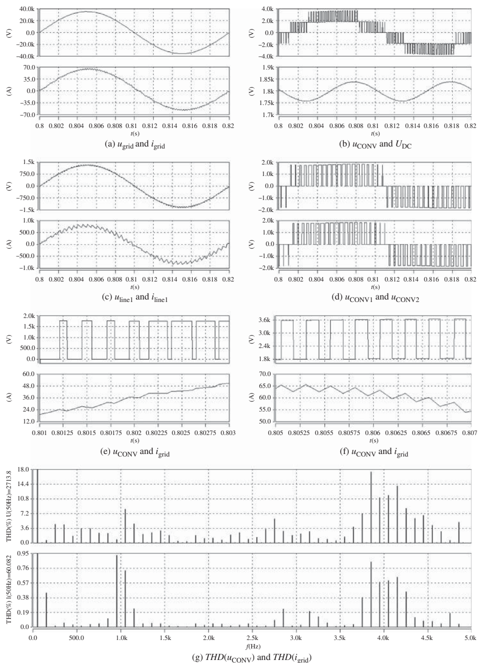
Figure 23.13 Operation of parallel-connected H-BC with UPWM: (a) grid voltage u_{\text{grid}} and current i_{\text{grid}} , (b) converter voltage u_{\text{CONV}} and DC-link voltage U_{\text{DC}} , (c) module 1 line voltage u_{\text{line1}} and current i_{\text{line1}} , (d) module 1 and 2 voltage u_{\text{CONV1}} and u_{\text{CONV2}} (e) and (f) two periods zoom for lower and upper u_{\text{CONV}} converter voltage level and grid current i_{\text{grid}} and (g) grid current and converter voltage harmonics
