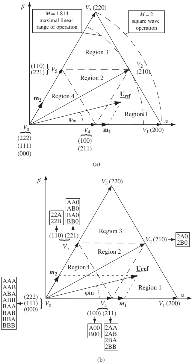
Figure 11.10 First sector with all possible switching states for (a) DCC and (b) FCC topologies
