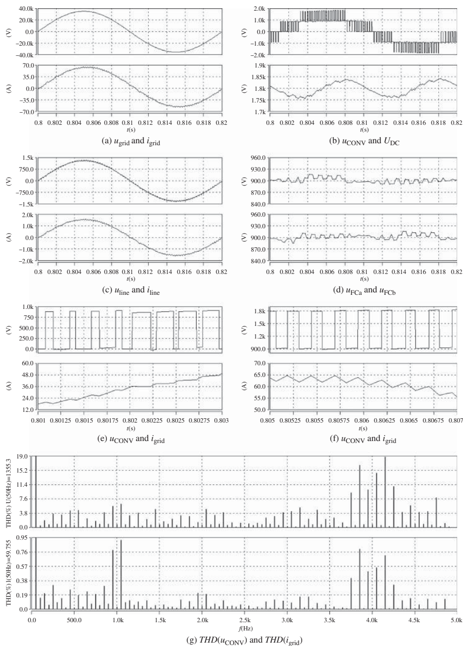
Figure 23.15 Operation of H-FCC with 1D-N(3 + 2R)V: (a) grid voltage u_{\text{grid}} and current i_{\text{grid}} , (b) converter voltage u_{\text{CONV}} and DC-link voltage U_{\text{DC}} , (c) line voltage u_{\text{line}} and current i_{\text{line}} , (d) flying capacitor voltages U_{\text{FCa}} and U_{\text{FCb}} , (e) and (f) two periods zoom for lower and upper u_{\text{CONV}} converter voltage level and grid current i_{\text{grid}} and (g) grid current and converter voltage harmonics spectrum THD(u_{\text{CONV}}) and THD(i_{\text{grid}}) .
