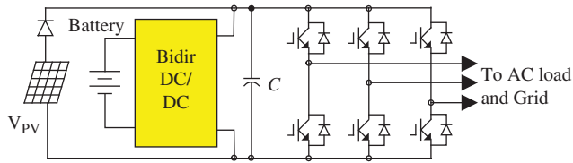
Figure 24.8 Traditional scheme
