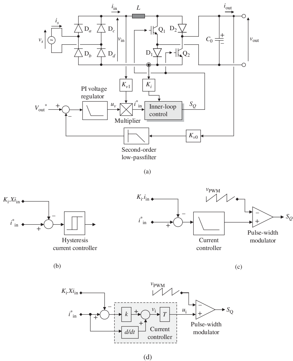
Figure 16.14 (a) Control system with different control strategies for the inner loop, (b) hysteretic control, (c) carrier-based linear control and (d) carrier-based nonlinearity compensating control [97]
