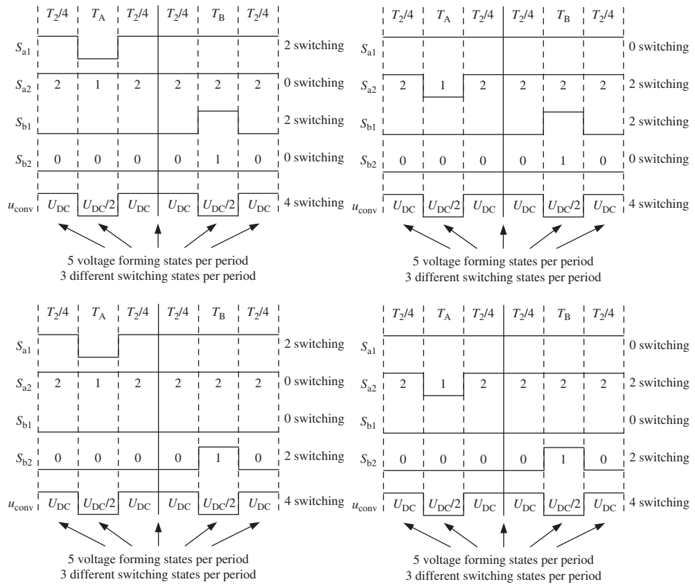
Figure 23.10 Duty cycles for the H-FCC with 1D-N3V modulation generating u_{\text{CONV}} positive upper output voltage level \frac{1}{2}U_{\text{DC}} \leftrightarrow U_{\text{DC}} \leftrightarrow \frac{1}{2}U_{\text{DC}} with different redundant switching states
