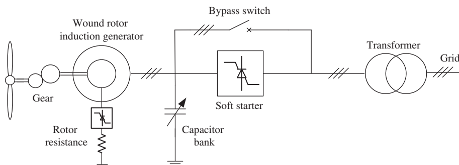
Figure 6.7 Partial-scale variable speed wind turbine with variable rotor resistance
