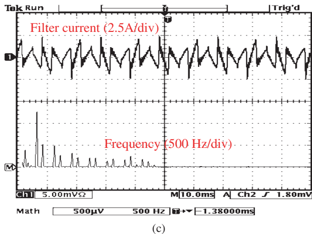
Figure 17.24 Practical results: (a) the load current and its spectrum (5 A/div), (b) the supply current and its spectrum (5 A/div) and (c) the active filter current and its spectrum (2.5 A/div) [62]
