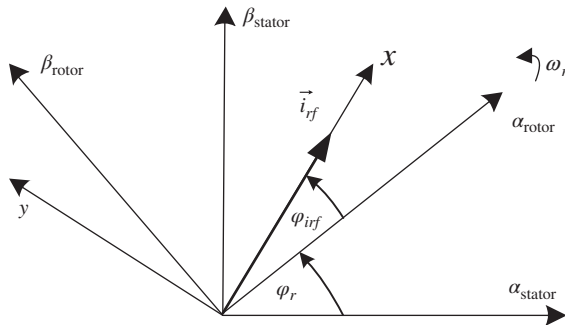
Figure 20.32 The vectors in \alpha\beta_{\text{rotor}} (coordinate system connected with the rotor), \alpha\beta_{\text{stator}} (coordinate system connected with the stator) and xy (coordinate system connected with output current vector \vec{i}_{rf} )
