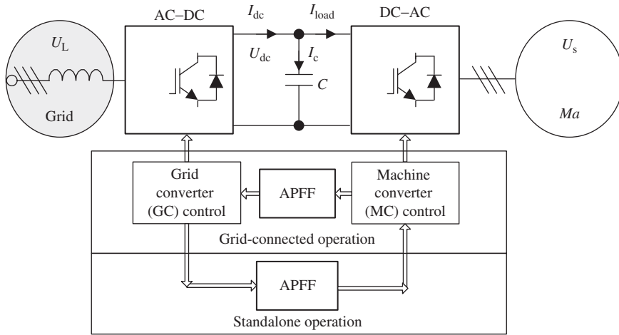
Figure 11.40 Simplified block diagram of the AC–DC–AC converter, which consists of an AC–DC converter, and APFF. Note: Direction of APFF changes in respect of grid-connected or standalone operation
