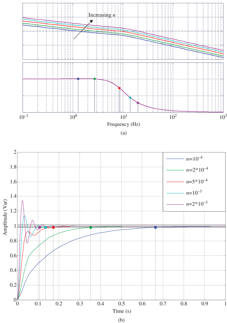
Figure 9.23 (a) Open-loop Bode diagram, (b) step response, (c) family of root locus diagram of the reactive power loop in the case of proportional gain variations fixing the integral gain at TiQ=0.03
