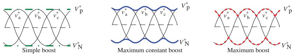
Figure 24.6 Three boost control methods with different V_p^* and V_N^*
