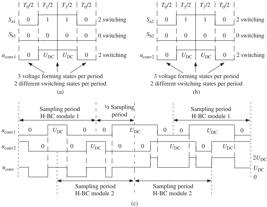
Figure 23.2 Duty cycles for parallel-connected H-BC with hybrid modulation: (a) module 1, (b) module 2 and (c) parallel-connected H-BC u_{\text{CONV}} voltages with interleaved sampling periods 1/2 T_s between modules
