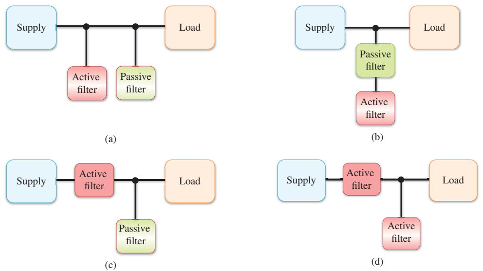
Figure 17.10 Filter combinations: (a) parallel active and passive filters, (b) active filter in series with the parallel passive filter, (c) series active and parallel passive filter and (d) unified power quality conditioner
