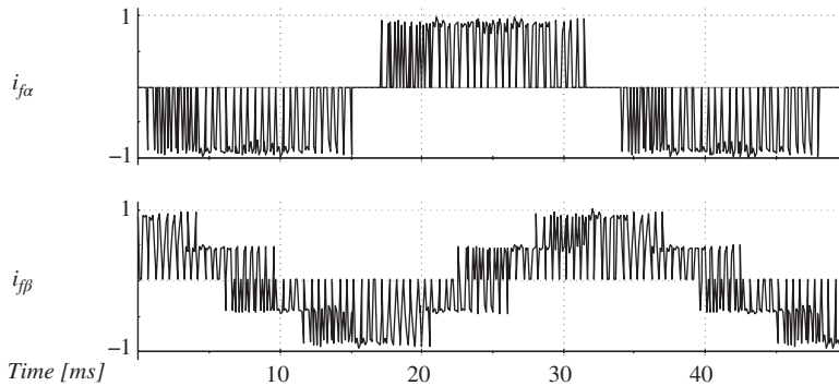
Figure 20.7 The output current vector coefficients in per unit values
