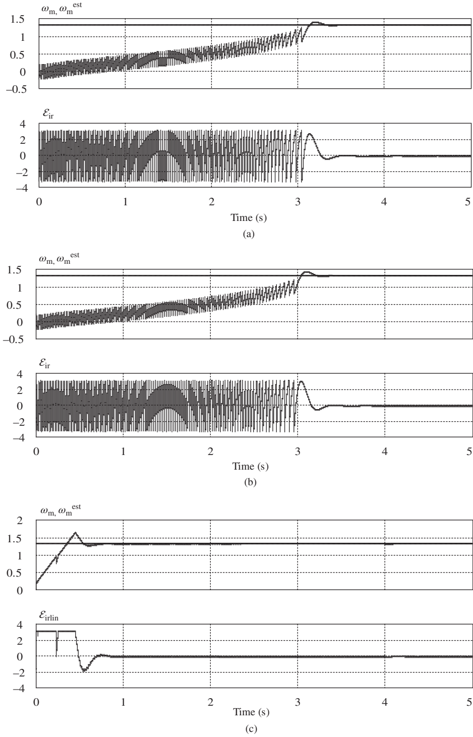
Figure 10.28 Simulation results of modified MRAS observers based on (a, c) the flux–current model and (b, d) the voltage–current model; (a, b) without and (c, d) with linearization of the controller error
