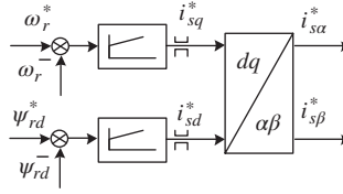
Figure 20.14 The FOC control system structure with PI controllers without decoupling variables
