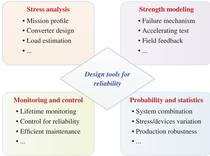
Figure 6.27 Multidiscipline approaches for more reliable power electronics
