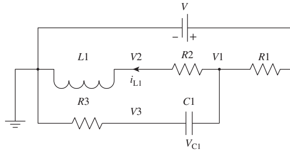
Figure 18B.1 Circuit illustrating state-space versus nodal approach
