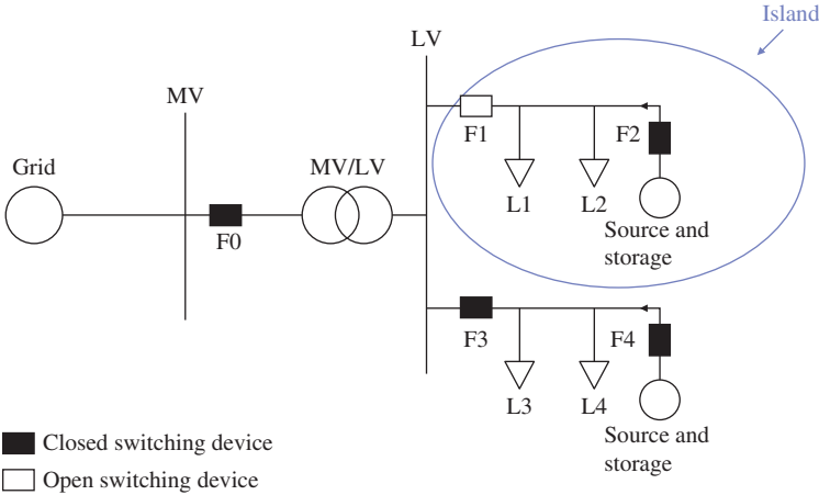
Figure 9.9 Basic microgrid architecture [29]
