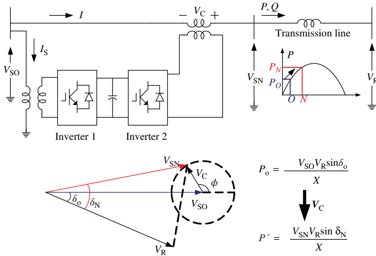
Figure 14.32 Conventional UPFC
