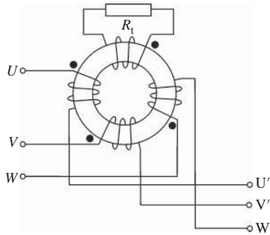
Figure 21.23 Common-mode transformer
