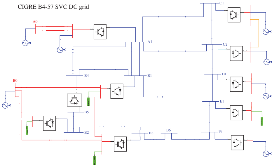
Figure 18B.11 CIGRE B4-57 HVDC grid
