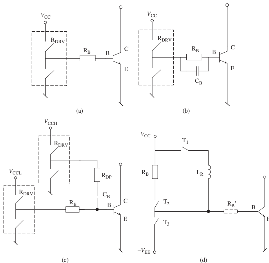
Figure 4.19 Base-drive units for SiC BJT: (a) simple totem-pole driver, (b) driver with speed-up capacitor, (c) dual source with resistors and capacitors (2SRC) and (d) current source driver [36, 37]
