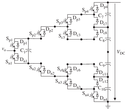
Figure 14.22 Active NPC converter III
