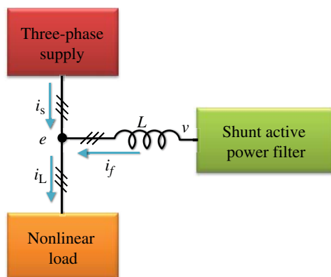
Figure 17.17 Shunt APF single-line diagram [62]
