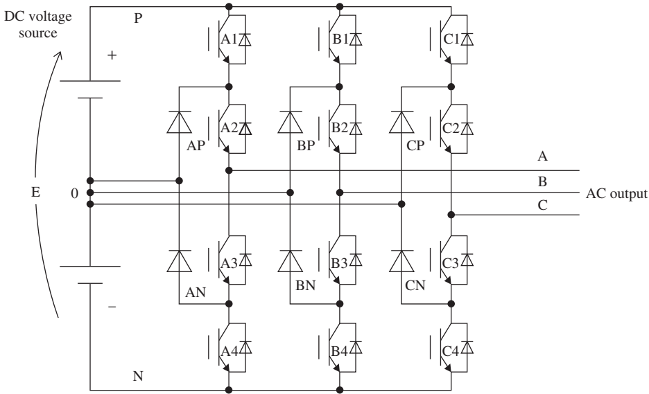
Figure 22.23 Circuit configuration of NPC three-level inverter
