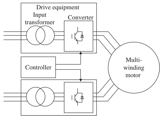
Figure 22.14 Multiwinding motor drive using dual converters
