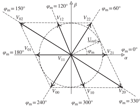
Figure 11.19 Space vector V_{(S_a, S_b)} representation of three-phase three-level simplified converter
