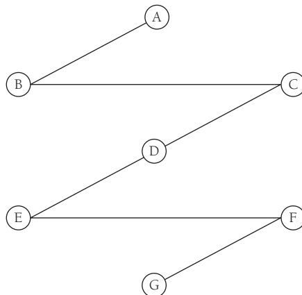
FIGURE 16.8. The Minimum Spanning Tree for Figure 16-7.
