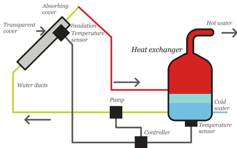
Figure 10.7 Active flat collector system.
