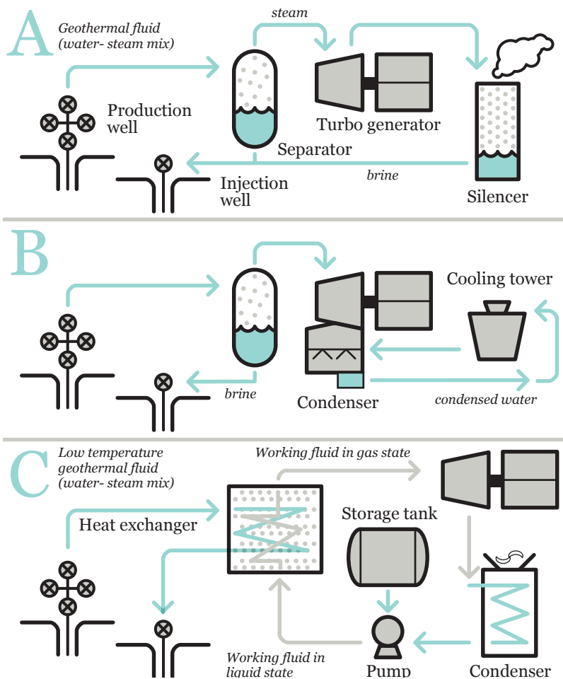
Geothermal generation schemes.
