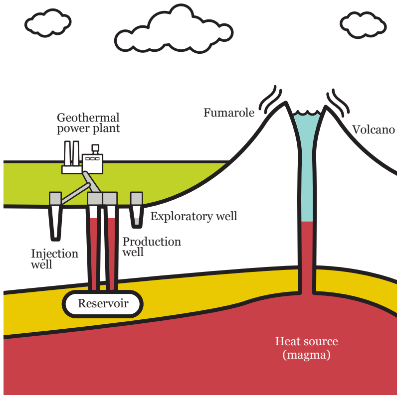
Figure 8.1 Schematic model of a geothermal reservoir.
