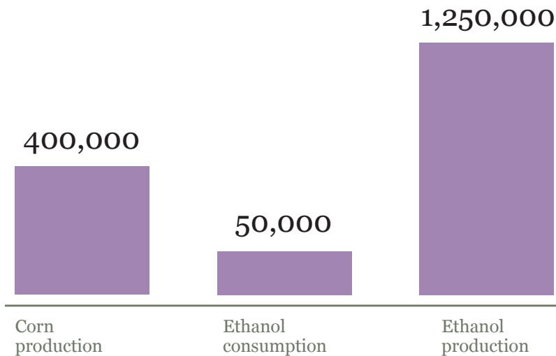
Figure 6.4 Energy requirements in ethanol lifecycle.
