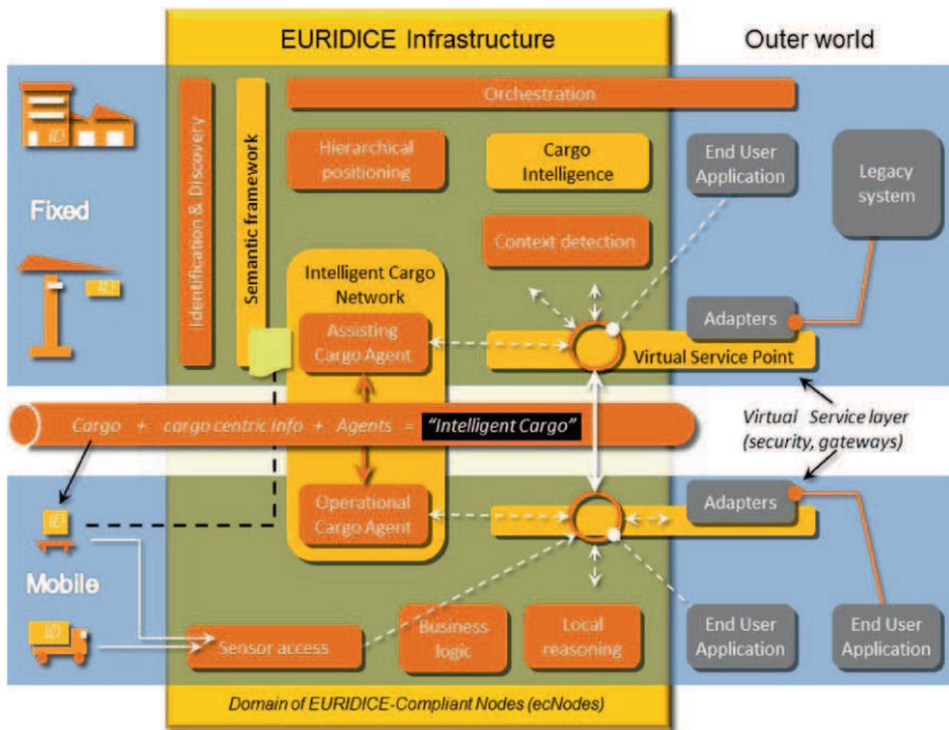
Fig. 12.9 EURIDICE Architecture Overview (Schumacher et al. 2009)
