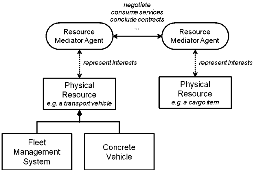
Fig. 12.4 Example Mediation Architecture in a Logistics Use Case (adapted from Maturana et al. 1999)
