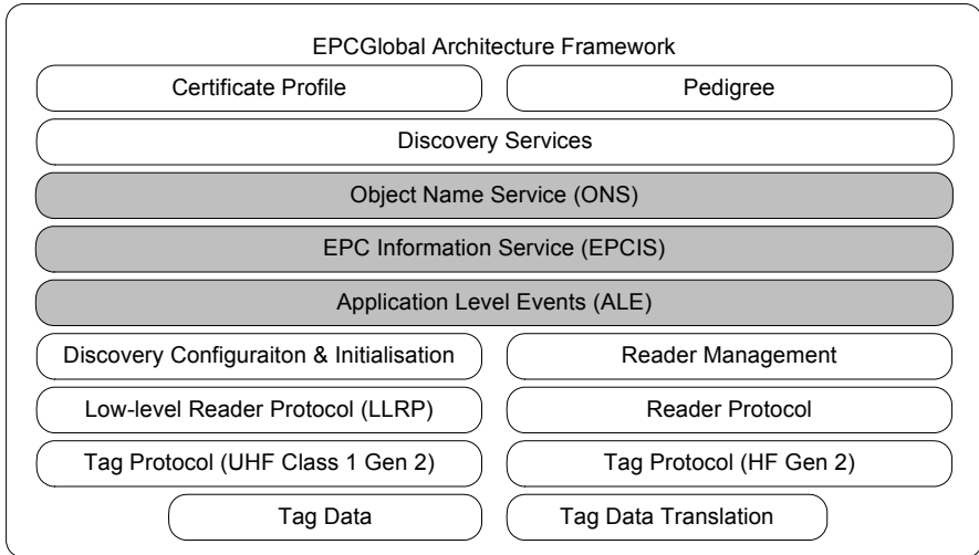
Fig. 6.2: The EPCglobal Architecture Framework (EPCglobal 2009)
