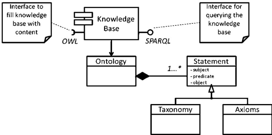
Fig. 12.8 The EURIDICE Knowledge Base Conceptual Model
