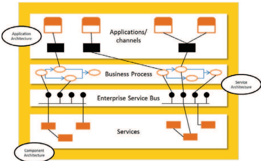
Fig. 12.10 Combination of EURIDICE Services to Business Processes (Schumacher et al. 2009)
