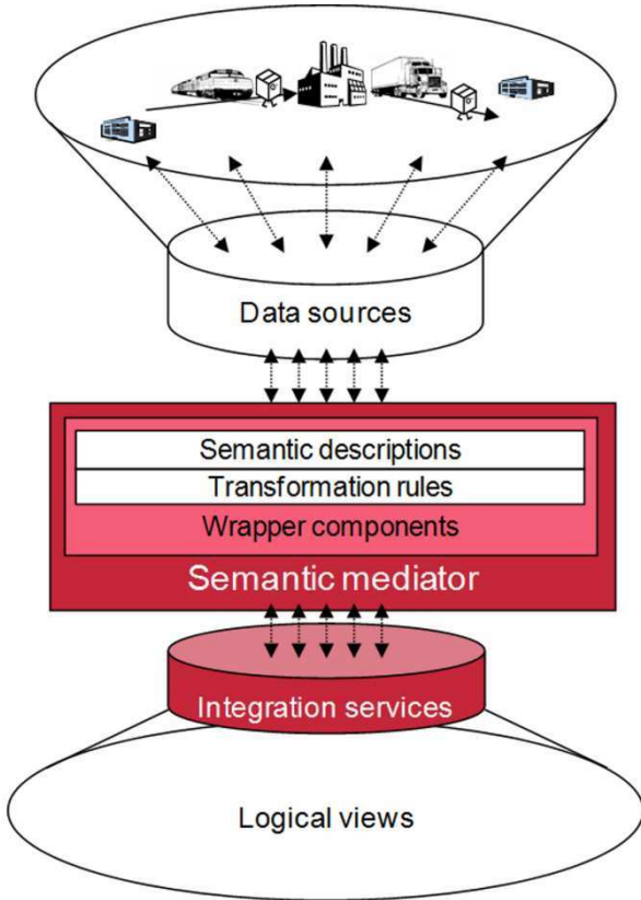
Fig. 6.3 Concept of a Service-oriented, Ontology-based Mediator
