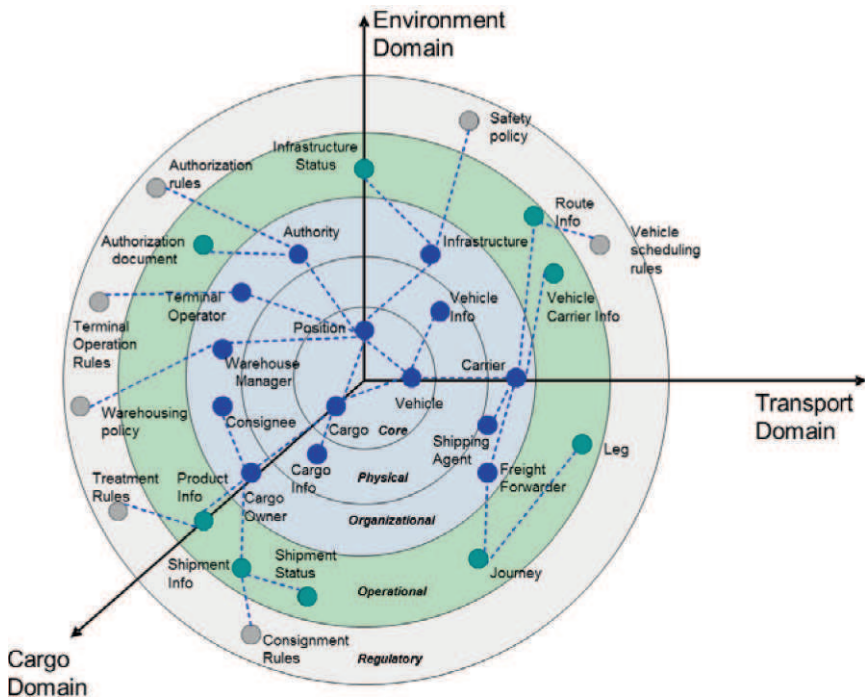
Fig. 12.7 The EURIDICE Context Model (Euridice 2009)
