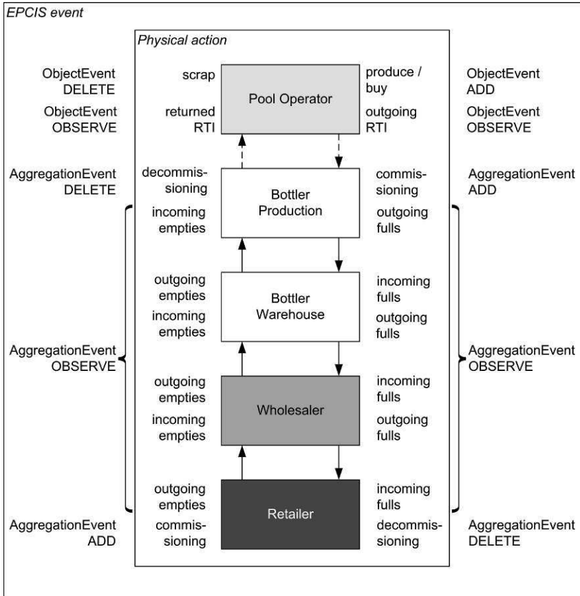
Fig. 9.3 A Simplified Supply Chain Scenario in the Beverage Industry
