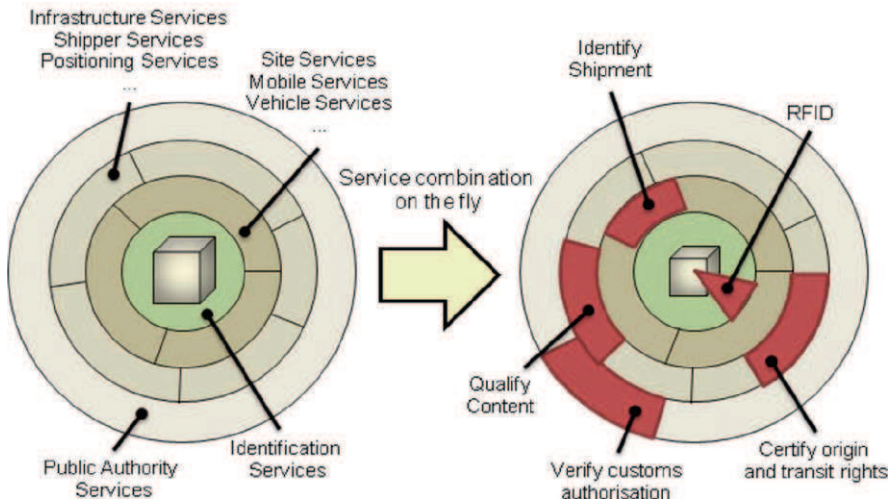
Fig.12.6 EURIDICE Cargo Centric Service Combination (Euridice 2009)
