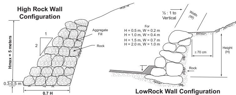
a. Common Types of Retaining Structures.
