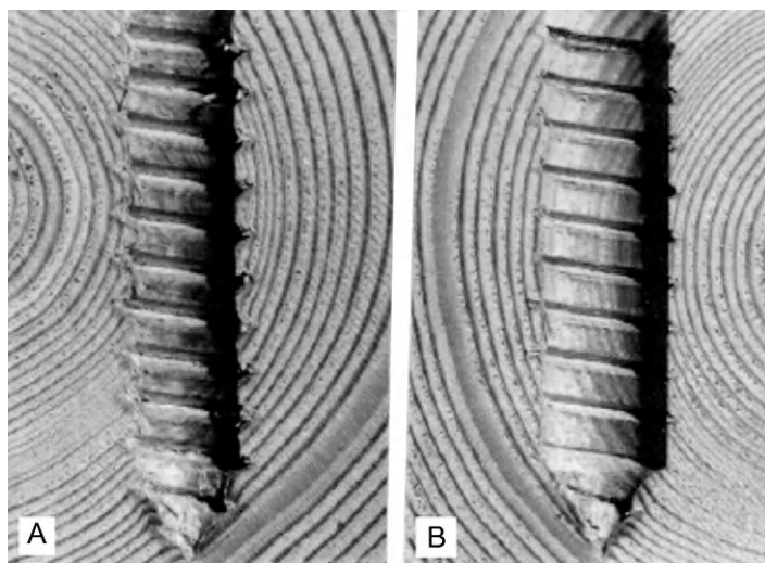
FIGURE 8-6 A, Clean-cut, deep penetration of thread made by lag screw turned into a lead hole of proper size, and B, rough, shallow penetration of thread made by lag screw turned into oversized lead hole.
