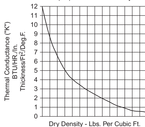
Relationship of Thermal Conductance ("K") To Concrete Density
