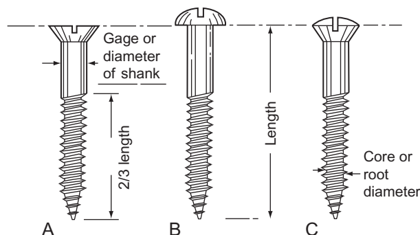
FIGURE 8–5 Common types of wood screws: A, flathead; B, roundhead; and C, ovalhead.
