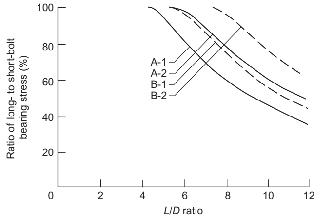
FIGURE 8-9 Variation in bolt-bearing stress at the proportional limit perpendicular to grain with L/D ratio. Relations obtained from experimental evaluation for materials with average compression perpendicular stress of 7,860 kPa (1,140 lb/in 2 ) (curve A-1) and 3,930 kPa (570 lb/in 2 ) (curve A-2). Curves B-1 and B-2, modified relations used for establishing design loads.
