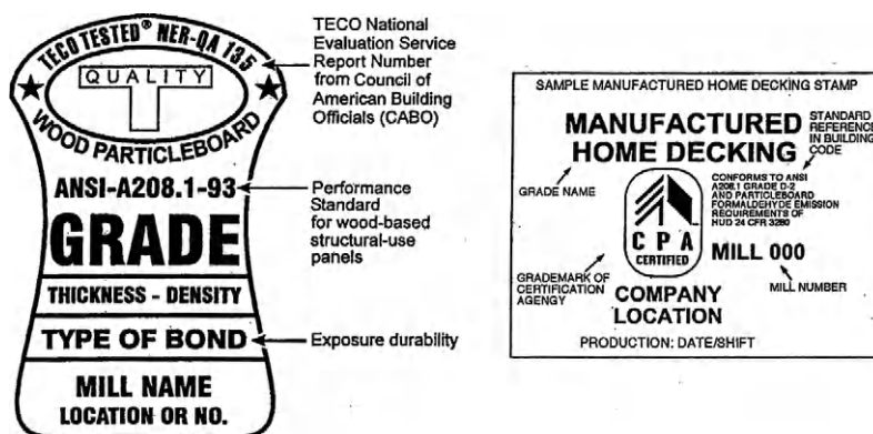
Examples of grade stamps for particleboard.
