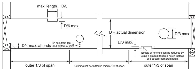
FIGURE 1 Placement of Cuts in Floor Joists
