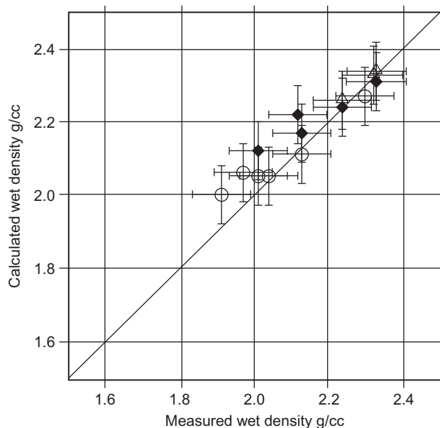
FIGURE 1 Measured wet densities compared with those calculated from dry densities using 2. Circles, wet density determined by saturation of dry sand, and triangles, of dry till, as described in 2.6. Diamonds, samples of glacial till collected wet and then oven-dried. Error-bars reflect what we believe to be measurement precision as described in 2.4.
