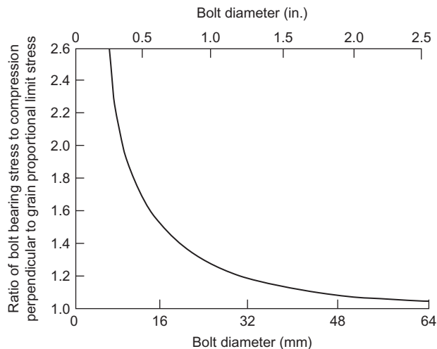
FIGURE 8-10 Bearing stress perpendicular to the grain as affected by bolt diameter.
