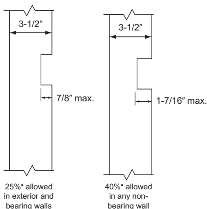
FIGURE 2 Notches in 2×4 Studs
