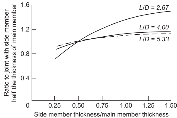
FIGURE 8-12 Proportional limit load related to side member thickness for three-member joints. Center member thickness was 50.8 mm (2 in.).
