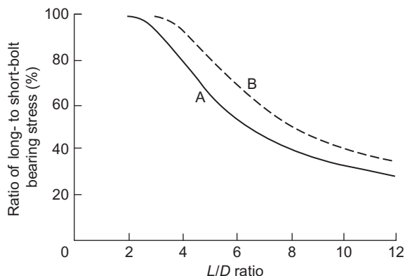
FIGURE 8-8 Variation in bolt-bearing stress at the proportional limit parallel to grain with L/D ratio. Curve A, relation obtained from experimental evaluation; curve B, modified relation used for establishing design loads.
