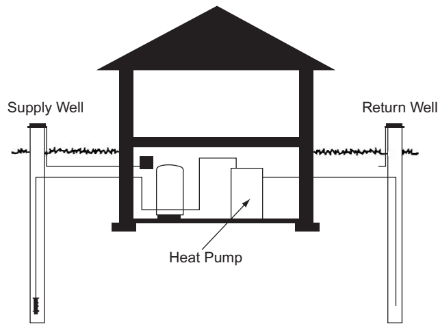
FIGURE 1 Groundwater heat pump.
