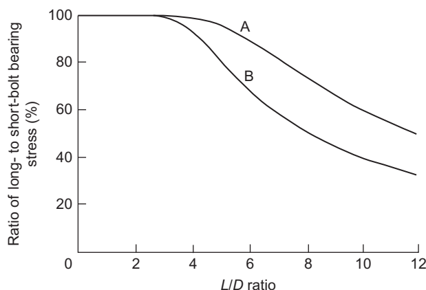
FIGURE 8–11 Variation in the proportional limit bolt-bearing stress parallel to grain with L/D ratio. Curve A, bolts with yield stress of 861.84 MPa (125,000 lb/in 2 ); curve B, bolts with yield stress of 310.26 MPa (45,000 lb/in 2 ).
