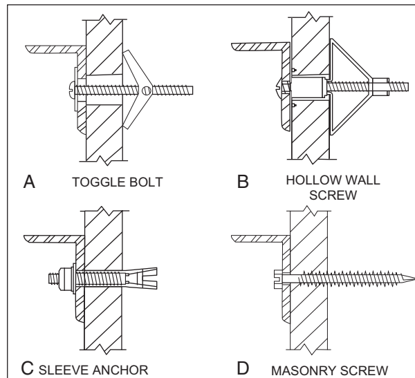
Fasteners Installed in Hollow Units
