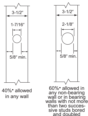
FIGURE 3 Bored Holes in 2×4 Studs
