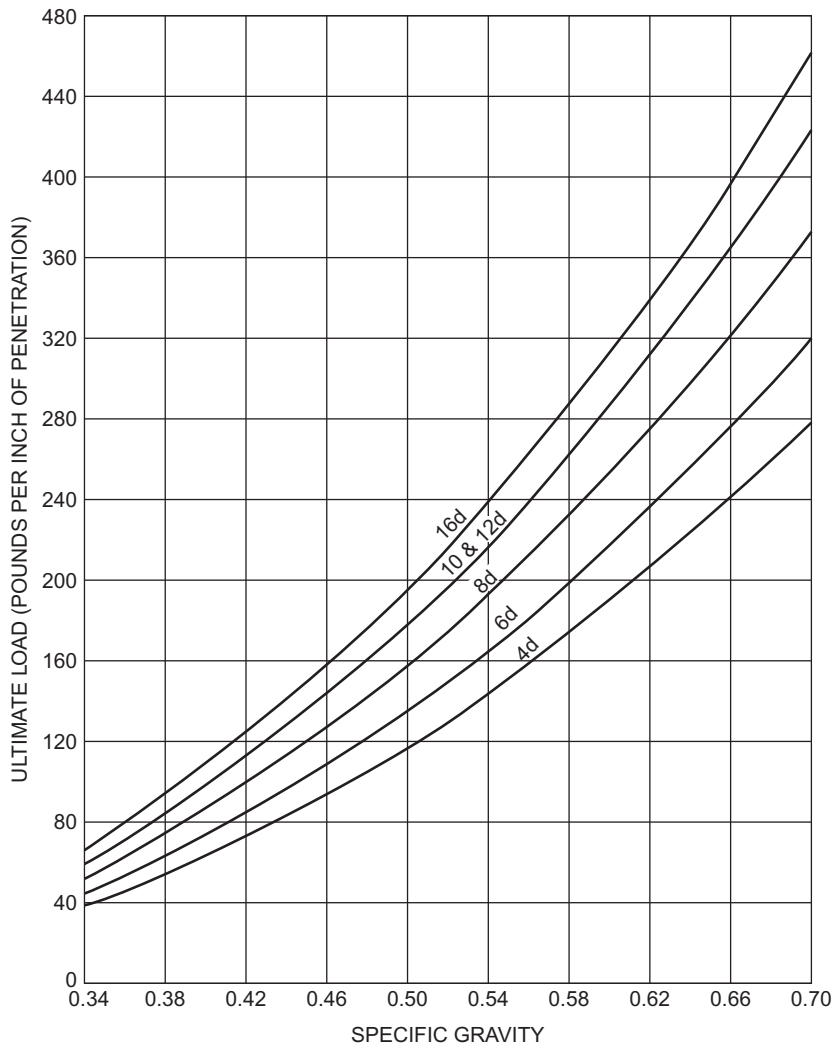
FIGURE 1 Load required to withdraw common nails from wood of different specific gravities immediately after nails were driven. Specific gravity is based on weight and volume of oven-dry wood.
