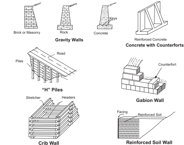
a. Common Types of Retaining Structures.
