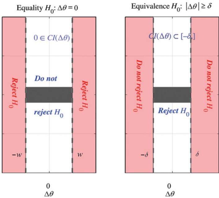
FIGURE 5.5 Confidence regions for statistical equality and equivalence.
