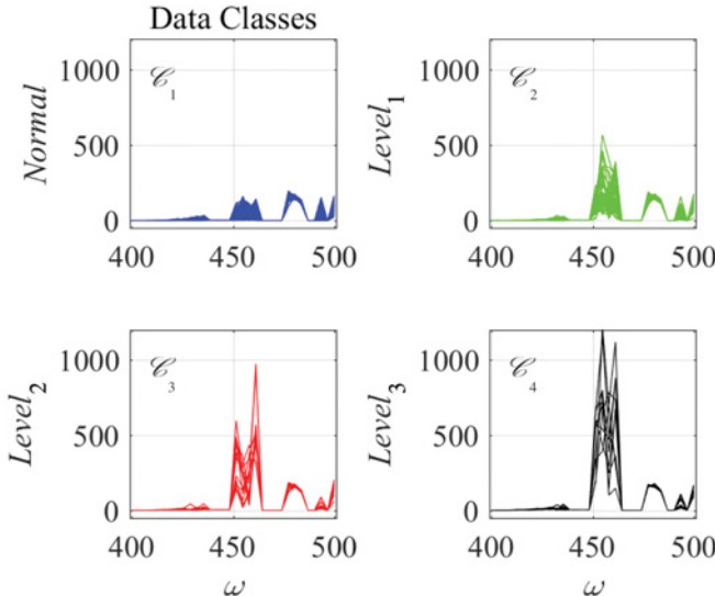
FIGURE 4.2 Multi-category, multivariate data.
