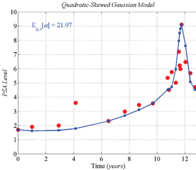
FIGURE 0.4 Data and quadratic-skewed Gaussian model.
