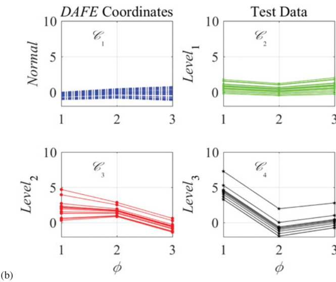
FIGURE 4.16 (a) DAFE coordinates (training). (b) DAFE coordinates (test).
