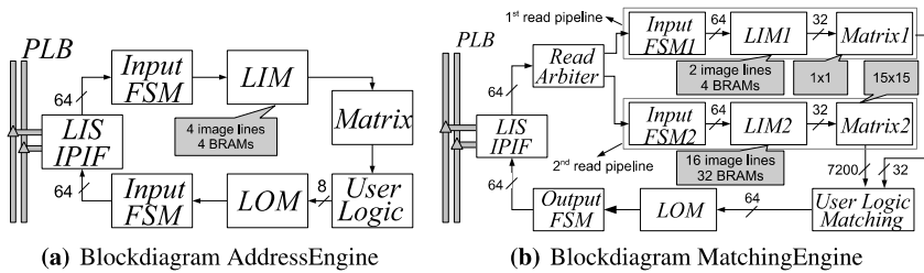
Fig. 18.3 Blockdiagrams of the AdressEngine in basic configuration and the MatchingEngine.
