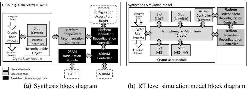
Fig. 7.7 Synthesis structure of Adaptive Crypto example.
