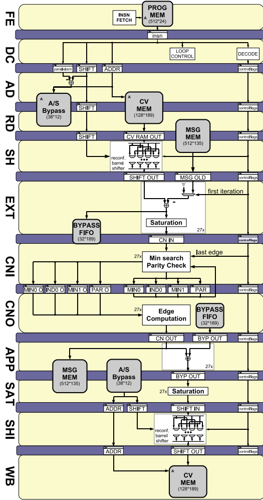
Fig. 14.7 Pipeline architecture as required for LDPC decoding. Pipeline stages are: fetch (FE), decode (DC), address (AD), read (RD), shift (SH), extrinsic computation (EXT), check node in (CNI), check node out (CNO), APP calculation (APP), saturation (SAT), shift inverse (SHI), write back (WB) [1].
