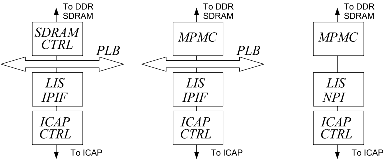
Fig. 18.7 Different interconnects used to connect ICAP and DDR SDRAM.
