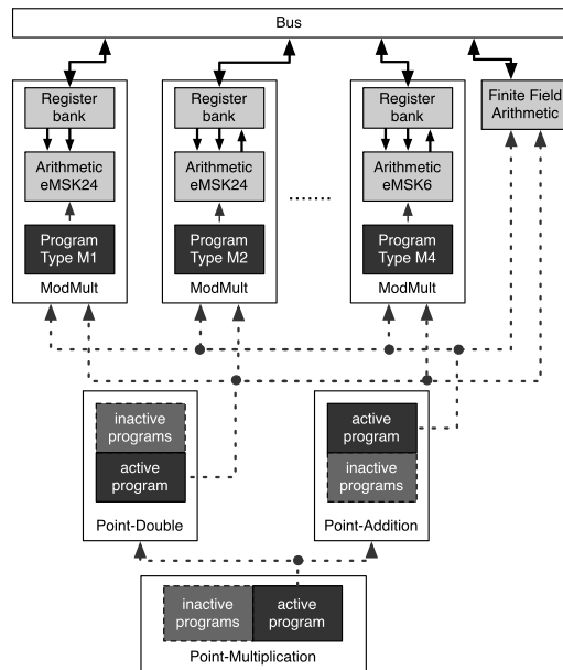
Fig. 19.5 Architecture of an arithmetic logic unit for ECC Point-Multiplication .
