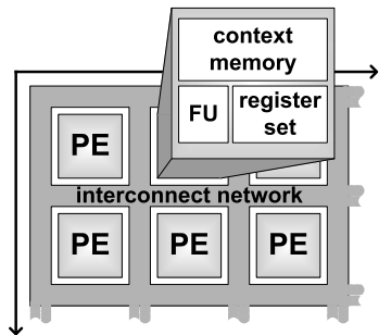
Fig. 5.2 General specification of the CRC model [21].
