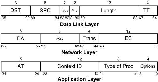
Fig. 16.4 CoNoChi protocol stack [20].
