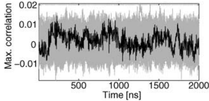
Fig. 19.8 HWPM on secured eMSK with 50,000 traces.
