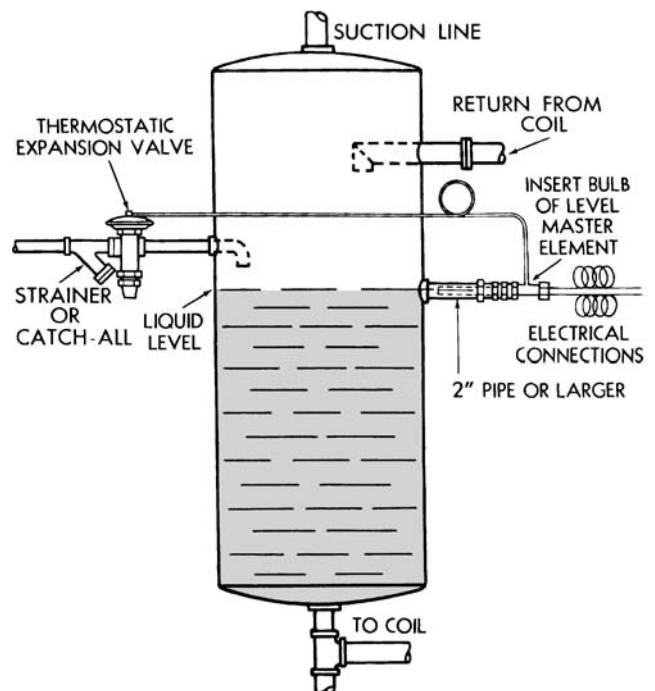
Fig. 11-46 Installation of the level-master control. (Sporlan Valve)
