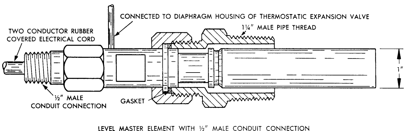
Fig. 11-45 Level-master control. (Sporlan Valve)
