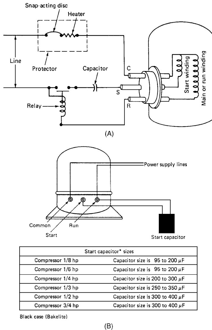
Fig. 5-24 (A) Capacitor-start, induction-run motor used for a compressor. (B) Location of the start capacitor in a compressor circuit.
