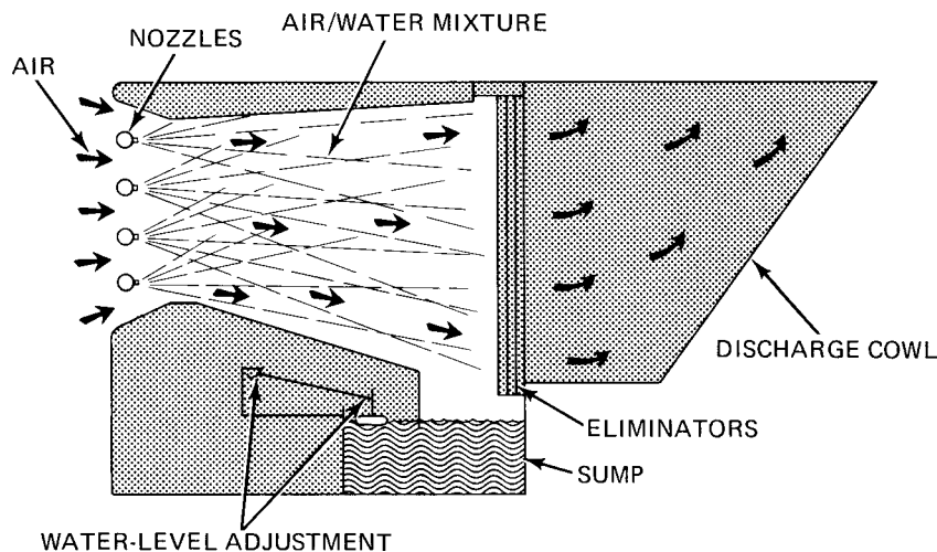
Fig. 8-19 Cooling tower with natural-draft properties. There are no moving parts in the cooling tower. (Marley)
