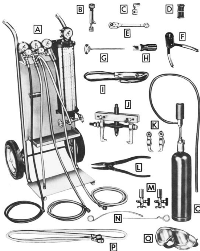
Fig. 1-18 Air-conditioning and refrigeration portable tool kit. (A) Air-conditioning charging station. (B) Excavating/charging valve. (C) 90 adapter service port. (D) O-ring installer. (E) Refrigeration ratchet. (F) Snap-ring pliers. (G) Stem thermometer. (H) Seal remover and installer. (I) Test light. (J) Puller. (K) Puller jaws. (L) Retainer ring pliers. (M) Refrigerant can tapper. (N) Dipsticks for checking oil level. (O) Halide leak detector. (P) Flexible charging hose. (Q) Goggles. (Snap-On Tools)
