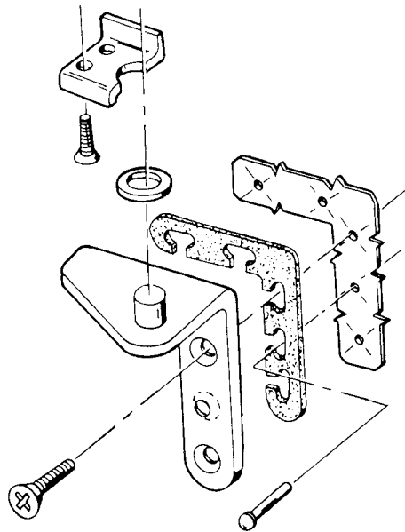
Fig. 13-11 Bottom hinge assemble. (Kelvinator)
