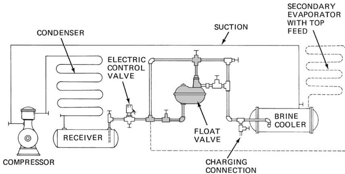
Fig. 11-44 High-pressure float-control system.
