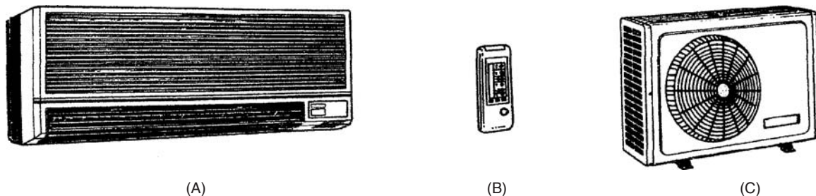
Fig. 15-29 Ductless wall-mounted air-conditioner system. (A) Wall-mounted unit in room to be cooled. (B) LCD wireless remote controller. (C) Outside unit consisting of compressor-condenser unit. (Mitsubishi)
