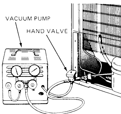
Fig. 12-8 Vacuum pump and hand valve. (Kelvinator)
