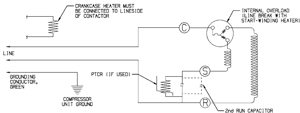
230 V-Schematic Wiring Diagram PSC - INTERNAL OVERLOAD (LINE BREAK) - START-WINDING HEATER - CRANKSPACE HEATER
