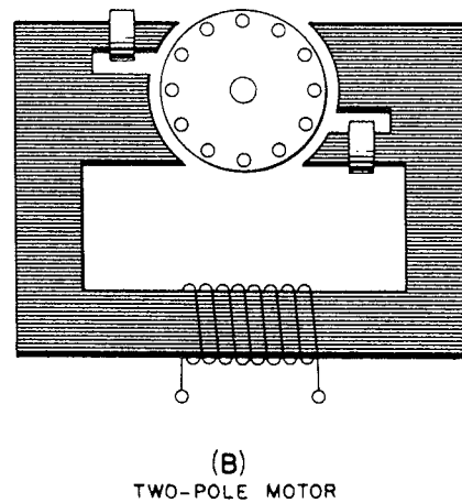
Fig. 5-2 Shaded-pole motor.
