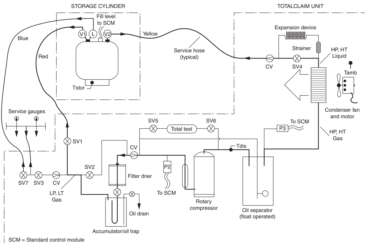
Fig. 6-16 Recycle—functional flow. (Carrier)
