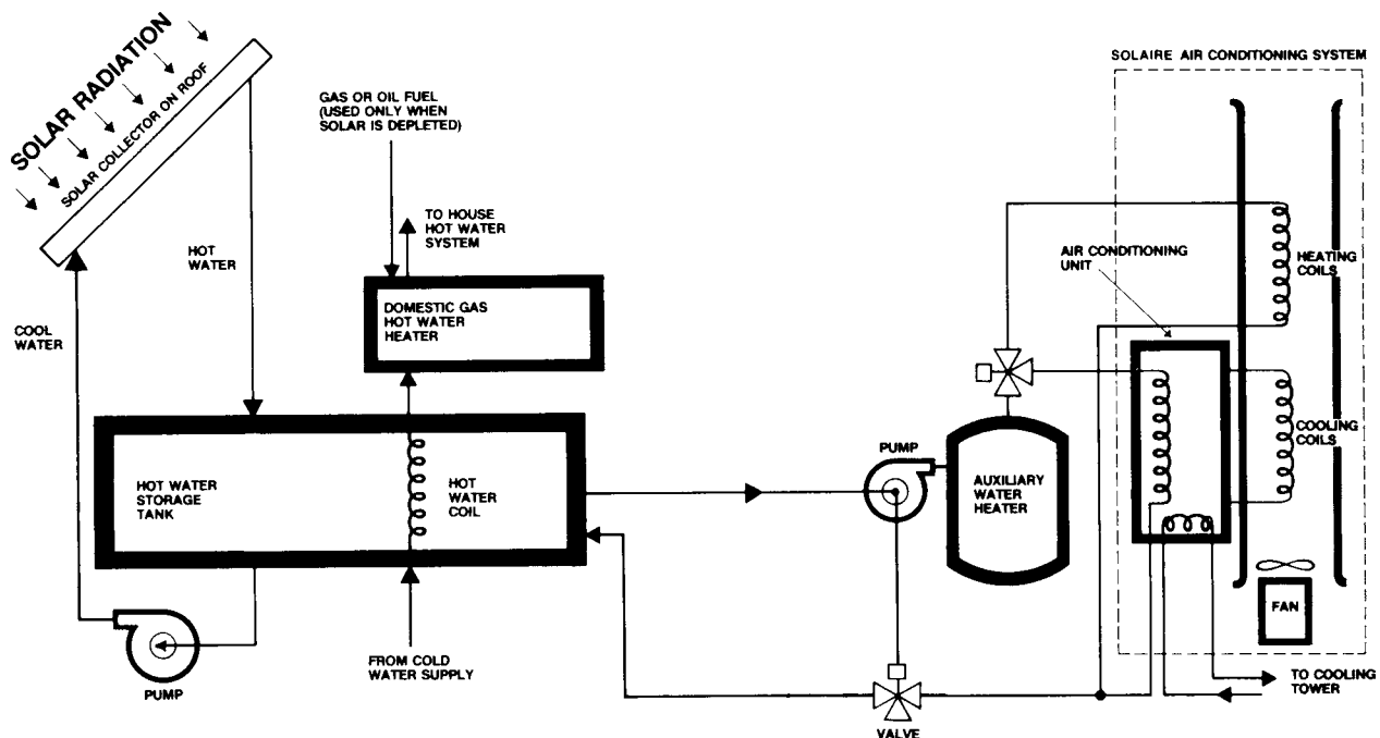
Fig. 17-9 Solar-energy air-conditioning unit—direct system. (Arkla)
