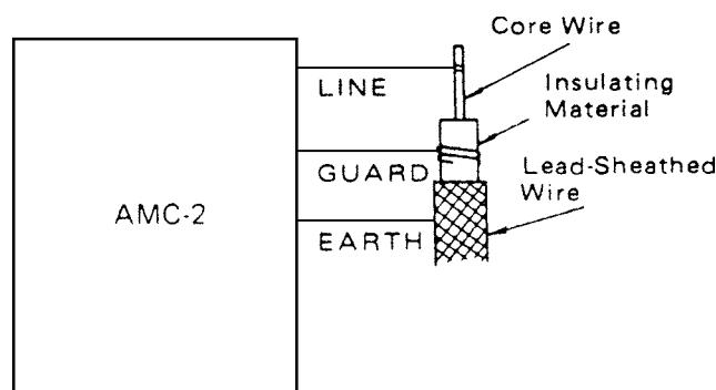
Fig. 5-69 Hand-cranked model used to test insulation of a cable.
