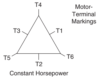
Fig. 5-50 Connections made by the starter for constant horsepower. (Allen-Bradley)
