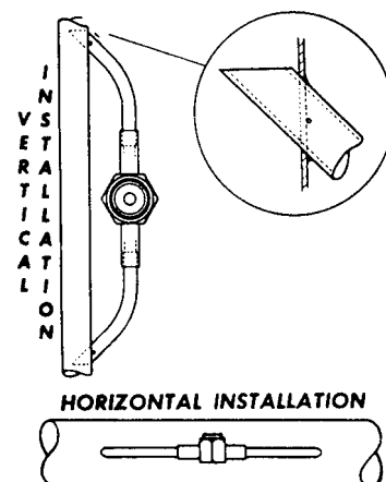
Fig. 11-17 Liquid-line indicator installation. (Sporlan Valve)
