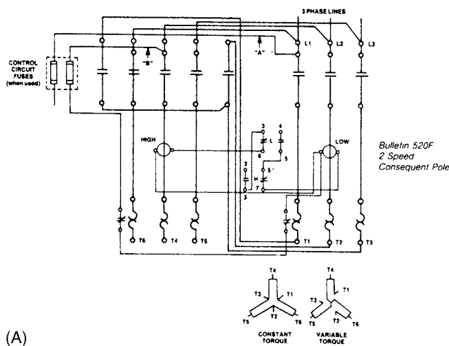
Fig. 5-54 (A) Typical wiring diagram for two-speed consequent-pole starter (Wye). (B) Typical wiring diagram for two-speed consequent-pole starter (Delta).
