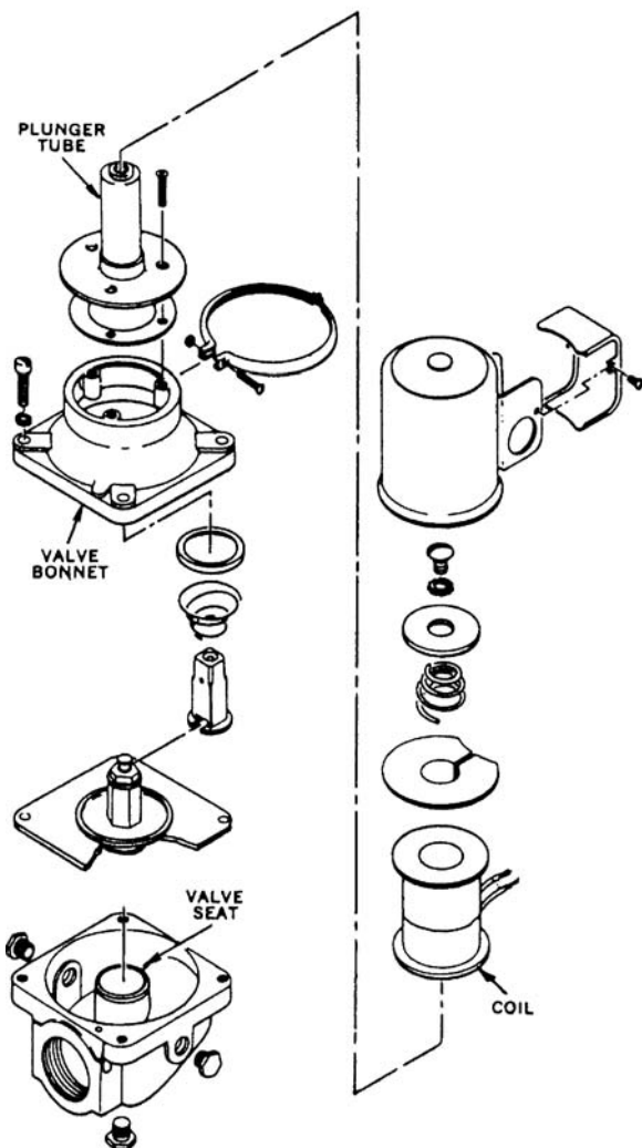
Fig. 4-7 Exploded view of balanced diaphragm valve
