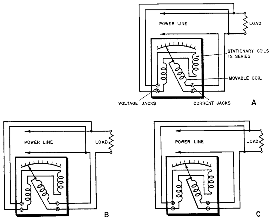
Fig. 1-48 (A) Wattmeter connection for measuring input power. (B) Alternate wattmeter connection. (C) With load disconnected, uncompensated wattmeter measures its own power loss.
