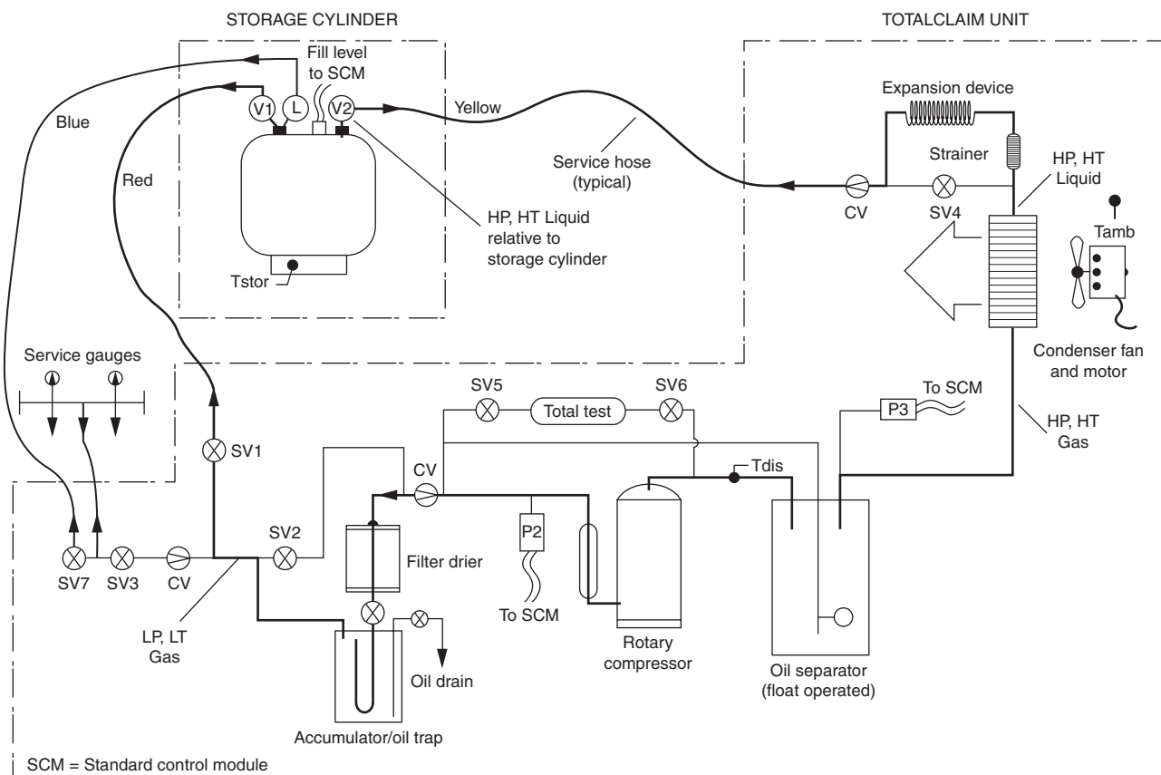
Fig. 6-15 Storage cylinder cooling—functional flow. (Carrier)
