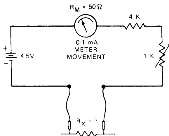
Fig. 1-45 Internal circuit of an ohmmeter.
