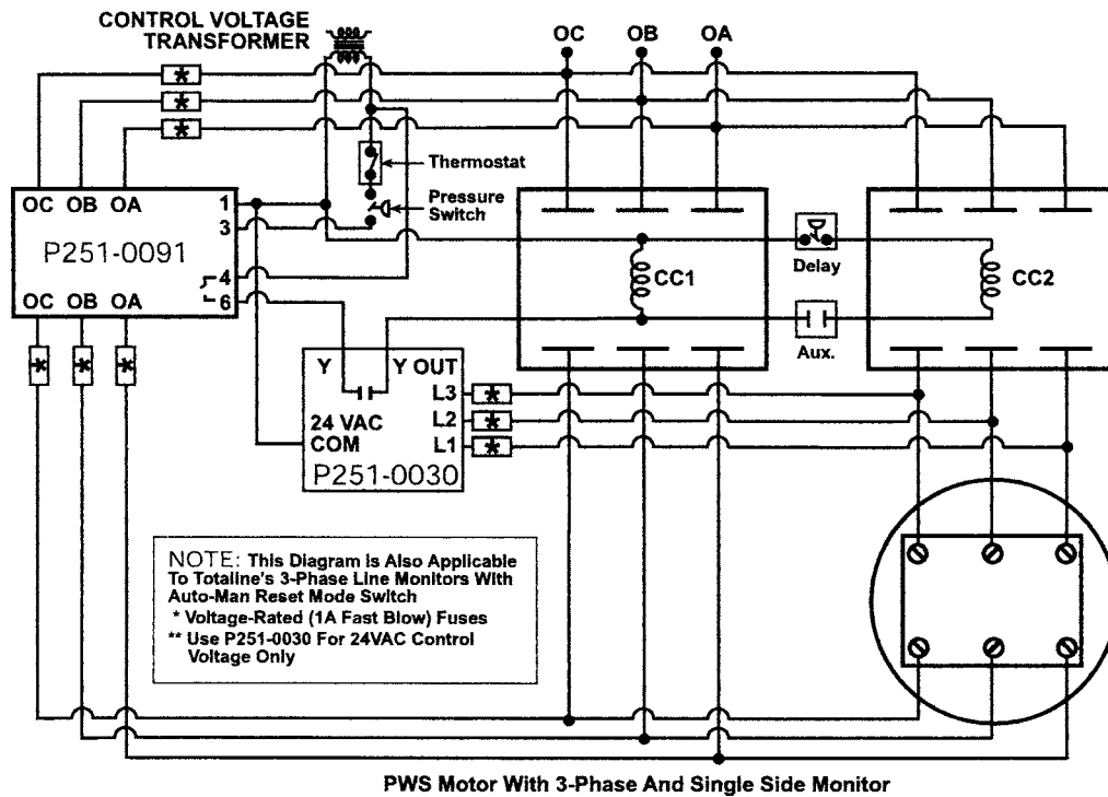
Fig. 19-21 Typical part winding start wiring diagram. (Carrier)
