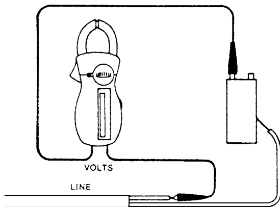
Fig. 5-66 Test for finding a grounded capacitor. (Amprobe)
