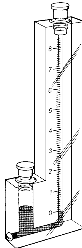
Fig. 14-4 Well-type manometer. (Johnson)
