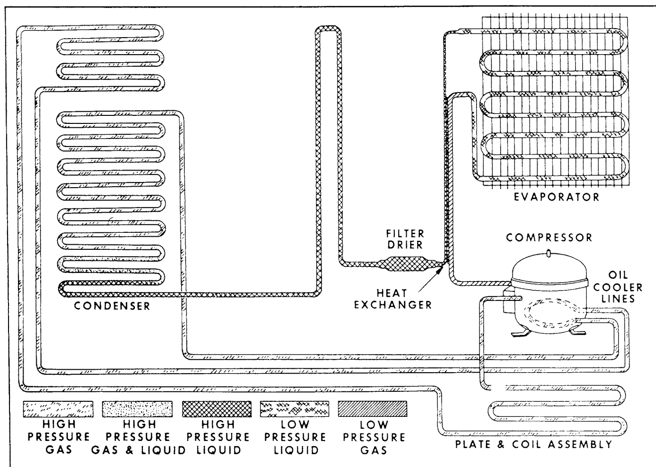
Fig. 12-3 Refrigerating system with various pressures located. (Kelvinator)
