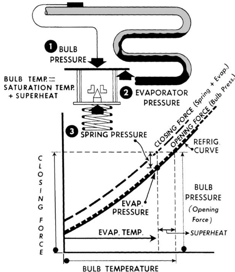
Fig. 11-20 Basic thermostatic-expansion valve operation. (Virginia Chemicals)
