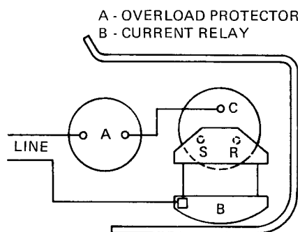
Fig. 7-69 Location of the terminals for the compressors and electrical connections on the Americold compressors. (Americold)
