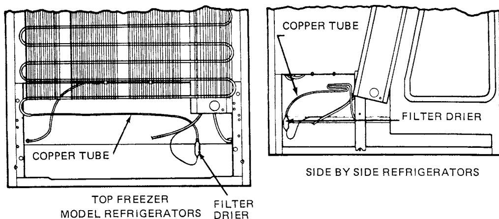
Fig. 12-19 Side-by side and top-freezer model refrigerator filter-drier location. (Kelvinator)
