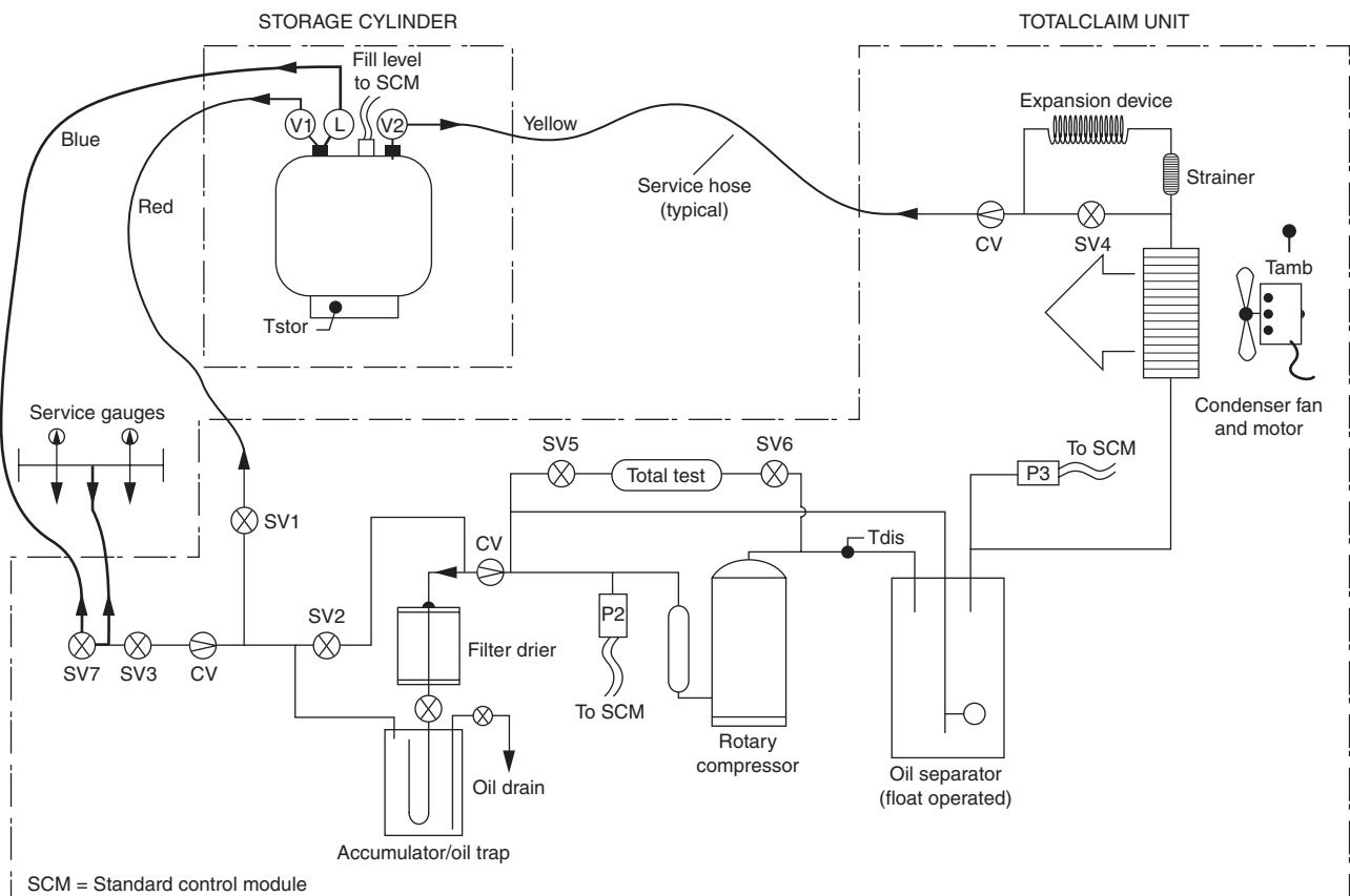
Fig. 6-17 Recharge (liquid)—functional flow. (Carrier)
