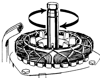
Fig. 7-26 An antislug feature is standard on all AJ1M12 models and on larger models of the AJ series. (Tecumseh)
