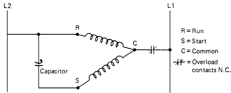
(A) Ladder diagram or schematic
