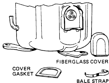
Fig. 7-20 Snap-on terminal cover assembly. (Tecumseh)
