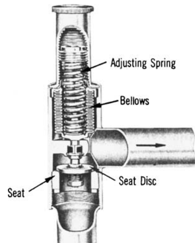
Fig. 11-32 Head-pressure control valve. (Sporlan Valve)
