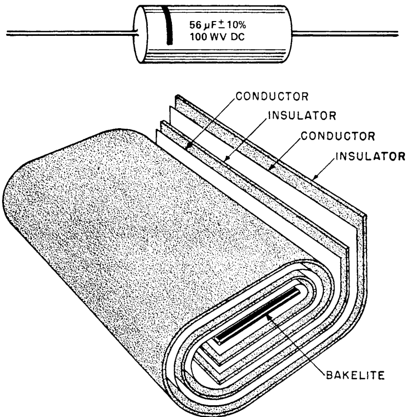
Fig. 3-15 A paper capacitor, encased, and with the top cover removed.
