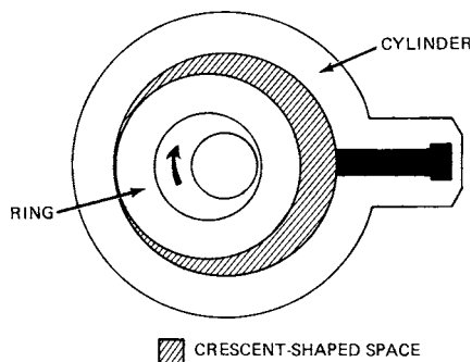
Fig. 7-72 Operation of a rotary compressor. (General Motors)
