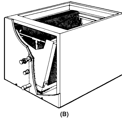
Fig. 10-1 Evaporators. (A) Evaporator used in home air-conditioning systems where the unit is placed in the bonnet of the hot-air furnace. (B) Slanted evaporator used in home air conditioning. (Lennex)
