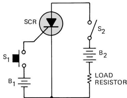
Fig. 3-31 A silicon controlled rectifier (SCR) circuit.
