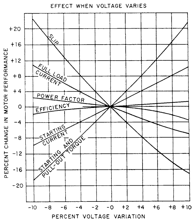
Fig. 19-3 General effects of voltage variations on induction motor characteristics.
