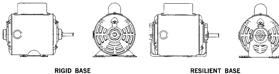
Fig. 5-23 Capacitor-start motor.
