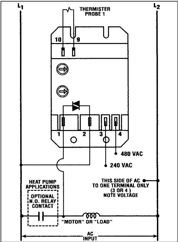
Fig. 19-16 Connection diagrams for Fig. 21-14. (Carrier)
