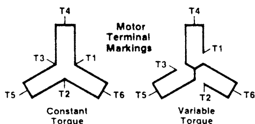
Fig. 5-46 Connections made by the consequent-pole starter for constant torque or variable torque. (Allen-Bradley)
