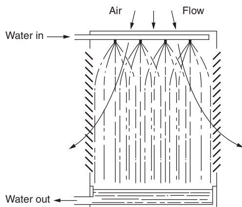
Fig. 8-20 Atmospheric tower.
