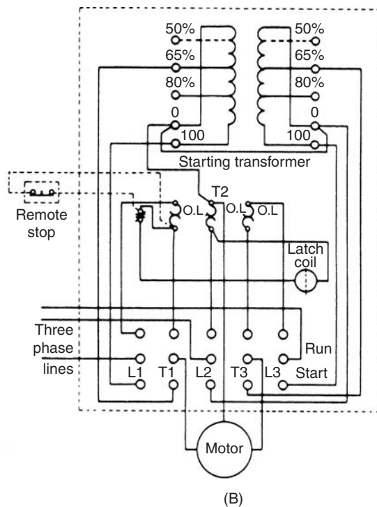
Fig. 5-38 (A) Autotransformer type of magnetic starter. (B) Corresponding wiring diagram. (Allen-Bradley)
