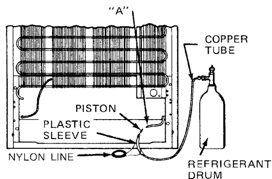
Fig. 12-20 An older technique using vapor pressure from refrigerant drum to blow the piston and nylon assembly through the hot tube. (Kelvinator)
