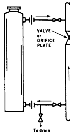
BY-PASS ARRANGEMENT Nonrecirculating, once through systems
