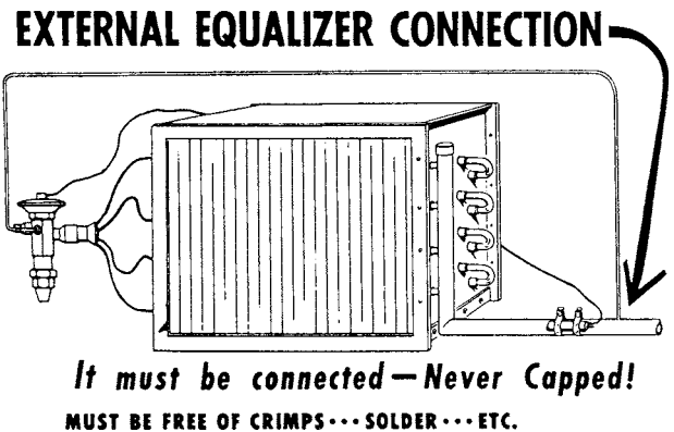
Fig. 11-24 External equalizer connection. (Virginia Chemicals)
