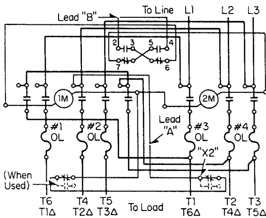
Fig. 5-33 (A) Nonreversing single-phase and nonreversing three-phase wiring diagrams. (B) Reversing three-phase wiring diagram. (C) Two-speed, one winding, three-phase delta. (D) Two-speed, two-winding, three-phase starter diagram. (Westinghouse)
