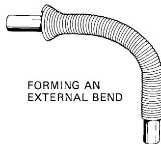
Fig. 1-71 Using a spring-type tool to bend tubing.
