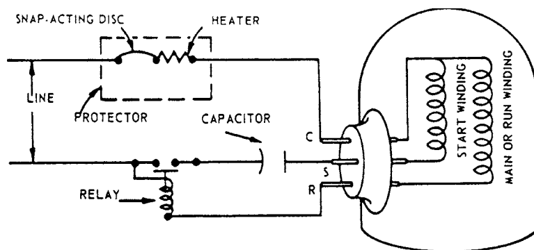
Fig. 7-16 (A) Capacitor-start induction-run motor for a compressor. (B) PTC/capacitor run (PTCS/CR). (C) PTC relay. (Tecumseh)
