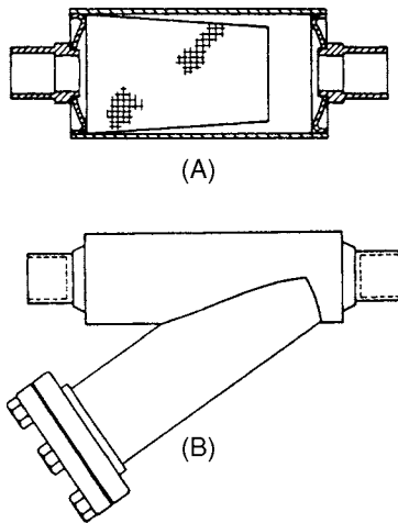
Fig. 11-14 Strainers. (A) Non-cleanable strainer. (B) Y-type line strainer. (Sporlan Valve)
