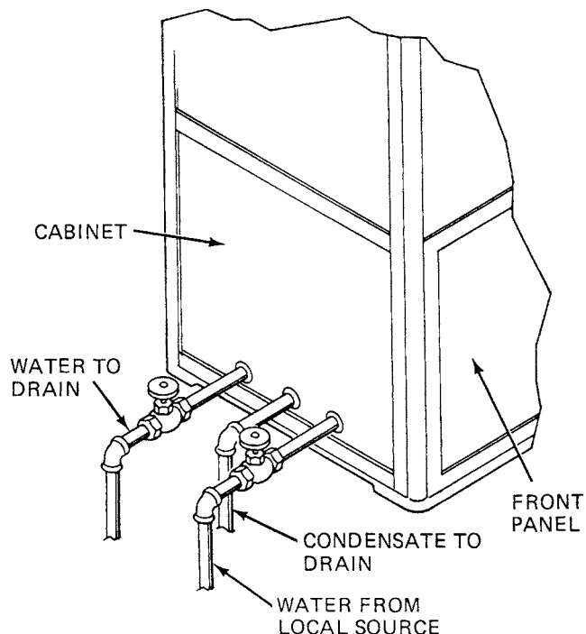
Fig. 16-20 Plumbing connections for a water-cooled, self-contained console air conditioner.
