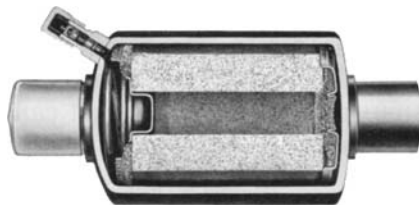
Fig. 11-13 Suction-line filter drier. (Mueller Brass)
