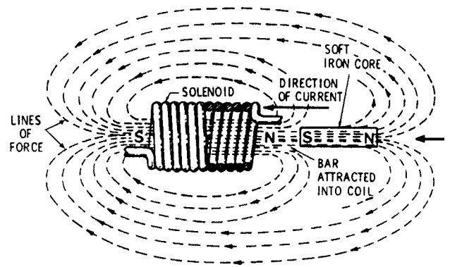
Fig. 4-1 Solenoid pulls core into the coil. Sucking effect of a coil.
