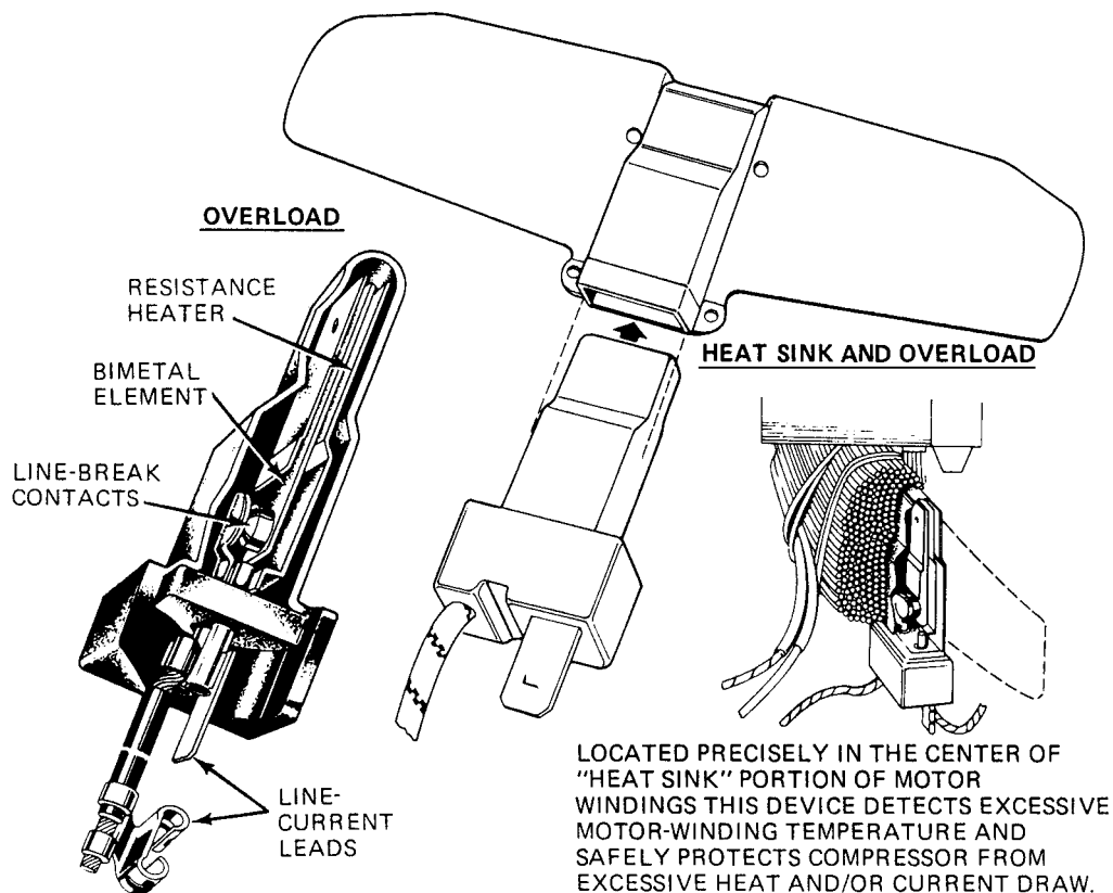
Fig. 7-19 Internal line-break motor protector. (Tecumseh)
