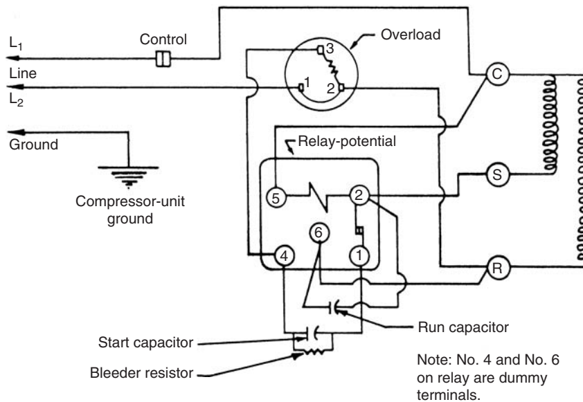
Fig. 7-57 High-starting torque motors (CSR) with a three-terminal external overload and potential relay mounted remote. (Tecumseh)
