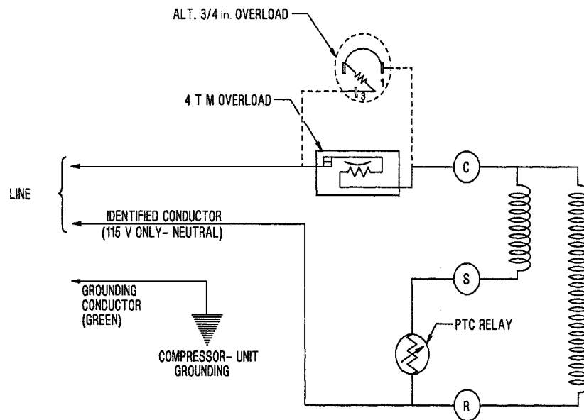
115 OR 230 V SCHEMATIC WIRING DIAGRAM- PTCS-IR
