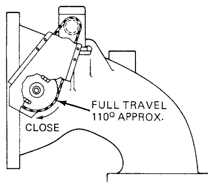
Fig. 8-13 Vane motor-crank angles. These are shown as No. 16 and No. 17 in Fig. 8-11.
