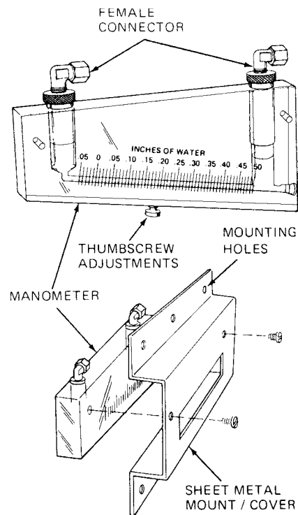
Fig. 14-5 Incline manometer. (Dwyer)
