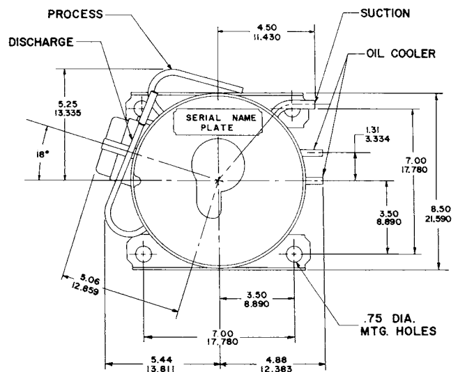
Fig. 7-70 Location of process, discharge, suction, and oil-cooler stubs on Americold compressors. (Americold)
