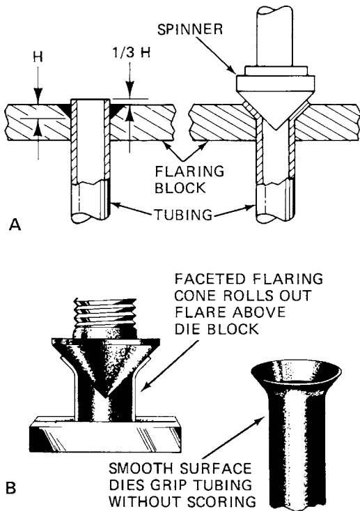
Fig. 1-64 Flaring tools. (A) This type of tool calls for the tubing to be inserted into the proper size hole with a small amount of the tube sticking above the flaring block. (B) This type of tool calls for the tubing to stick well above the flaring block. This type is able to maintain the original wall thickness at the base of the flare. The faceted flaring cone smooths out any surface imperfections.
