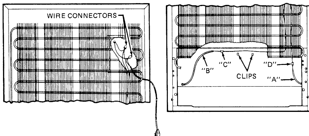
Fig. 12-18 Top-freezer refrigerator-cord splice location. (Kelvinator)
