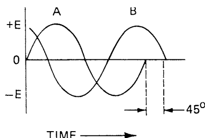
Fig. 3-8 Two AC waveforms, out-of-phase by 45°.
