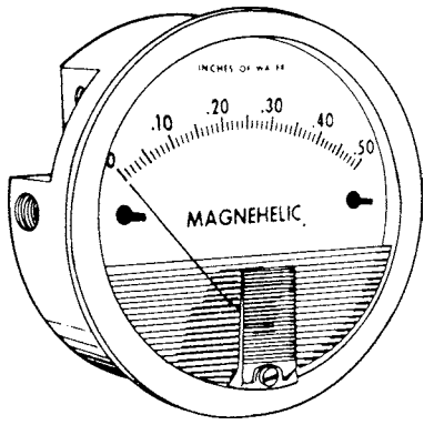
Fig. 14-6 Magnahelic manometer.
