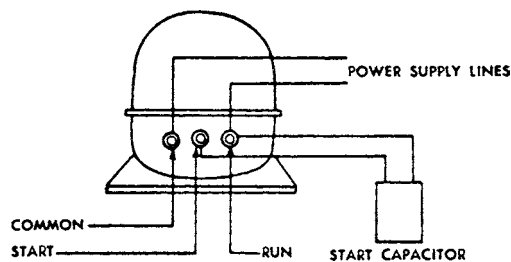
Fig. 12-31 Location of start capacitor in a circuit. (Tecumseh)
