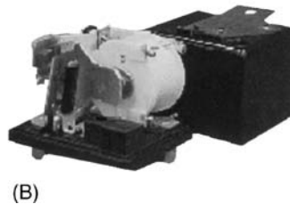
Fig. 7-41 (A) Potential-type relay. Usually found on large commercial and air-conditioning compressors to 5 hp. (B) Potential relay. (Tecumseh)
