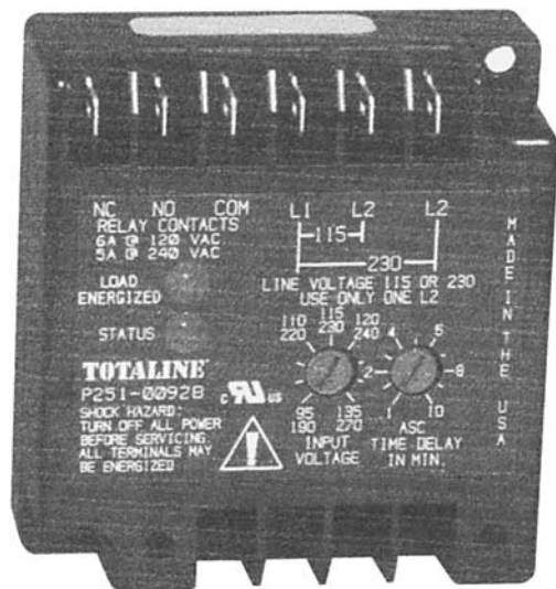
Fig. 19-9 Single-phase line monitor. (Carrier)
