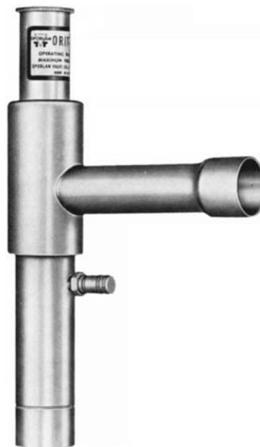
Fig. 11-29 Evaporator pressure-regulating valve. (Sporlan Valve)
