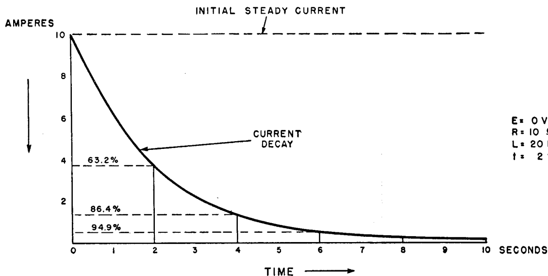
Fig. 3-21 The time lag produced by a coil. (A) The way in which a time lag is introduced in a circuit by an inductor. (B) It takes time for the magnetic field to collapse.
