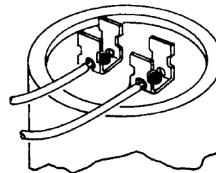
Fig. 12-25 There are three ways to attach terminals to an electrolytic capacitor. (Tecumseh)
