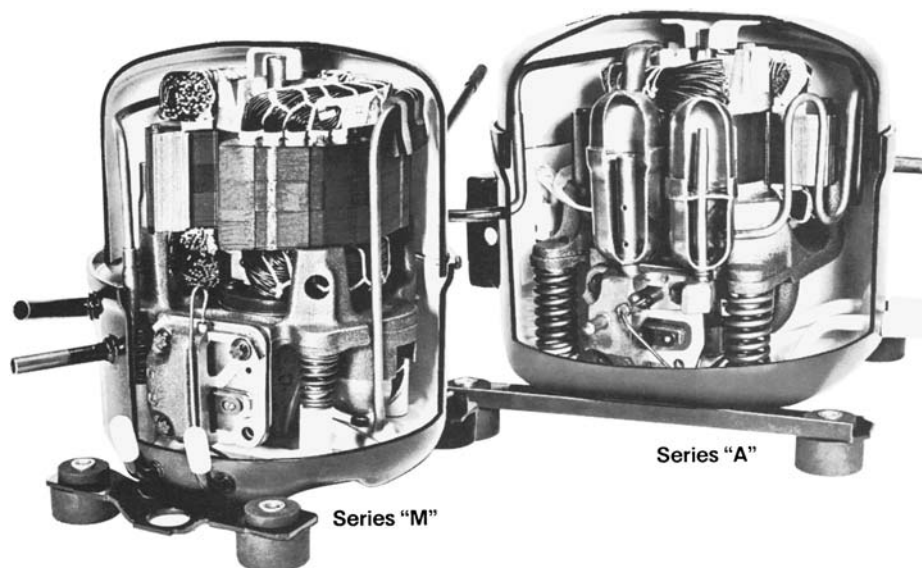
Fig. 7-68 Series M and series A compressors made by Americold.
