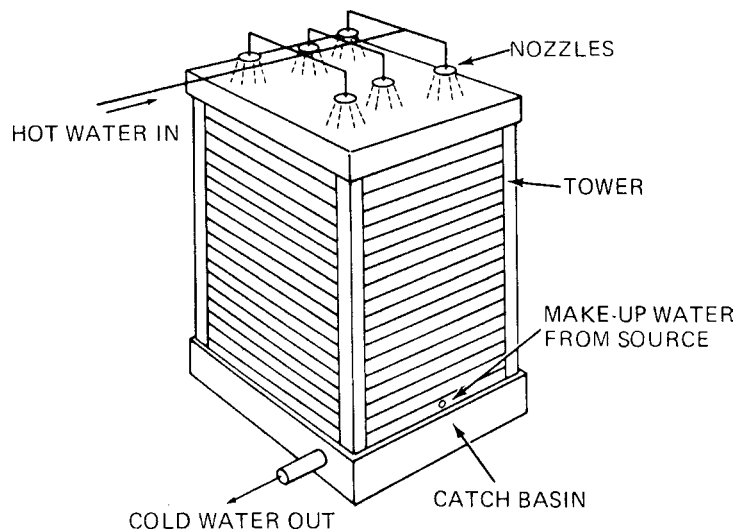
Fig. 8-15 Natural-draft cooling tower.
