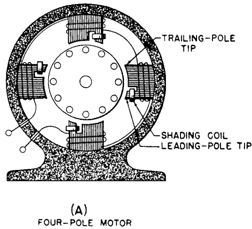
Fig. 5-2 Shaded-pole motor.
