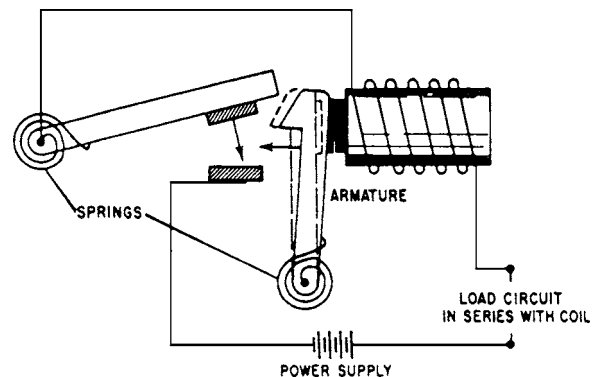
Fig. 4-5 Magnetic-circuit breaker.
