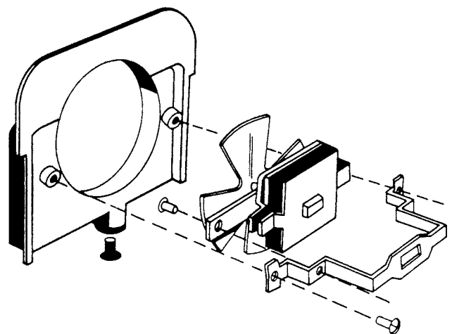
Fig. 5-29 Fan and fan-motor bracket assembly.
