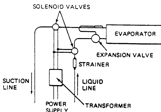
Fig. 4-10 Solenoid valves connected in the suction and liquid evaporator lines of a refrigeration system.
