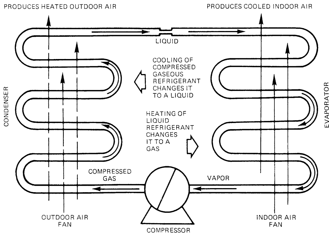
Fig. 8-1 Refrigeration cycle.
