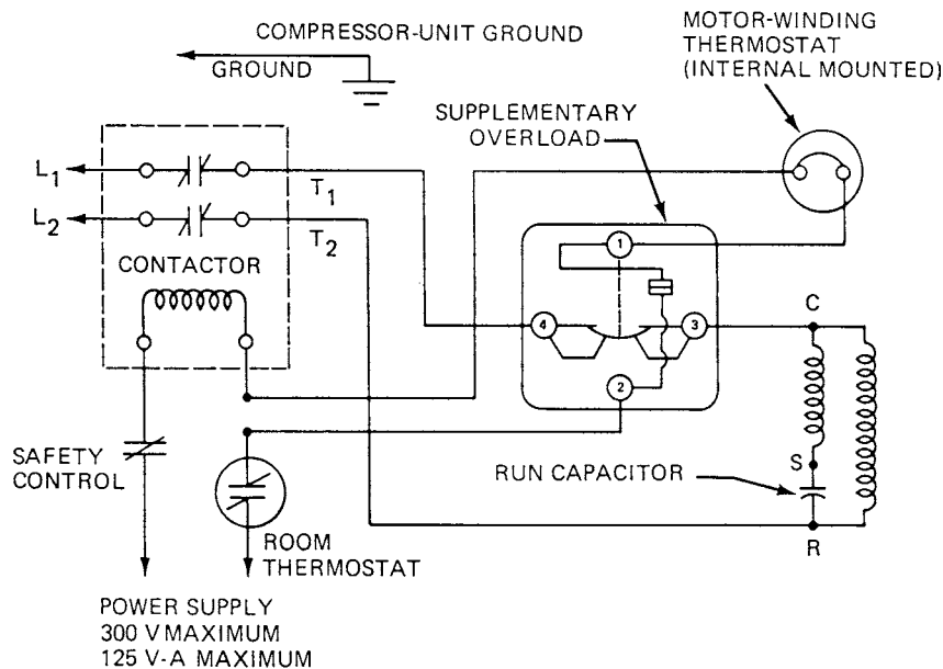
Fig. 7-62 PSC motors with internal thermostat and supplementary external overload. (Tecomseh)
