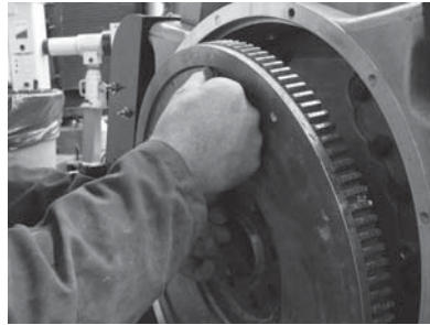
P3-2 When the flywheel fasteners have been removed, remove the flywheel from the flywheel housing. Place on hardwood blocks taking care not to damage the ring gear teeth.
