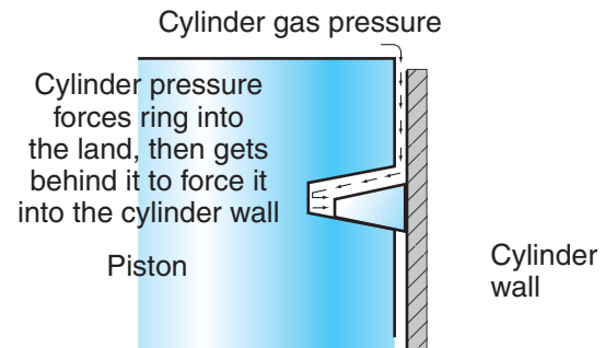
Compression Ring Action
