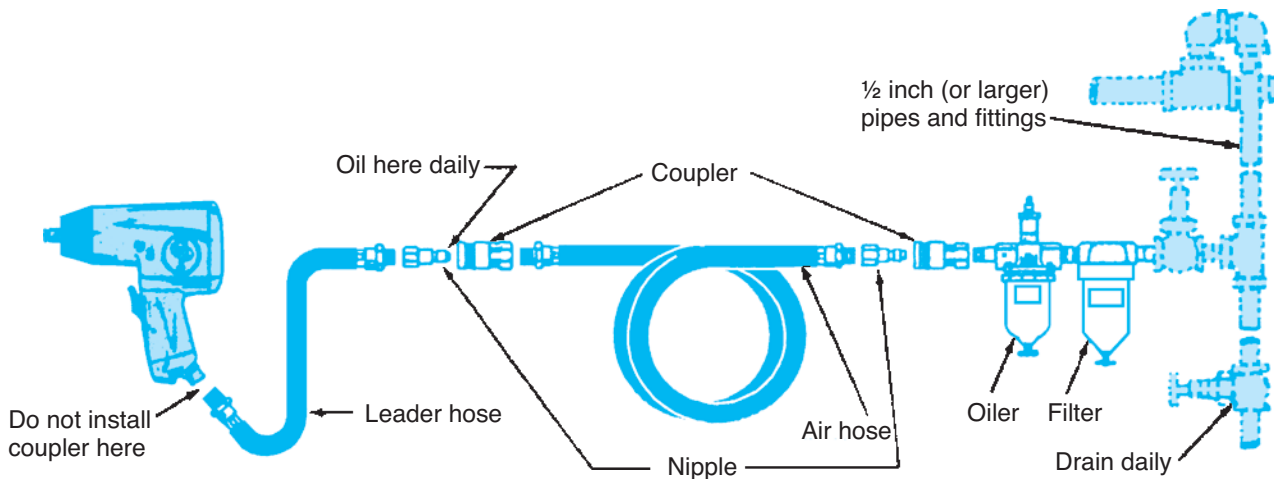
Figure 1-9 Typical setup for a 1/2-inch drive impact gun.
