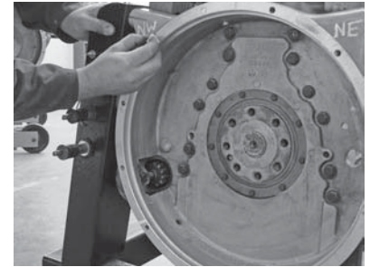
P3-3 Next, use chalk to mark four reference points on the flange face of the flywheel housing approximately 90 degrees apart. Use an emery cloth to clean up the inside bore of the flywheel housing removing any dirt or scratches: this must be clean to ensure accurate measurements.
