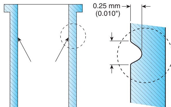
Figure 6-6 Cylinder wear ridge. (Courtesy of Caterpillar)
