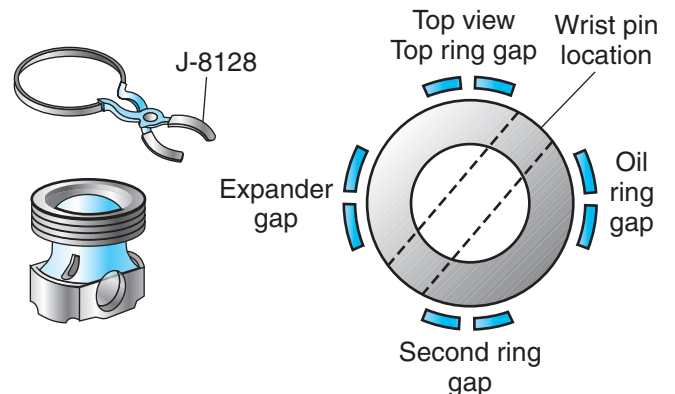
Figure 11-9 DDC Mono-therm piston ring stagger. (Specifications are subject to change without notice. Detroit Diesel Corporation is registered to ISO 9001:2001. Courtesy ©Detroit Diesel Corporation. All rights reserved. Detroit Diesel is a Daimler company)
