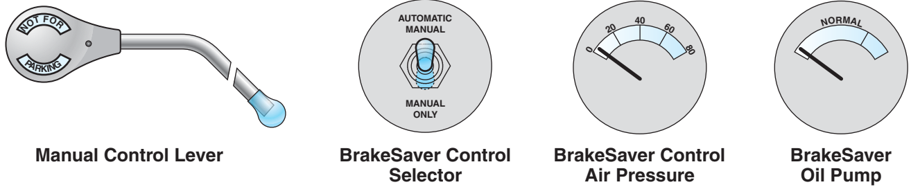
Figure 10-8 Caterpillar BrakeSaver controls. (Courtesy of Caterpillar)
