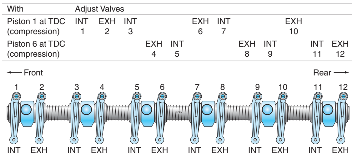
Figure 5-17 Valve lash adjustment positions on a Navistar International DT-466E. (Courtesy of Navistar International)
