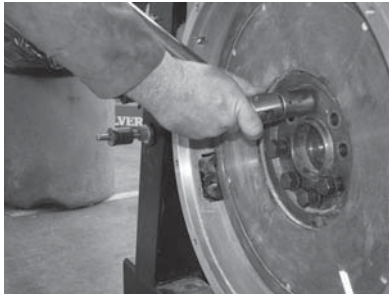
P3-1 Hold the engine in a fixed position (so it cannot rotate) and remove the flywheel bolts.
