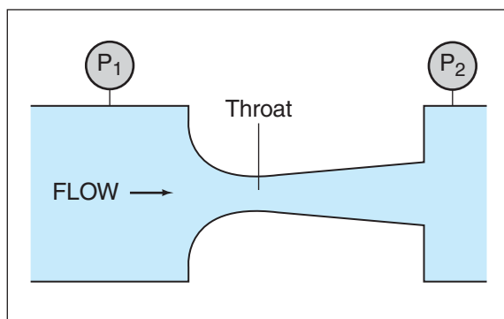
Figure 14-6 Critical flow venturi, pressure differential MAF sensor.
