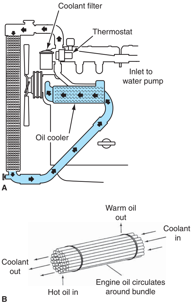
Figure 7-10 Oil flow through a bundle-type cooler.
