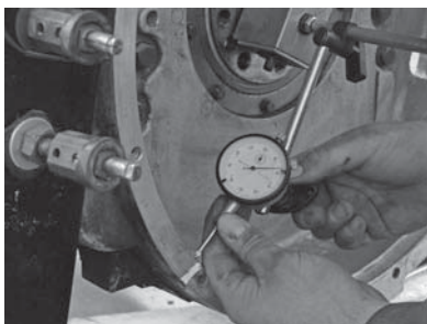
P3-7 Record the indicator reading at the SW location. Make sure you note whether this reading occurs on the plus or minus side of the indicator zero point. Bar the engine to the next reference point.
