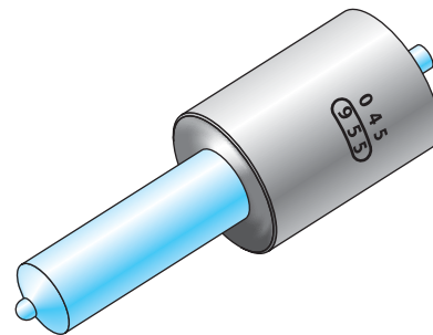
Figure 13-1 External view of a multi-orifice injector nozzle. (Courtesy of Robert Bosch GmbH, www.bosch-presse.de )
