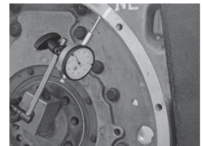
P3-9 Record the indicator reading at the NE location. Make sure you note whether this reading occurs on the plus or minus side of the indicator zero point. Now bar the engine back to the starting reference point at NW.
