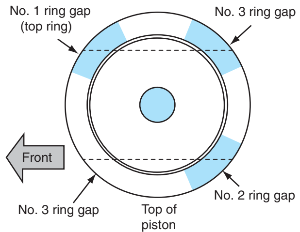
Figure 4-9 Ring stagger.
