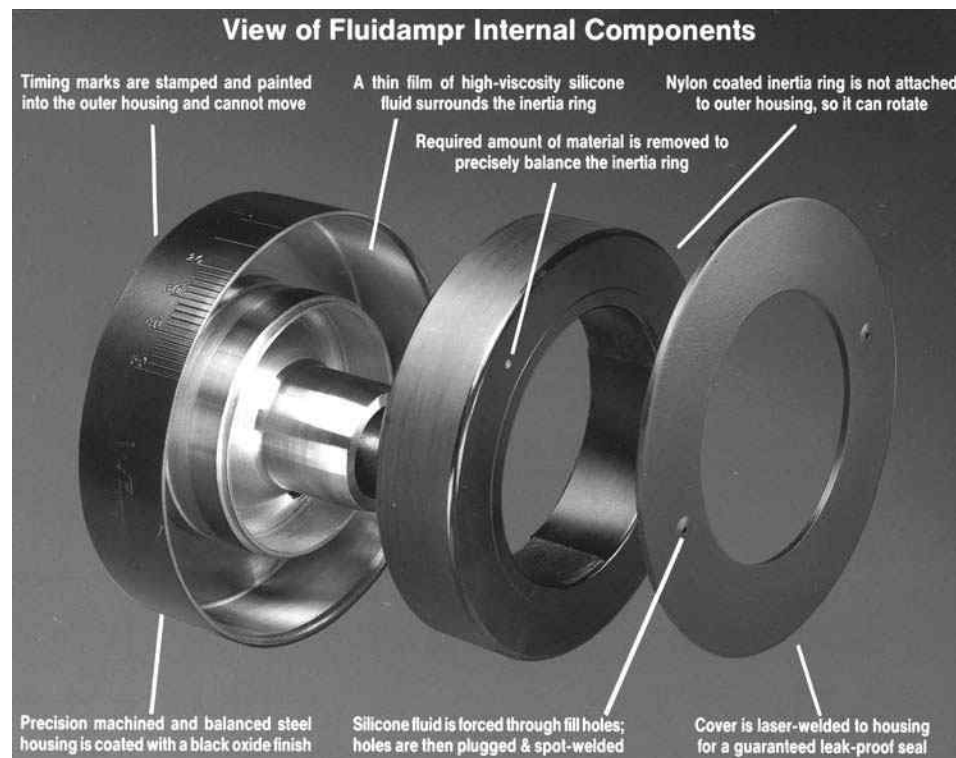
Figure 4-23 Exploded view of a viscous vibration damper. (Courtesy of Vibratech IDEX)
