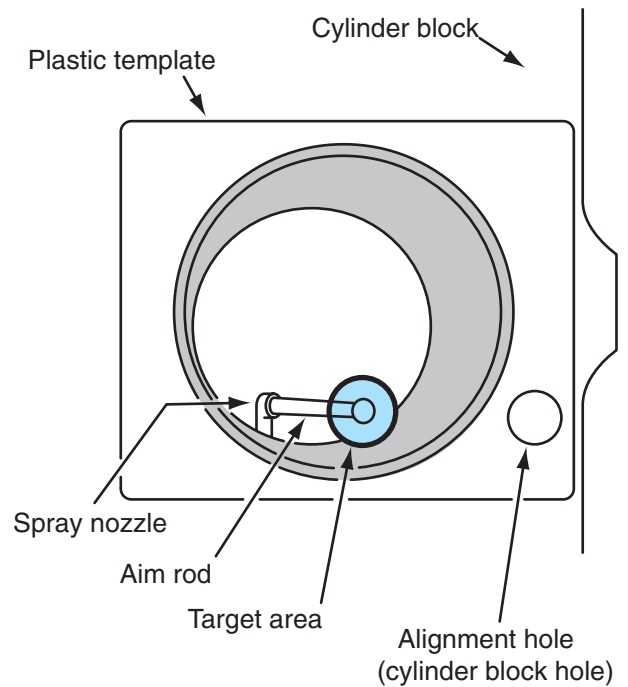
Figure 4-6 Spray nozzle targeting.
