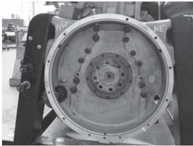
P3-4 On this engine we have marked reference points at NW, SW, SE, and NE. You may also use N, W, S, and E but check with the manufacturer service literature for their recommended method.
