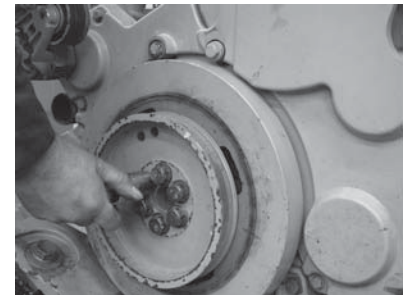
P3-6 Bar the engine in its correct direction of rotation (CCW from rear of engine, clockwise [CW] from front of engine) exactly 90 degrees to the SW reference point.
