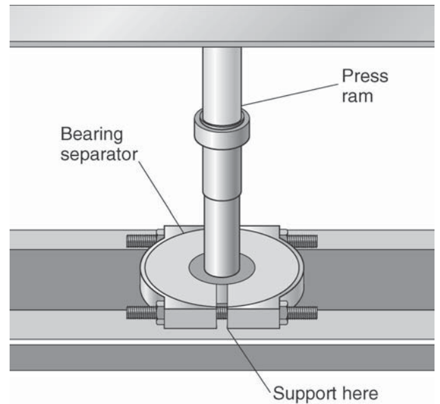
Figure 2-15 Press and bearing puller used to install a bearing on a shaft. (Courtesy of Ford Motor Company)
