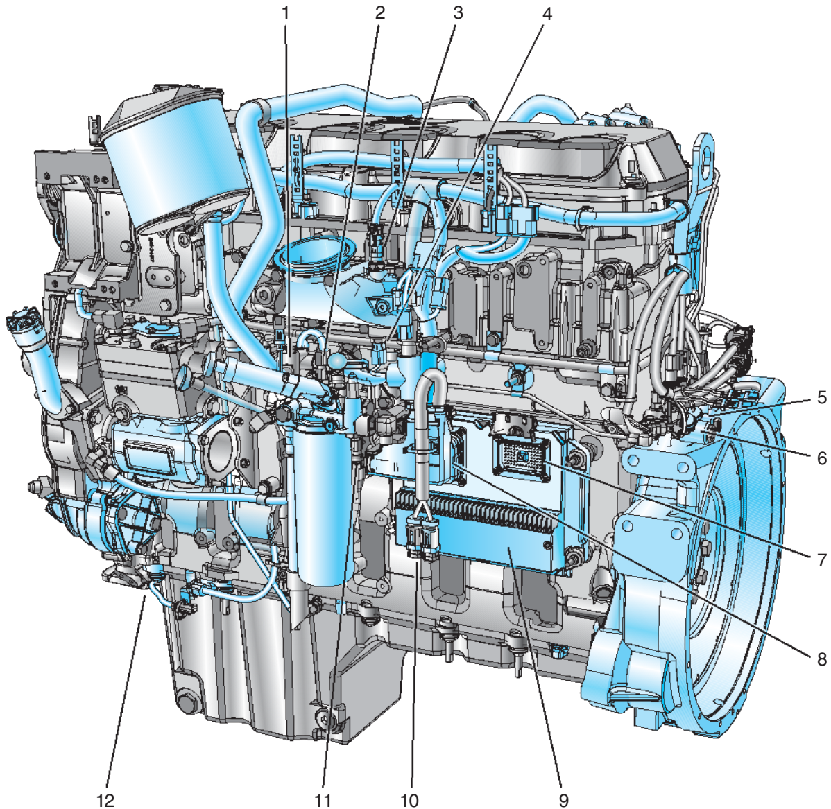
TYPICAL VIEW OF THE LEFT SIDE OF THE ENGINE
