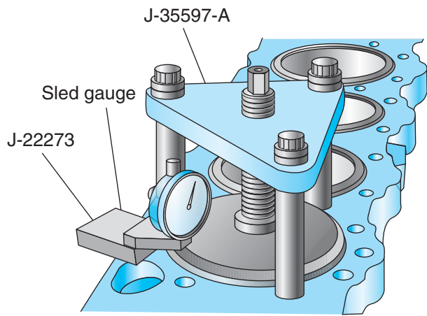
Figure 11-3 Measuring cylinder sleeve protrusion. (Courtesy of Navistar)
