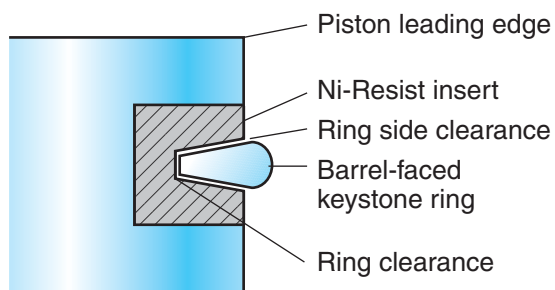
Ring Geometry Terminology
