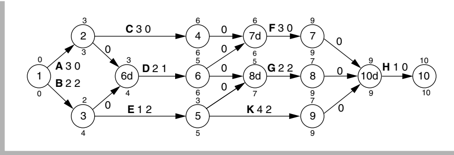
figure 14.37 Earliest completion time, latest completion time, and slack (additional edge item)
