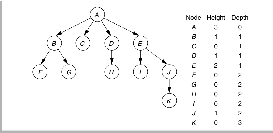
figure 18.1 A tree, with height and depth information
