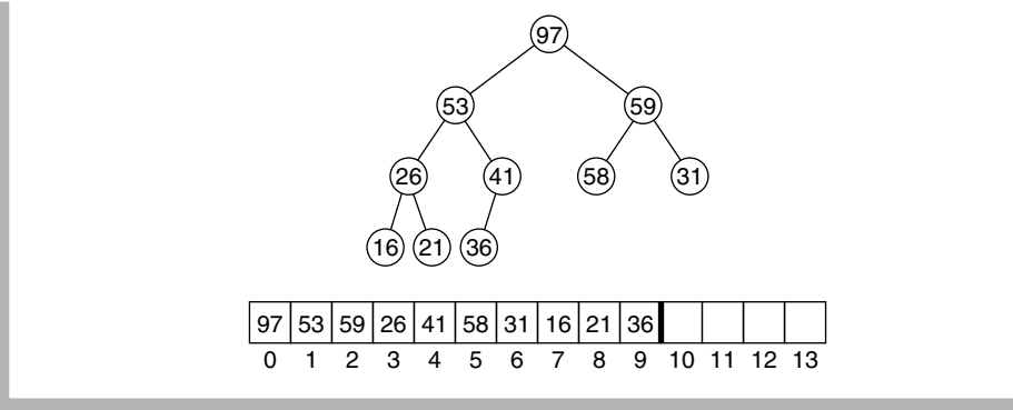
figure 21.25 Max heap after the buildHeap phase
