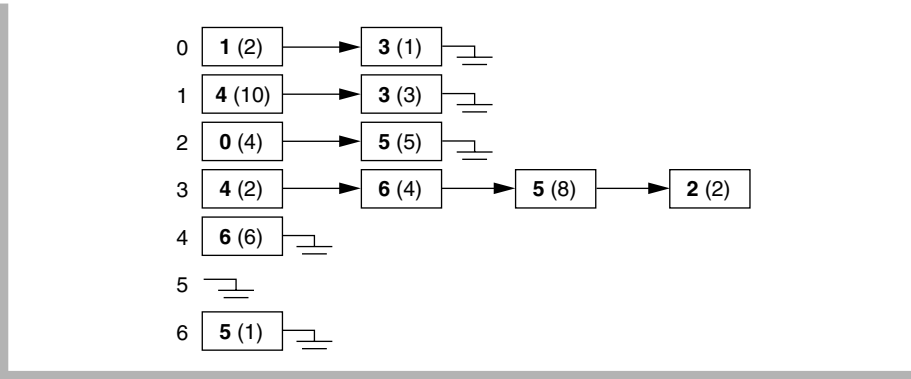
figure 14.2 Adjacency list representation of the graph shown in Figure 14.1; the nodes in list i represent vertices adjacent to i and the cost of the connecting edge.
