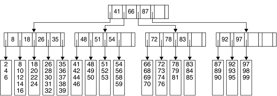
figure 19.84 A B-tree of order 5
