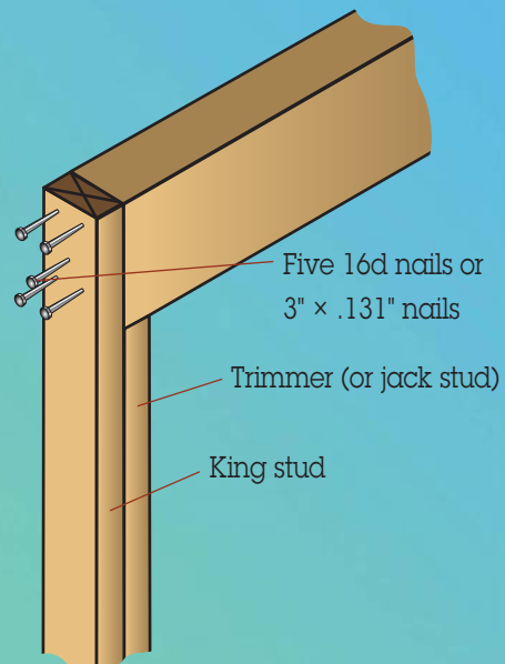
4 × 10 or 6 × 10 Header
