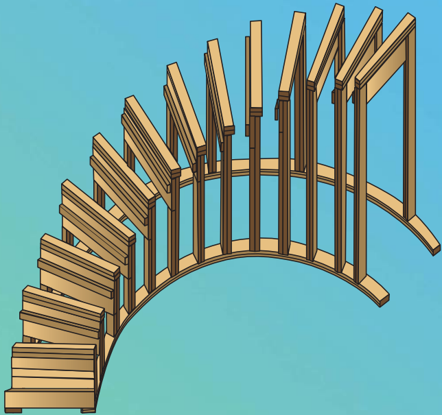
Tread Walls Nailed in Place
