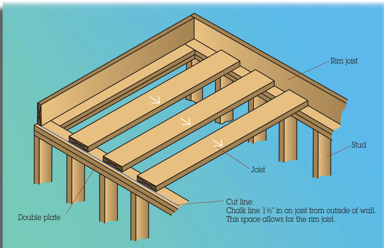
Joist spread and marked, ready to cut
