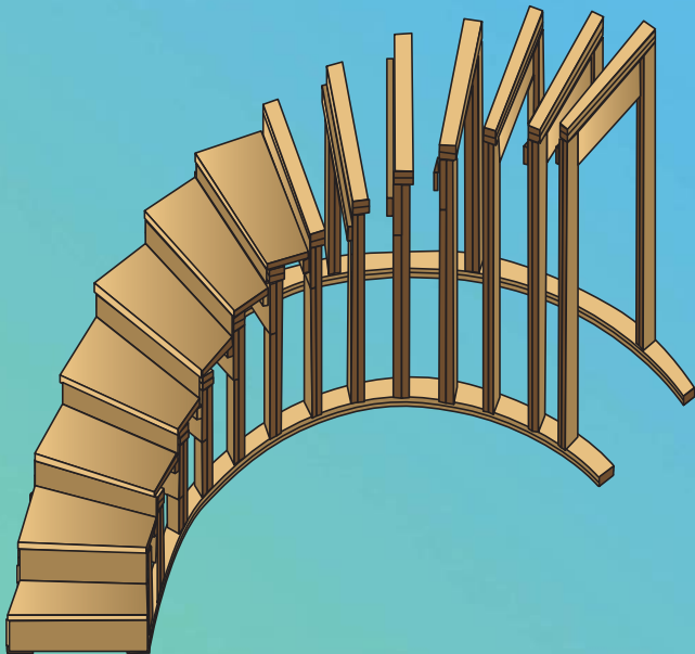
Tread Halfway Up Stairs
