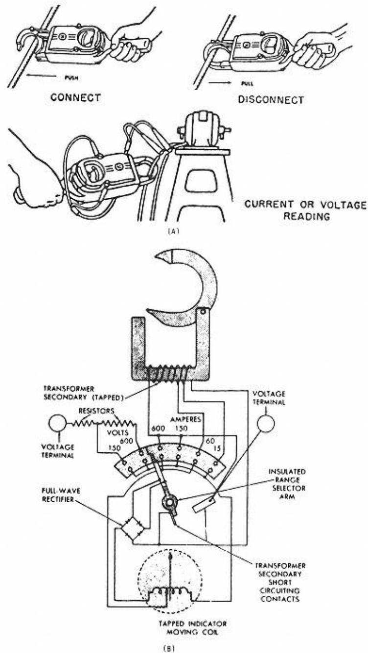
Figure 17-24 Clamp-on volt-ammeter: (A) Connecting, disconnecting, and reading; and (B) internal connections.
