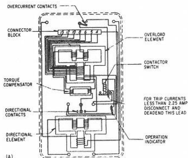
Figure 13-9 Directional overcurrent relays: (A) Rear view of internal wiring.
