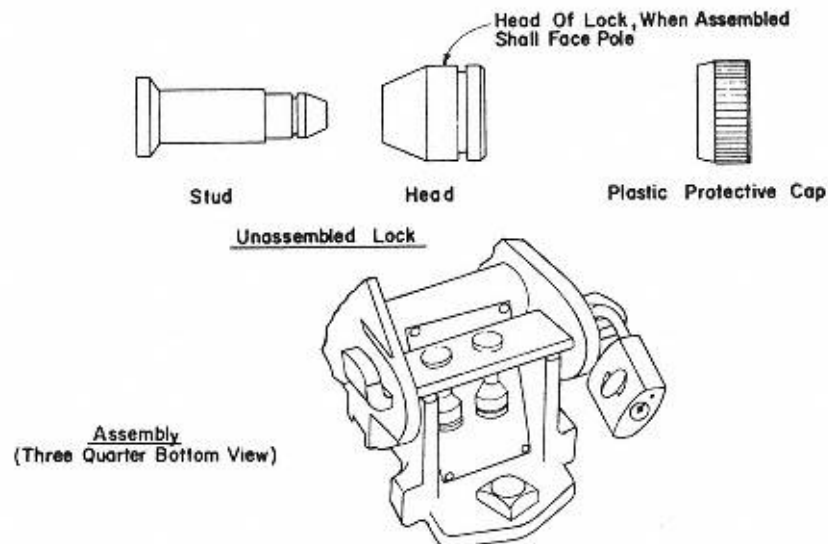
Figure 10-18 Locks and locking arrangements.
