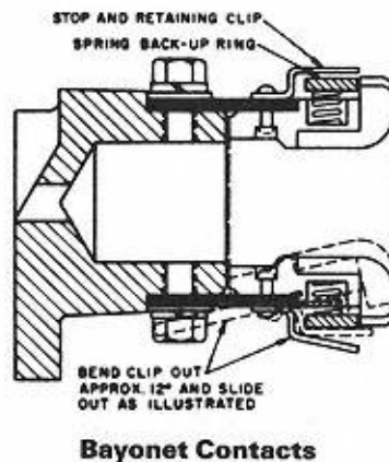
Figure 8-12 Bayonet contact.
