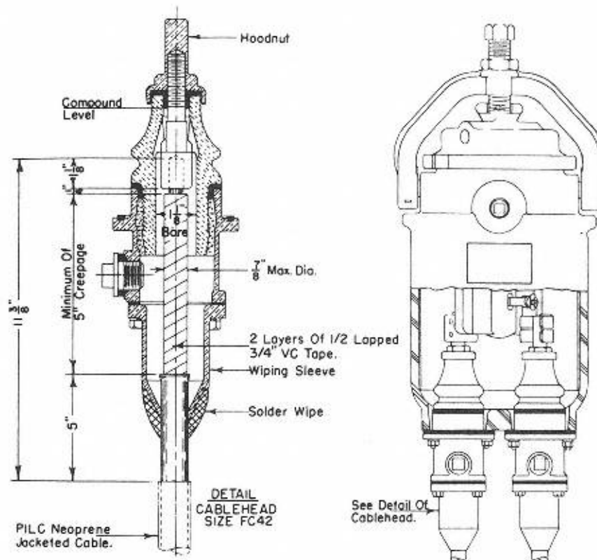
Figure 11-9 Oil fuse.
