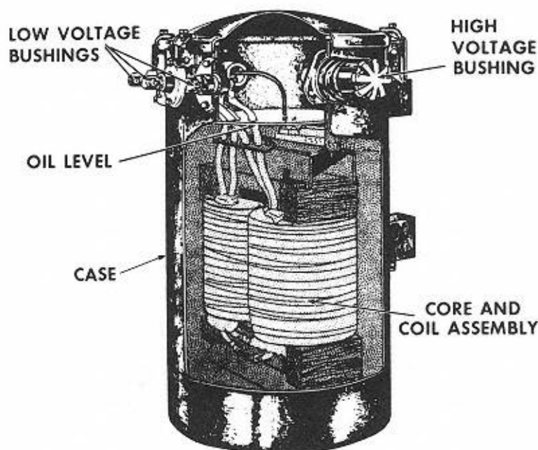
Figure 2-1 Basic components of a distribution transformer.
