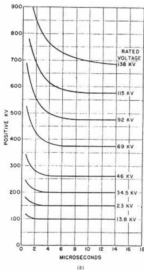
Figure 12-10 (cont.) (B) impulse characteristics of power class arresters. (Courtesy, McGraw Edison Co.)
