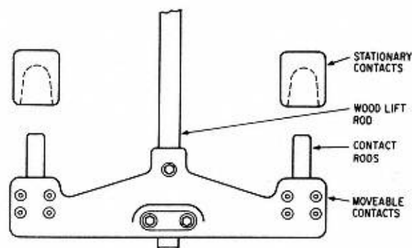
Figure 8-18 Lift rod assembly.
