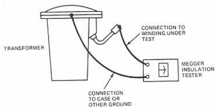
Figure 4-6 Megger testing of transformer winding.
