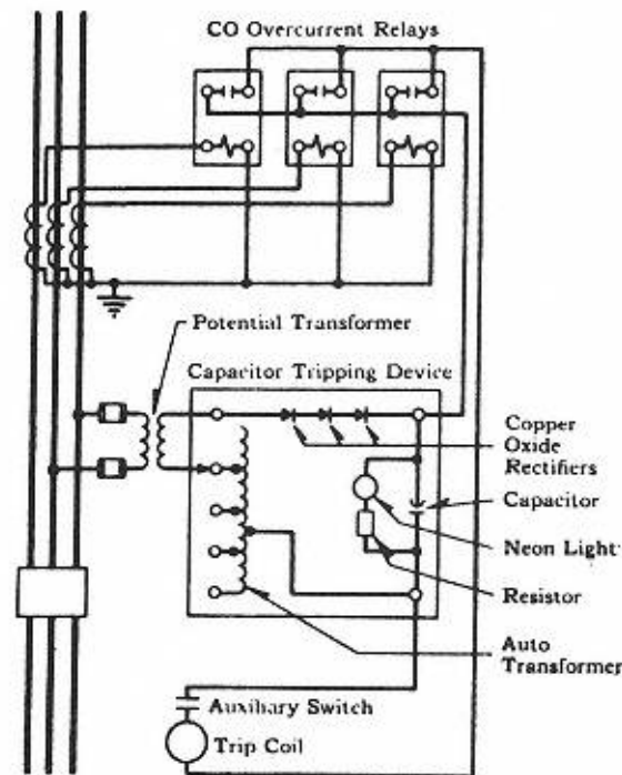
Figure 13-14 Capacitor as a source of tripping energy.
