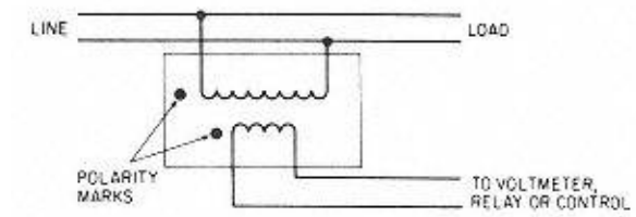
Figure 6-8 Potential transformer connection.
