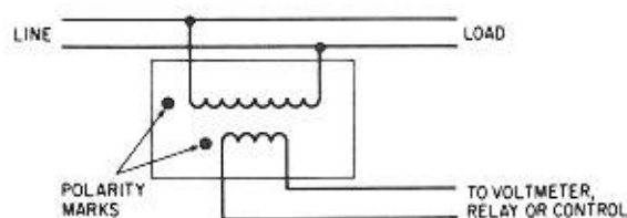
Figure 14-18 Potential transformer connection.
