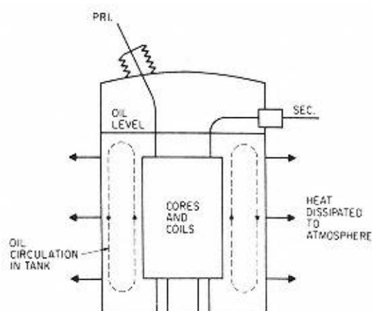
Figure 2-11 Cooling of core and coils by oil circulation.
