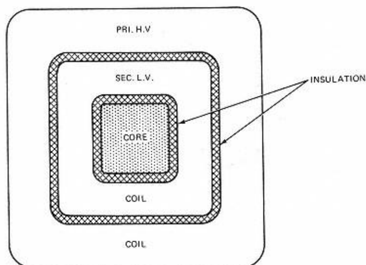
Figure 2-7 Concentric windings.
