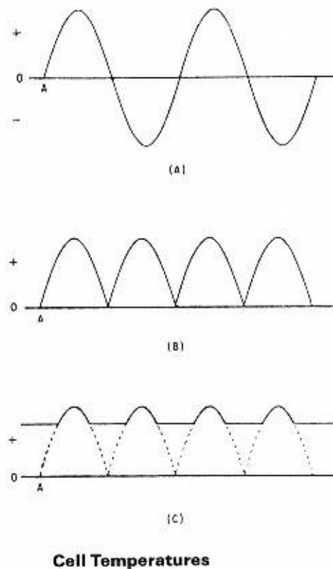
Figure 15-11 Rectifier method of battery charging: (A) A-C voltage wave shape, (B) rectified A-C voltage wave shape, (C) rectifier voltage impressed on battery voltage (solid line shows combination output voltage wave shape with ripples greatly exaggerated).
