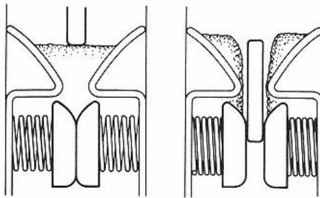
Figure 10-11 Area contact.
