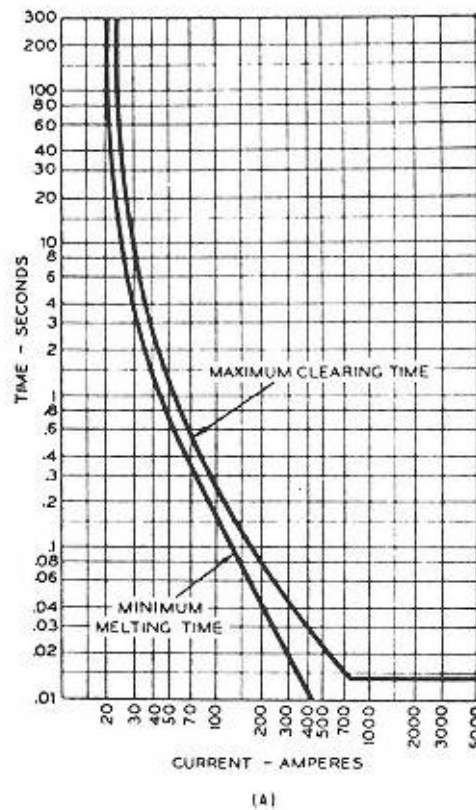
Figure 14-2 (A) Typical time-current curves for link fuse.
