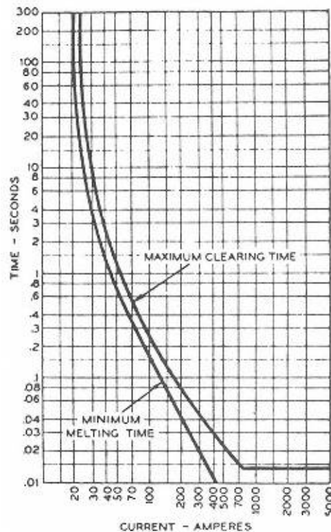
Figure 11-2 Typical time-current curves for a 10-k link. (Courtesy, McGraw-Edison Co.)
