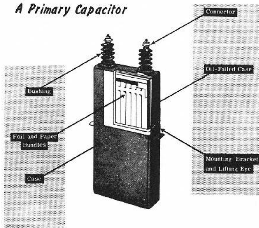
Figure 16-4 Capacitor construction.
