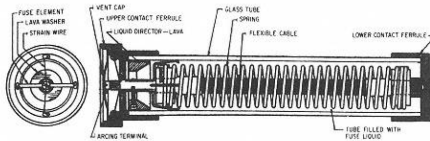
Figure 11-7 Liquid fuse with separate expulsion chamber.
