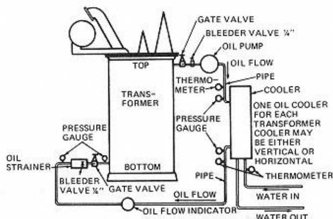
Figure 2-16 Piping diagram for forced, oil-cooled transformer.
