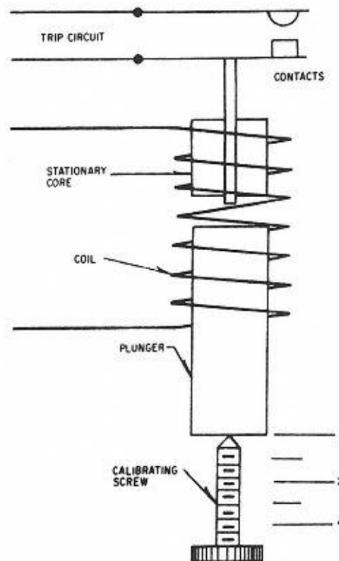
Figure 14-13 Plunger type of relay with coil wound for operation on either current or voltage.
