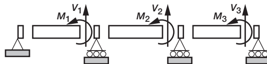
(b) Force model 1.
