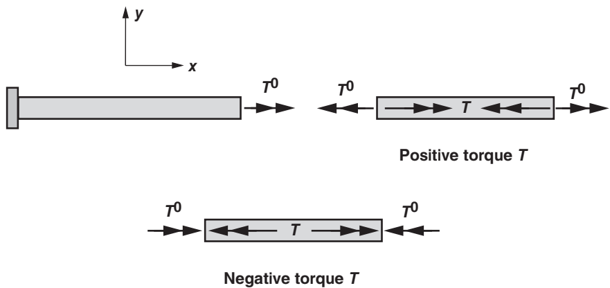
FIGURE 1-16 t-sign convention for internal torque T .
