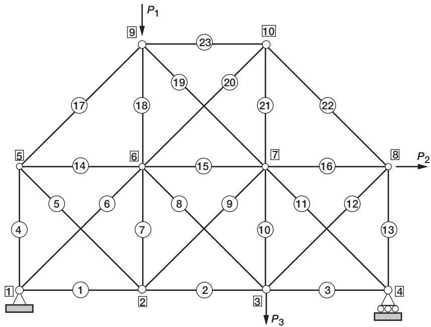
FIGURE 14-2 Six-bar truss.
