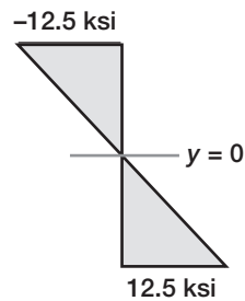
(c) Normal stress distribution.
