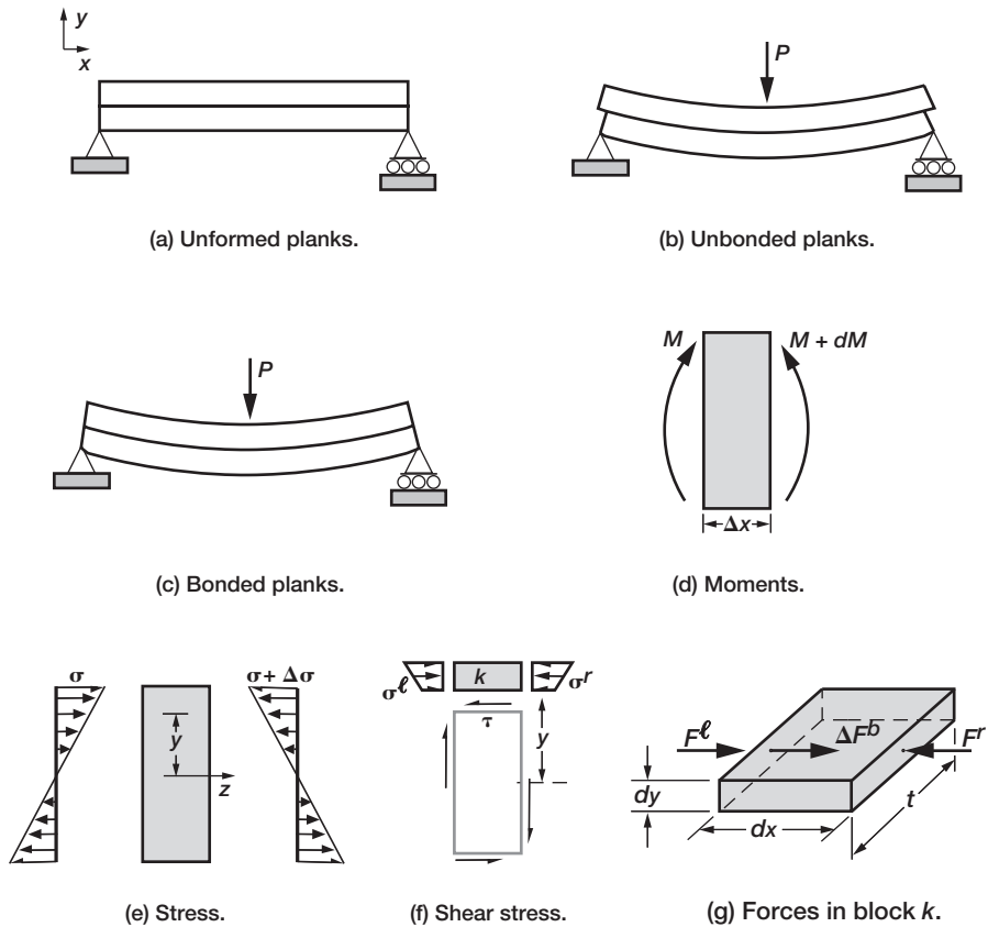
FIGURE 3-24 Shear stress in a beam.
