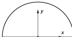
I_{xy} = 0 Semicircle
