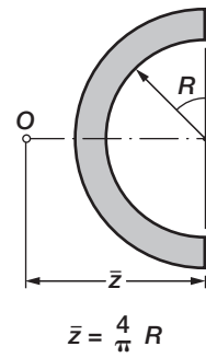
(c) Semicircular section.
