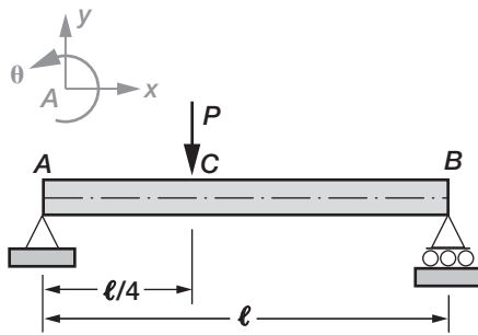
(a) Simply supported beam.
