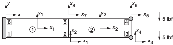
FIGURE 13-8 Cantilevered beam idealized by two membrane elements.
