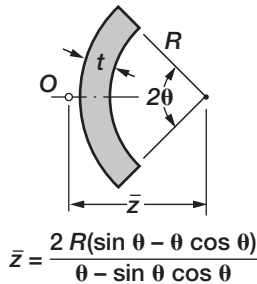
(e) Sector section.
