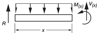
(c) Internal forces in beam.
