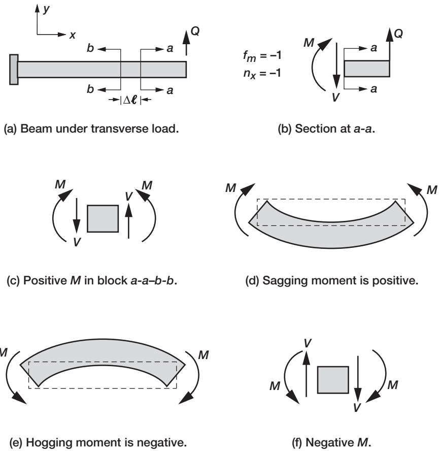
FIGURE 1-15 t-sign convention for bending moment and shear force in a beam.
