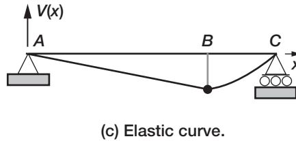
FIGURE 3-32 Elastic curve diagrams for Example 3-13.
