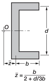
(a) Channel section.
