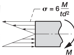
Correct solution by Coulomb
