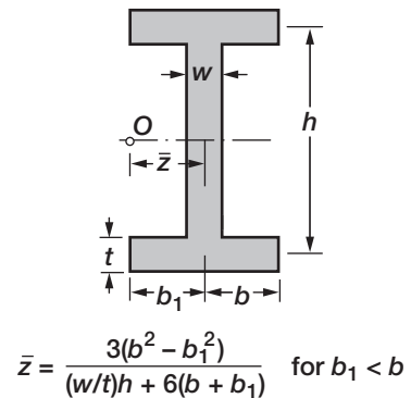
(f) Unequal I-section.
