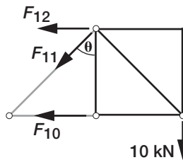
(b) Free body at C_1 – C_1 .
