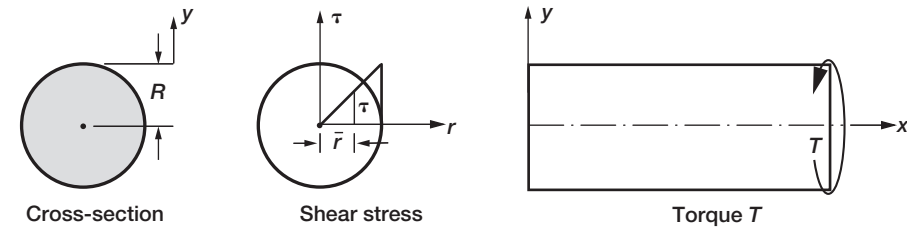
FIGURE A6-4 Shear stress distribution due to torque.
