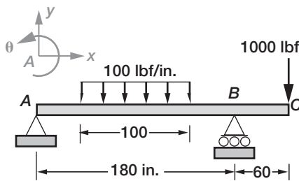
(a) Overhung beam.
