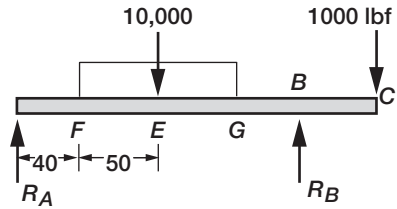
(b) Support reactions.
