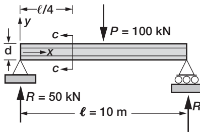
(a) I-beam.
