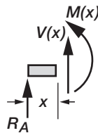
(c1) Segment AF.
