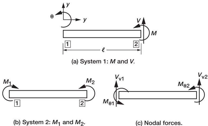
FIGURE 7-3 Two internal force systems for a beam.
