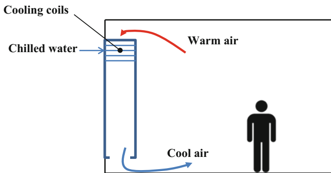
Fig. 5.8 Passive Displacement Ventilation illustration
