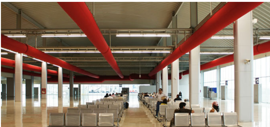
Fig. 5.9 Photo of a site with fabric duct installed (DuctSox.com)
