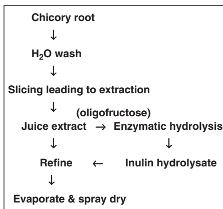
Fig. 6.4 Inulin and oligofructose manufacturing process. Adapted from Tunglund (2003).
