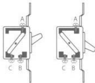
Fig. 6-13 This shows what happens inside a 3-way switch when the handle is thrown from one position to another. The current enters by the common terminal A, and leaves by either C or B depending on the position of the handle.
