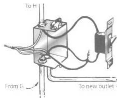
Fig. 10-8 Tapping in and splicing to add an outlet beyond an existing outlet. Be sure the box is large enough.
