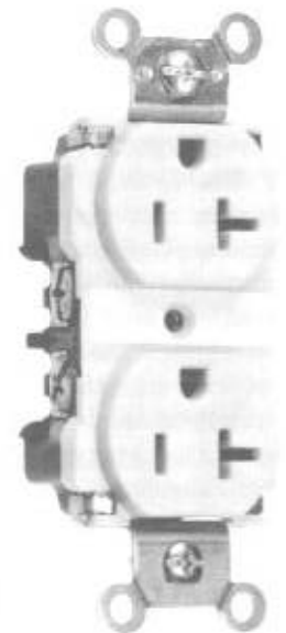
Fig. 2-2 A duplex receptacle, rated at 20 amps, 125 volts. The more common 15-amp version is identical in configuration except it does not have the horizontal slots extending to the right. The duplex receptacle has two terminal screws on each side, plus one green grounding screw (in this case at the upper right and not visible in this photo). The terminal screws at the left (ungrounded terminals) are finished with a brass or copper color; the screw terminals to the right (not visible) are for the grounded circuit conductor, and have a white or silvery white finish. (Pass & Seymour/Legrand)
