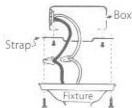
Fig. 15-5 Sometimes a strap is first mounted on the box, then the fixture is mounted on the strap. Straps with grounding terminals are available for nonmetallic boxes.
