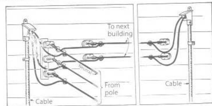
Fig. 17-6 When two buildings are near each other, tap the service wires from the pole where they are anchored on the first building and run them to the second building.
