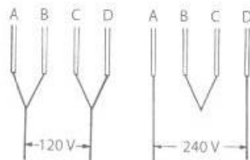
Fig. 16-1 By reconnecting the leads, the motor can be used on either 120 or 240 volts.
