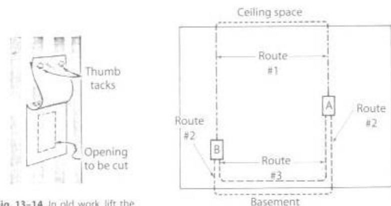
Fig. 13-15 In running cable from A to B (both on same wall) there is usually a choice of three routes for the cable. The best route depends on the structure of the building.
