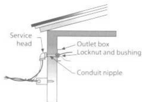
Fig. 10-17 Another method of entering a building, using an ordinary entrance cap, conduit, and a box inside.
