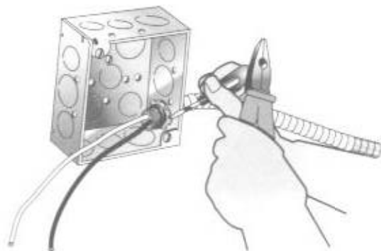
Fig. 9-13 Connector is then anchored to the box by means of a locknut inside the box.
