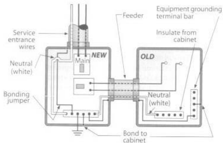
Fig. 13-1 Here the original equipment is not a part of the service equipment. It is only a "load center" for the original circuits.
