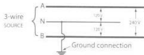
Fig. 7-1 The power supplier’s three wires provide two different voltages. Use the lower voltage (120 V) for low-wattage loads, and the higher voltage (240 V) for high-wattage loads such as range and water heater. Note the symbol for a connection to ground.
