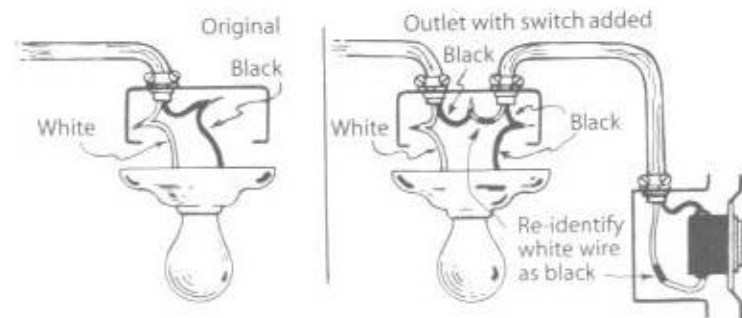
Fig. 13-19 Proper method of adding a single-pole switch to an existing outlet.
