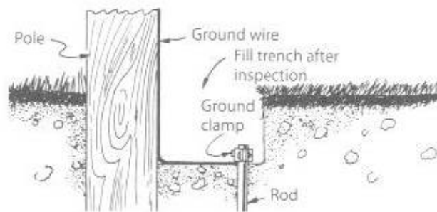
Fig. 17-2 The top of the usual 8-ft ground rod should end up below the surface of the ground. Fill the trench after inspection. If the ground rod is copper, use only a copper clamp. Per listing restrictions, insist on a DIRECT BURIAL or DB marking on the clamp.
