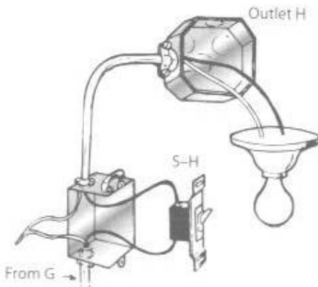
Fig. 10-7 Sometimes the cable from source does not run first to the outlet and then to the switch. Use this diagram when the cable runs first to the switch and then to the outlet.
