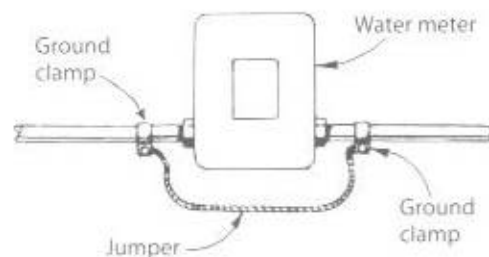
Fig. 8-27 Install a jumper around the water meter.
