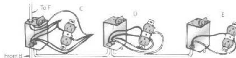
Fig. 10-5 Receptacle outlets are easy to connect, as this diagram shows.
