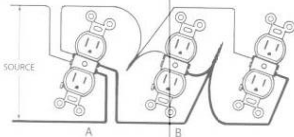
Fig. 6-10 Except where the white wire is part of a 3-wire circuit, feeding through may use the two screws on the device, as at A, but pigtailling as at B is a much better job.
