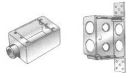
Fig. 9-18 PVC boxes with integral hubs and with standard knockouts.
