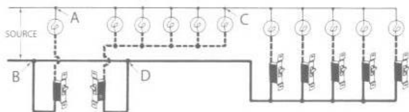
Fig. 6-12 The diagram of Fig. 6-11 rearranged to use less material.
