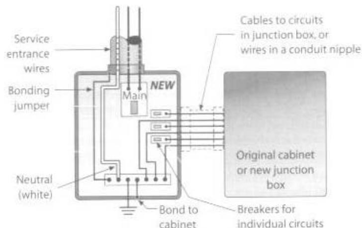
Fig. 13-2 Here the cabinet of the old equipment, if retained, serves only as a junction box.
