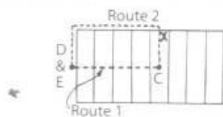
Fig. 13-18 At right, choice of routes for cable in Fig. 13-17 if joists run in the direction shown.
