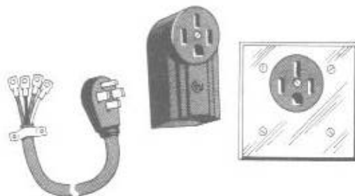
Fig. 14-2 Ranges are connected to 50-amp, 125/250-volt receptacles of the type shown here. The pigtail is connected to the range, then plugged into the receptacle.
