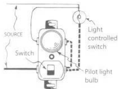
Fig. 6-23 The wiring scheme of a combination pilot light and switch. Another brand might be wired somewhat differently.
