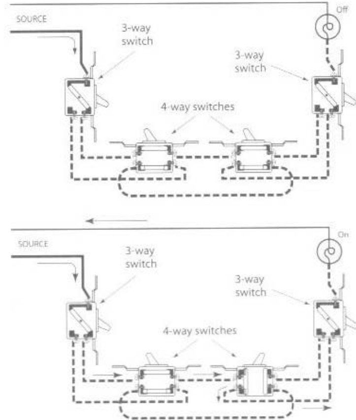
Fig. 6-21 Some brands of 4-way switches are connected as shown. With the 4-way switch handles in the positions shown in the upper diagram, the light is off; in the lower diagram, the light is on. Refer to Fig. 6-20 to identify terminals. ▼
