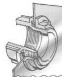
Fig. 8-26 Two-piece threaded hub. Serrations on both pieces bite into enclosure metal, making a bonding jumper unnecessary. O-ring in outside piece forms a raintight seal.
