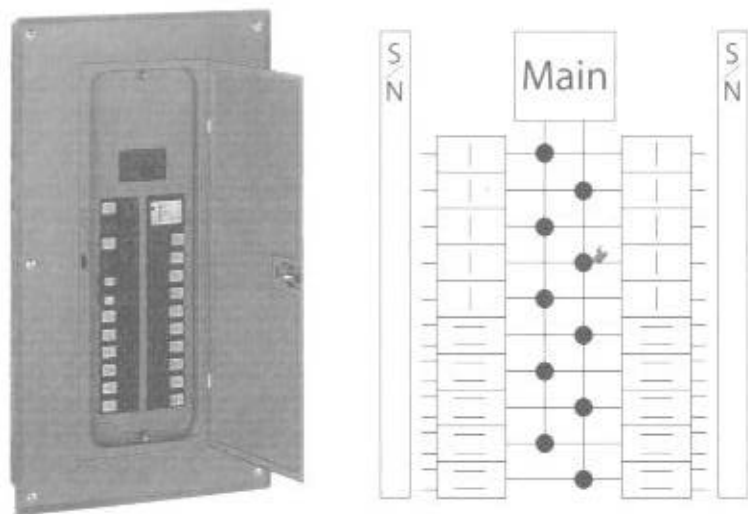
Fig. 8-1 On the left, a circuit breaker cabinet with main breaker ( Square D Company ). On the right, diagram showing space for 20 circuits. ( Square D Company ) Arrangements for mounting plug-in circuit breakers vary by manufacturer; a label in the panelboard lists catalog numbers of breakers permitted to be installed.
