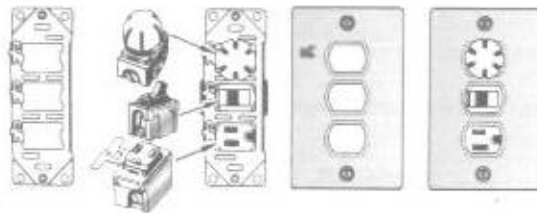
Fig. 9-16 Interchangeable devices permit 3 switches, receptacles, and the like to be installed in a single-gang box.
