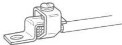
Fig. 4-12 Solderless connectors of this type are used with heavy sizes of wire. (The Halex Company)
