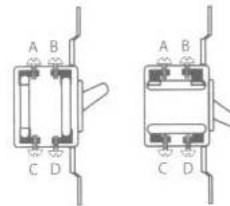
◀ Fig. 6-20 Internal connections of the other style of 4-way switch with the handle in the up and the down positions. Terminals are labeled A , B , C , and D .
