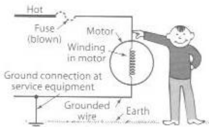
◀ Fig. 7-2 A 120-V motor with grounded wire correctly connected to the grounded neutral and a fuse correctly placed in the hot wire. (Grounding wire not yet installed.)
