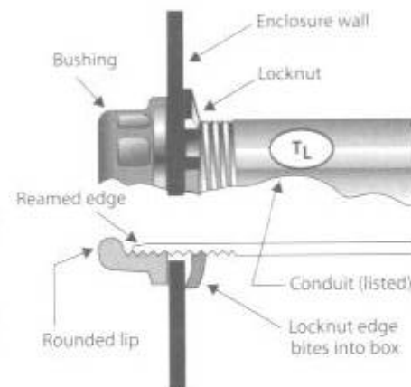
Fig. 12-3 Conduit is fastened to boxes by means of locknuts and bushings, both shown above.
