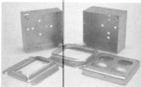
Fig. 9-6 Four-inch square boxes and covers. Use covers on the left and middle when wiring is concealed. For permanently exposed wiring, use the type of cover shown on the right. (Hubbell Electrical Products)
