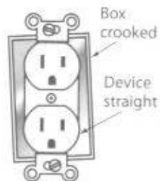
Fig. 15-2 Elongated holes in strap allow devices to be mounted straight in a crooked box.
