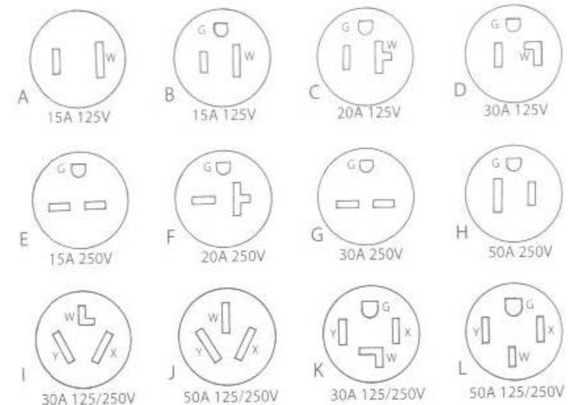
Fig. 14-1 An assortment of receptacles. Those rated at 15 and 20 amps have a diameter of 1.32 inches. Those rated at 30 and 50 amps have a diameter of 2.12 inches. In the illustrations, the opening marked G is for the equipment grounding wire; the one marked W is for the white circuit wire; those marked X, Y or Z are for the hot circuit wires.
