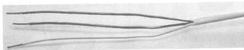
Fig. 18-3 Shown above are wires for connecting doorbells and chimes. This cable is listed as "CL2" which means it can be used for most general-purpose applications, but not in risers and plenum cavities in high-rise or commercial occupancies, which are beyond the scope of this book.
