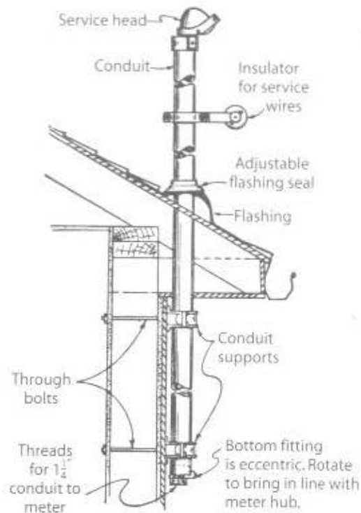
◀ Fig. 8-10 On rambler or ranch-house construction, a mast gives the service wires necessary clearance above ground.
