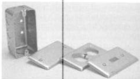
Fig. 9-5 This box is known as a "handy box" or "utility box." Use it for permanently exposed surface wiring as in basements, garages, etc. The box and covers have rounded corners for safety. (Hubbell Electrical Products)
