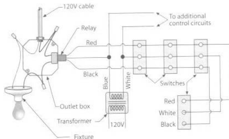
Fig. 18-7 Typical remote-control circuit, in this case with the outlet controlled at four locations. One transformer is used for the entire house. The same circuit is often used for remote control yard lights.
