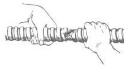
Fig. 11-11 A twist will remove the cut end of the armor. Let about 8 inches of wire extend beyond the armor. ▶
