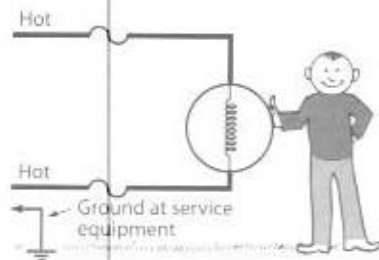
◀ Fig. 7-6 A 240-V motor with each hot wire correctly protected by fuse/breaker. The grounded wire does not run to 240-V loads. Because the grounding wire has not been installed, shock hazard is avoided only if the motor remains in perfect condition.
