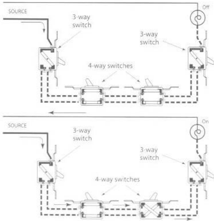
Fig. 6-19 Four-way switches are usually connected as shown here. With the 4-way switch handles in the positions shown in the upper diagram, the light is off; in the lower diagram, the light is on. Two 4-way switches are shown in the circuit, but any number may be installed depending on need. Refer to Fig. 6-18 to identify the terminals. ▼
