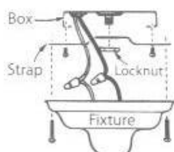
Fig. 15-6 Another method of mounting a fixture.
