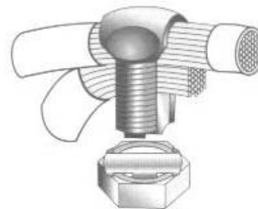
Fig. 4-23 Use this split-bolt connector when splicing a heavy wire to another continuous heavy wire. The assembled connector and wires must be taped.
