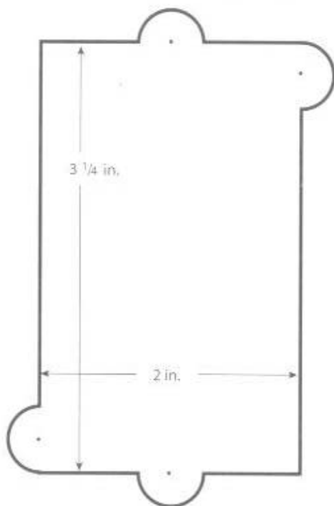
Fig. 13-5 Dimensions of hole for installing a switch box. To save time, make a template. Photocopy this page, glue it to a piece of stiff cardboard, and cut to size.
