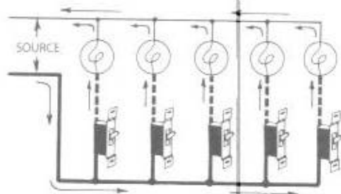
Fig. 6-8 This diagram shows the same parallel wiring as Fig. 6-7, but with each lamp controlled by a separate switch. Note that the white wire runs directly from SOURCE to each lamp.
