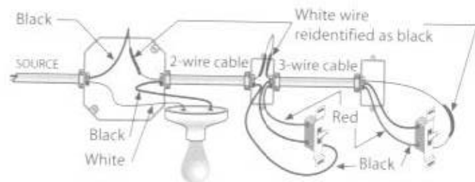
Fig. 10-6 The wiring of outlet F of Figs. 10-1 and 10-2, with the two 3-way switches that control the outlet. This is the diagram for any outlet controlled by 3-way switches when using cable. Study carefully the colors of the wires in this cable. Compare it with Fig. 6-14.
