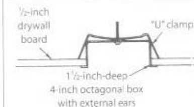
Fig. 13-12 Recessed box supported from drywall board by U-clamp and box ears.
