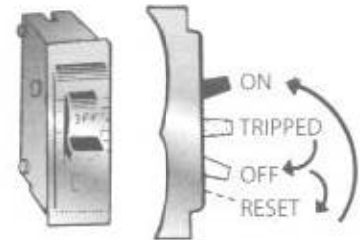
Fig. 5-6 A single circuit breaker (left) and method of resetting the breaker if it trips.
