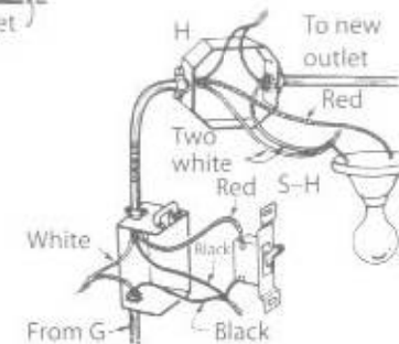
Fig. 10-9 Running three-wire cable and splicing to add an outlet beyond an existing outlet. ▶
