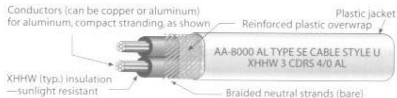
Fig. 8-12 In service entrance cable the neutral wire is not insulated, but is bare and wrapped spirally around the insulated wires. The drawing shows 3-wire cable.
