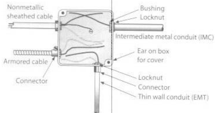
Fig. 17-16 How to change from one wiring method to another. Install a cover on the box upon completion.
