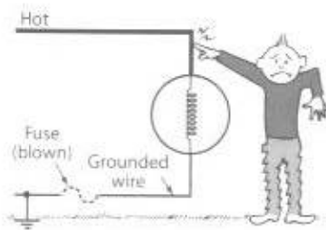
Fig. 7-3 A 120-V motor with a fuse wrongly placed in the grounded wire. It is a dangerous installation. ▶
