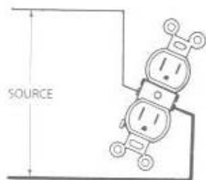
Fig. 6-9 Wiring for a receptacle. (To simplify the drawing, the connection to the green grounding screw on the receptacle is not shown. See page 126 for requirements.)
