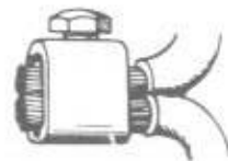
Fig. 4-22 For heavier wires, use metal connectors. The assembled connector and wires must be taped.
