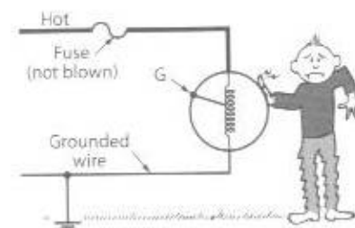
◀ Fig. 7-4 The same motor as in Fig. 7-2, but the motor is defective. G represents an accidental grounding of the winding to the frame. The grounding wire has not been installed. This is a dangerous installation.
