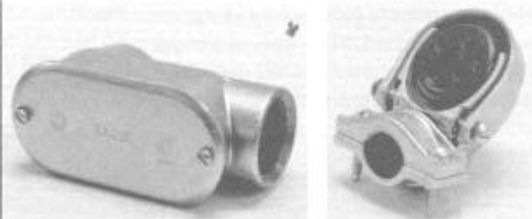
Fig. 8-21 Service head (at right) is for use when wires run through raceway. Use with special entrance ell (at left) which has a removable cover. (Hubbell Electrical Products)
