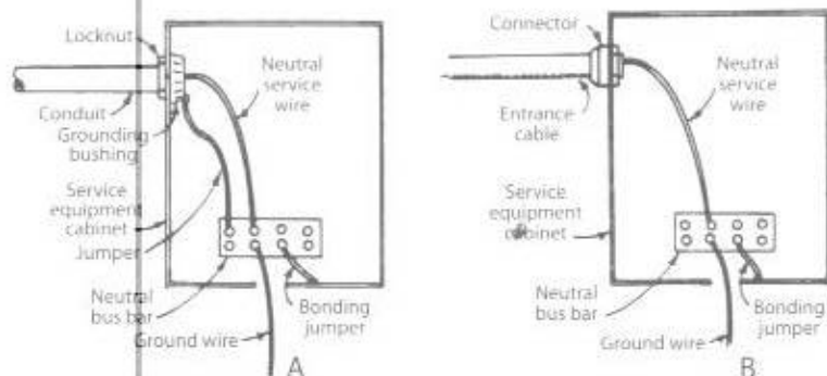
Fig. 8-24 Typical grounding connections. Only the white wire is shown. The wire marked "bonding jumper" is usually part of the service equipment as purchased; it could be either a green screw or a flexible strap.
