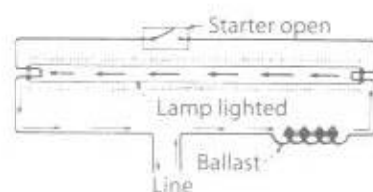
Fig. 2-4 The starter has opened, current flows through the tube; the lamp is lighted.
