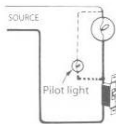
Fig. 6-22 The basic circuit of a pilot light.
