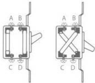
◀ Fig. 6-18 Internal connections of one style of 4-way switch with the handle in the up and the down positions. The terminals are labeled A , B , C , and D .
