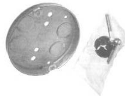
Fig. 13-3 This ceiling pan, with a volume of 6 cubic inches and no required fill adjustments for an internal cable clamp, can just accommodate a single 14-2 AWG Type NM cable, or a 14, 12, or 10-2 AWG Type AC cable.
