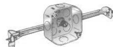
Fig. 9-10 Boxes preassembled with hangers are often used.
