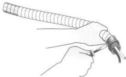
Fig. 9-12 Connector is first attached to the cable by means of a clamp screw.
