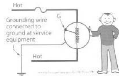
◀ Fig. 7-8 The same defective motor as Fig. 7-7, but a grounding wire has been installed from the frame of the motor to ground. Even though the winding is accidentally grounded to the frame, as represented by G, the shock hazard is minimized.
