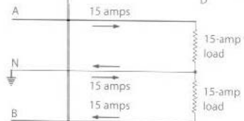
◀ Fig. 10-15 One 3-wire circuit. Each half carries 15 amps but the neutral N carries no current. The NEC term is "multiwire branch circuit." Both terms are used in this book.
