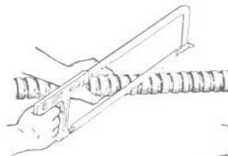
Fig. 11-10 In cutting armored cable with a hacksaw, note the proper angle of the blade. Be careful not to damage the wires.
