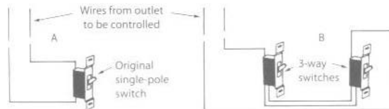
Fig. 10-10 It is a simple matter to substitute a pair of three-way switches for a single-pole switch in any wiring diagram. Simply substitute the right-hand combination for that at left.
