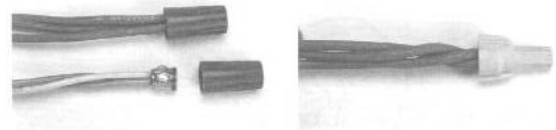
Fig. 4-18 Two types of solderless connectors for smaller wires, often called by the trade name "Wire Nut." The version with the setscrew maintains the integrity of the electrical connection even with the insulating cap removed. This makes it a good choice if the connection will be tested with diagnostic equipment while energized, such as with some motor connections.
