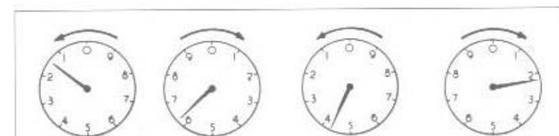
Fig. 3-1 To read this meter, write down the numbers the pointers have passed.
