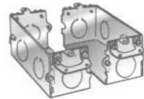
Fig. 9-2 Two single boxes are easily changed into one larger “two gang” box. Made the same way are still larger boxes of three or four or more units ganged together. Ready-made two-gang and larger boxes are also available.
