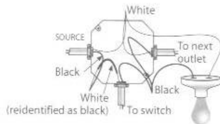
Fig. 10-4 Outlet B of Figs. 10-1 and 10-2. This is an important diagram. It shows how to connect white wire in cable to the switch.
