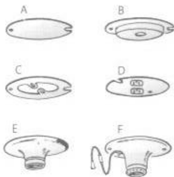
Fig. 9-4 Every outlet box must be covered. Some common covers: A) blank cover; B) drop cord cover; C) spider cover; D) cover with duplex receptacle; E) keyless receptacle for lamp; F) same as E but with pull chain.
