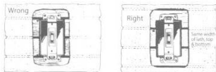
Fig. 13-4 In cutting an opening for a switch box, cut away one whole lath and part of another lath on each side of the one completely cut. This provides a rigid mounting for the box.
