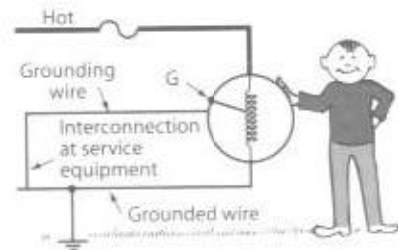
Fig. 7-5 The same defective motor as Fig. 7-4, but now a grounding wire has been installed from the frame of the motor to ground. Even though the winding is accidentally grounded to the frame, as represented by G , there is no shock hazard. ▶
