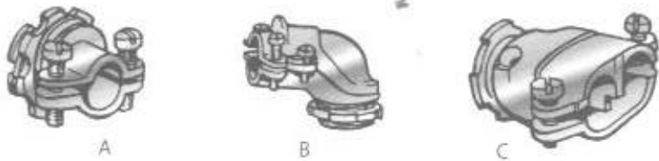
Fig. 9-11 Connectors used in anchoring cable to boxes.
