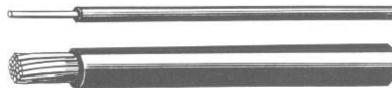
Fig. 4-3 Type TW is seldom used today, having been largely replaced by dual-rated THHN/THWN, which uses the same insulating compound, but in a much thinner layer overlaid by a tough outer layer of clear nylon that provides excellent mechanical protection. It may be used in wet or dry locations. Number 6 AWG or larger must be stranded, and 8 AWG must be stranded if pulled into conduit.
