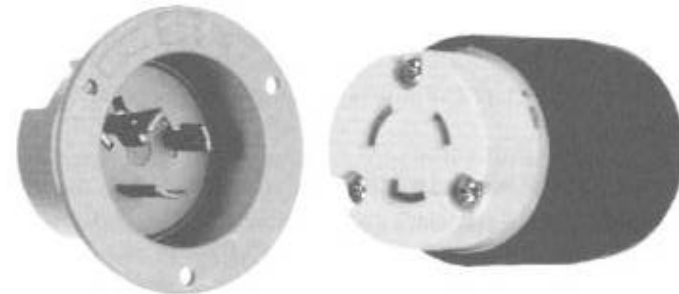
Fig. 8–28 Flanged inlet and the mating receptacle cord body that could energize it. (Pass & Seymour/LeGrand)
