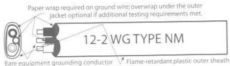
Fig. 4-5A Nonmetallic-sheathed cable consists of two or more individual wires assembled into a cable. The Type NM two-wire with ground shown here may be used only in dry locations.
