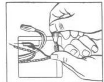
Fig. 4-19 This kind of connector contains a tapered coil spring inside the insulating cover.
