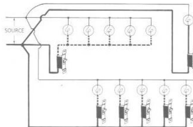
Fig. 6-11 The outlets of Figs. 6-5, 6-7, and 6-8 have been combined into a single group of outlets. In other words, here they form one circuit. This still uses a great deal of material. To reduce the amount required, the circuit can be arranged as the next diagram shows.
