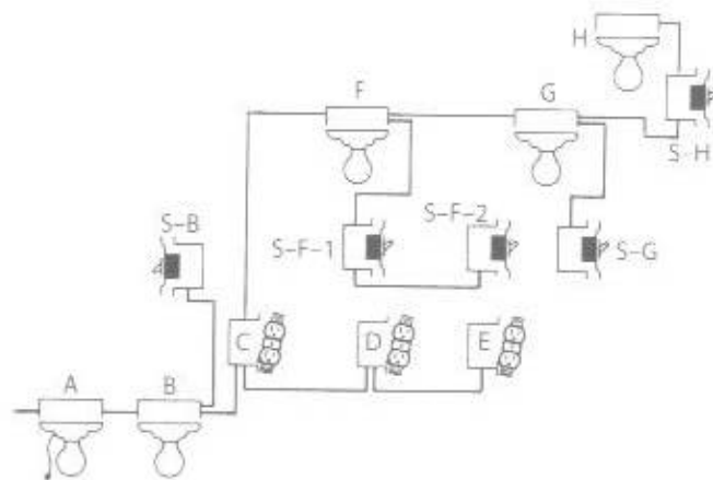
Fig. 10-1 Before doing any wiring, make a rough layout of each circuit showing location of each outlet and how cable will run from box to box. Shown here is a layout of a circuit with 8 outlets labeled A to H, 3 single-pole switches S-B, S-G, and S-H, and a pair of 3-way switches S-F-1 and S-F-2. The wires for this circuit begin in the basement and run to main floor living room, kitchen, and dining room, and then to a bedroom.
