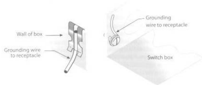
Fig. 11-5 The grounding wire to the green terminal of a receptacle may be grounded to the box using either a grounding screw or grounding clip as shown at left above.
