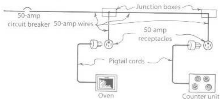
Fig. 14-3 It is common to provide separate circuits for oven and counter units, but both may be placed on one circuit as shown.
