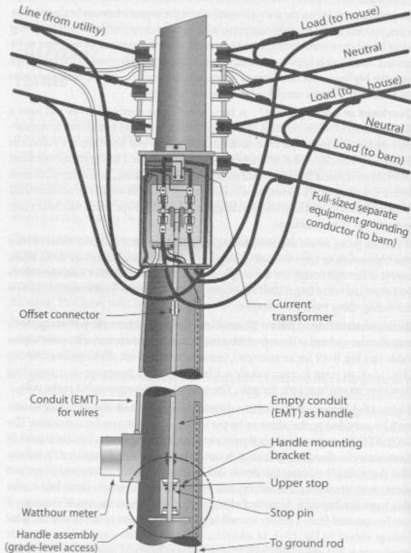
Fig. 17-1 Pole top switch and remote metering as anticipated by the 2002 NEC. Leave at least half the circumference of the pole clear to allow line workers and repair workers to climb the pole without trouble.
