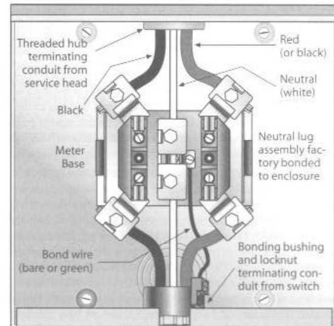
Fig. 8-20 How wires are connected to the meter base or socket. If cable is used, the bare uninsulated wire is always connected to the neutral center contact of the socket, and the bonding bushing and wire are not used.
