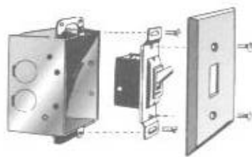
Fig. 15-1 The switch or other device is first mounted in the box, and the plate is then fastened to the device.
