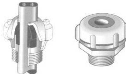
Fig. 8-14 Watertight connectors for outdoor use. To prevent leaks, apply duct seal around the cable entry.
