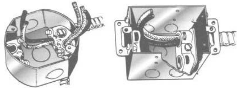
Fig. 9-14 With boxes of this type, separate connectors are not used. The boxes have clamps to hold the cable.
