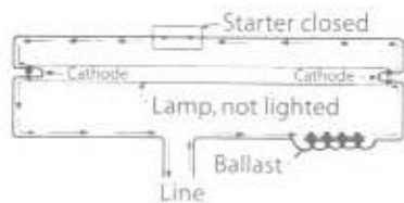
Fig. 2-3 The current has just been turned on. The starter is still closed.
