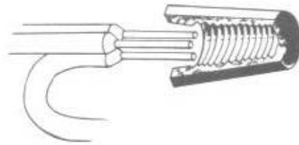
Fig. 4-15 Use this method, commonly called a "pigtail" splice, when you would otherwise have to connect two wires under a terminal screw.
