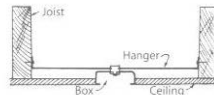
Fig. 9-9 Hanger with box supported in ceiling.
