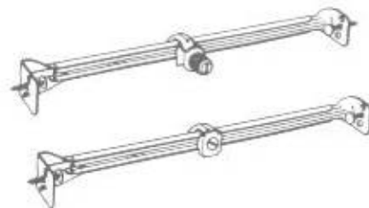
Fig. 9-9 Hanger with box supported in ceiling.
