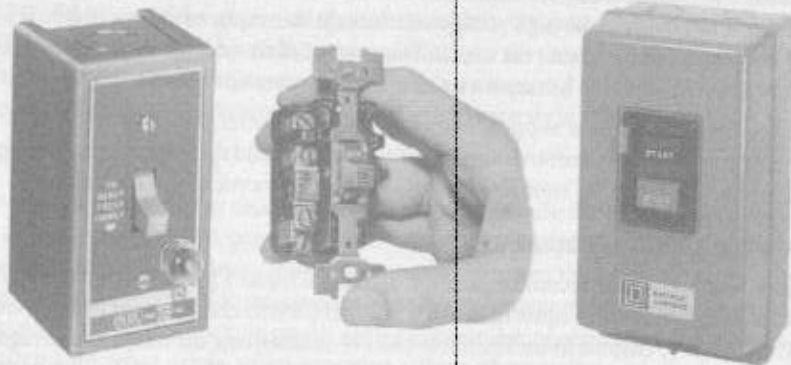
Fig. 16-2 Controls of these types are "manual motor controllers." They are used to start and stop a motor; they also contain motor overload devices. If marked SUITABLE AS MOTOR DISCONNECT they can additionally function as the required disconnecting means. (Square D Company)
