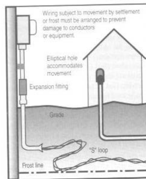
Fig. 17-9 Support hardware and expansion fitting for RNC that will be exposed to outdoor conditions.
