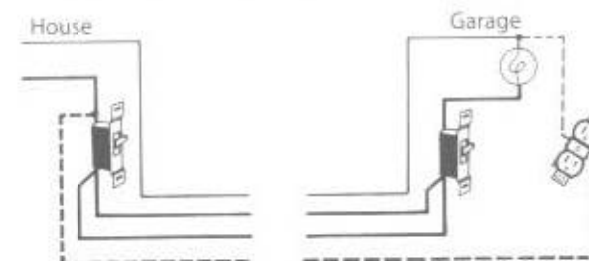
Fig. 10-19 If a receptacle that is to be permanently on is added, 4 wires are needed.
