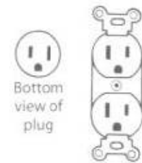
Fig. 7-11 Grounding receptacle and plug. Plugs with either 2 or 3 blades will fit.
