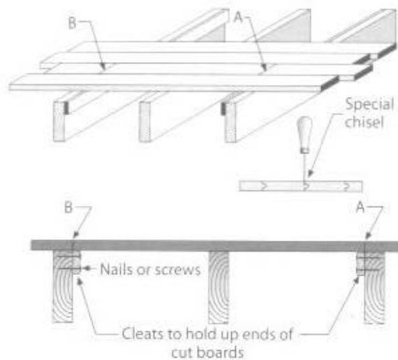
Fig. 13-13 Sometimes floor boards must be lifted. If the boards are tongued and grooved, cut off the tongue on each side with a very thin chisel, then saw across next to the joists. To simplify the drawing, the subfloor is not shown.
