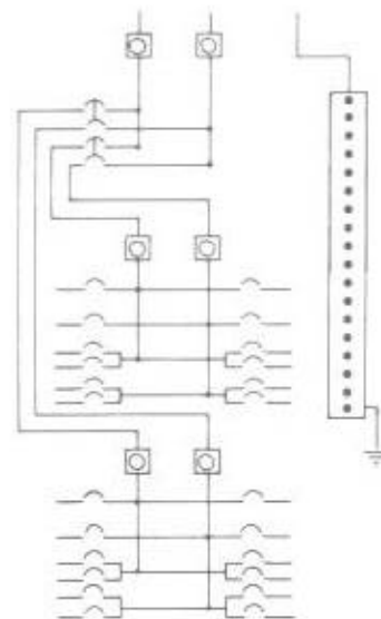
Fig. 8-2 Diagram for a split-bus circuit breaker cabinet.
