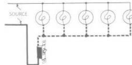
Fig. 6-7 Style of wiring known as "parallel" wiring. It is used for all ordinary purposes.
