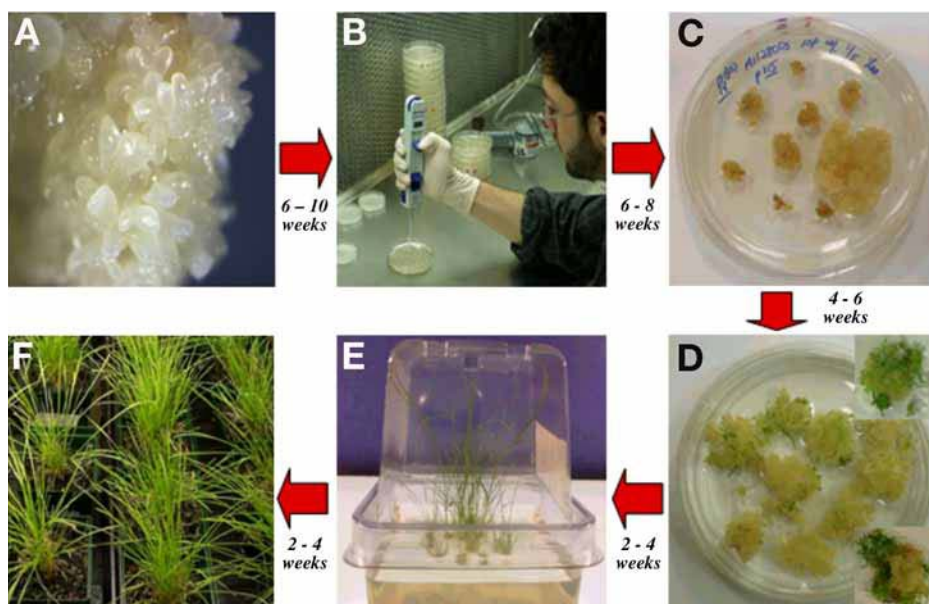
Fig. 3. Standard operating procedures for Agrobacterium -mediated transformation of turfgrass. (A) Induction and selection of embryogenic creeping bentgrass calli. (B) DNA delivery using Agrobacterium tumefaciens and the “spotting” method. (C) Selection of transformed calli using bar or hyg resistance. The colonies that do not carry the transgene die while putative transformants thrive and continue to grow under selection pressure. (D) Regeneration 1 for transformed calli under continued selection pressure. (E) Regeneration 2 for transformed calli under continued selection pressure. (F) Regenerated transformed plants are placed into soil for further growth and development.
