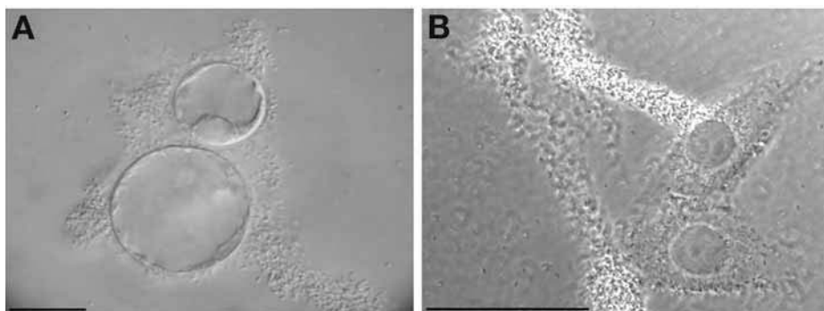
Fig. 1. Agrobacterium cells are capable of attaching to cells of evolutionary-distant host species. Similar attachment patterns, with characteristic bacterial aggregates at and around the host cells, were observed when Agrobacterium was co-incubated with petunia protoplasts ( A ) and HeLa cells ( B ). Bars = 50 \mu\text{m} . reproduced from ref. 23 with permission from The National Academy of Sciences of the United States of America.
