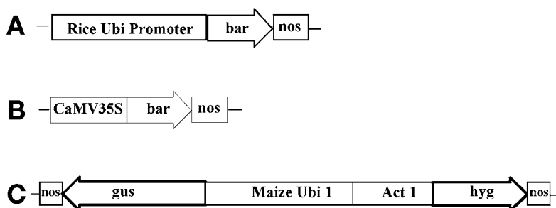
Fig. 1. Diagrams of the plasmid constructs used for turfgrass transformation. Plasmids with the Rice Ubi:bar ( A ); CaMV35S:bar ( B ) are vectors utilizing bar as a selectable marker for PPT selection. Plasmid pUbi-gus/Act-hyg ( C ) contains a Maize Ubi promoter-driving reporter gus gene and a rice actin promoter-driving hygromycin resistance gene for selection.
