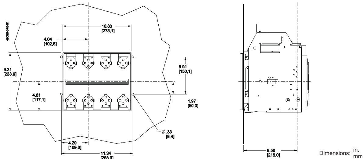
Figure 58: 800–1200 A Masterpact NT IEC 4P Drawout—Rear Cutout Dimensions
