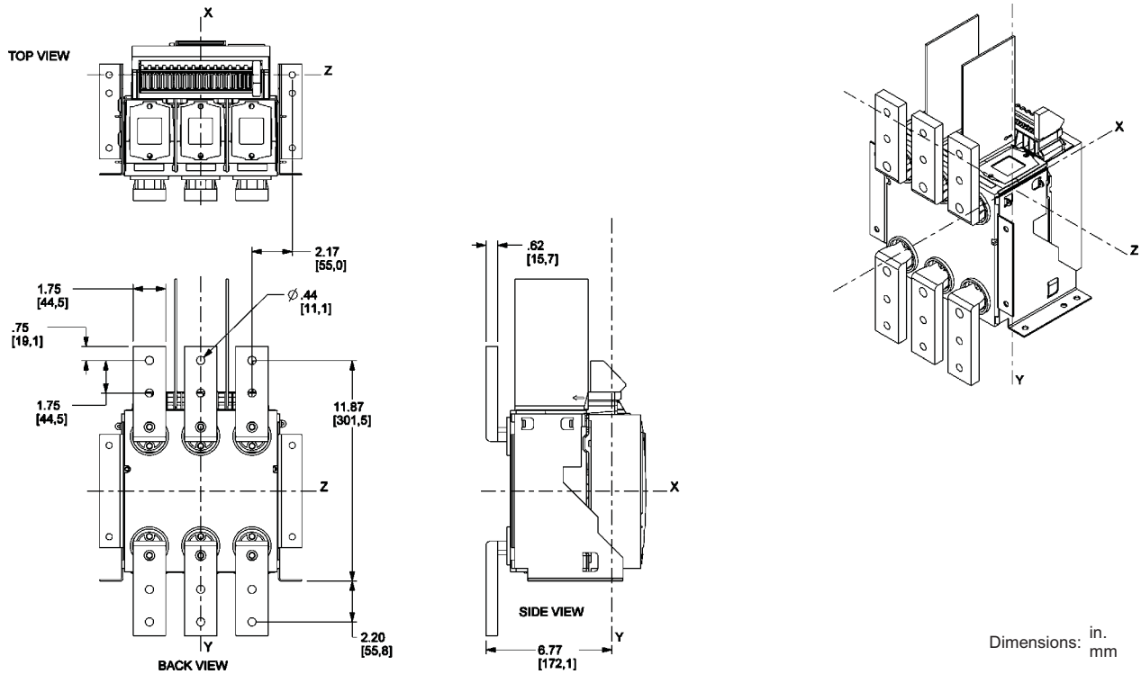
Figure 28: 800–1200 A Masterpack NT UL/ANSI 3P Fixed—FCF Front-Connected Flat
