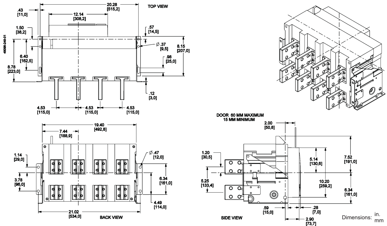
Figure 115: 800–2000 A Rear-Connected "T" Vertical (RCTV)
