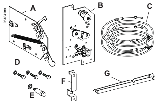
Figure 11: Cable Door Interlock Kit Contents
