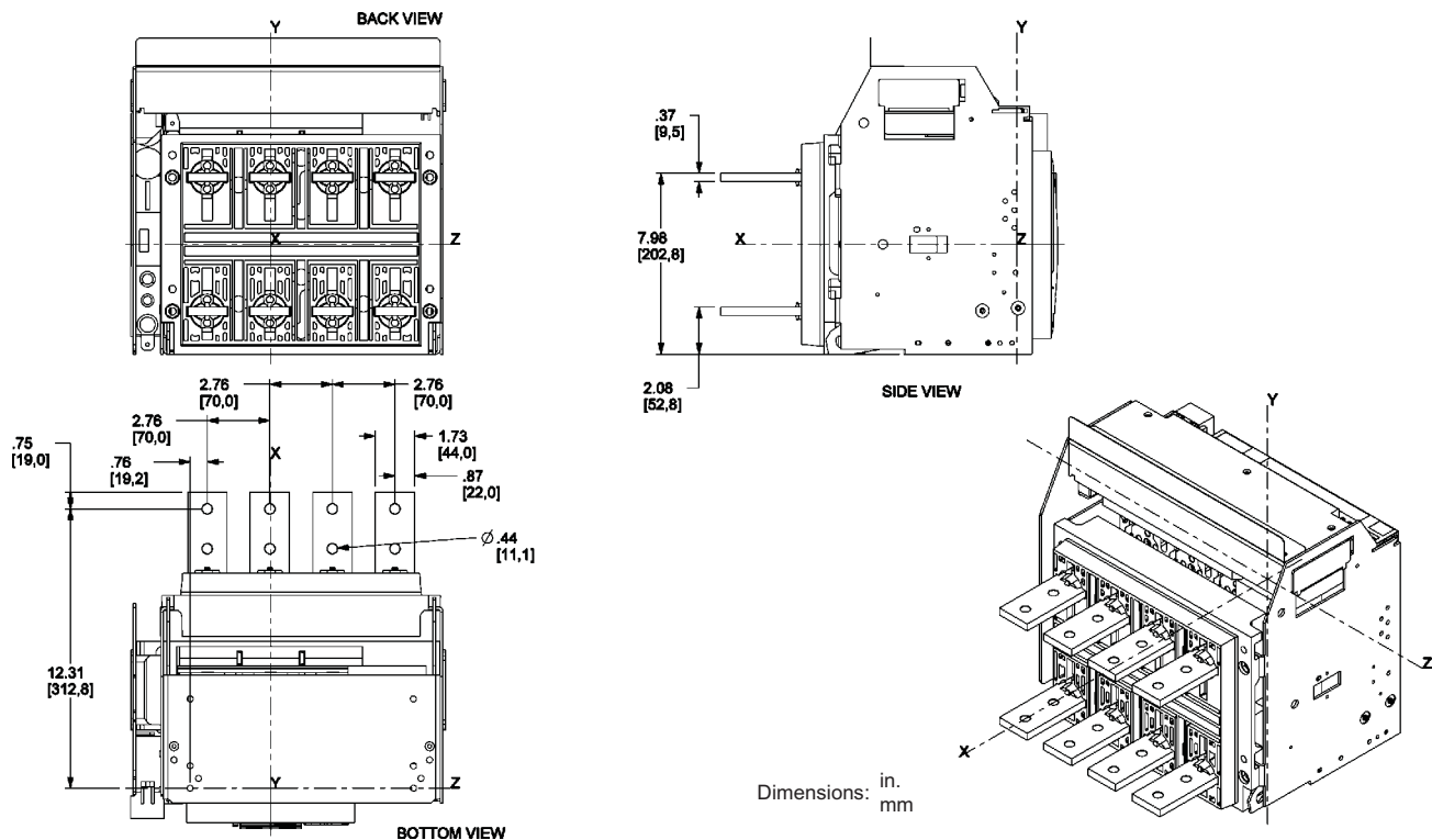
Figure 33: 800–1200 A Masterpact NT UL/ANSI 4P Drawout—RCTH Rear-Connected “T” Horizontal
