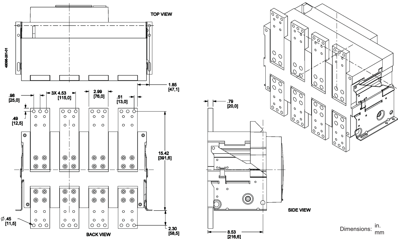
Figure 157: 800–3200 A Front-Connected Flat (FCF)
