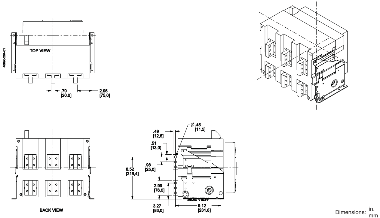
Figure 140: 800–3200 A Rear-Connected "T" Horizontal (RCTH)
