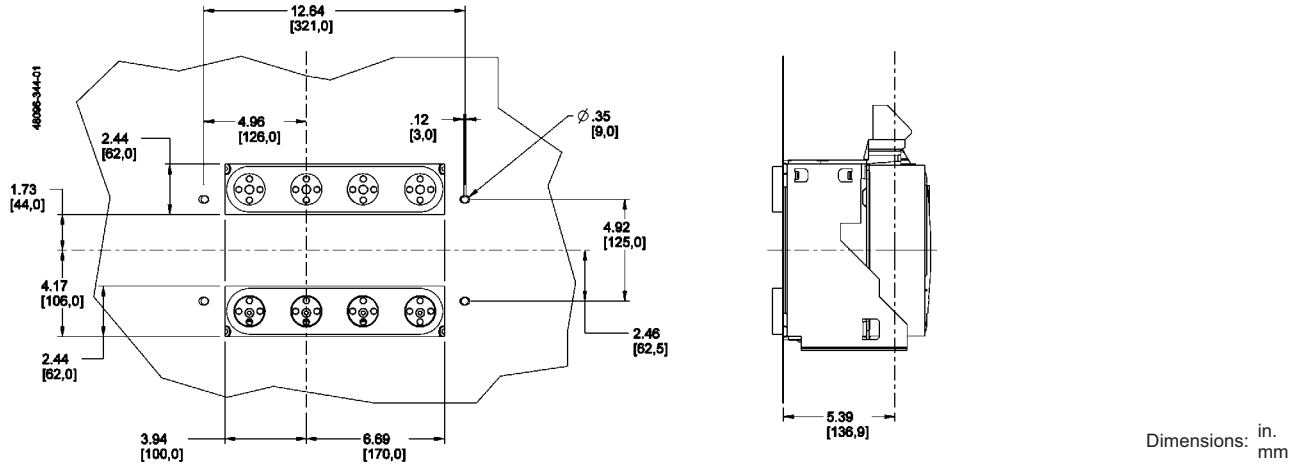
Figure 63: 800–1200 A Masterpack NT IEC 4P Fixed—Rear Cutout Dimensions
