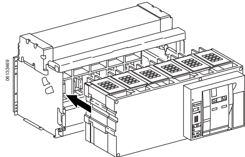
4000–6300 A Masterpack NW Drawout Circuit Breaker
