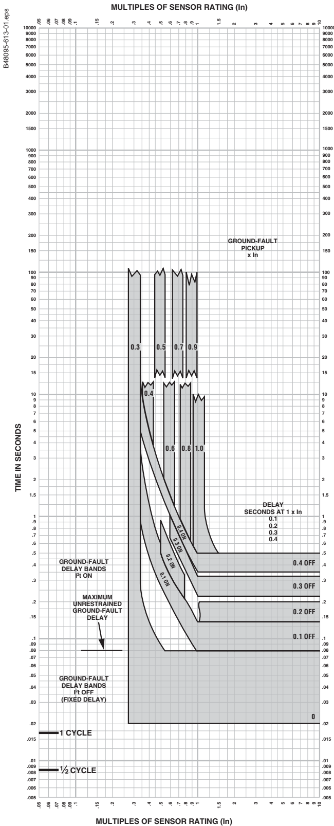
Figure 163: Micrologic 6.0 A/P/H Trip Units: I_n \leq 400 A
