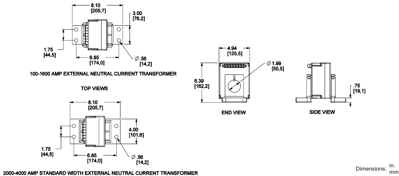
Figure 128: Neutral Current Transformer 2000–4000 A
