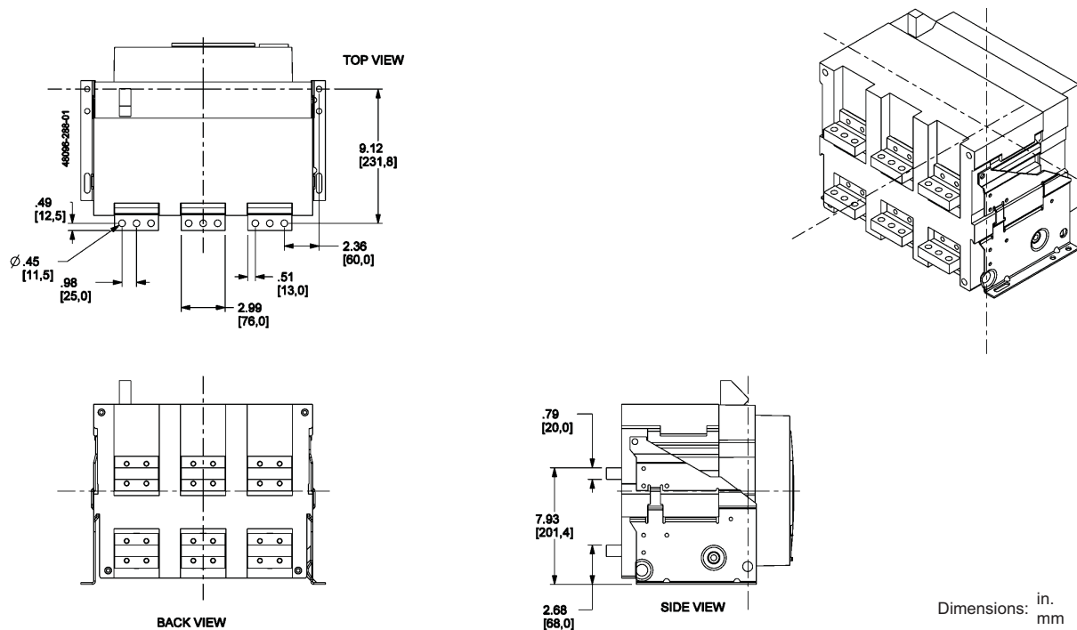
Figure 140: 800–3200 A Rear-Connected "T" Horizontal (RCTH)
