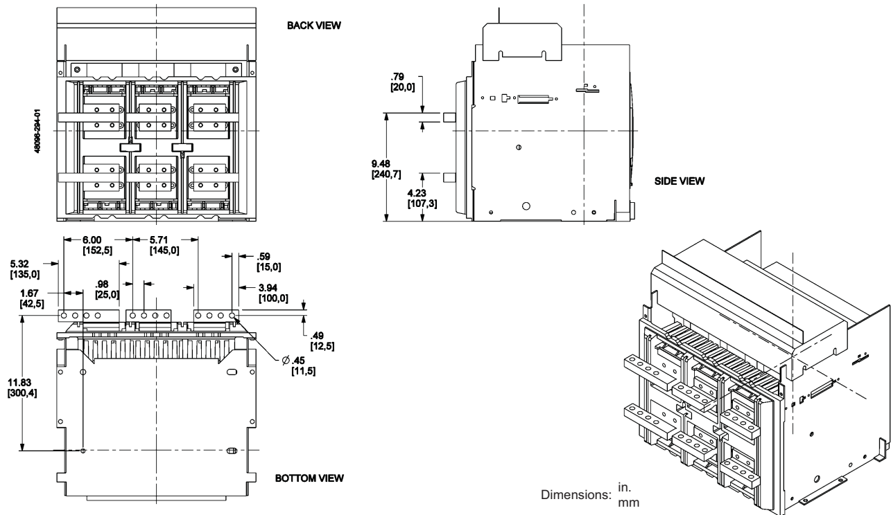
Figure 135: 4000 A Rear-Connected "T" Horizontal (RCTH)
