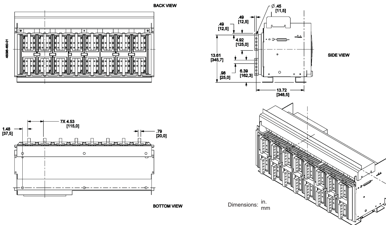
Figure 154: 6300 A Rear-Connected “T” Vertical (RCTV)
