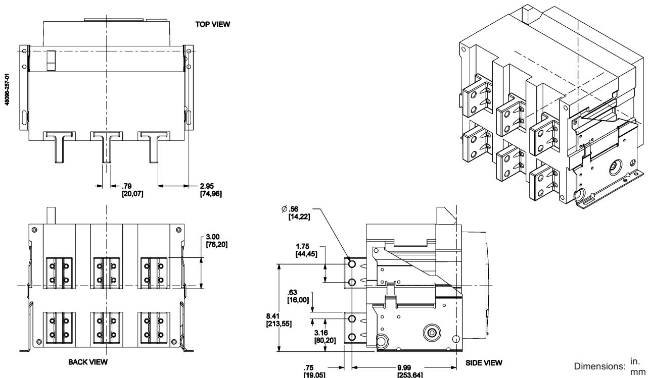
Figure 87: 800–2000 A Rear-Connected "T" Horizontal (RCTH)
