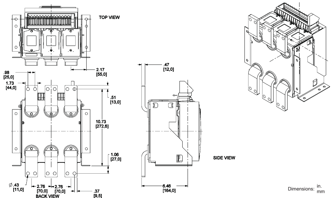
Figure 52: 800–1600 A Masterpack NT IEC 3P Fixed—FCF Front-Connected Flat
