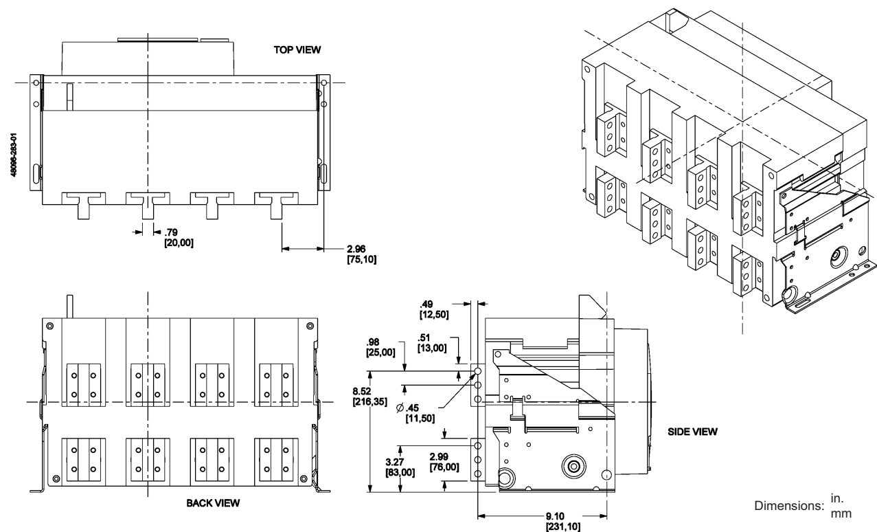
Figure 155: 800–3200 A Rear-Connected "T" Vertical (RCTV)
