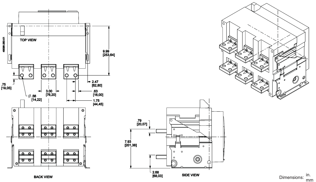
Figure 87: 800–2000 A Rear-Connected "T" Horizontal (RCTH)
