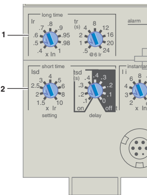
Micrologic 5.0 Basic Trip Unit
