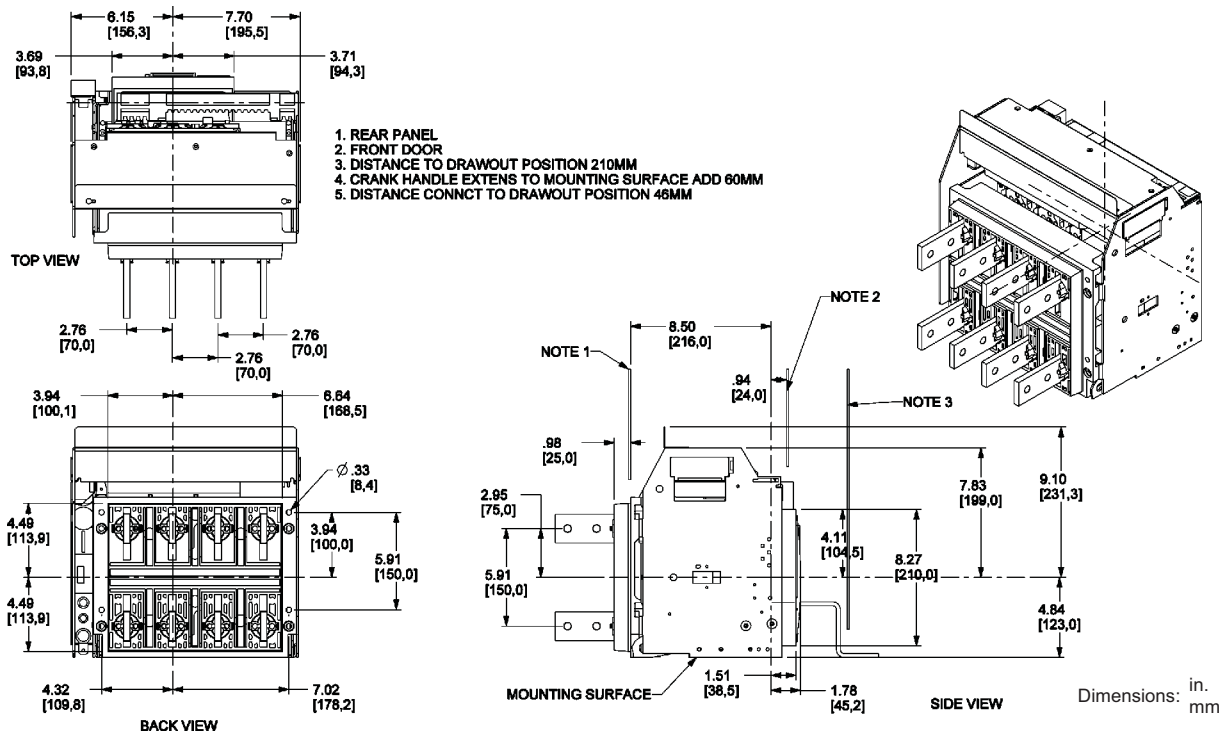
Figure 33: 800–1200 A Masterpact NT UL/ANSI 4P Drawout—RCTH Rear-Connected “T” Horizontal
