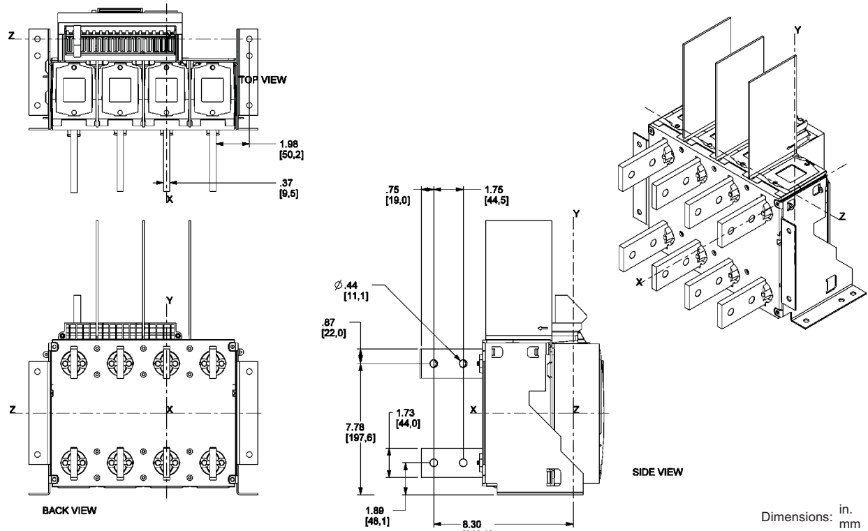
Figure 41: 800–1200 A Masterpack NT UL/ANSI 4P Fixed—FCF Front-Connected Flat
