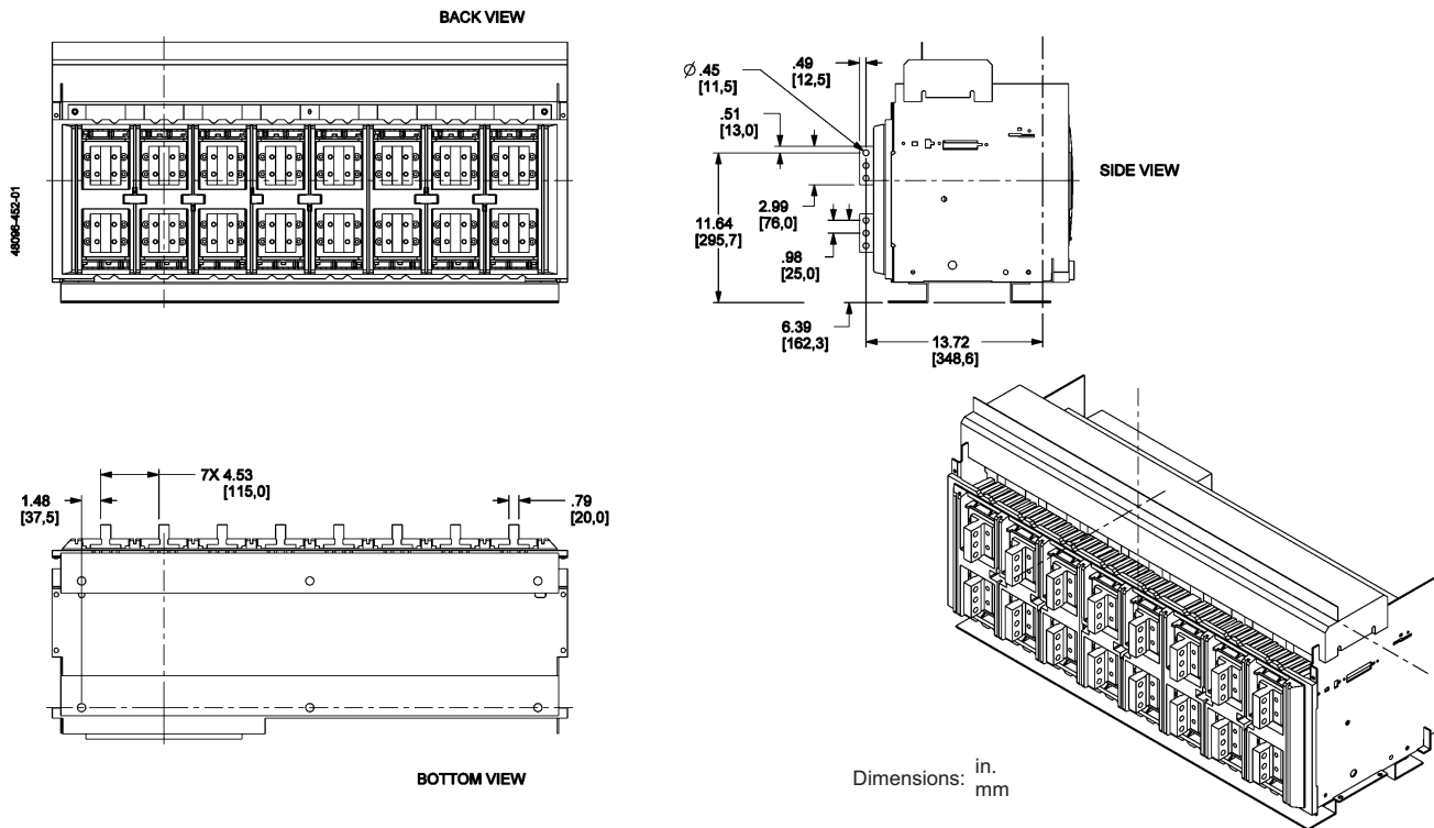
Figure 153: 5000 A Rear-Connected “T” Horizontal (RCTH)
