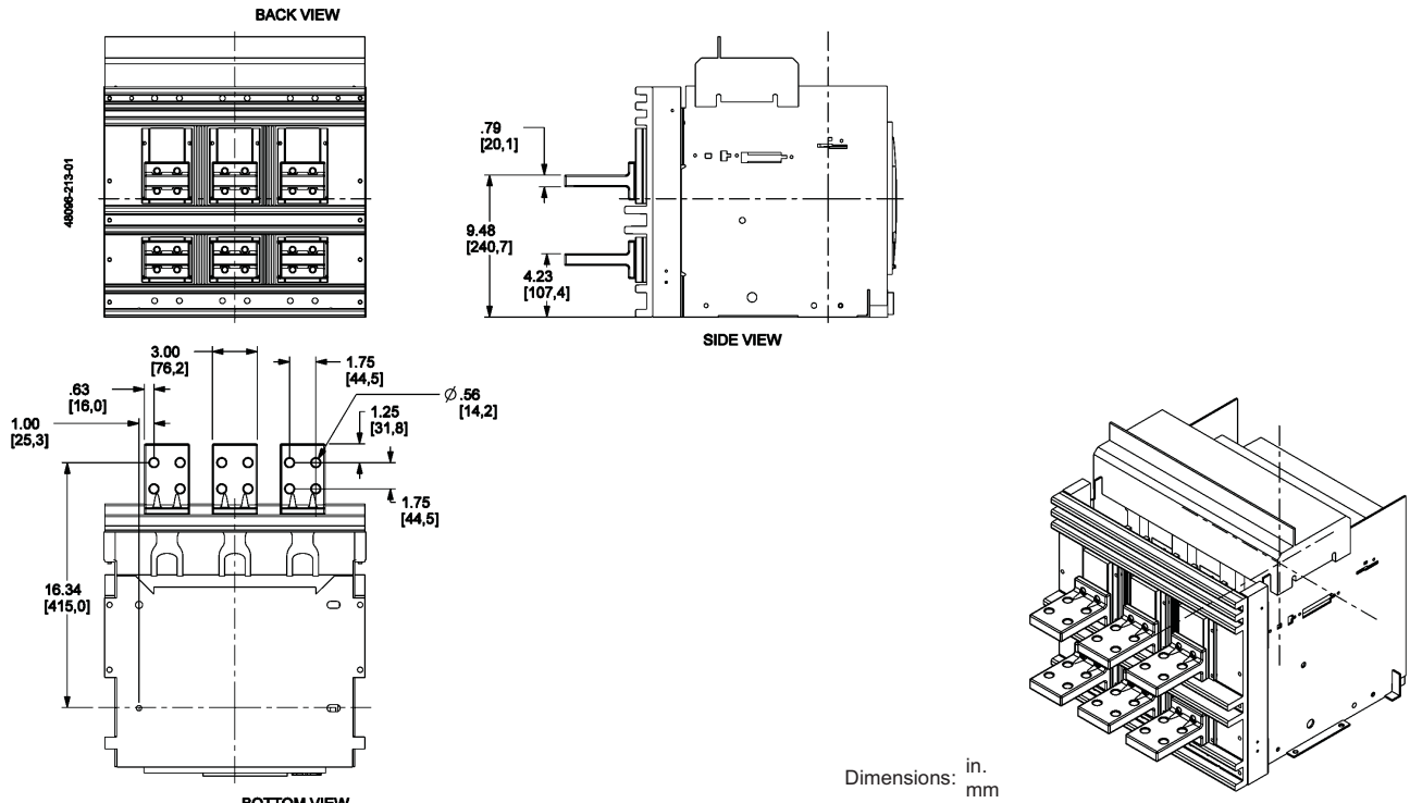
Figure 72: 2500–3000 A Rear-Connected "T" Horizontal (RCTH)
