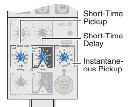
Short-Time and Instantaneous Trip Functions
