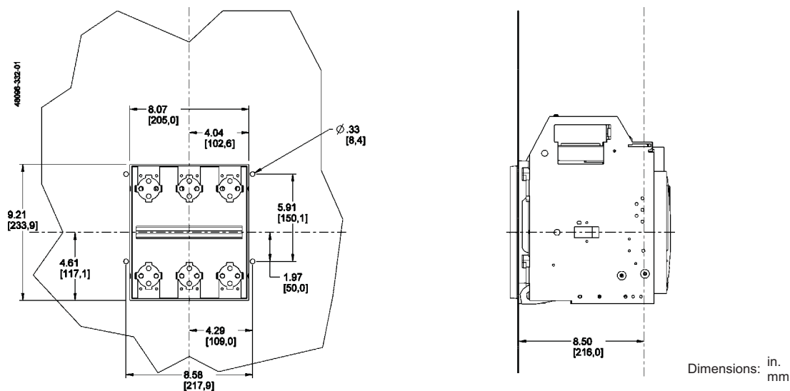
Figure 48: 800–1200 A Masterpact NT IEC 3P Drawout—Rear Cutout Dimensions
