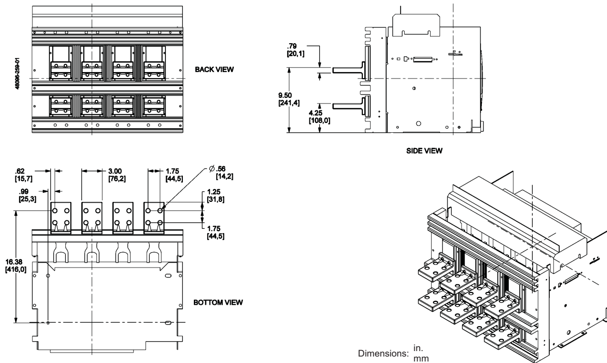
Figure 106: 2500–3000 A Rear-Connected "T" Horizontal (RCTH)
