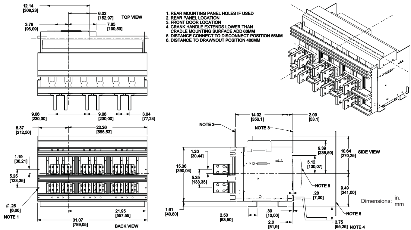
Figure 75: 3200 A L1 and 4000–6000 A Master Drawing
