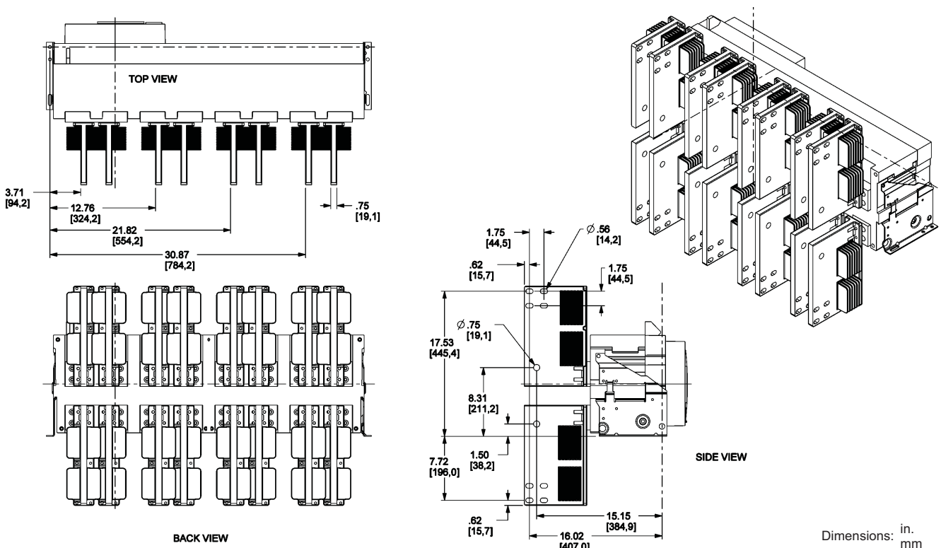
Figure 125: 6000 A Rear-Connected "T" Vertical (RCTV)
