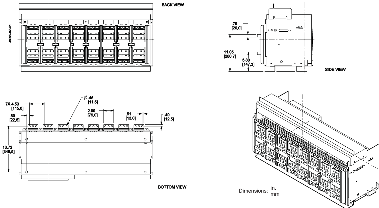
Figure 153: 5000 A Rear-Connected “T” Horizontal (RCTH)
