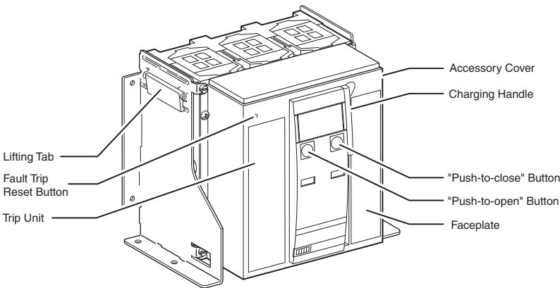
Fixed Circuit Breaker
