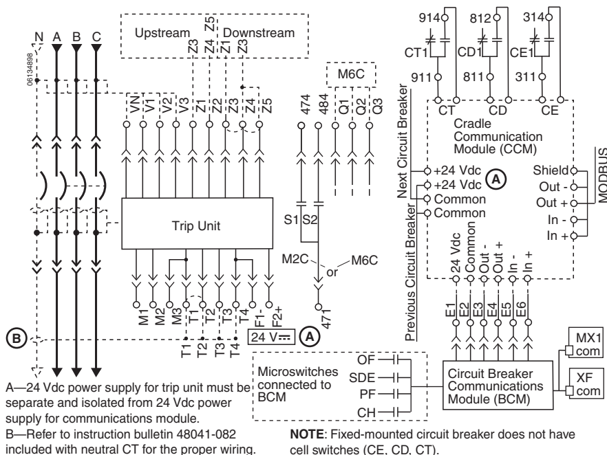
Figure 18: Connection of the Communications Option
