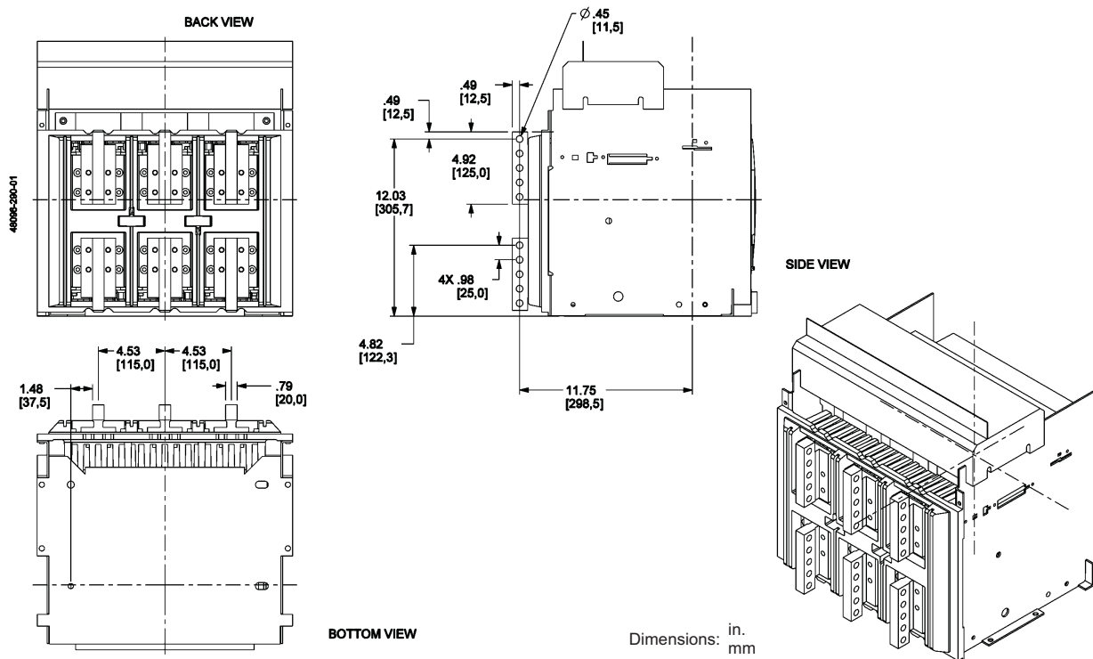
Figure 135: 4000 A Rear-Connected "T" Horizontal (RCTH)
