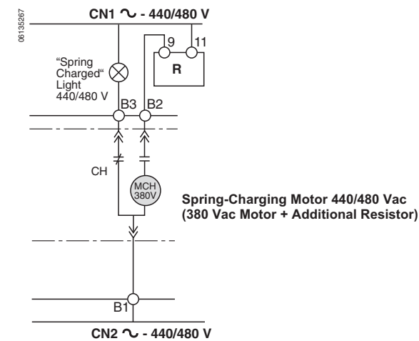
Figure 17: Spring-Charging Motor
