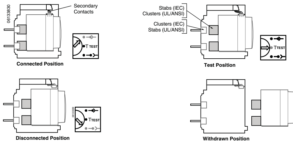
Figure 3: Racking Positions
