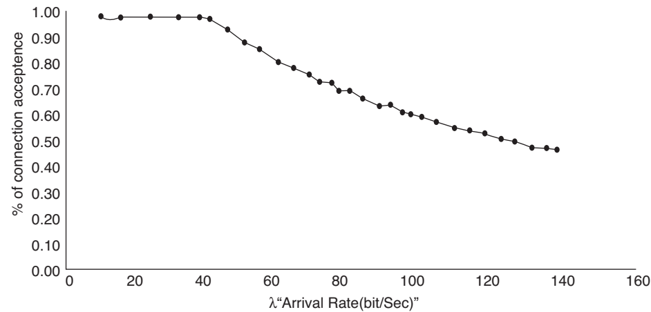
Figure 18.10 Acceptance ratio for UGS class using interactive_CAC.
