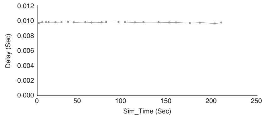
Figure 18.11 UGS delay (sec.).
