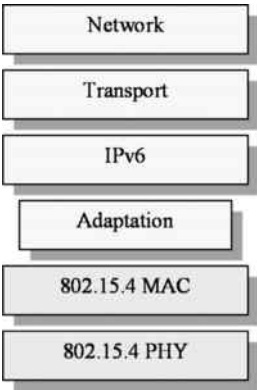
Figure 9.3 Protocol stack of 6LoWPAN.
