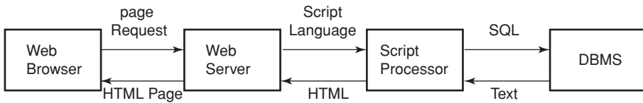
Figure 1.4 Client-server requests.
