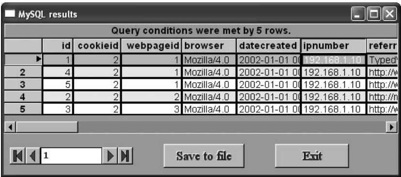
Figure 5.7 The Log table populated by LOAD DATA.
