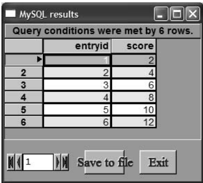
Figure 8.10 UPDATE calculating values for each row.
