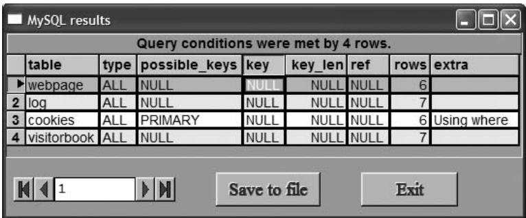
Figure 13.6 EXPLAIN on a restricted cross join.
