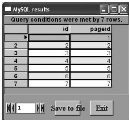
Figure 6.10 Selecting the same column twice with an alias.
