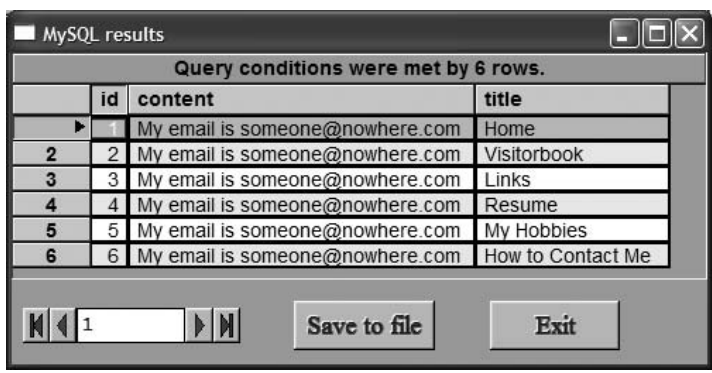
Figure 8.3 The damage caused by omitting the WHERE.
