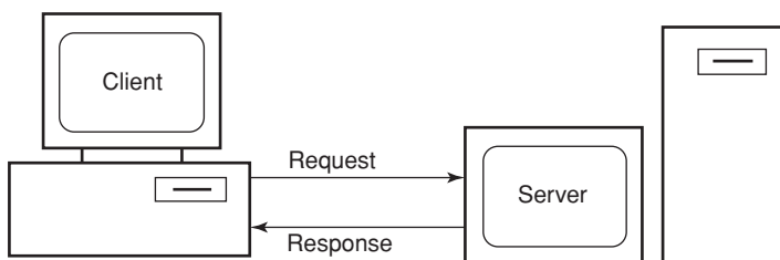
Figure 1.3 Client-server system.
