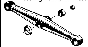
Removing center bushing with No. 1744 set.
