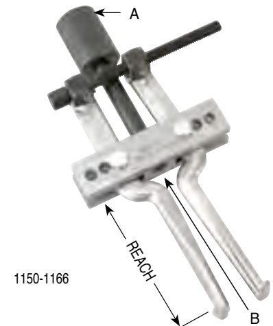
A = Thread of tapped hole in adapter. B = Distance between adjusting screws.
