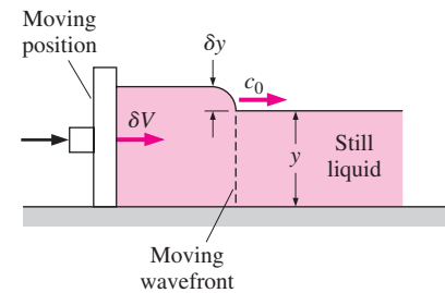
(a) Generation and propagation of a wave
