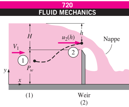
FIGURE 13–43 Flow over a sharp-crested weir.
