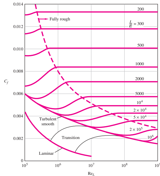
FIGURE 11-31 Friction coefficient for parallel flow over smooth and rough flat plates.
