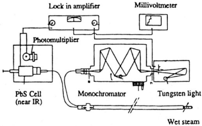
Fig. 2-31. Optical attenuation probe for measuring fog droplet size Source: A. R. Laali, J. J. Courant, and A. Kleitz 63
