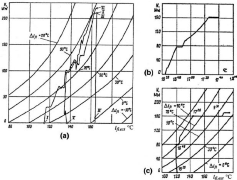
Fig. 4-71. Two-coordinate loading diagram for Turboatom's K-220-44 turbine and its application to start-ups at the Kola nuclear plant (a: daily loading diagram with two start-ups [I: 3:40 A.M.—generator is switched on to grid after two-day outage; II: 5:30 A.M.—turbine reaches the final load of 210 MW; III: 11:40 A.M.—turbine unloading begins; IV: 12:00 P.M.—generator is switched off; V: 9:07 P.M.—generator is repeatedly switched on to the grid; VI: 10:45 P.M.—turbine reaches the final load of 220 MW]; b: loading diagram of automated start-up after two-day outage; c: N - t diagram of the same automated start-up after two-day outage)
