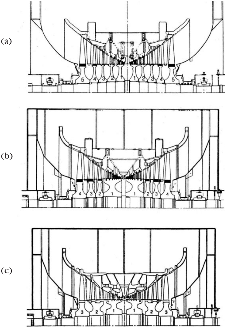
Fig. 5-8. Improvements of the LP cylinder design for Siemens' low-speed wet-steam turbines (from a ten-disk rotor to a six-disk rotor) Source: By courtesy of Siemens
