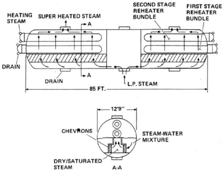
Fig. 3-77. Principle schematic of Westinghouse's third-generation MSR
