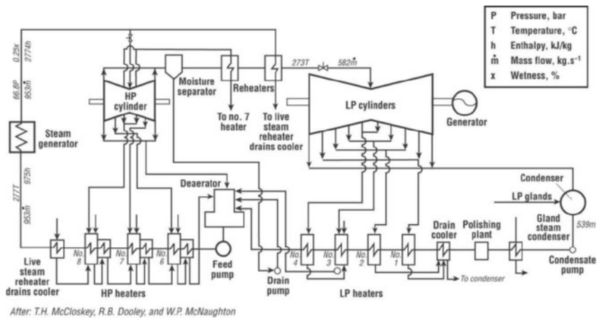
Fig. 2-1. Schematic diagram of a large double-circuit nuclear power unit turboset with operating conditions corresponding to 100% MCR
