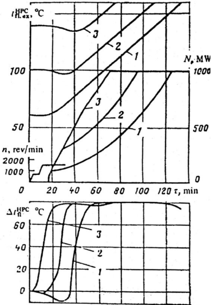
Fig. 4-65. Optimized calculated schedules of hot (1), warm (2), and cold (3) start-ups for Turboatom's K-1000-60/1500 turbine ( t_{fl,ex}^{HPC} : metal temperature on the external HP flange surface; \Delta t_{fl}^{HPC} : temperature difference along the flange width in the HP steam admission zone)
