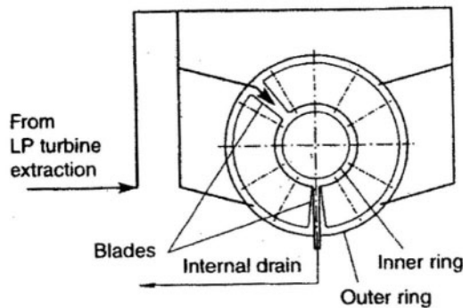
Fig. 3–74. Heating hollow nozzle vanes for the last stages of Siemens' turbines
