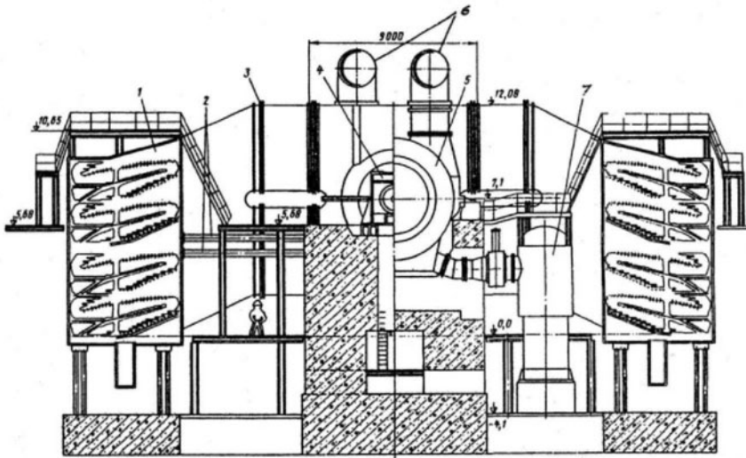
Fig. 3-17. Rear-view and cross-section of the LP cylinder for Turboatom's 500- and 1,000-MW 1,500-rpm wet-steam turbines with side condensers (1: condenser; 2: flexible joint; 3: sylphon; 4: bearing casing; 5: LP cylinder's casing; 6: crossover pipes; 7: LP regenerative heater)
