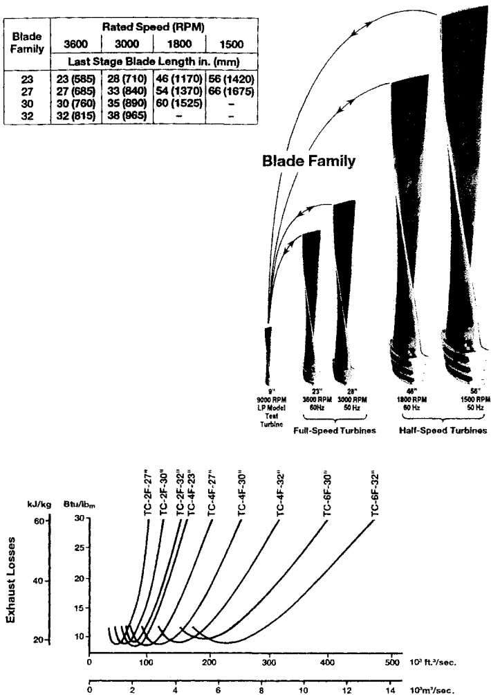
Fig. 3-46. Families of Siemens LSBs and selection diagram for 3,600-rpm turbines
