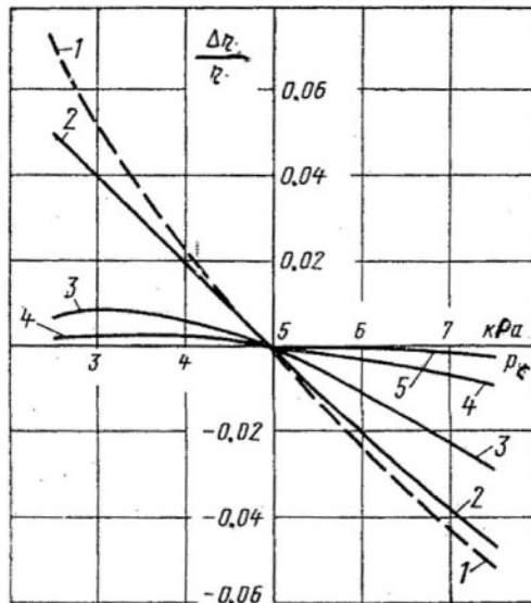
Fig. 2-4. Influence of the end steam pressure in the condenser, p_c , on wet-steam turbine thermal efficiency (initial steam pressure, p_0 = 7 MPa [1,015 psi]; 1: invariable outlet steam velocity, G_c \times v_c / F ; 2, 3, 4, and 5: N/F = 5, 10, 15 and 20 MW/m 2 , respectively)
