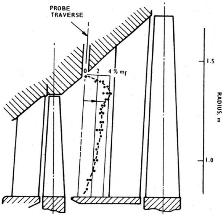
Fig. 2-28. Typical distribution of coarse-grain water before the last LP stage of a 500-MW turbine
