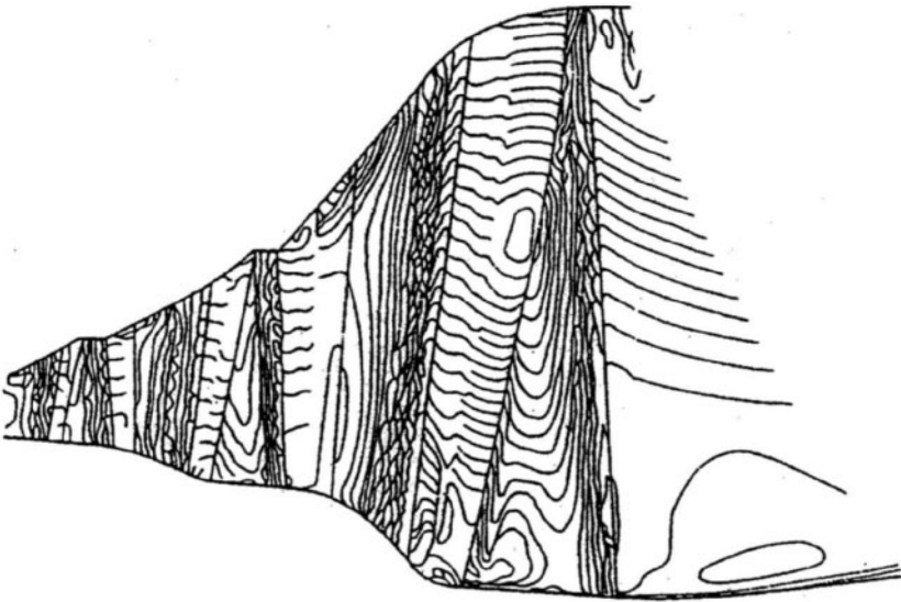
Fig. 3-57. Calculated isotach field for the steam path of three last LP stages with 1,143-mm titanium LSB of MHI's 3,600-rpm turbine
