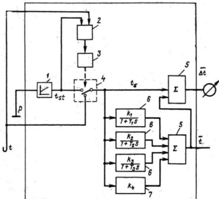
Fig. 4-72. Functional chart of a device for temperature monitoring of the HP rotor for wet-steam turbines (1: nonlinear transducer; 2: logic element; 3: switchboard; 4: switch; 5: summators; 6: aperiodic elements; 7: amplifier)
