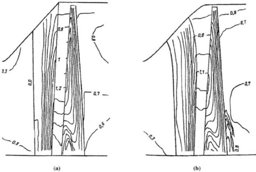
Fig. 3-59. Isotach fields for the last LP stages of LMZ's newly designed and refurbished turbines with conventional (a) and saber-type (b) vanes
