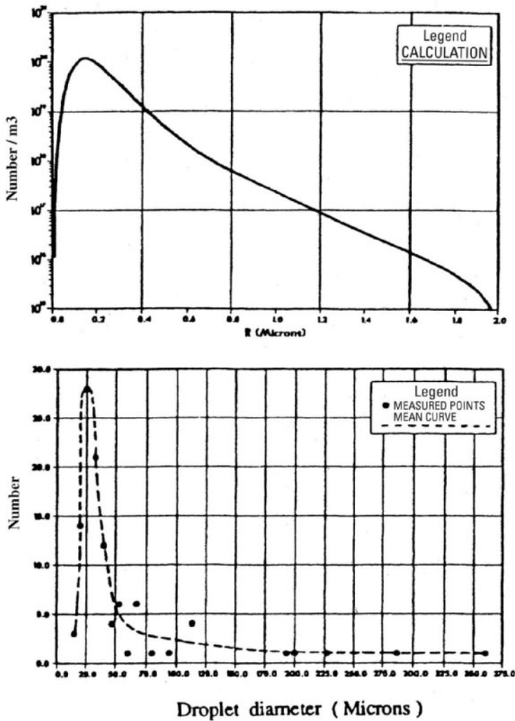
Fig. 2-33. Experimental distributions of fog droplets and large drops downstream of the LSB Source: A. R. Laali, J. J. Courant, and A. Kleitz 65
