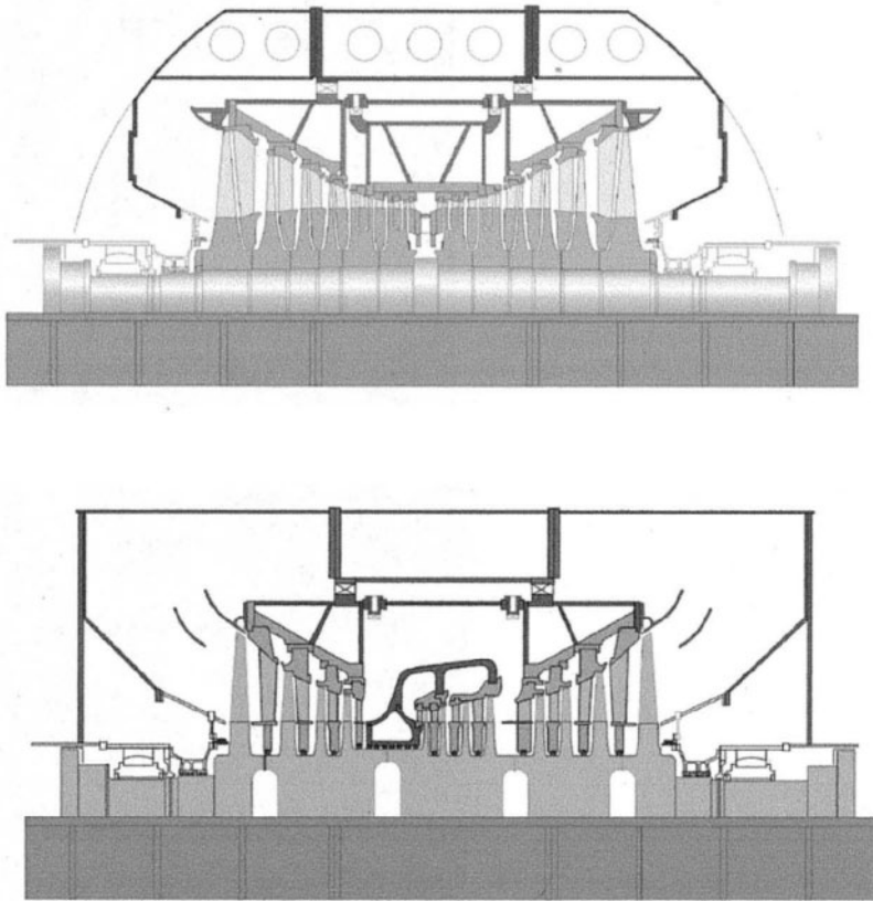
Fig. 5-12. Original design of disk-type LP rotors of SONGS' 1,127-MW turbines (a) and their retrofitted optiflow configuration design (b)
