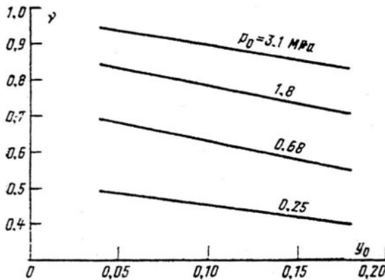
Fig. 2-16. Influence of initial steam pressure, p_0 , and wetness, \gamma_0 , on the slide factor for a supersonic nozzle
