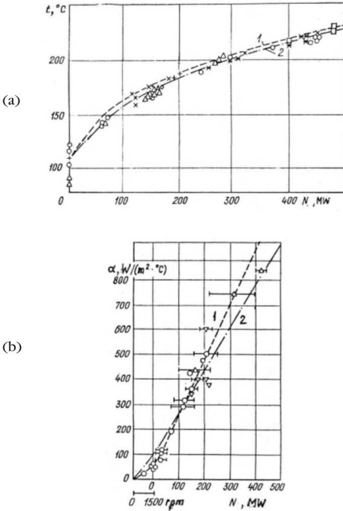
Fig. 4-47. Static dependencies on turbine load for heating steam temperature in the first steam extraction chamber (a) and heat transfer conditions in the IP steam admission chamber (b) of the HP-IP cylinder of a K-500-50/1500 turbine based on start-up tests at the Novovoronezh nuclear power plant (1: approximate generalization of calculated procession of experimental data; 2: approximate generalization of preliminary calculated data)
