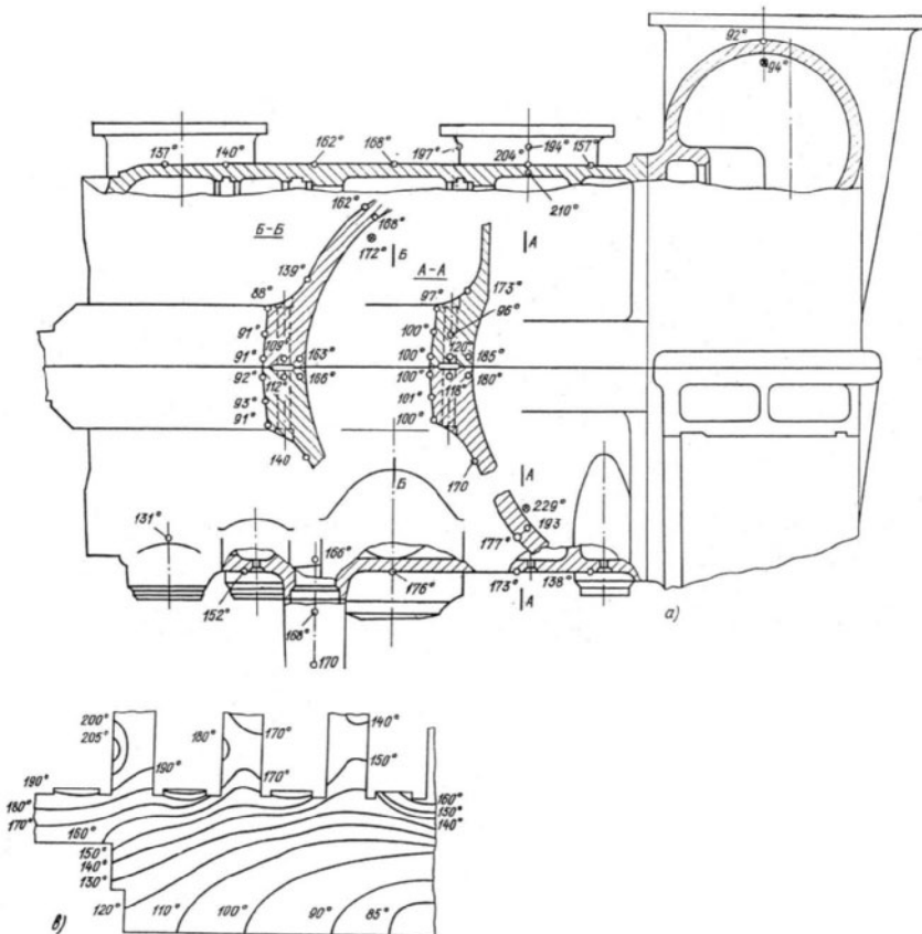
Fig. 4–8. Measured temperature distribution ( ^{\circ}\text{C} ) in outer casing (a) and calculated temperature field in rotor in the first IP stages zone (b) for the integrated HP–IP cylinder of Turboatom’s K-500-60/1500 turbine for a typical start-up instant
