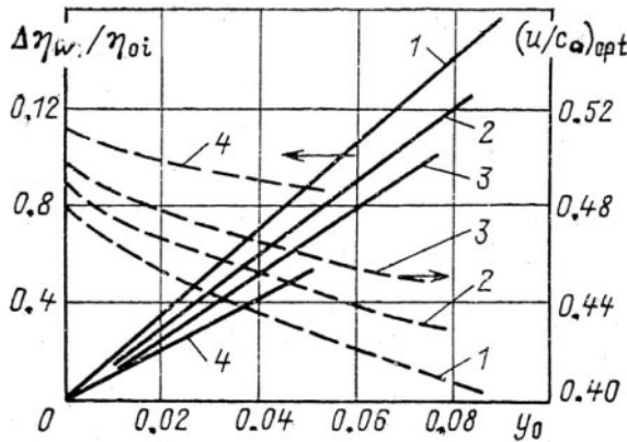
Fig. 2-19. Changes in optimal velocity ratio and internal stage efficiency for turbine stages with different median-diameter-to-height ratios, depending on initial wetness (1: d/l_1 = 27 , l_1 = 15 mm; 2: d/l_1 = 16 , l_1 = 25 mm; 3: d/l_1 = 8 , l_1 = 48 mm; 4: d/l_1 = 2.7 , l_1 = 207 mm)
