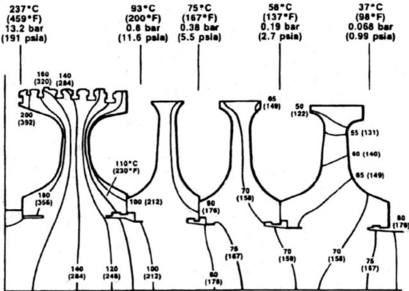
Fig. 4-61. Calculated temperature field for a combined LP rotor (right half) Source: H. Oeynhausen, G. Roettger, J. Ewald, et al. 160
