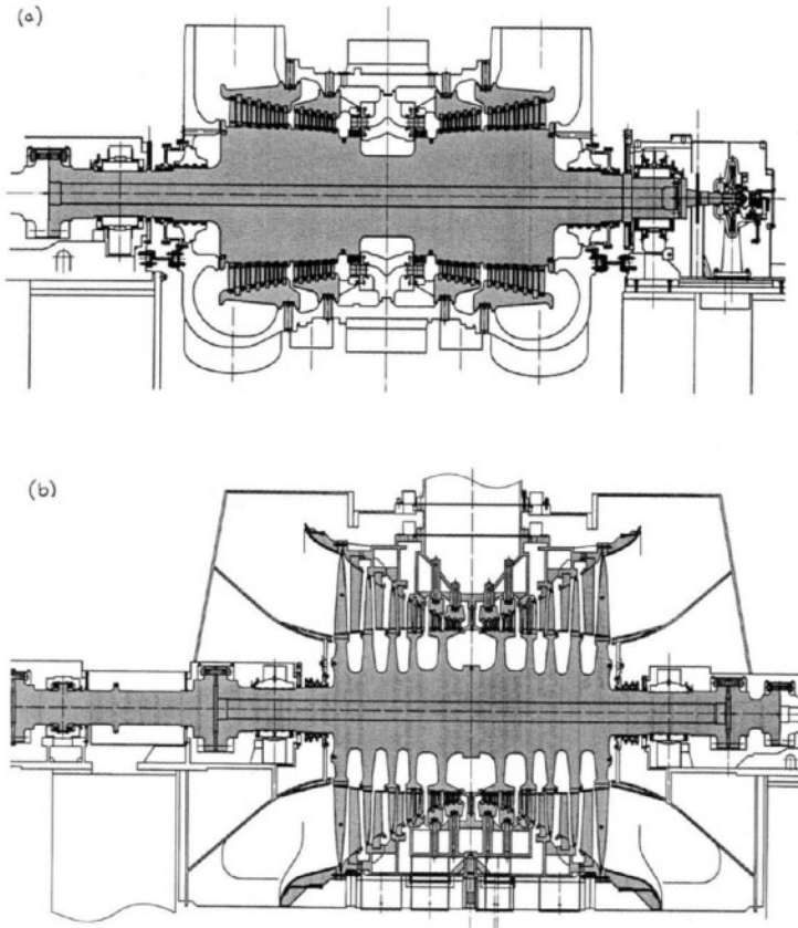
Fig. 5-11. Refurbished HP (a) and LP (b) cylinders of the 1,000-MW-class wet-steam turbine at Vandellós Unit 2 (replaced components are shaded) Source: By courtesy of Mitsubishi Heavy Industries
