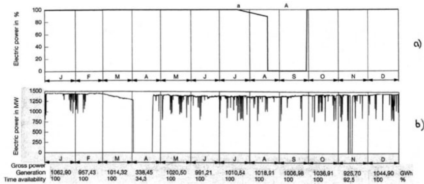
Fig. 4-2. Operation diagrams for German nuclear power units Neckar 2 (a) and Grohnde (b) in 2002 (a: stretch out, unloading before refueling A)
