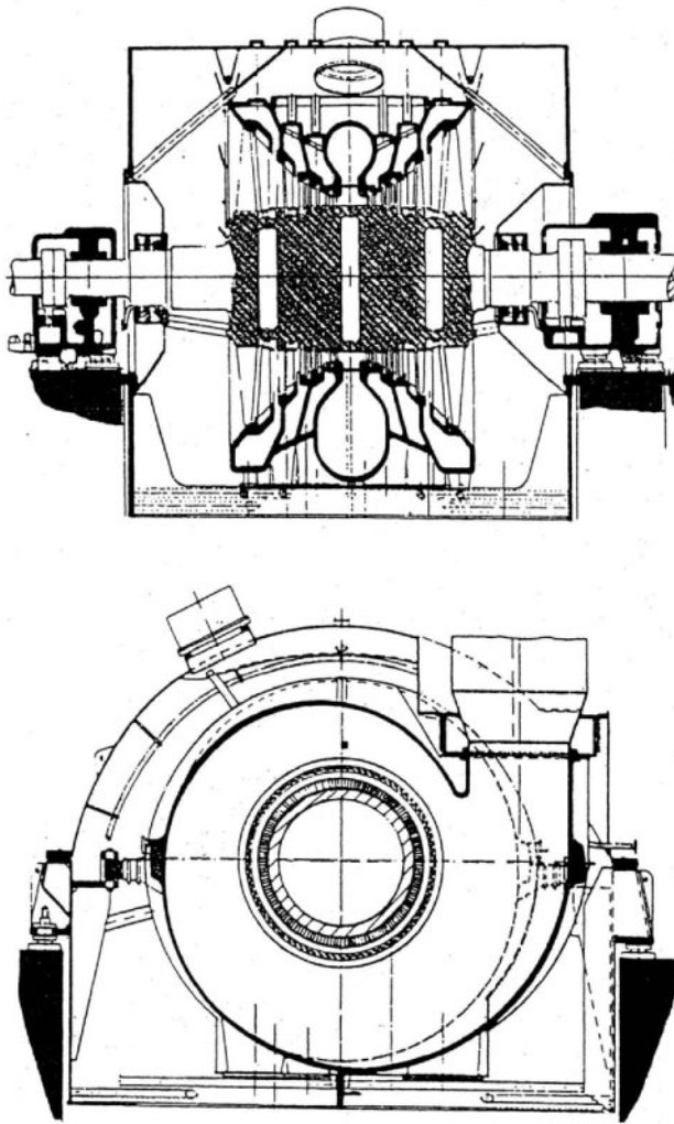
Fig. 5-5. Longitudinal and cross sections of ABB's LP cylinder with a scroll-type steam inlet
