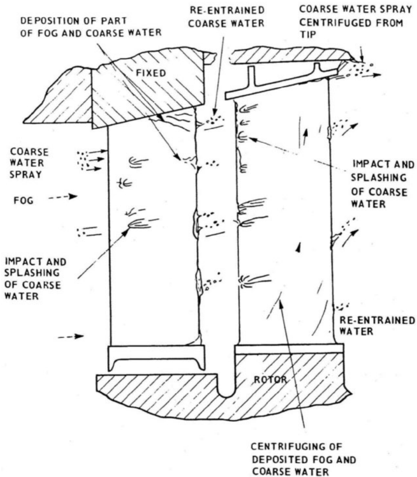
Fig. 2-8. Various forms of water existing in a wet-steam turbine stage
