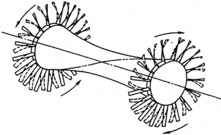
Fig. 4-40. Phenomenon of shaft-blade coupled torsional oscillations
