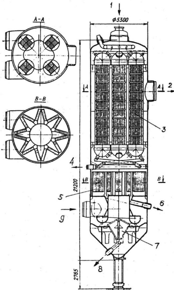
Fig. 3-81. One of two vertical MSRs for Siemens' 1,300-MW wet-steam turbines (1: working steam inlet; 2: superheated steam outlet; 3: steam reheater; 4: heated steam condensate outlet from steam reheater; 5: separator's modules; 6: separated water outlet; 7: preseparator; 8: drain; 9: working steam inlet)
