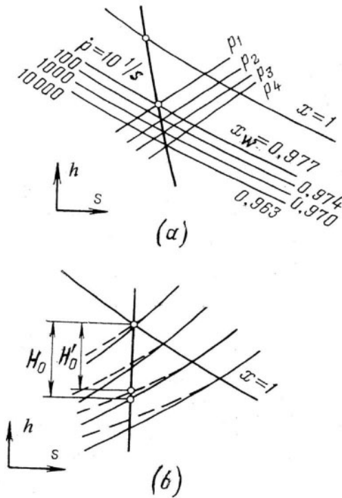
Fig. 2-10. Steam expansion process with subcooling shown on h - s axes (a: Wilson lines x_w = \text{const} depending on p , isobars in the wet-steam region for subcooled steam)
