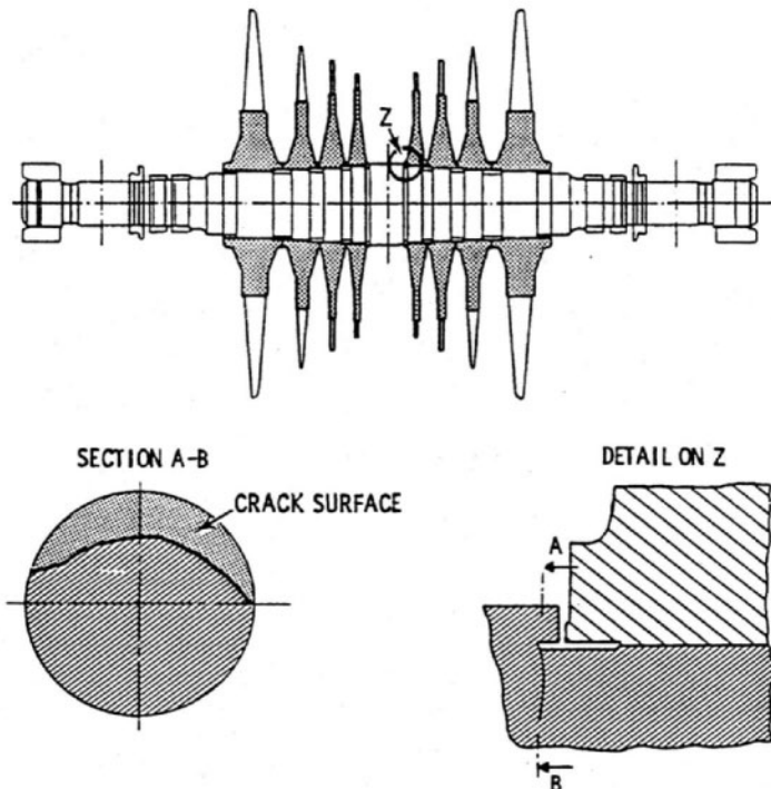
Fig. 4-24. Crack damage on the LP-1 rotor of AEG's 660-MW wet-steam turbine at Würgassen
