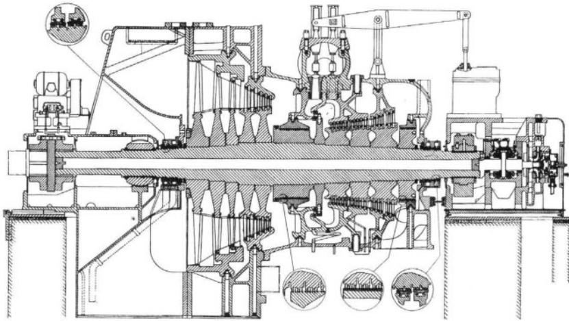
Fig. 1-1. Westinghouse nuclear wet-steam turbine (100-MW, 1,800 rpm) used at Shippingport Station, 1957
