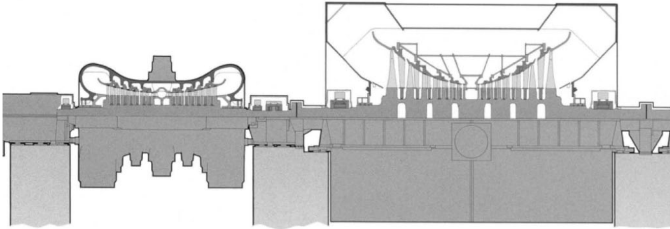
Fig. 3-2 Longitudinal section of the HP cylinder and one of three LP cylinders of ALSTOM's 1,200-to-1,500-MW 1,800-rpm wet-steam turbine Source: By courtesy of ALSTOM
