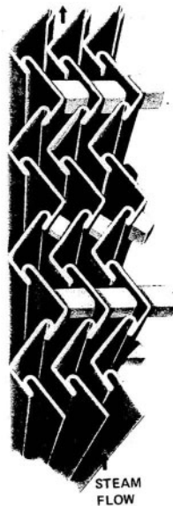
Fig. 3-78. Part of a chevron-plate separator
