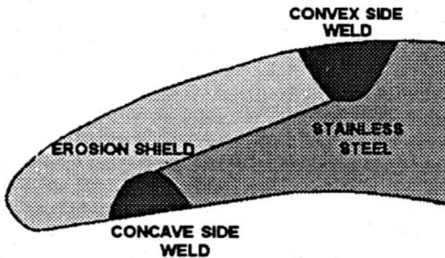
Fig. 4-39. Shielding the leading edge of a steel last stage blade from WDE
