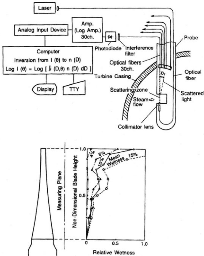
Fig. 2-37. Schematic diagram of steam wetness measurement system (a); wetness distribution over the stage height at a model turbine outlet (b) Source: T. Sakamoto, S. Nagao, and T. Tanuma 71
