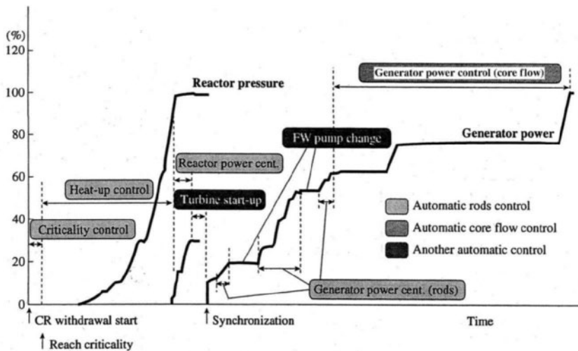
Fig. 4-5. Cold start-up of 1,356-MW Kashiwazaki-Kariwa Unit 7 with ABWR
