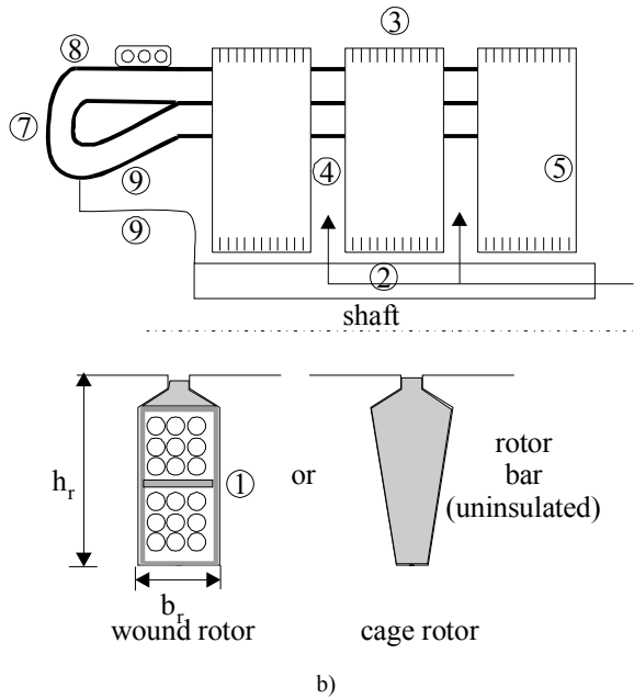
Figure 12.9 (continued): b) rotor winding
