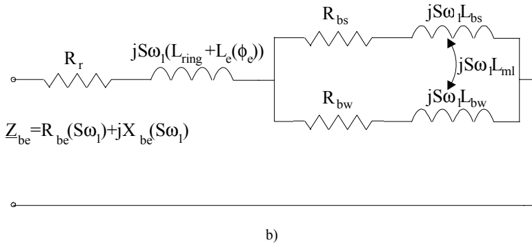
Figure 9.18 (continued): equivalent circuit b)
