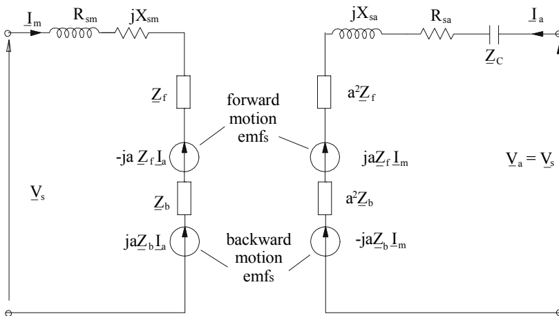
Figure 24.22 The revolving theory equivalent circuit of the capacitor motor
