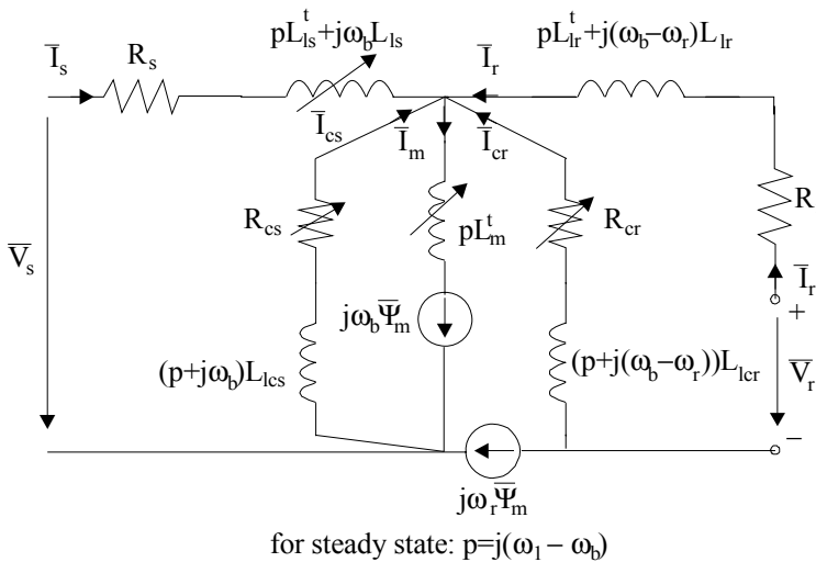
Figure 13.14 Space phasor T equivalent circuit with saturation and rotor core loss (or rotor skin effect)
