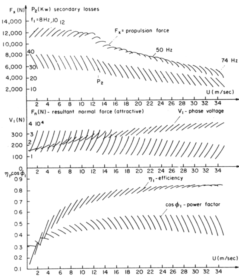
Figure 20.31 Motoring performance
