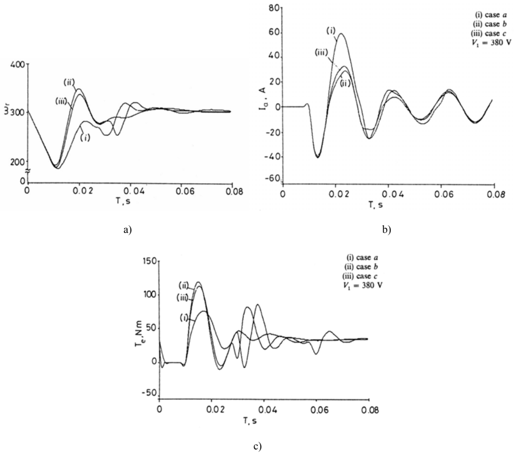
Figure 13.18 Disconnection–reconnection transients at high voltage: V_{\text{phase}} = 380\text{V} (RMS)
