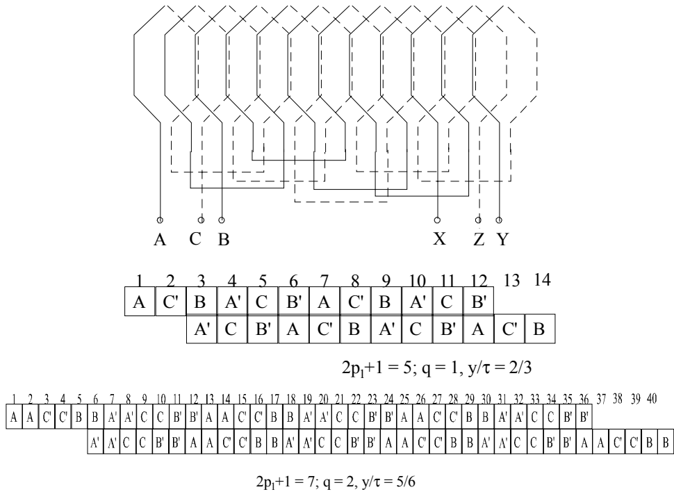
Figure 20.8 Double-layer chorded coil windings with 2p_1 + 1 poles
