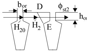
Figure 9.31 Rotor slot neck flux \Phi_{st2}
