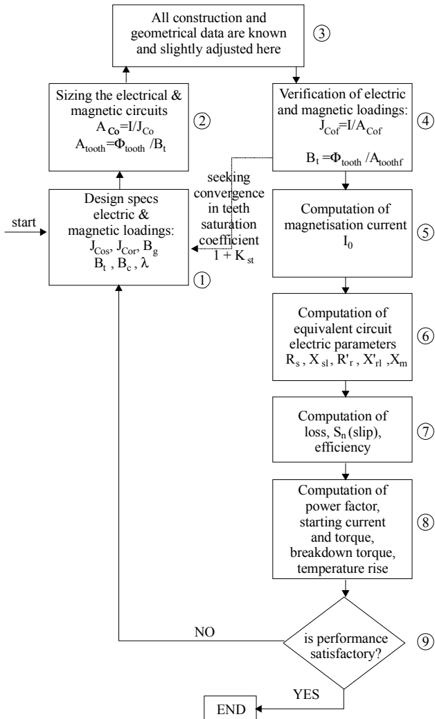
Figure 15.2 The design algorithm
