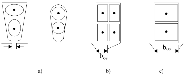
Figure 2.3 Slot geometrics to locate coil windings: a) semiclosed, b) semiopen, c) open
