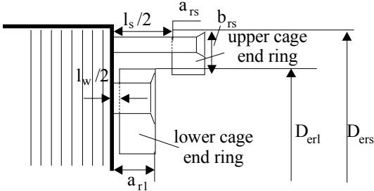
Figure 16.11 Separate end rings
