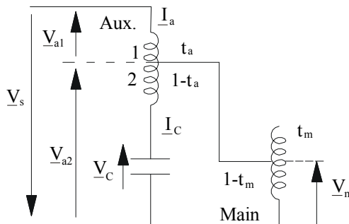
Figure 24.19 Doubly tapped winding capacitor IM
