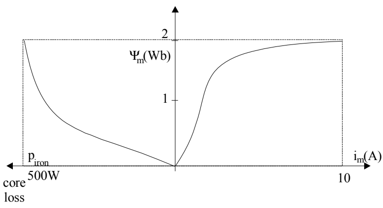
Figure 13.15 Magnetization curve and stator core loss
