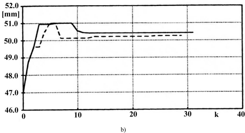
Figure 27.8 Evolution of the optimization process: a) Efficiency and material costs: F_1 and F_2 , b) Stack length for F_1 and F_2 .
