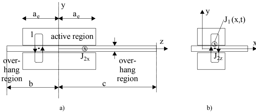
Figure 20.11 Transverse cross section of a double-sided LIM a), and longitudinal view b)
