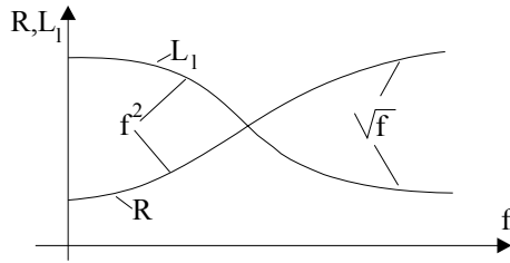
Figure 11.8 R and L_l variation with frequency
