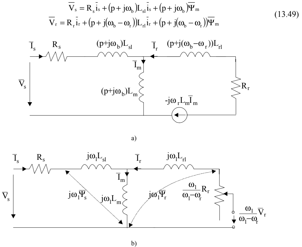
Figure 13.3 The general equivalent circuit a) and for steady-state b)
