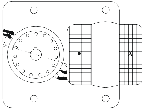
Figure 23.12 Two-pole C-shape shaded-pole induction motor
