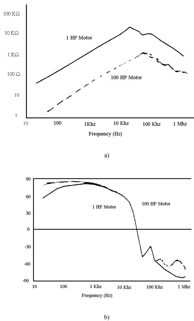
Figure 21.5 Differential impedance Z_m versus frequency: a) amplitude, b) phase angle
