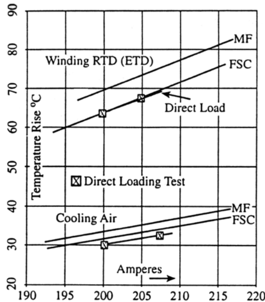
Figure 22.15 Steady-state temperature rises with three tests
