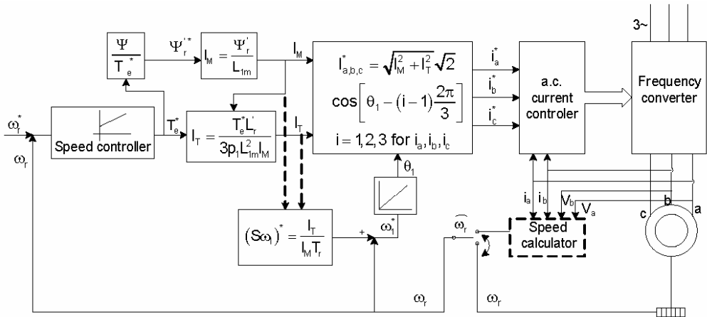
Figure 8.17 Basic rotor flux vector control system
