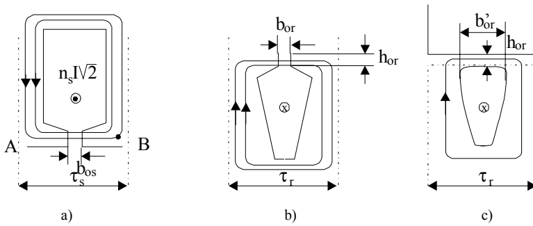
Figure 6.14 Slot neck leakage flux:
