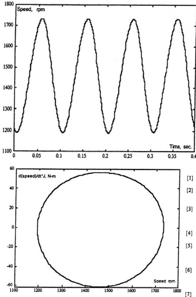
Figure 22.11 Speed oscillation and instantaneous active power variation ( P_n = 7.5 \text{ kW} )
