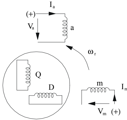
Figure 23.18 The d-q model of single-phase IM
