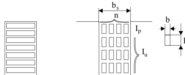
Figure 9.6 Multiple conductors in rectangular slots
