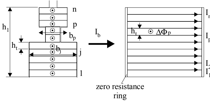
Figure 9.12 More general shape rotor bars
