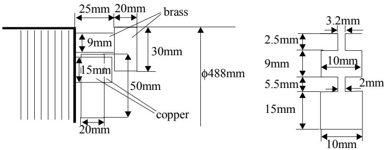
Figure 16.13 Double cage design geometry
