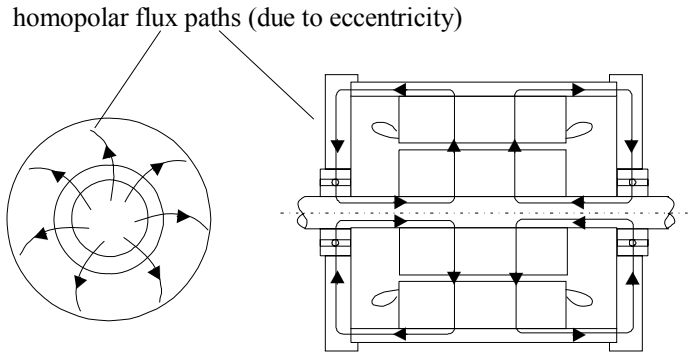
Figure 10.3 Homopolar flux due to rotor eccentricity
