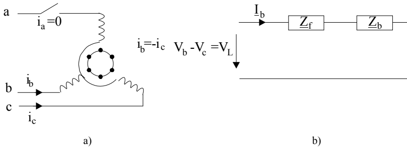
Figure 7.30 One stator phase is open:
