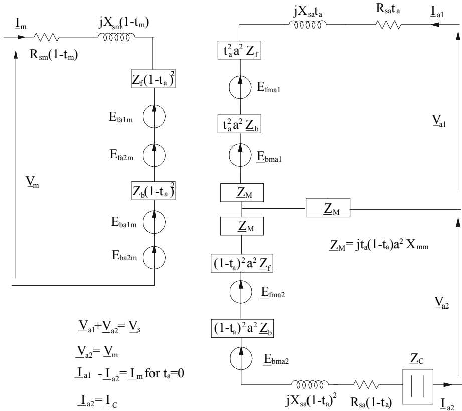
Figure 24.21 The equivalent circuit of dualy tapped winding capacitor induction motor
