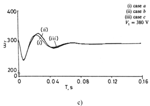
Figure 13.18 (continued): c) speed
