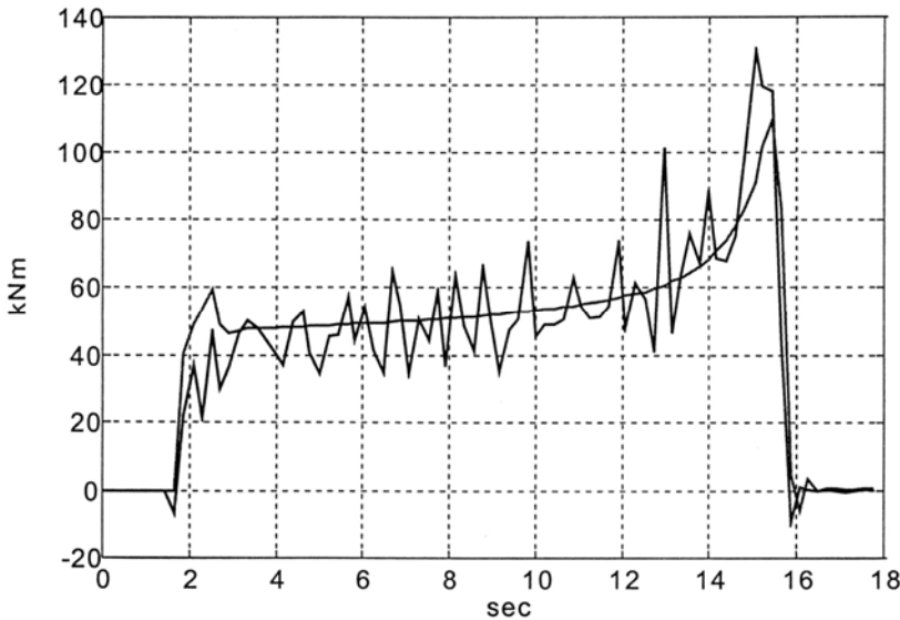
Figure 22.30 Torque versus time during acceleration [23] from (22.109) and from (22.110)
