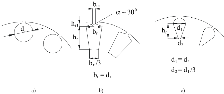
Figure 17.2 Rotor bar slots with low skin effect: a) round shape, b) rectangular, c) pair shape
