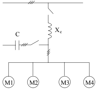
Figure 13.36 A group of induction motors
