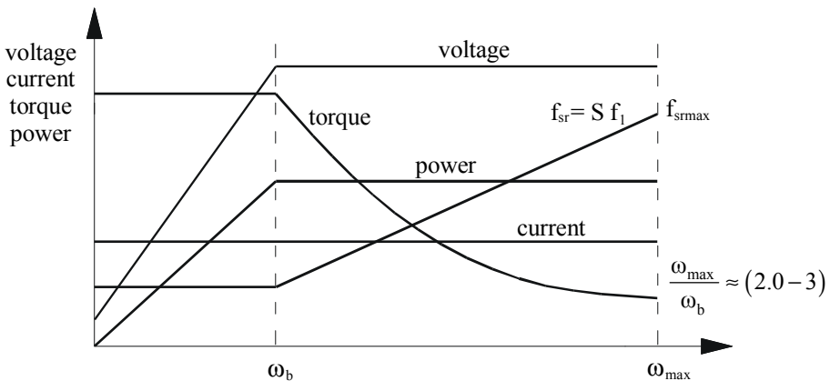
Figure 17.5 Torque, voltage, current versus frequency
