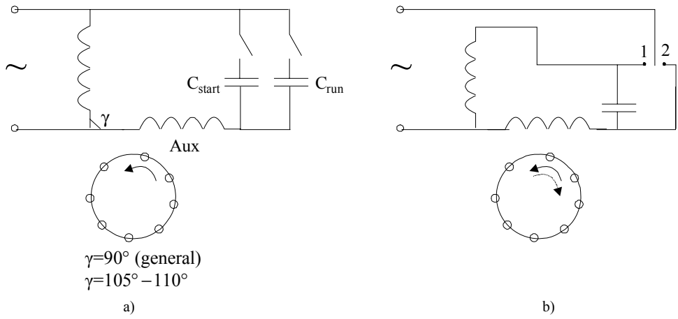
Figure 4.17 Two-phase induction motor: a) for unidirectional motion, b) for bidirectional motion (1 - closed for forward motion; 2 - closed for backward motion)
