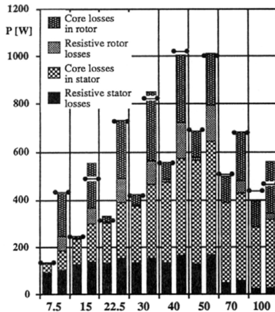
Figure 11.15 No-load losses (37kW IM) at 7.5Hz, ..., 100Hz fundamental frequency. Left column for sinusoidal voltage and right column for PWM voltage. Measured losses marked by cross bars [16]
