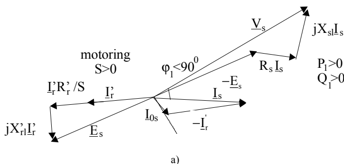
Figure 7.21 Standard phasor diagrams (continued): a) for motoring,
