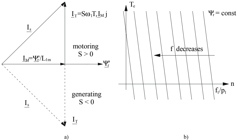
Figure 8.16 Rotor flux vector control: a) stator current components, b) torque versus speed curves for variable frequency f_l at constant rotor flux
