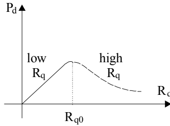
Figure 11.6 Transverse losses versus transverse resistance R_q
