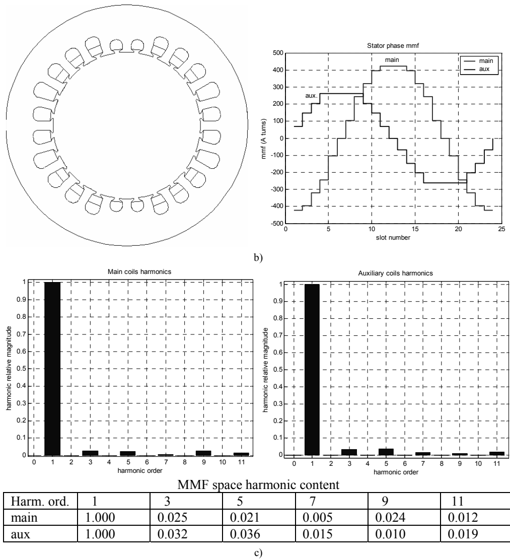
Figure 4.21 (continued): b) practical case, c) mmf harmonics content.
