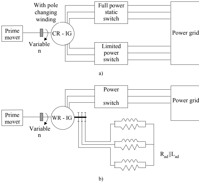
Figure 19.4 Simplified IG systems:
