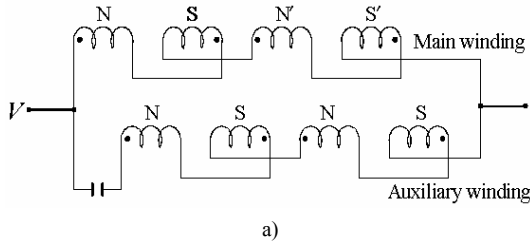
Figure 24.26 Winding pattern (continued): a) 4 poles operation
