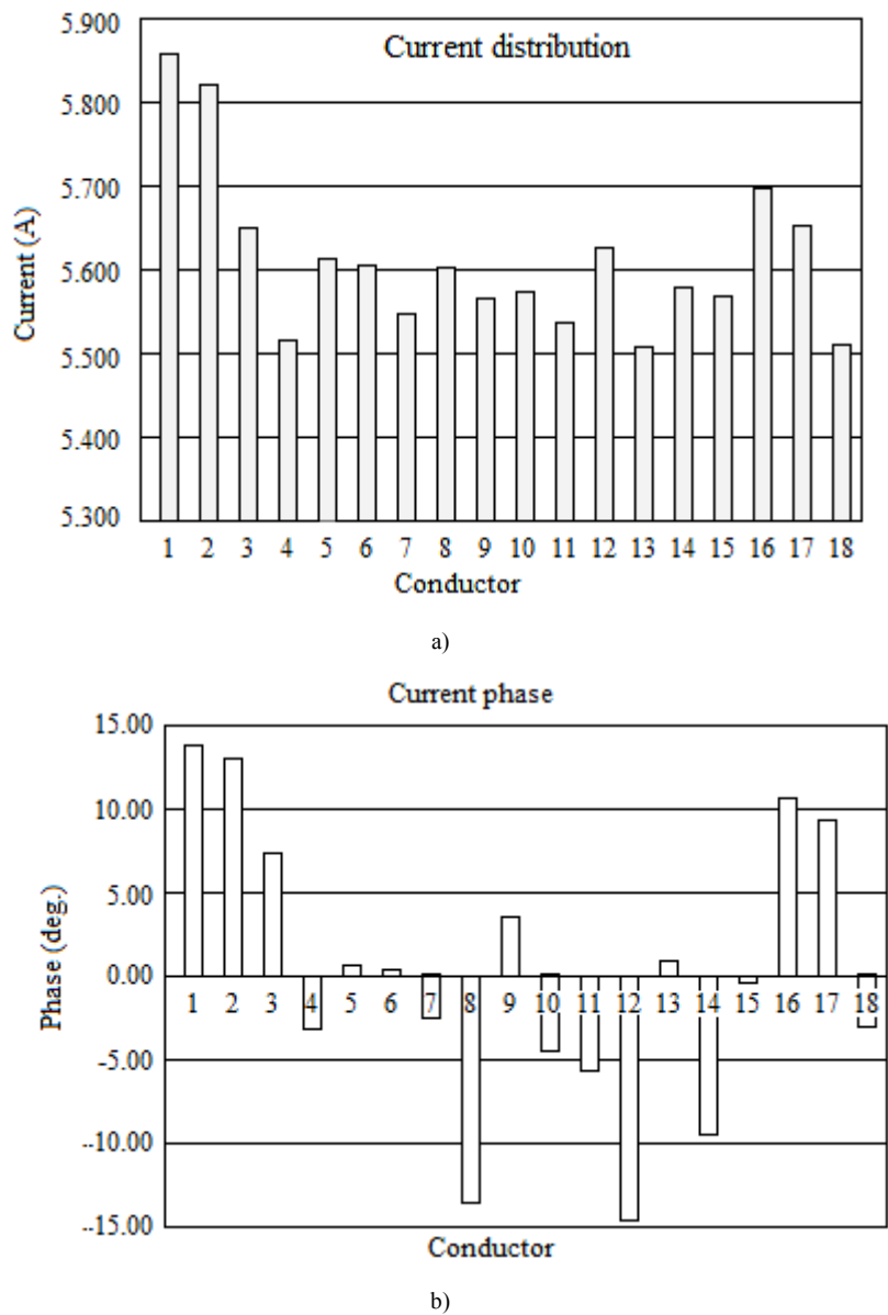
Figure 9.40 Current distribution between paralleled elementary conductors for 180° stranding, 2 coils, 3 turns/coil, 100 A per coil at 2333 Hz, conductor diameter 0.63 mm: a) amplitude, b) phase
