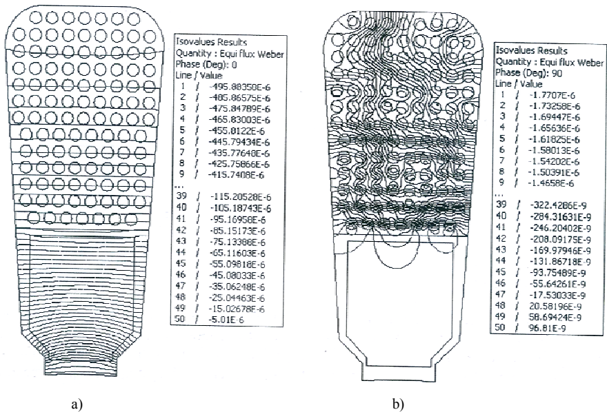
Figure 9.39 Flux lines for 180° stranding/18 conductors in parallel, 2 coils, 3 turns/coil, at 2333 Hz, conductor diameter 0.63 mm: a) max coil current, b) zero coil current
