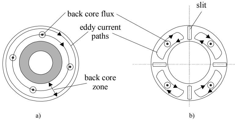
Figure 20.27 Tubular LIM back core disk-shape lamination a) and its slitting b) to reduce eddy current losses
