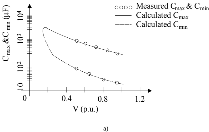
Figure 19.18 Min-max capacitors on no-load (continued): a) balanced capacitor
