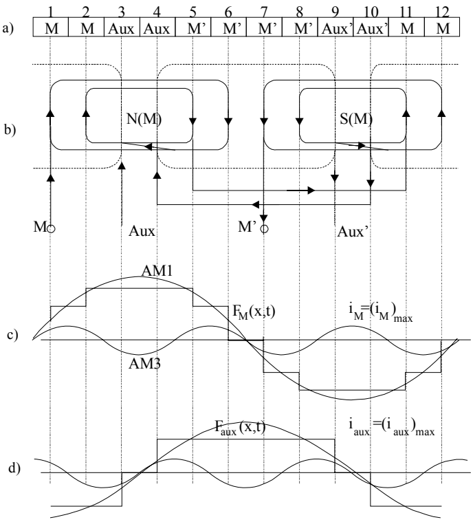
Figure 4.18 Capacitor start motor two-phase single-layer winding; 2p_1 = 2 poles, N_s = 12 slots (continued): a) slot/phase allocation: M/Aux = 2/1, b) coils per phase connections, c) mmf distribution for main phase (M), d) mmf distribution for auxiliary phase (Aux)
