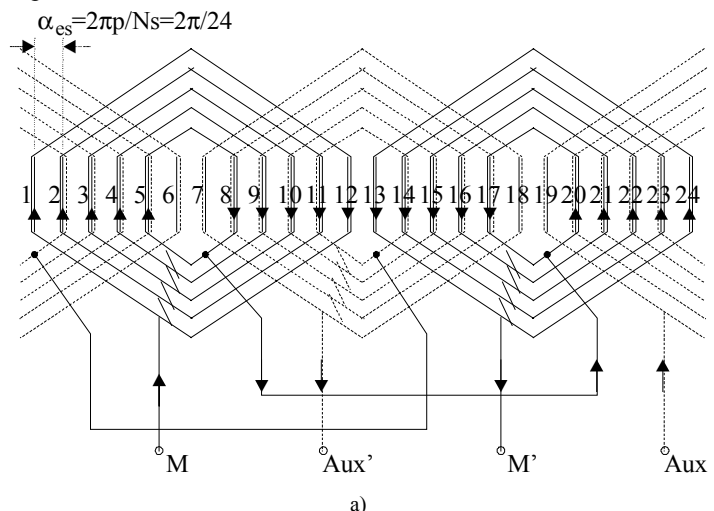
Figure 4.21 Two-pole two-phase winding with sinusoidal conductor count/slot/phase distribution (continued): a) All slots are filled,
