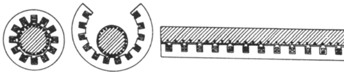
Figure 20.1 Imaginary process of obtaining a LIM from its rotary counterpart
