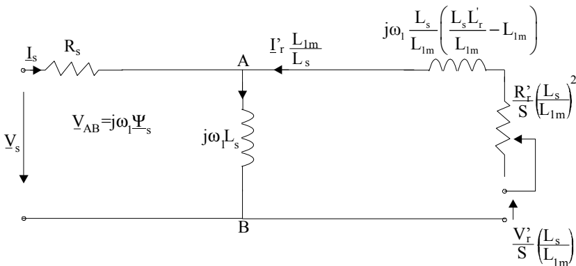
Figure 7.25 Equivalent circuit (continued): a) with stator flux shown,
