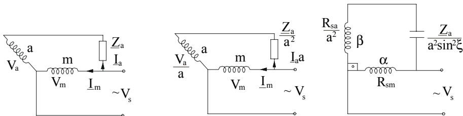
Figure 24.9 Evolutive equivalent schematics of nonorthogonal winding IM
