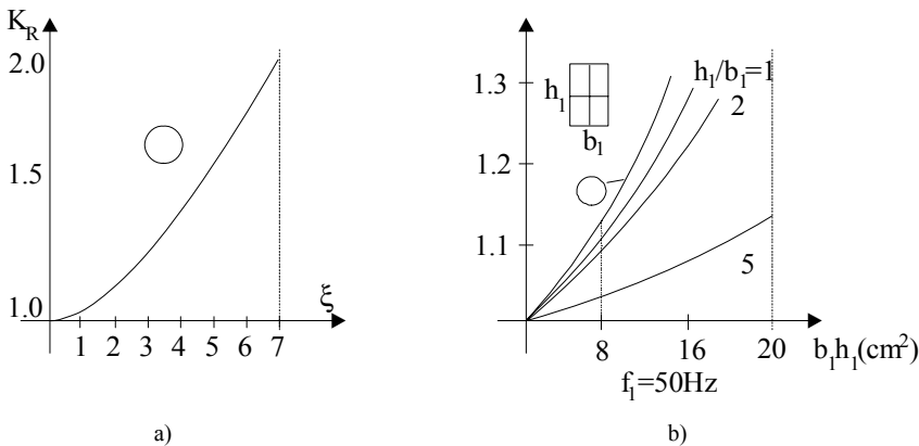
Figure 9.10 Skin effect correction factor K_R for a conductor in air: a) circular cross-section, b) rectangular cross-section
