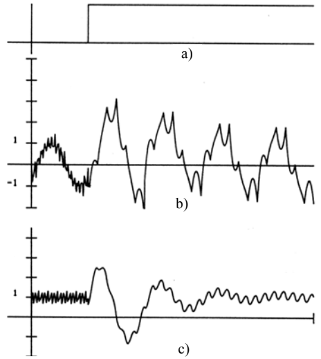
Figure 13.31 Computed transient response for a change from harmonic ( N = 5 ) elimination PWM to square wave excitation at 60Hz: a) voltage, b) current, c) torque
