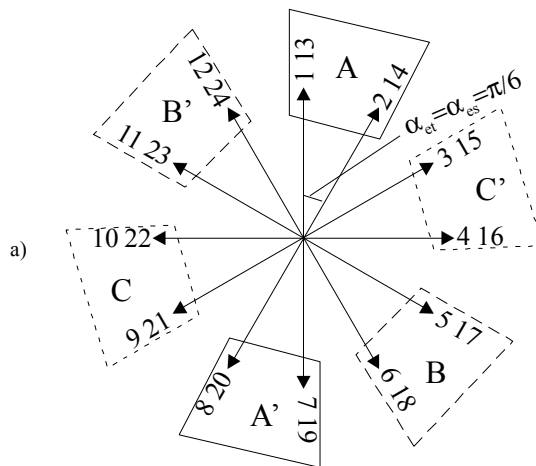
Figure 4.15 2/4 pole winding ( N_s = 24 ) (continued): a) emf star,
