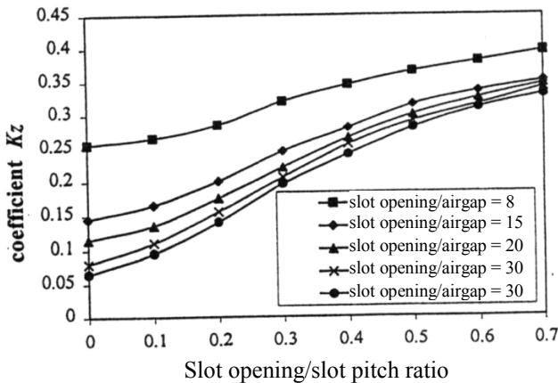
Figure 9.26 Correction coefficient for differential leakage damping
