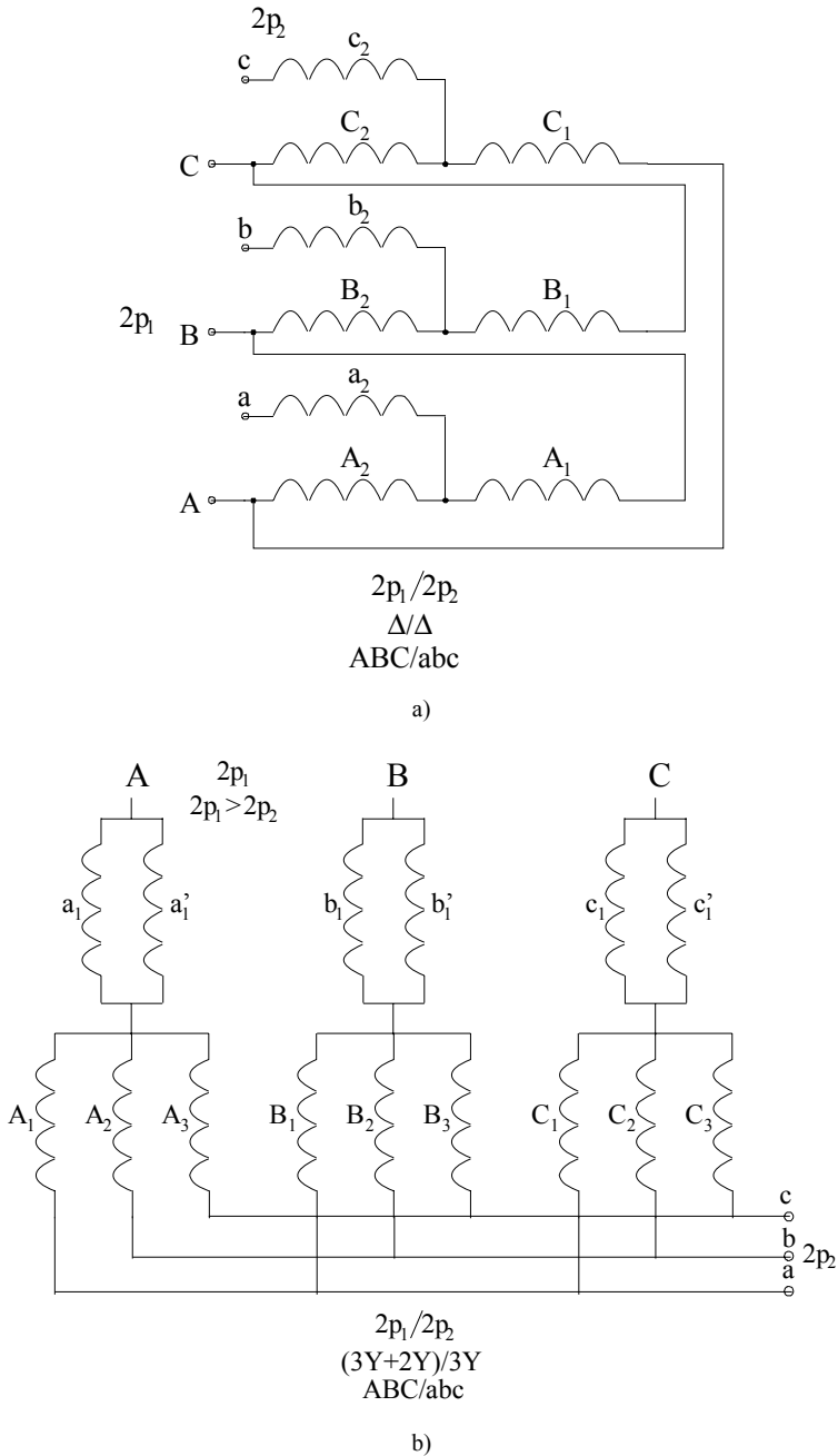
Figure 4.24 2p_1/2p_2 pole connections: a) \Delta/\Delta , b.) (3Y + 2Y)/3Y
