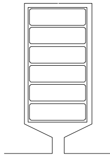
Figure 6.12 Multi-conductor single-turn coils for high power IMs
