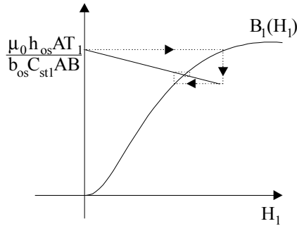
Figure 9.30 Tooth top flux density
