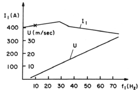
Figure 20.30 Imposed current and speed dependence of frequency
