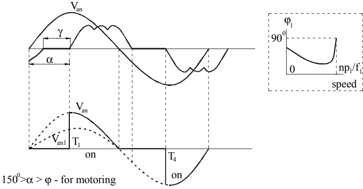
Figure 8.5 Soft starter phase voltage and current
