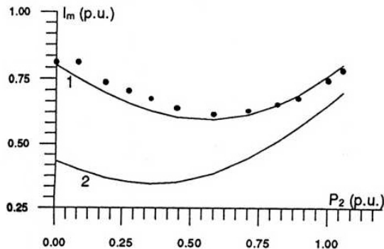
Figure 25.4 RMS of main winding current versus output power
