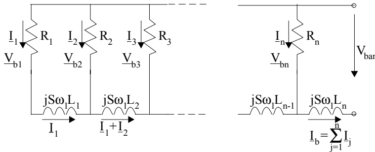
Figure 9.13 Equivalent circuit for skin effect evaluation
