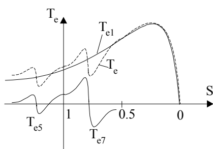
Figure 10.5 Torque/slip curve with 5 th and 7 th harmonic asynchronous parasitic torques
