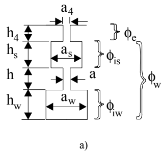
Figure 9.18 (continued): Double cage rectangular-shape geometry a)
