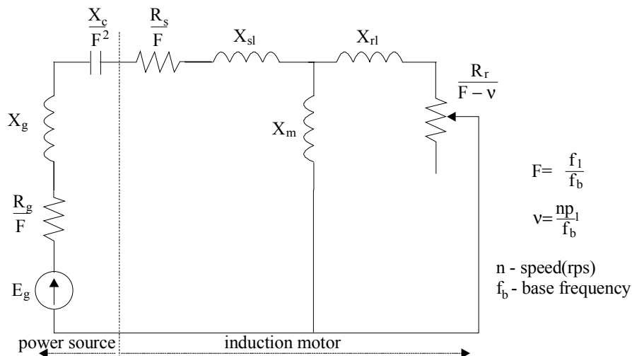
Figure 13.37 Equivalent circuit with power source parameters, R_g , X_g , X_c in series
