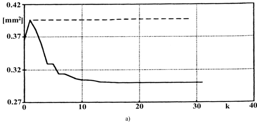
Figure 27.9 (continued): a) Main winding wire sizes evolution during the optimization process,
