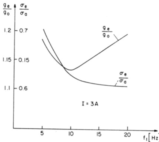
Figure 20.23 Equivalent airgap ( g_e/g_o ) and secondary conductivity ( \sigma_e/\sigma_{Al} ) thrust F_x and goodness factor G_e versus frequency at standstill (continued)
