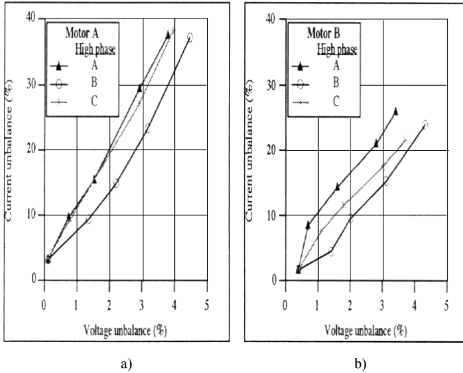
Figure 7.27 Current unbalance versus voltage unbalance [2]:
