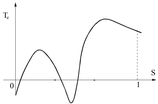
Figure 24.14 Grossly oversized capacitor IM torque-speed curve
