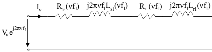
Figure 11.9 Equivalent circuit for time harmonic v
