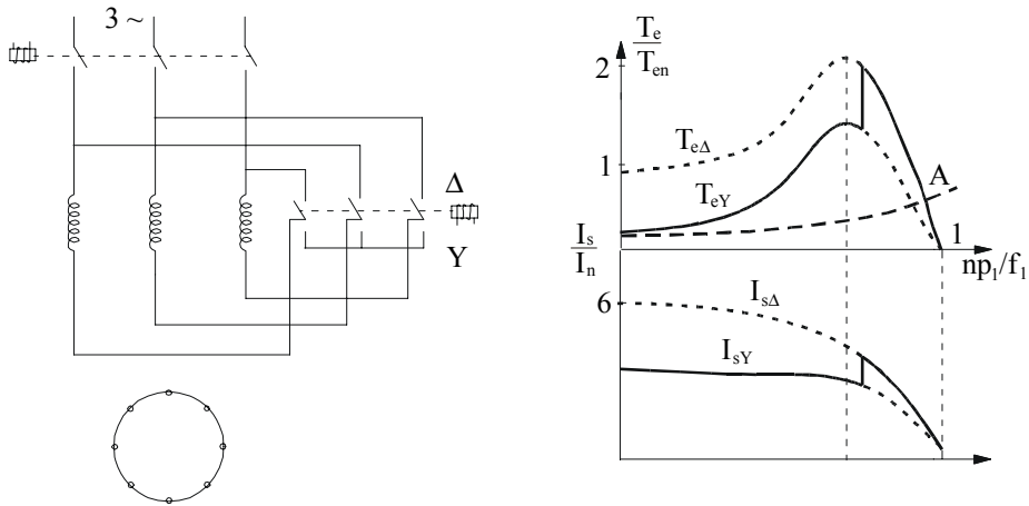
Figure 8.3 Wye-delta starting
