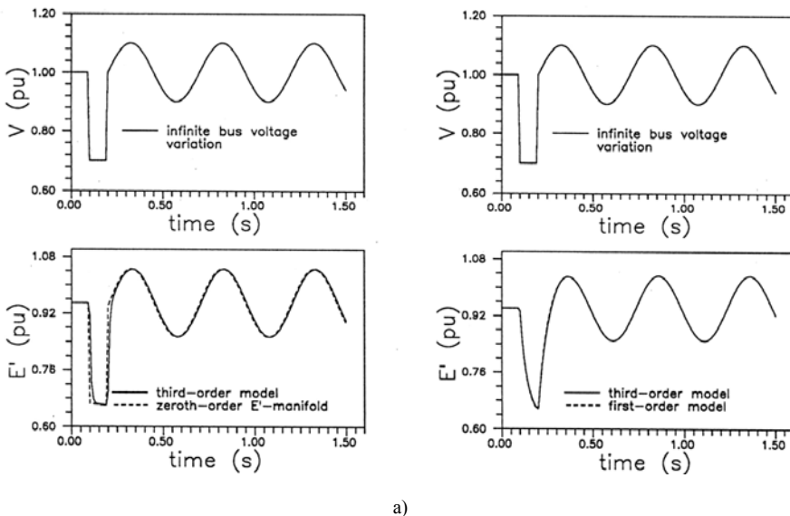
Figure 13.35 Third and first order model transients (continued):
