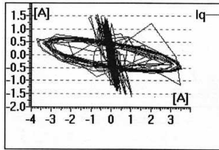
Figure 25.6 Current hodograph during starting
