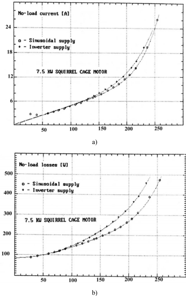
Figure 22.7 No-load testing: a) current, b) losses
