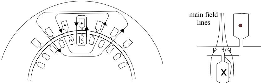
Figure 2.16 Flux paths in IMs
