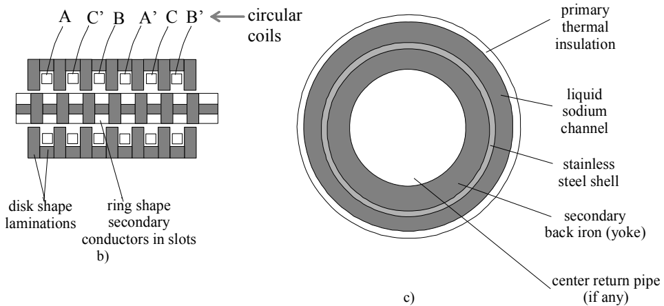
Figure 20.5 (continued): b) with disk-shape laminations, c) liquid metal tubular LIM pump: the secondary
