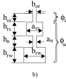
Figure 16.12 (continued): slot geometrical parameters b)
