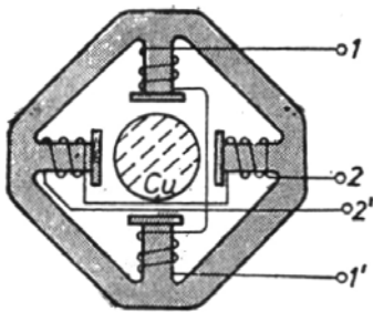
Figure 1.1 Ferrari's induction motor (1885)
