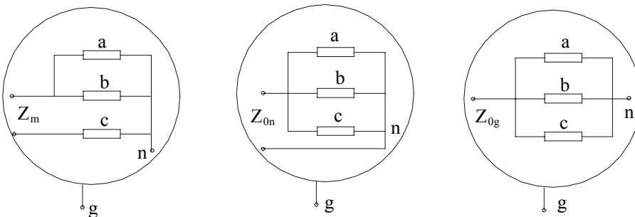
Figure 21.3 Line ( Z_m ) neutral ( Z_{on} ) and ground (common mode Z_{0g} )
