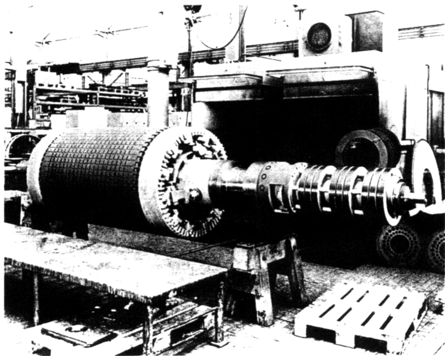
Figure 2.9 Three-phase wound rotor
