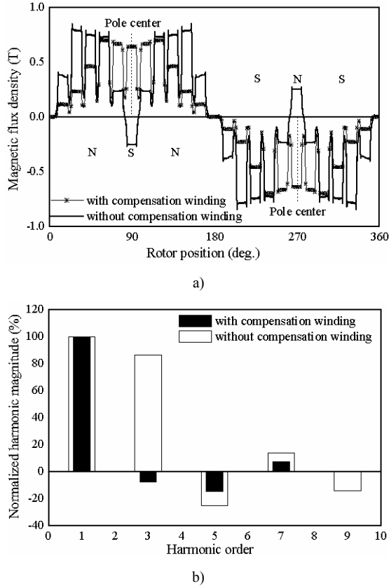
Figure 24.25 Airgap flux density distribution for 2p = 2 (with a 4 pole winding in 2p = 2 connection) with and without compensation winding (Figure 24.26): a) Magnetic flux density distribution [12], b) Discrete Fourier transform (DFT) of the magnetic flux density distribution
