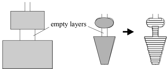
Figure 9.15 Treating skin effect with equivalent circuit (or multilayer) method
