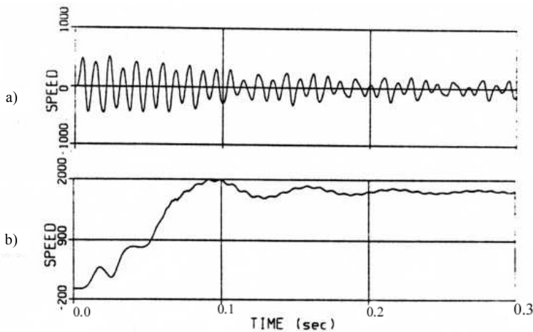
Figure 25.8 Starting speed transients for N_s = N_r : a) without skewing, b) with skewing
