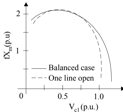
Figure 19.17 Positive sequence magnetizing characteristics
