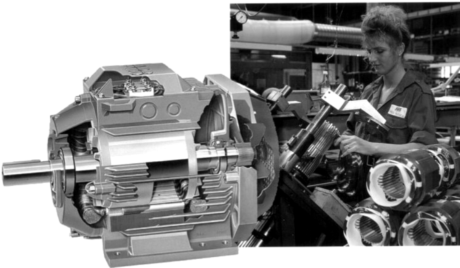
Figure 1.5 Aluminum frame induction motor (Source: ABB)
