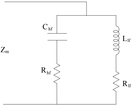
Figure 21.6 Differential mode IM equivalent circuit
