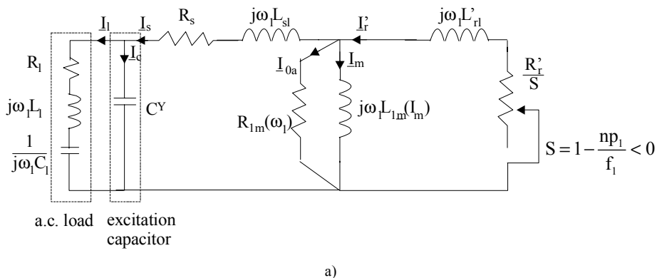
Figure 7.15 Autonomous induction generator on load (continued): a) equivalent circuit
