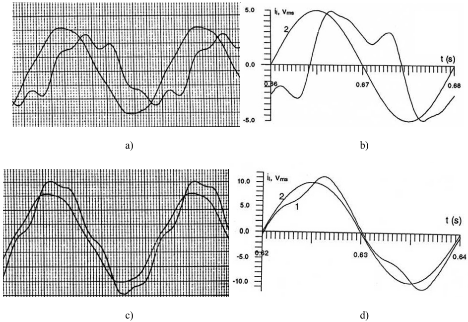
Figure 25.3 Steady state by the d-q model with saturation included:
