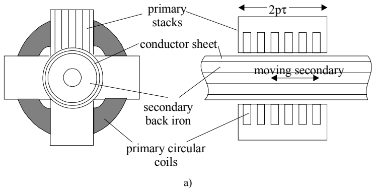
Figure 20.5 Tubular LIMs (continued): a) with longitudinal primary lamination stacks,
