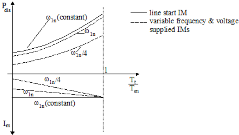
Figure 12.8 Electromagnetic losses P_{\text{dis}} and magnetization current I_m versus torque
