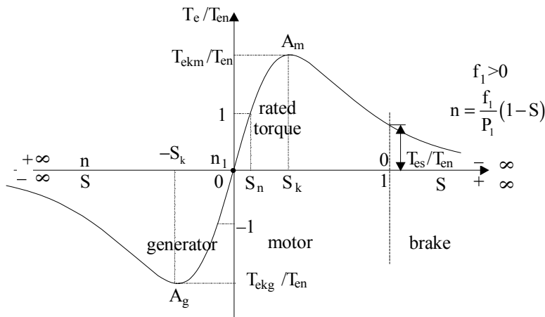
Figure 7.17 The electromagnetic torque T_e (in relative units) versus slip (speed)
