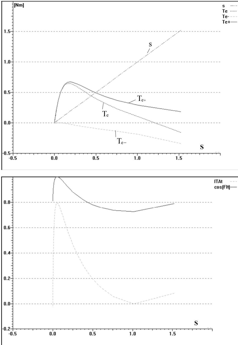
Figure 24.10 (continued): T_e , T_{e-} , T_{e+} – total, positive and negative sequence torques, S(T_e) – slip, IT_{At} – efficiency, \cos Fl_t – power factor
