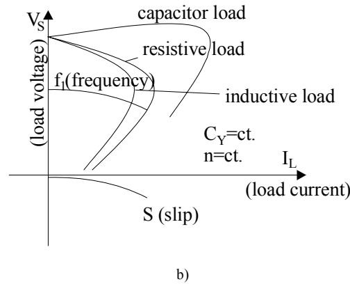
Figure 7.15 (continued): b) load curves
