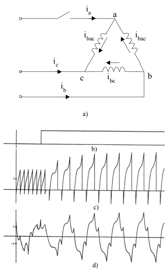
Figure 13.32 Computed transient response for a single phasing fault on line “a” at 60Hz: a) open line condition, b) instant when single phasing occurs, c) dc link current, d) line current i_s
