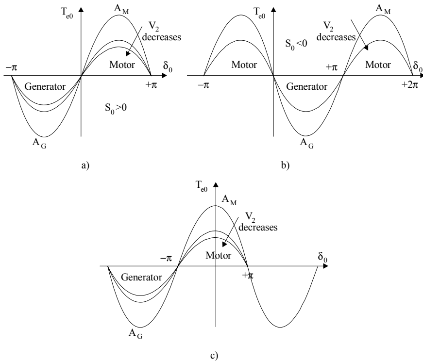
Figure 19.23 Ideal torque-angle curves:
