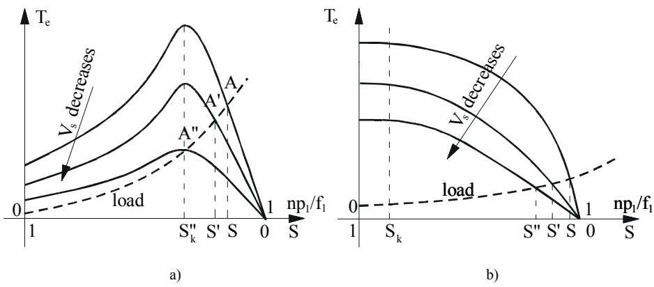
Figure 8.10 Torque versus speed for different voltage levels V_s : a) standard motor: S_K=0.04 - 0.10 , b) high resistance (solid iron) rotor motor S_K > 0.7 - 0.8
