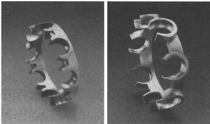
Fig. 5.15: Snap-in polyamide cage (left) and machined brass cage (right), both for Conrad-type bearings.
