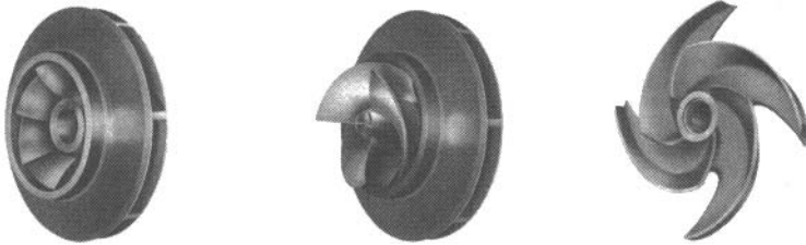
Figure 11.2: Closed impeller (left), impeller with inducer (center), open impeller (right).
