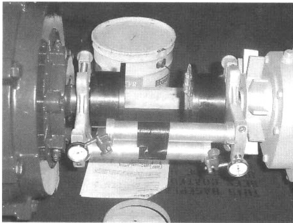
Figure 14.6: Reverse dial indicator alignment setup using low-sag tubular indicator mounting brackets (Ref. 3).
