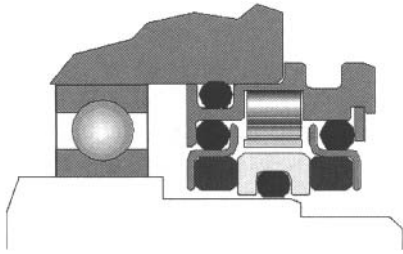
Figure 8.5: Dual-face magnetic bearing protector seal.
