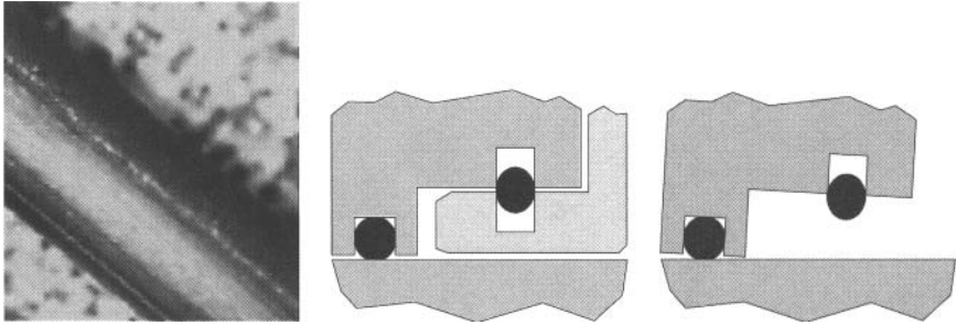
Figure 8.3: Inadequate shaft clamping, off-center mass, and O-ring contact with sharp edges can cause degradation and unforeseen contamination of lube oil.
