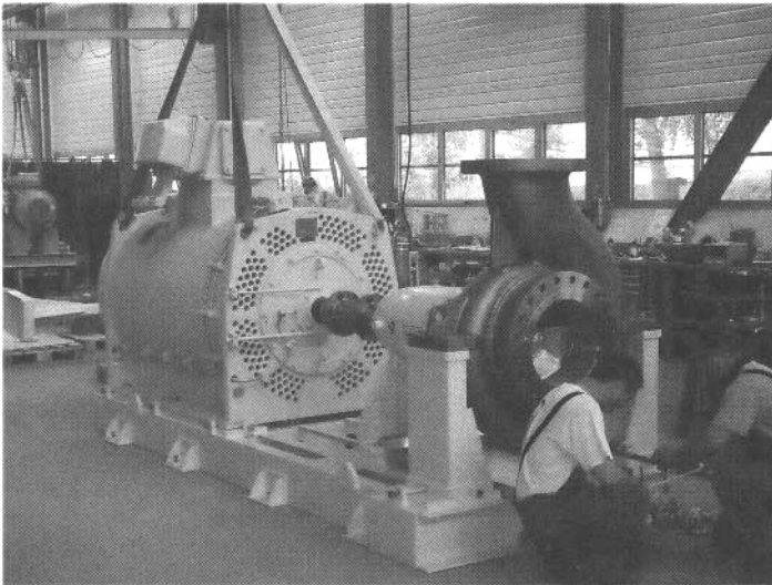
Figure 14.3: A quality process pump during factory assembly. Note alignment jacking bolts on pump supports and on motor (Source: Emile Egger & Cie., Cressier, NE, Switzerland).
