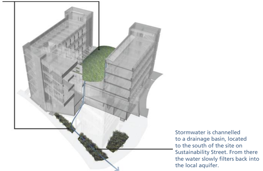
Figure 5.15 Rainwater to stormwater system. (Perkins+Will Architects)
