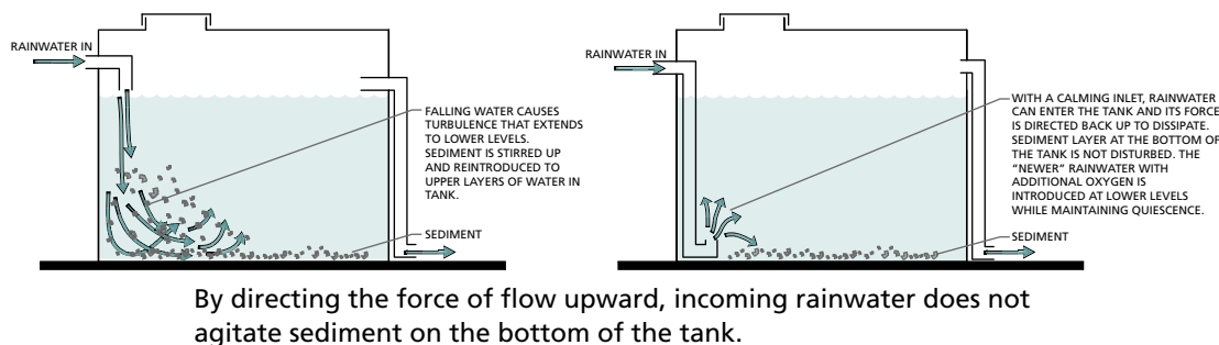
Figure 5.7 Purpose for Calming inlet.
