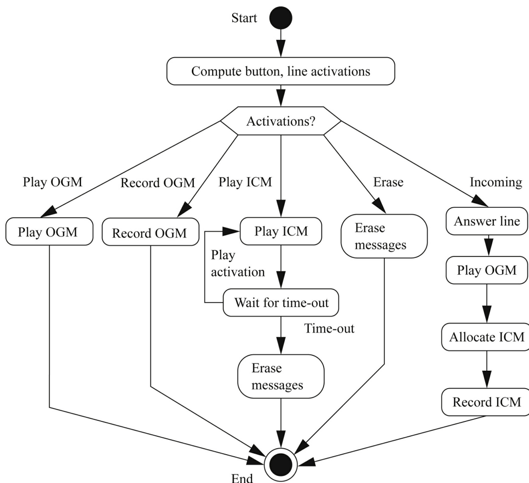
FIGURE 6.25 State diagram for the Controls activate behavior.
