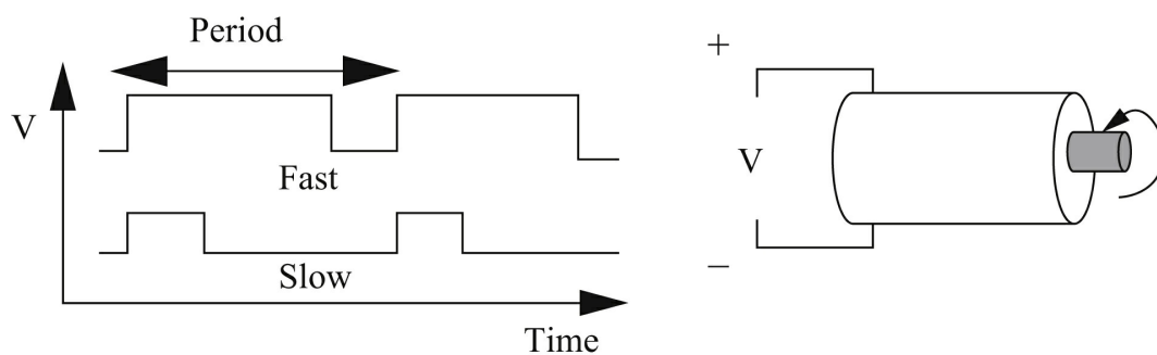
FIGURE 1.22 Controlling motor speed by pulse-width modulation.
