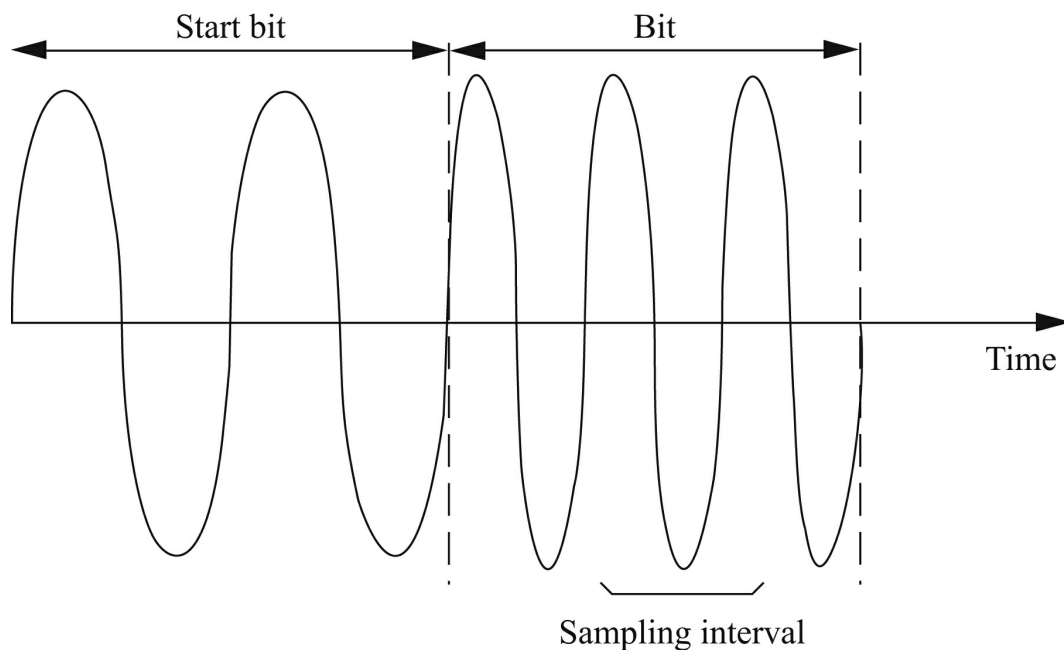
FIGURE 5.31 Receiving bits in the modem.
