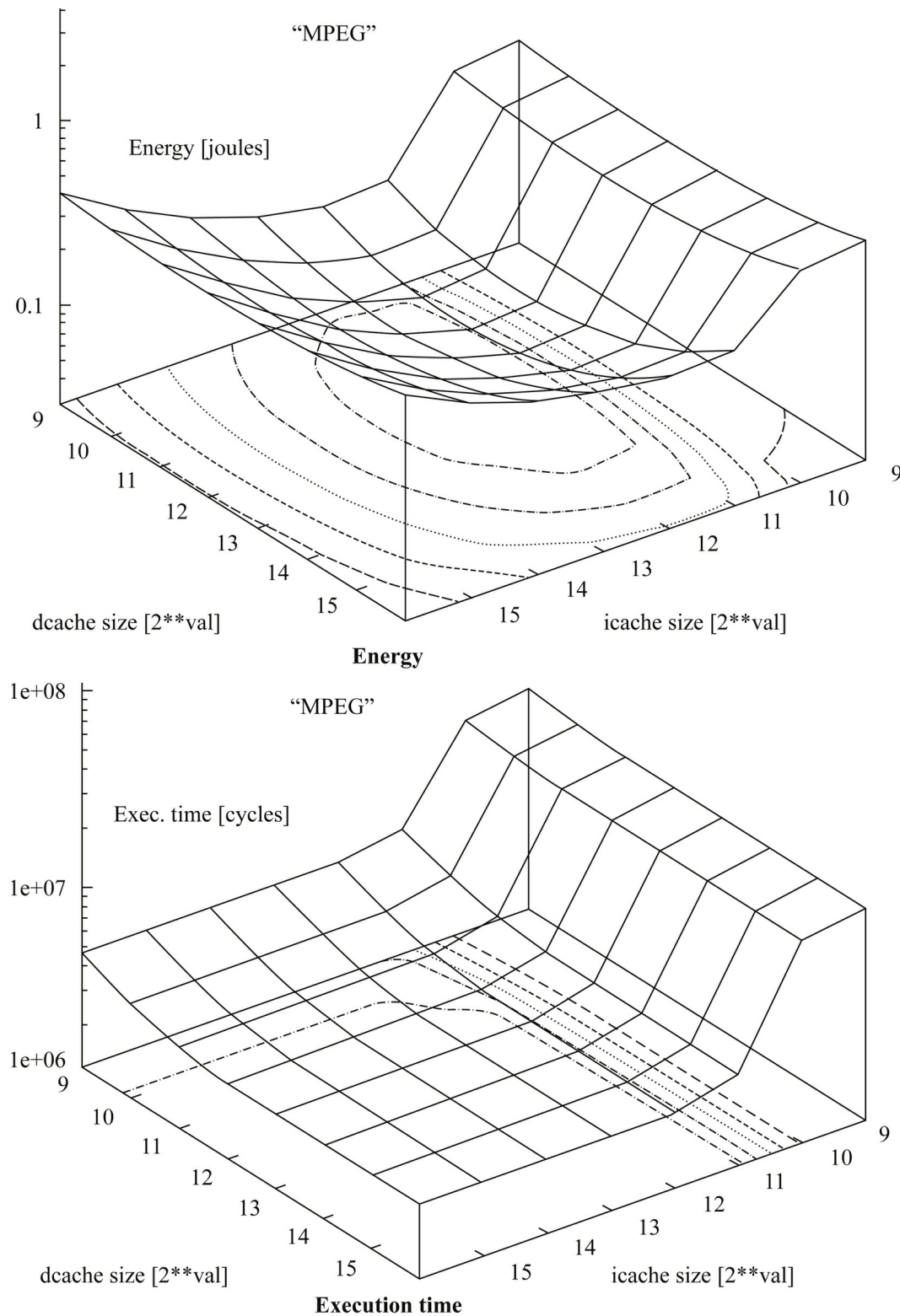
FIGURE 5.23 Energy and execution time versus instruction/data cache size for a benchmark program [Li98].
