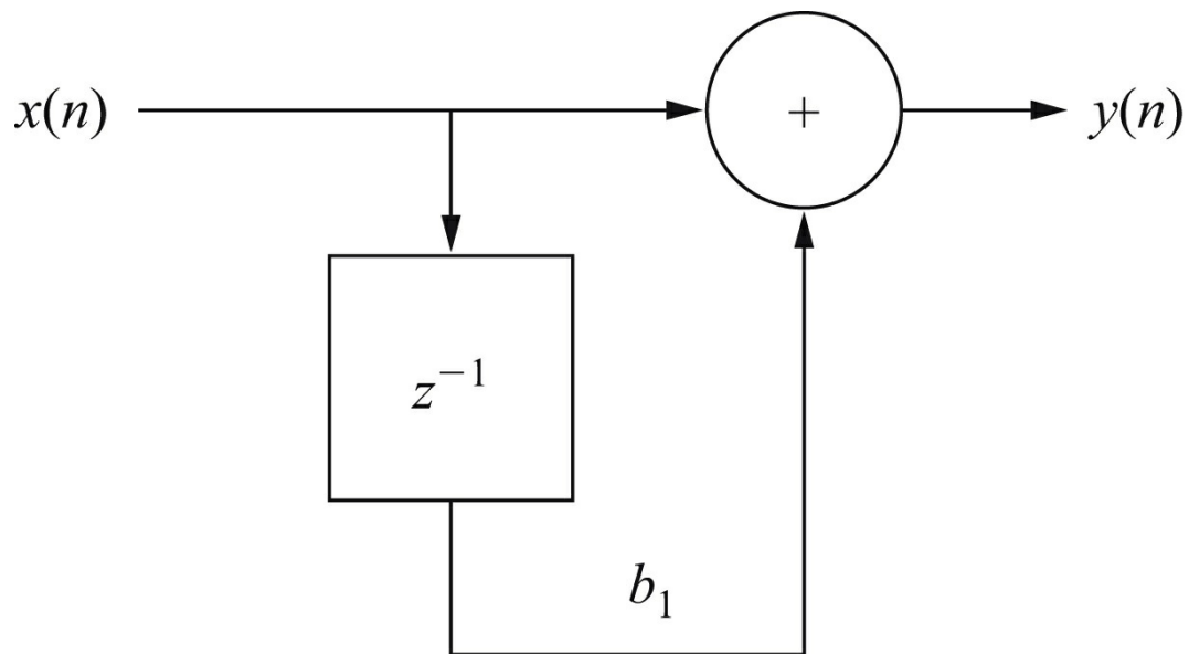
FIGURE 5.2 A signal flow graph.
