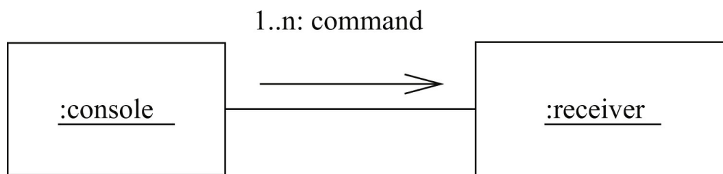
FIGURE 1.18 UML collaboration diagram for major subsystems of the train controller system.
