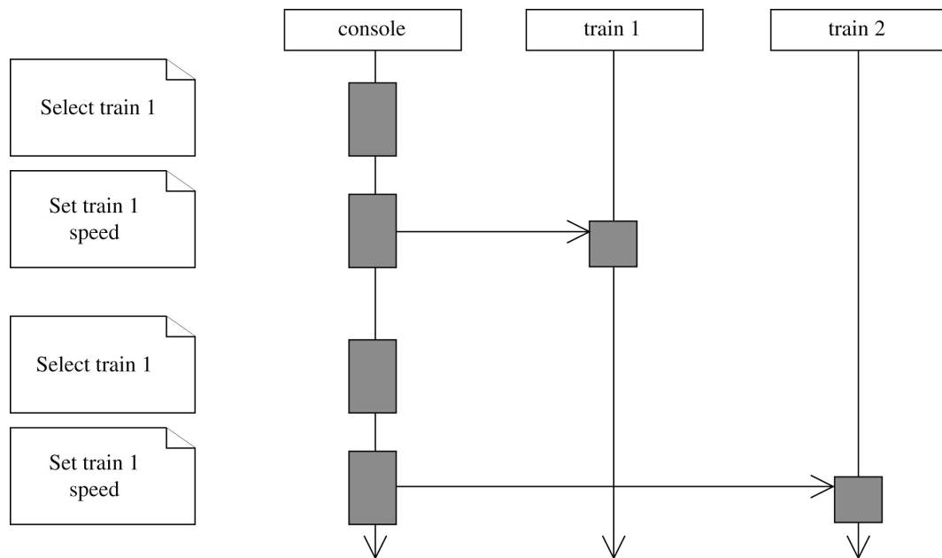
FIGURE 1.20 Use case for setting speeds of two trains.
