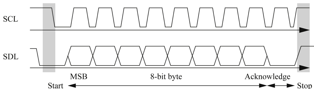
FIGURE 10.15 Transmitting a byte on the I 2 C bus.
