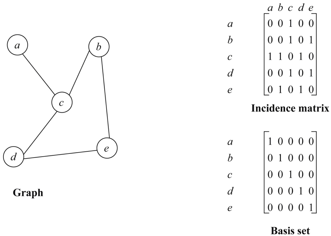
FIGURE 5.24 The matrix representation of a graph and its basis set.
