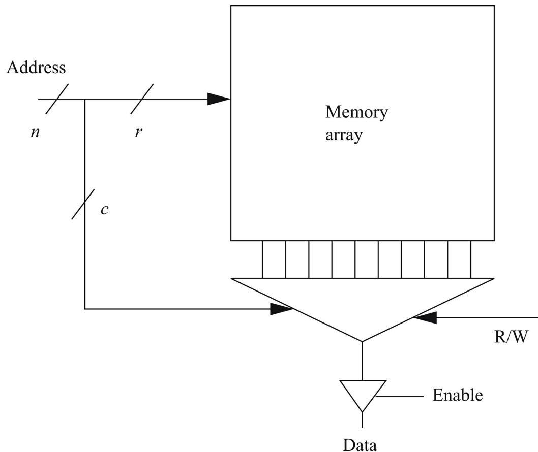
FIGURE 4.17 Organization of a basic memory.
