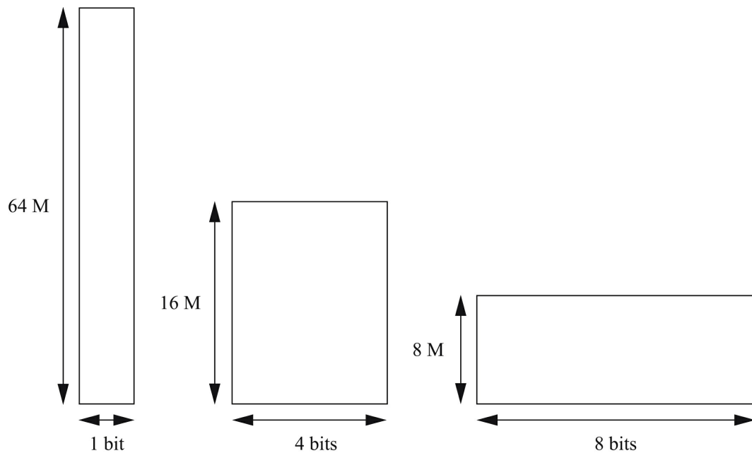
FIGURE 4.32 Memory aspect ratios.
