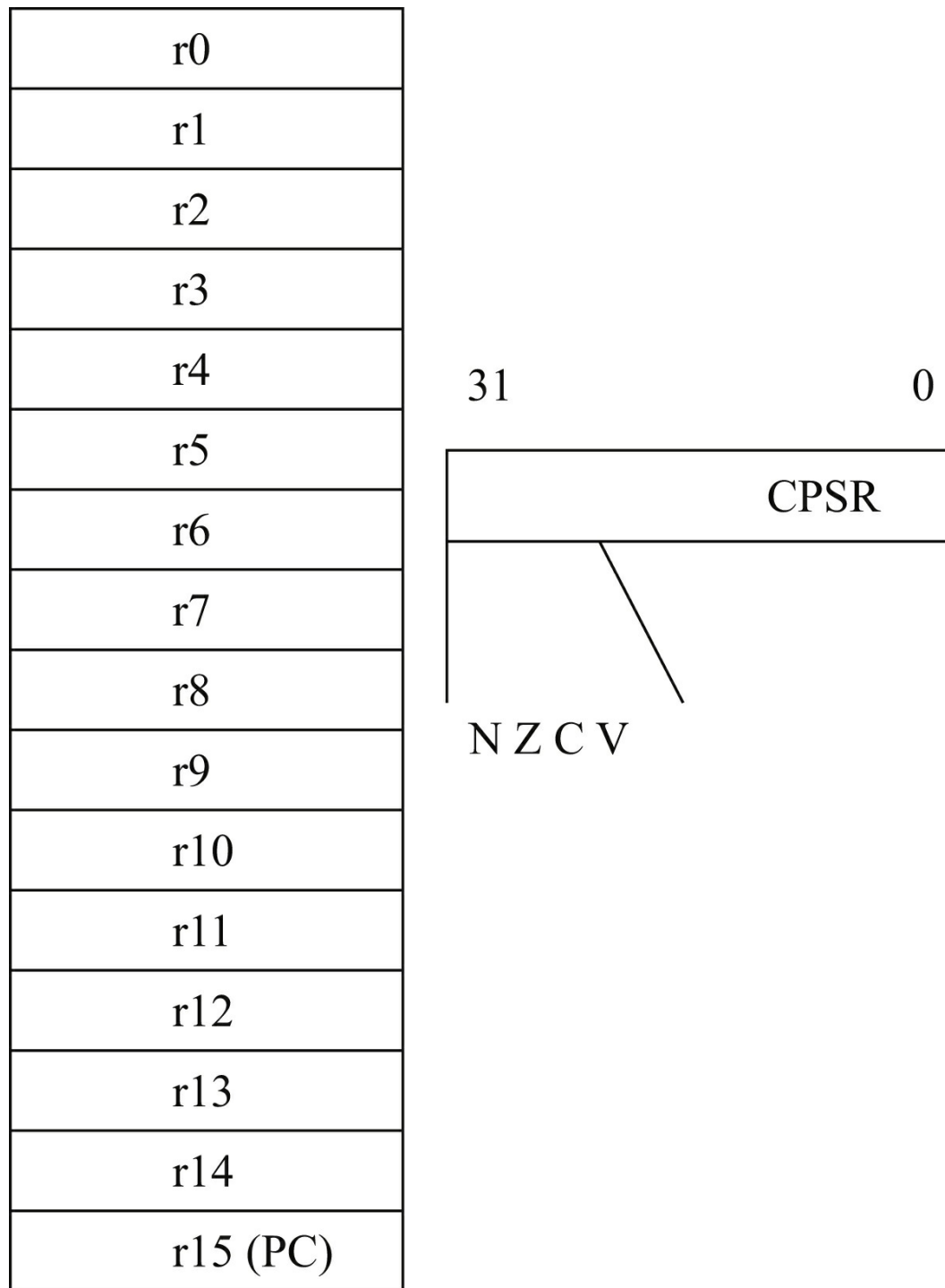
FIGURE 2.9 The basic ARM programming model.
