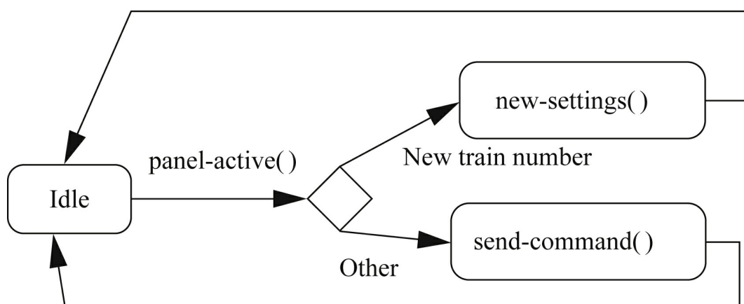
FIGURE 1.27 State diagram for the formatter operate behavior.
