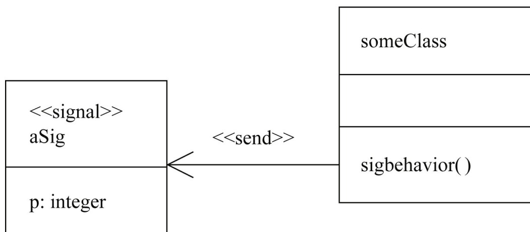
FIGURE 6.16 Use of a UML signal.
