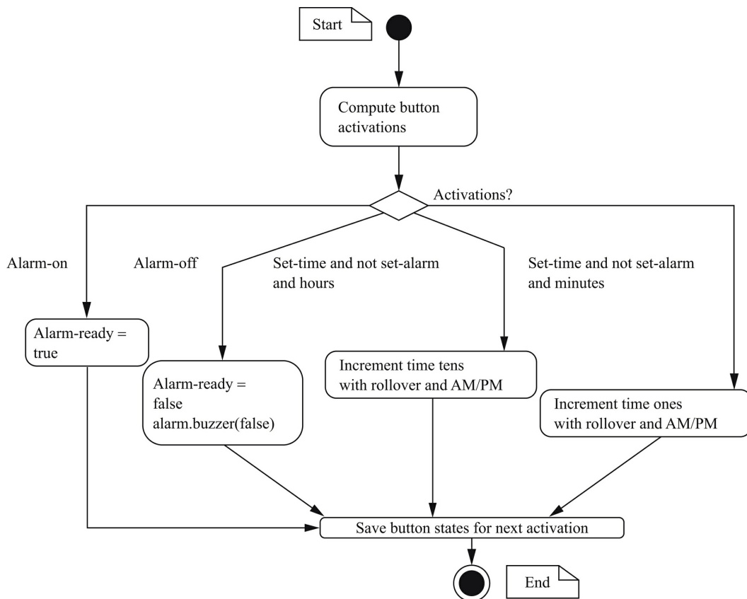
FIGURE 4.39 State diagram for scan-keyboard.
