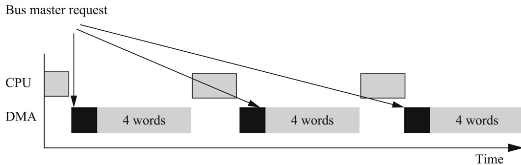
FIGURE 4.13 Cyclic scheduling of a DMA request.
