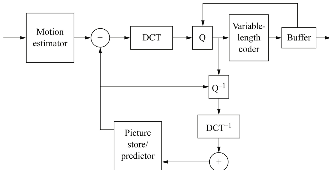
FIGURE 10.17 Block diagram of MPEG-2 compression algorithm.
