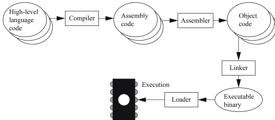
FIGURE 5.10 Program generation from compilation through loading.
