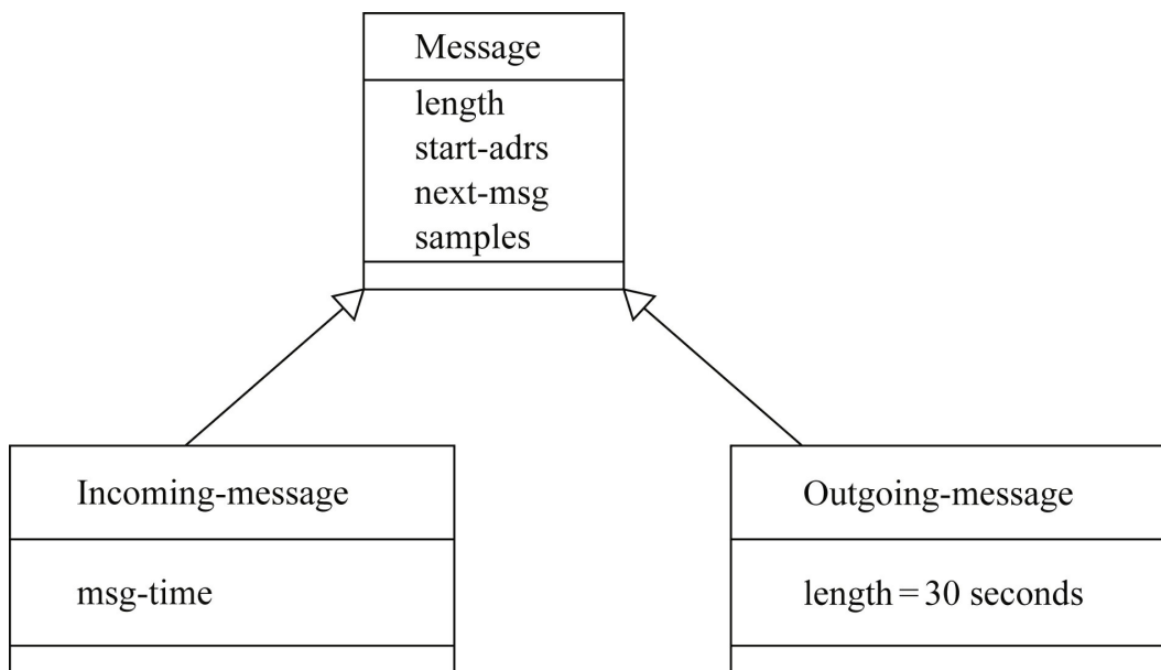
FIGURE 6.23 The message classes for the answering machine.
