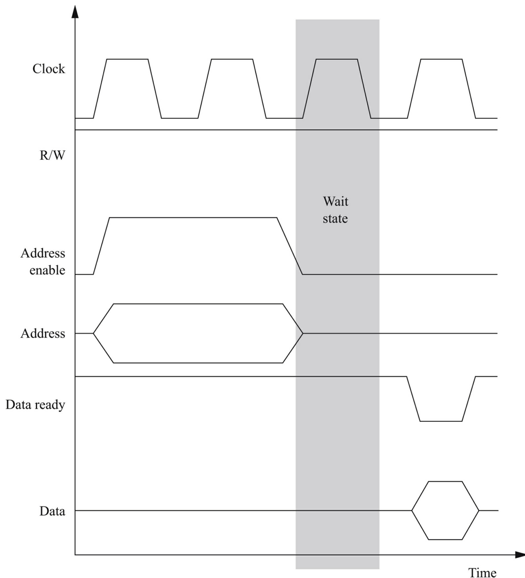
FIGURE 4.8 A wait state on a read operation.
