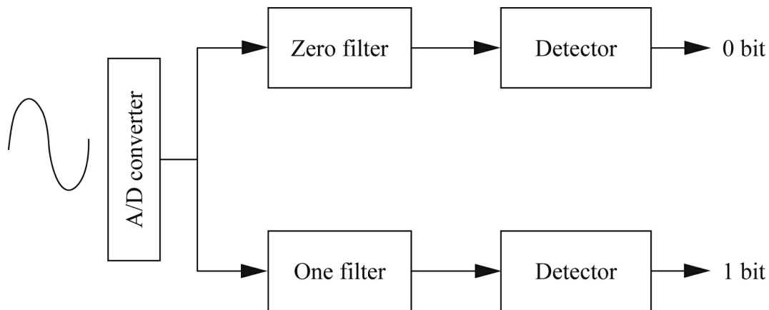
FIGURE 5.30 The FSK detection scheme.
