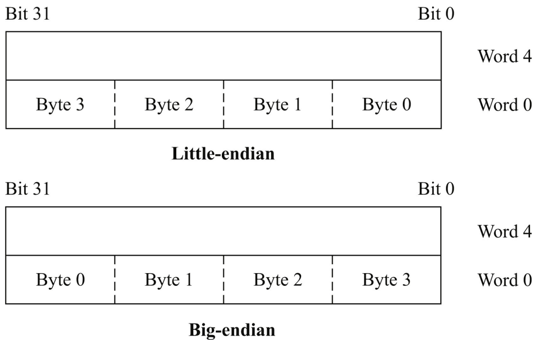
FIGURE 2.7 Byte organizations within an ARM word.
