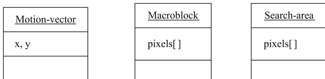
FIGURE 10.20 Classes describing basic data types in the video accelerator.
