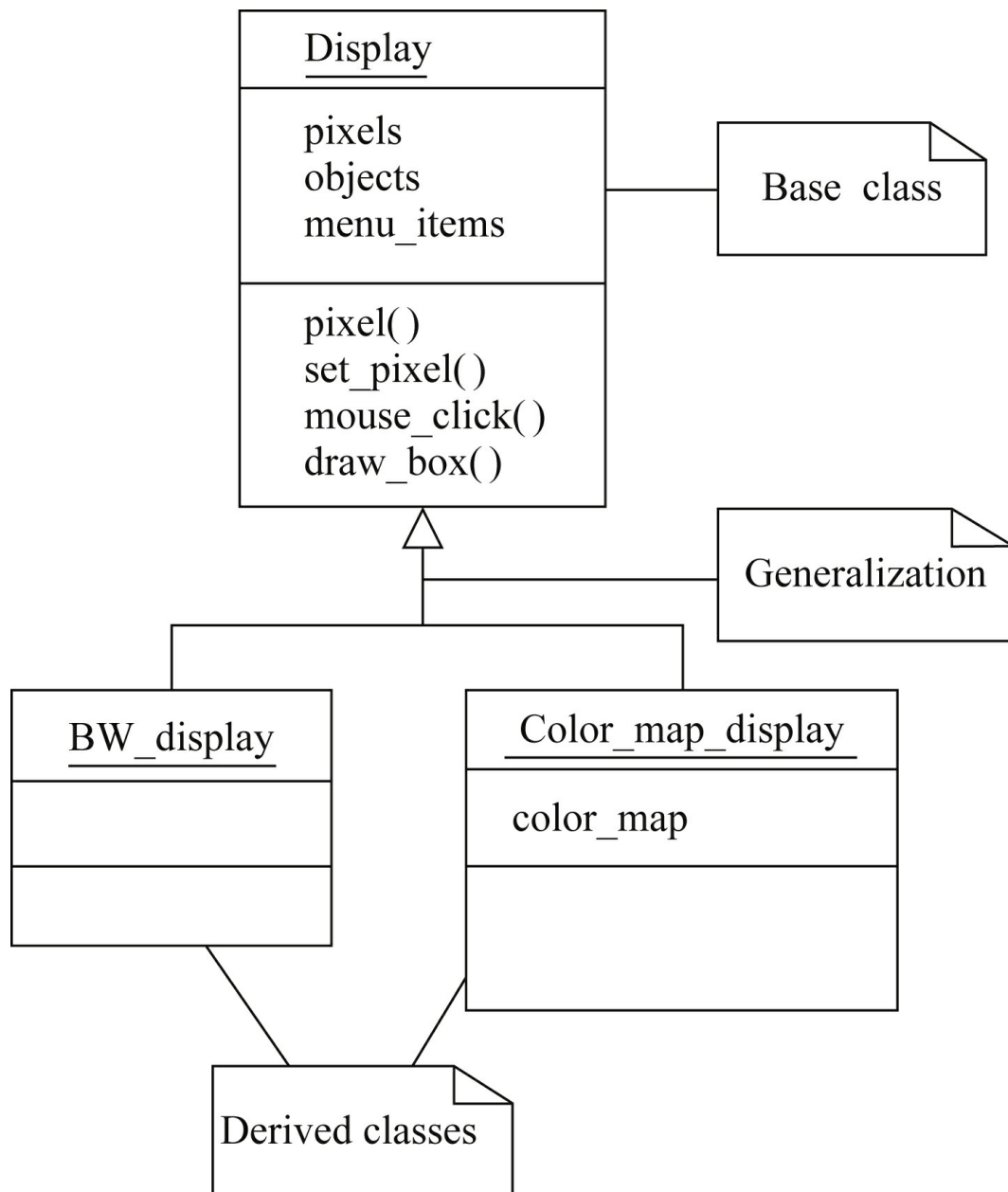
FIGURE 1.7 Derived classes as a form of generalization in UML.
