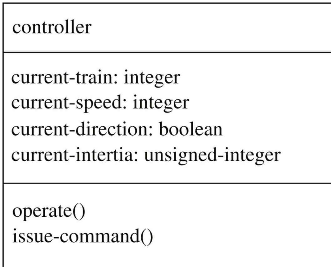
FIGURE 1.29 Class diagram for the Controller class.
