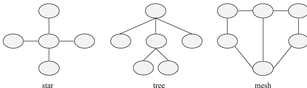
FIGURE 8.9 Example IoT network topologies.
