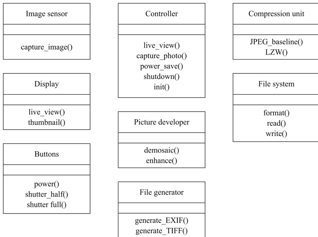
FIGURE 5.41 Basic classes in the digital still camera.
