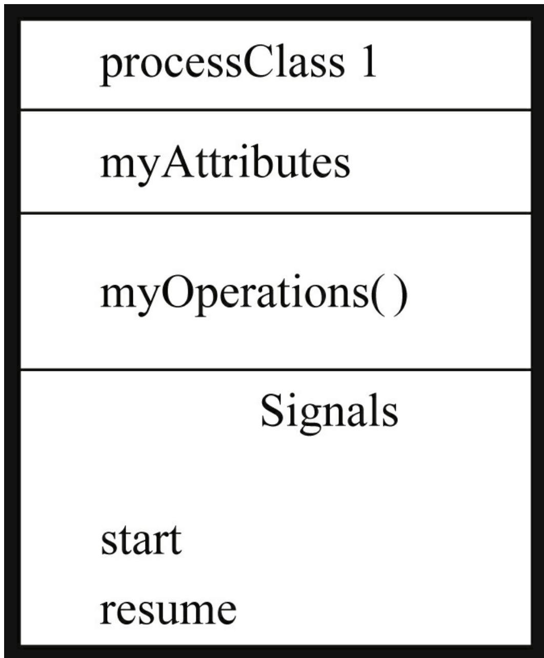
FIGURE 6.10 An active class in UML.
