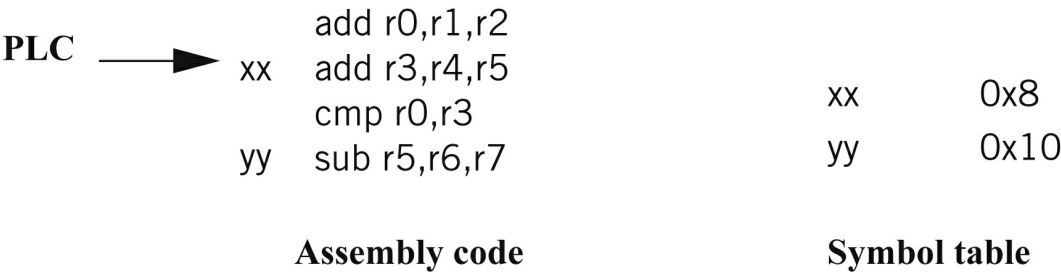
FIGURE 5.11 Symbol table processing during assembly.
