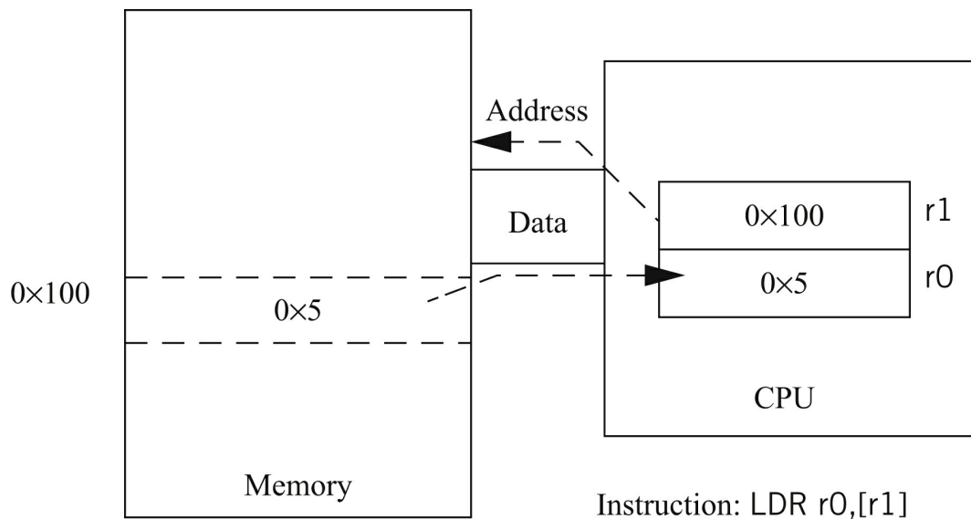
FIGURE 2.14 Register-indirect addressing in the ARM.
