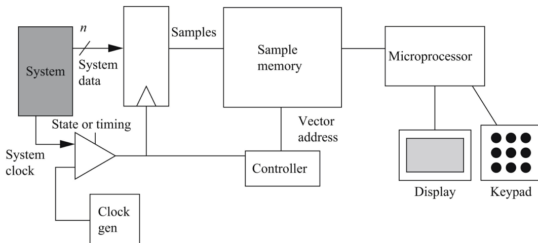
FIGURE 4.25 Architecture of a logic analyzer.
