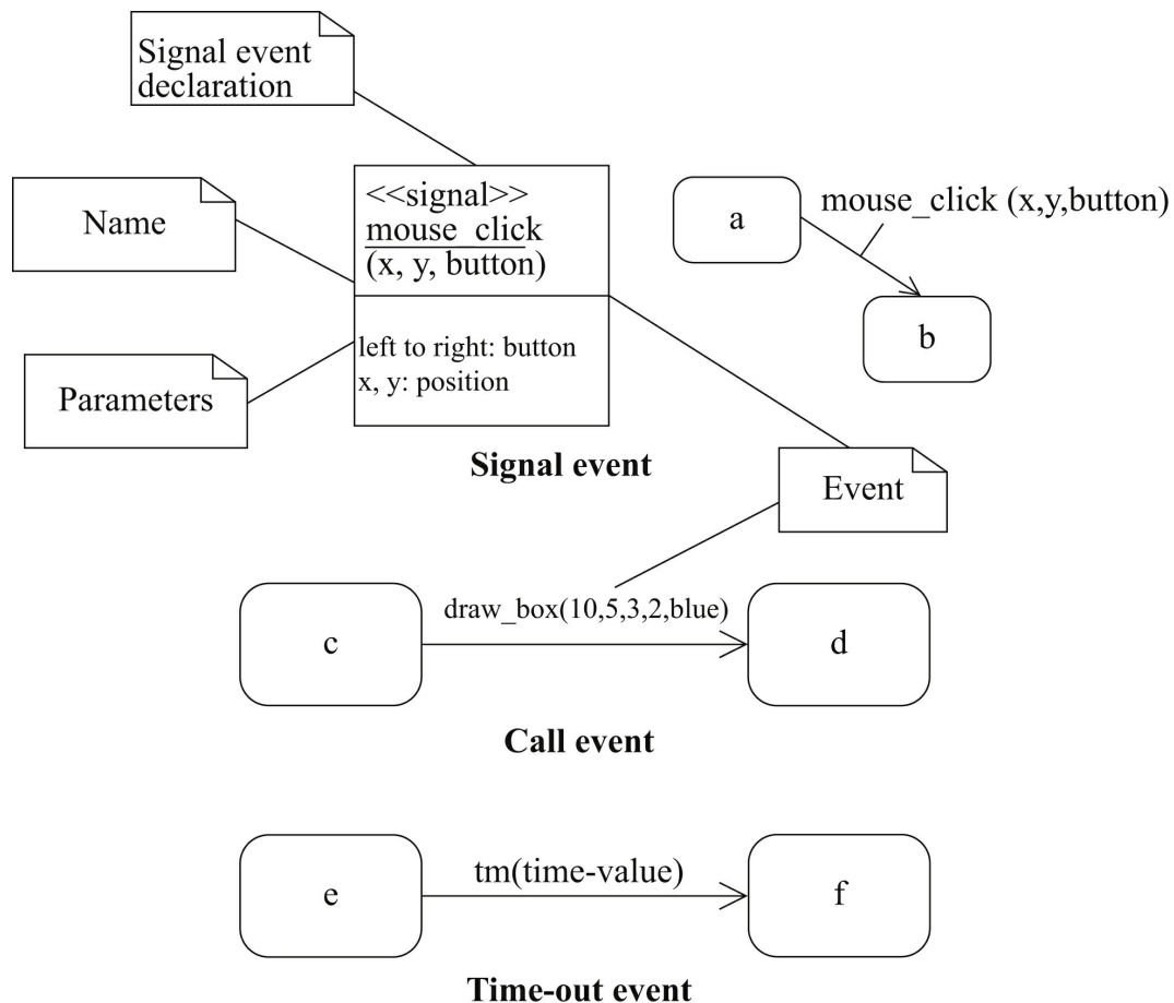
FIGURE 1.12 Signal, call, and time-out events in UML.
