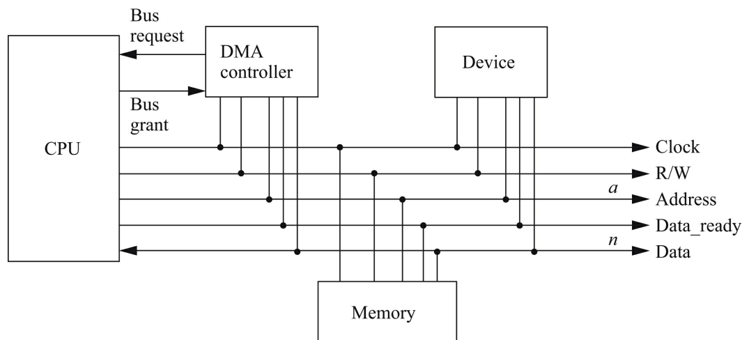
FIGURE 4.11 A bus with a DMA controller.
