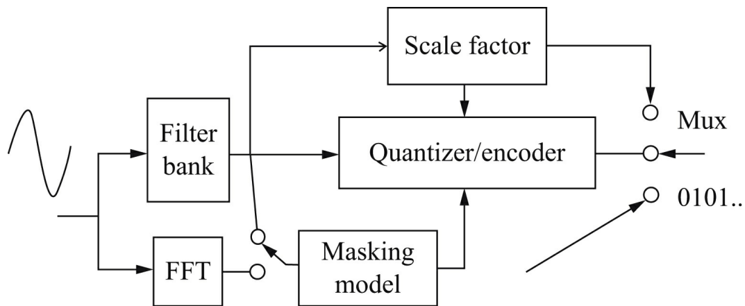
FIGURE 4.41 MPEG Layer 1 encoder.
