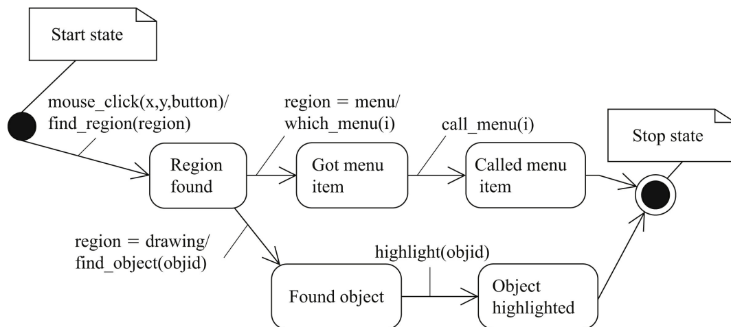
FIGURE 1.13 A state machine specification in UML.
