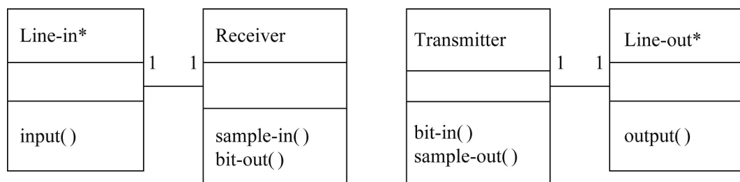
FIGURE 5.32 Class diagram for the modem.
