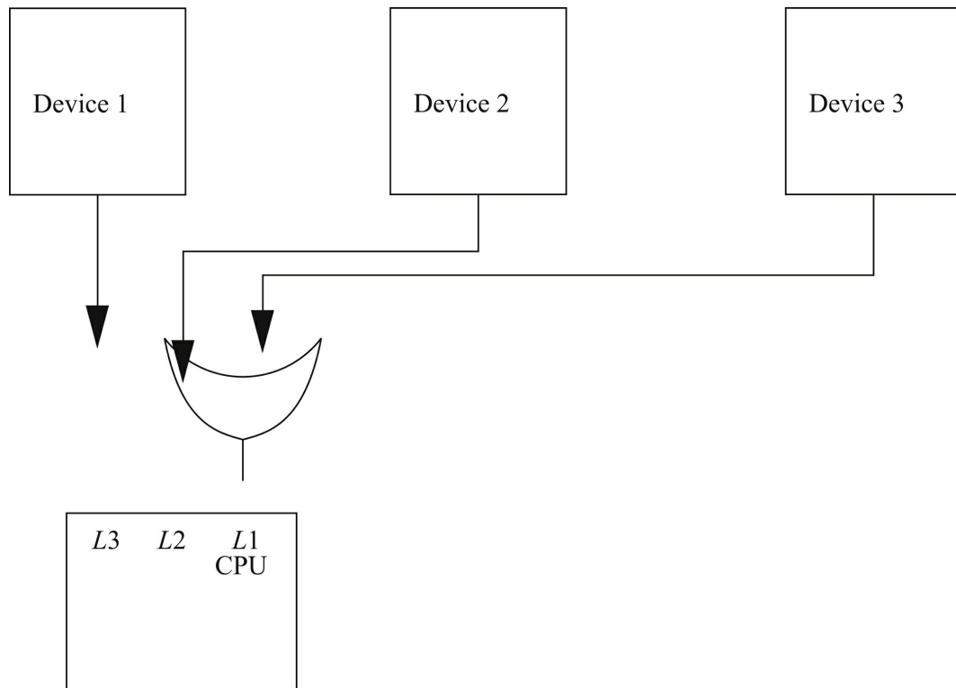
FIGURE 3.4 Using polling to share an interrupt over several devices.
