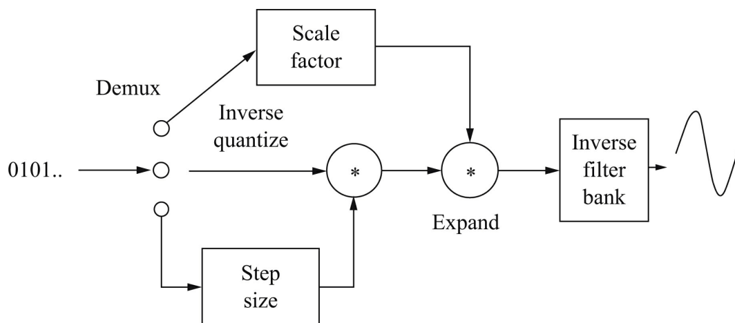
FIGURE 4.43 MPEG Layer 1 decoder.
