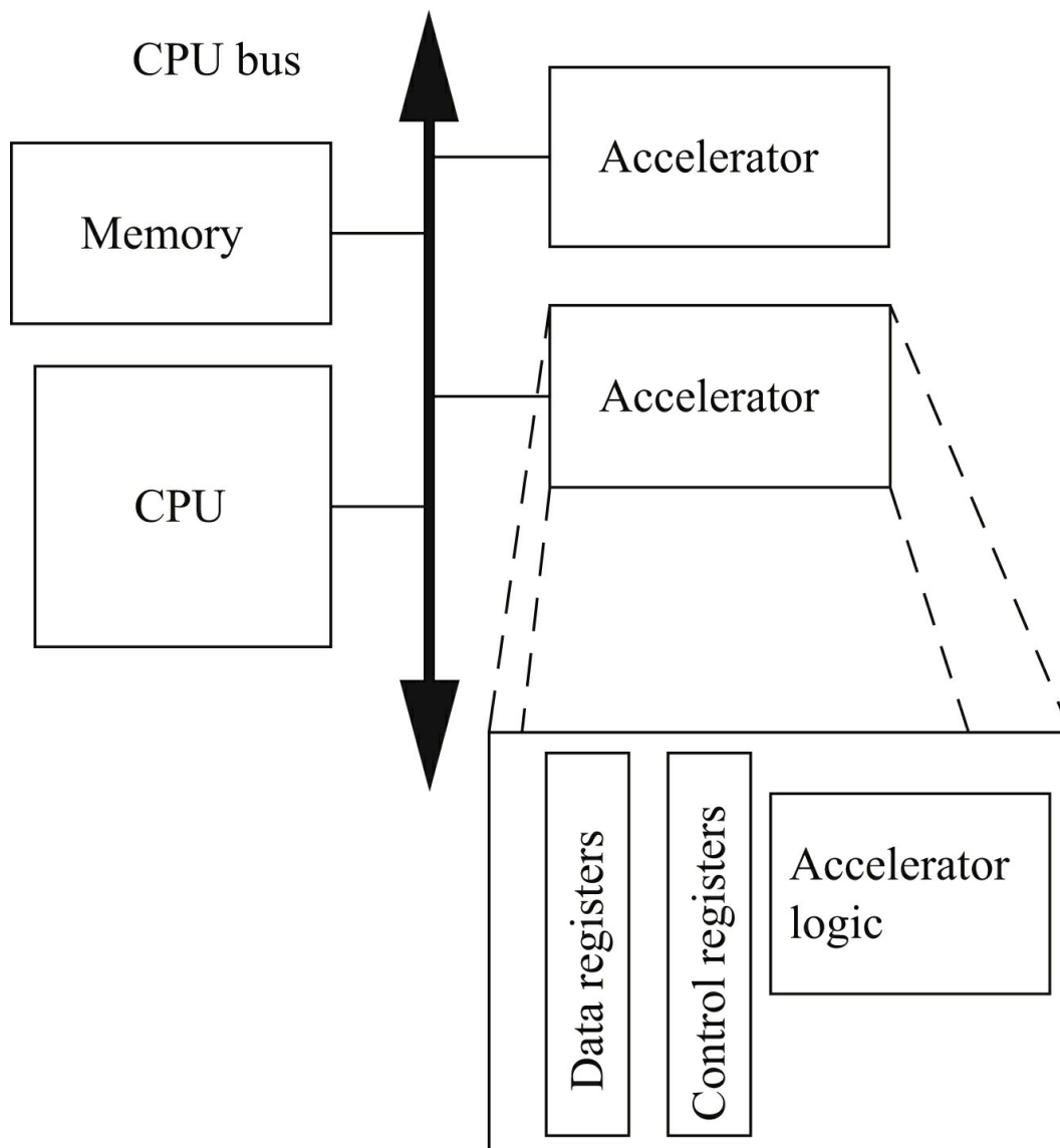
FIGURE 10.4 CPU accelerators in a system.
