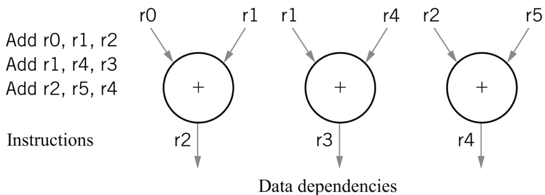
FIGURE 2.6 Instructions without data dependencies.
