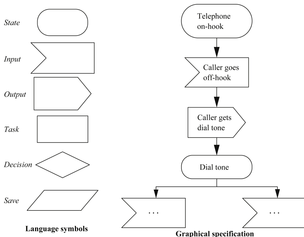
FIGURE 7.6 The SDL specification language.
