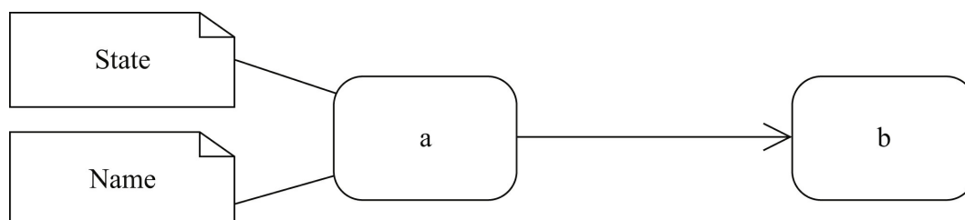
FIGURE 1.10 A state and transition in UML.
