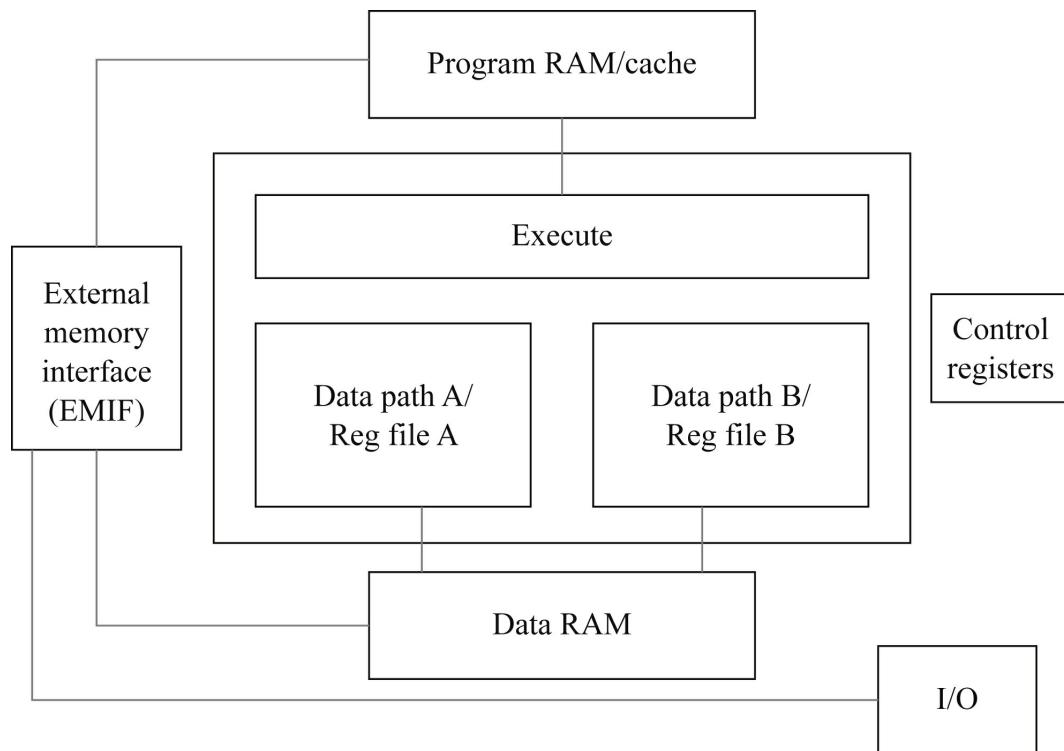
FIGURE 2.24 C64x block diagram.
