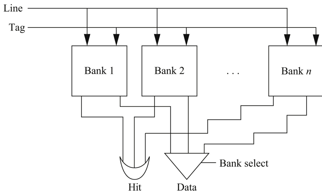
FIGURE 3.9 A set-associative cache.
