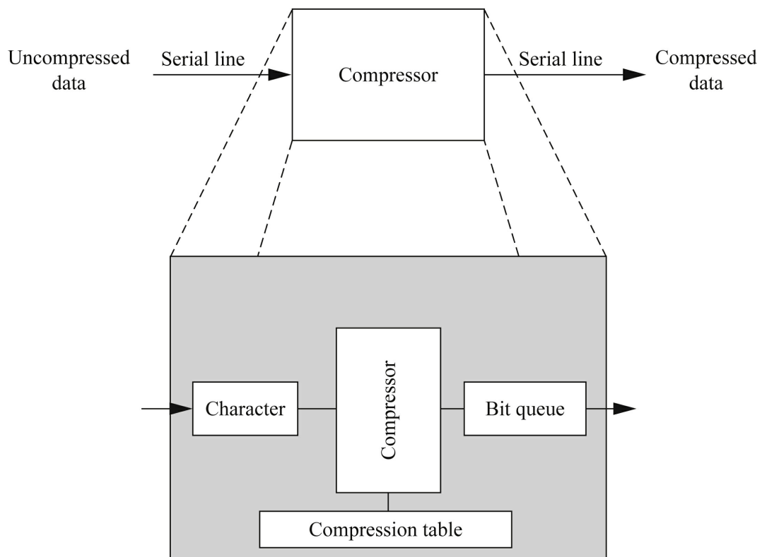
FIGURE 6.2 The compression engine as a multirate system.
