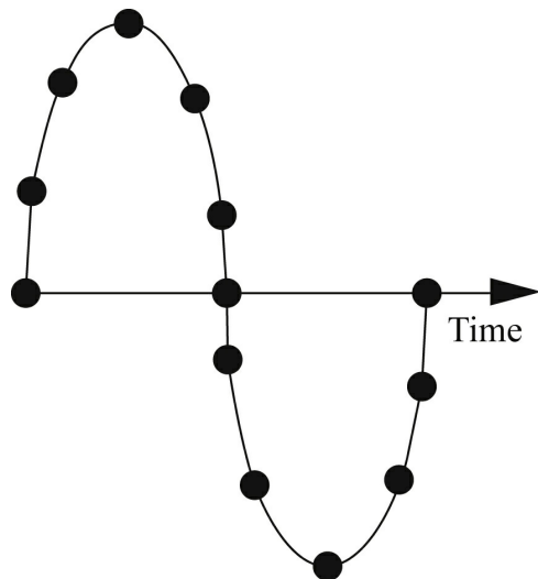
FIGURE 5.33 Waveform generation by table lookup.
