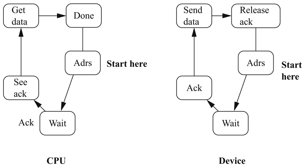
FIGURE 4.10 State diagrams for the bus read transaction.
