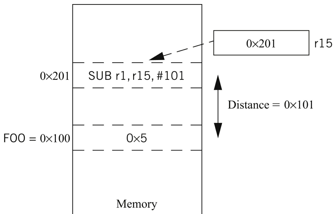
FIGURE 2.15 Computing an absolute address using the PC.
