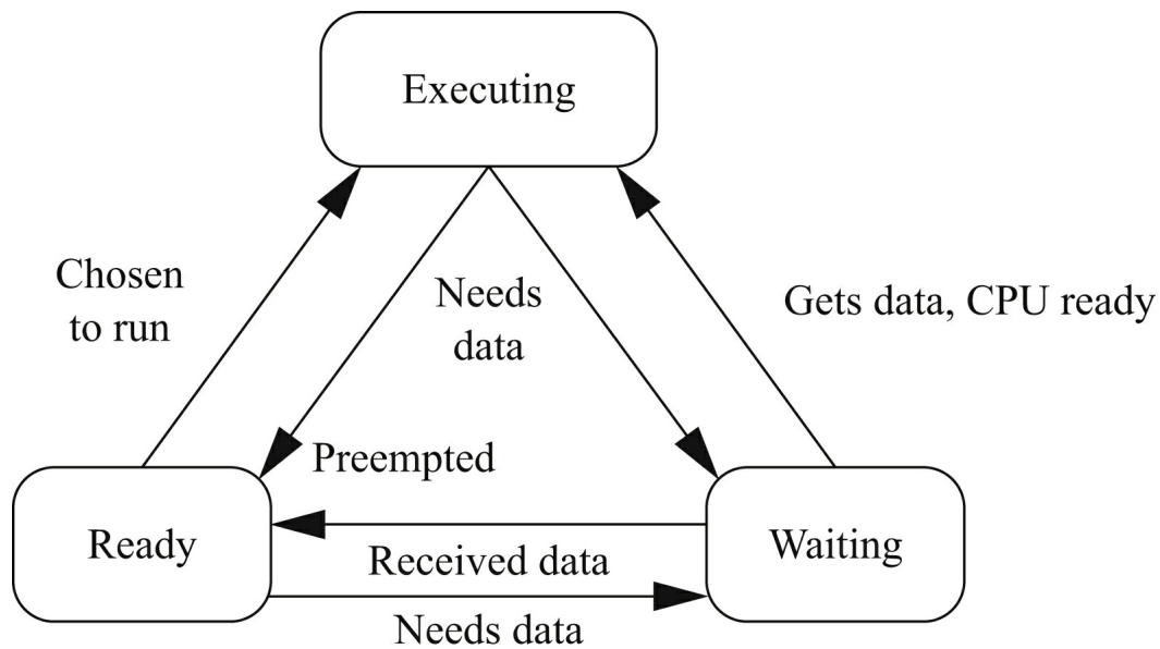
FIGURE 6.7 Scheduling states of a process.
