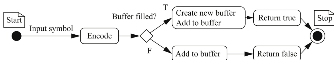
FIGURE 3.24 State diagram for encode behavior.
