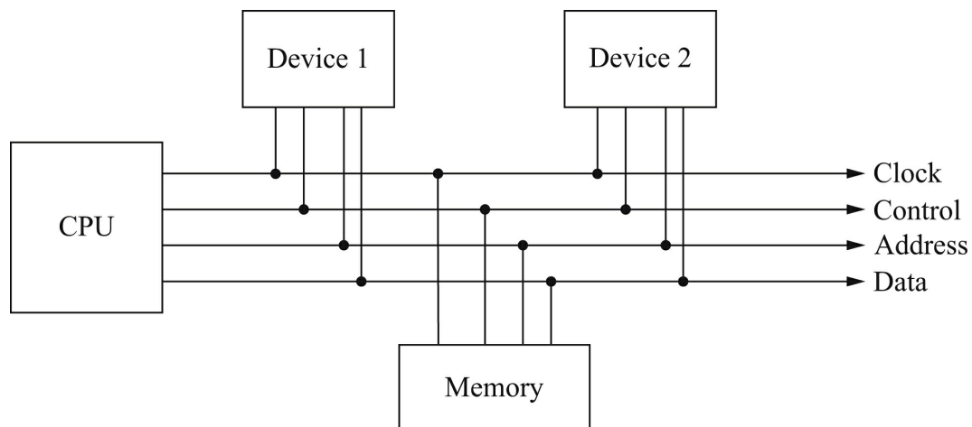
FIGURE 4.3 Organization of a bus.
