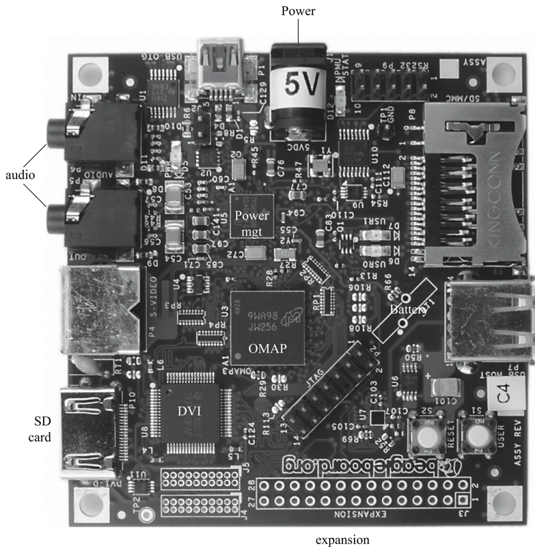
FIGURE 4.21 A BeagleBoard.
