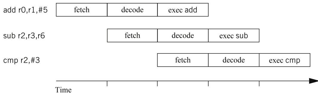
FIGURE 3.16 Pipelined execution of ARM instructions.
