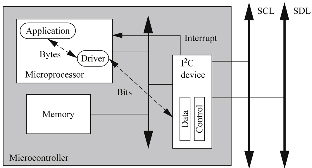
FIGURE 10.16 An I 2 C interface in a microcontroller.
