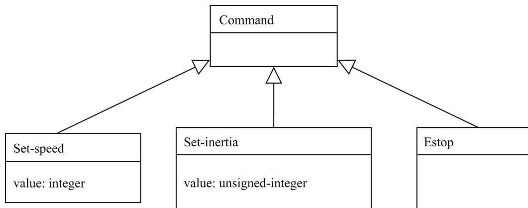
FIGURE 1.17 Class diagram for the train controller commands.
