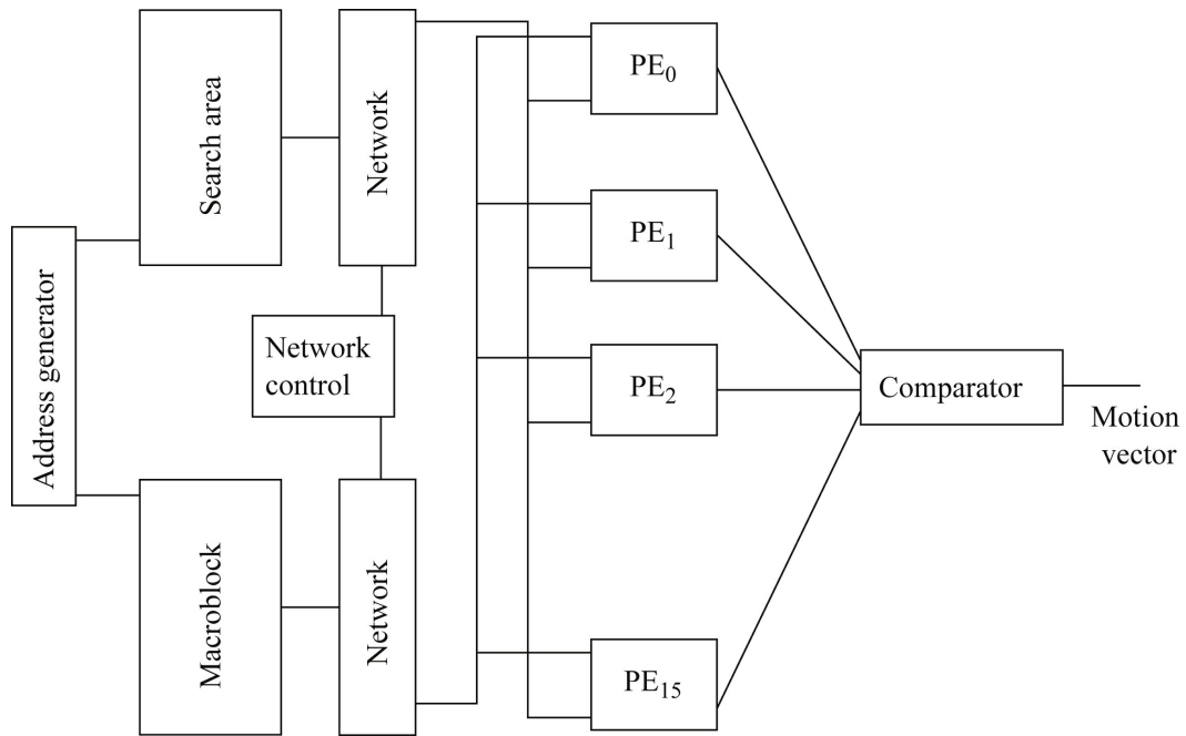
FIGURE 10.23 An architecture for the motion estimation accelerator [Dut96].
