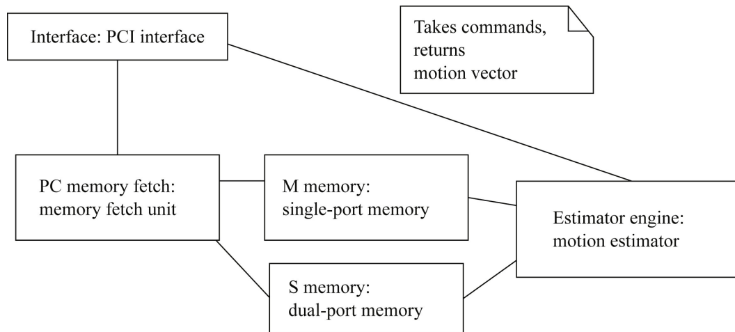
FIGURE 10.25 Object diagram for the video accelerator.
