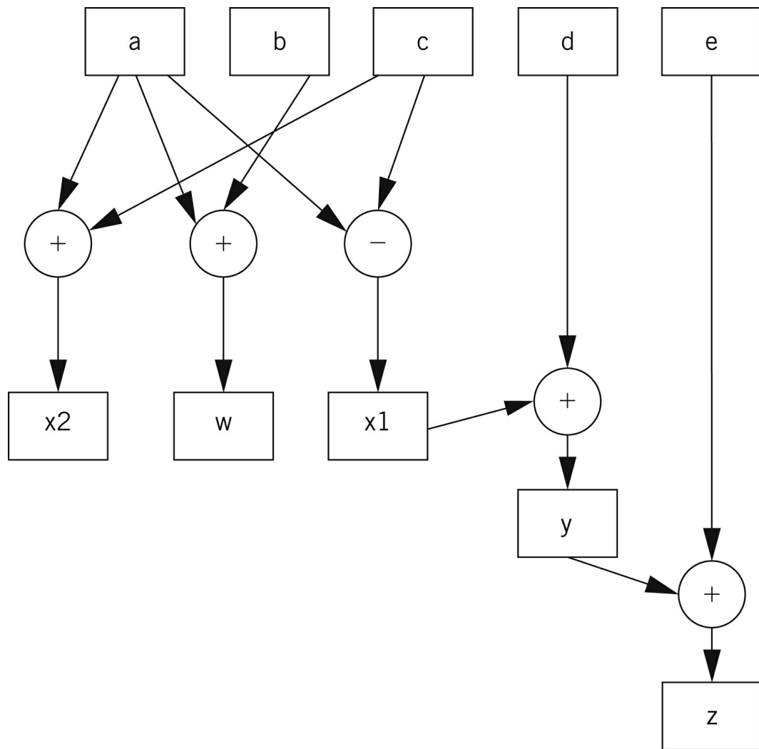
FIGURE 5.6 An extended data flow graph for our sample basic block.
