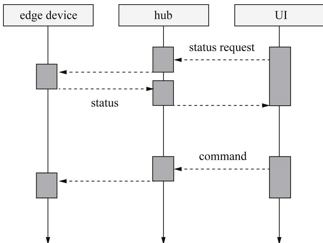
FIGURE 8.1 Use case for an IoT smart appliance.
