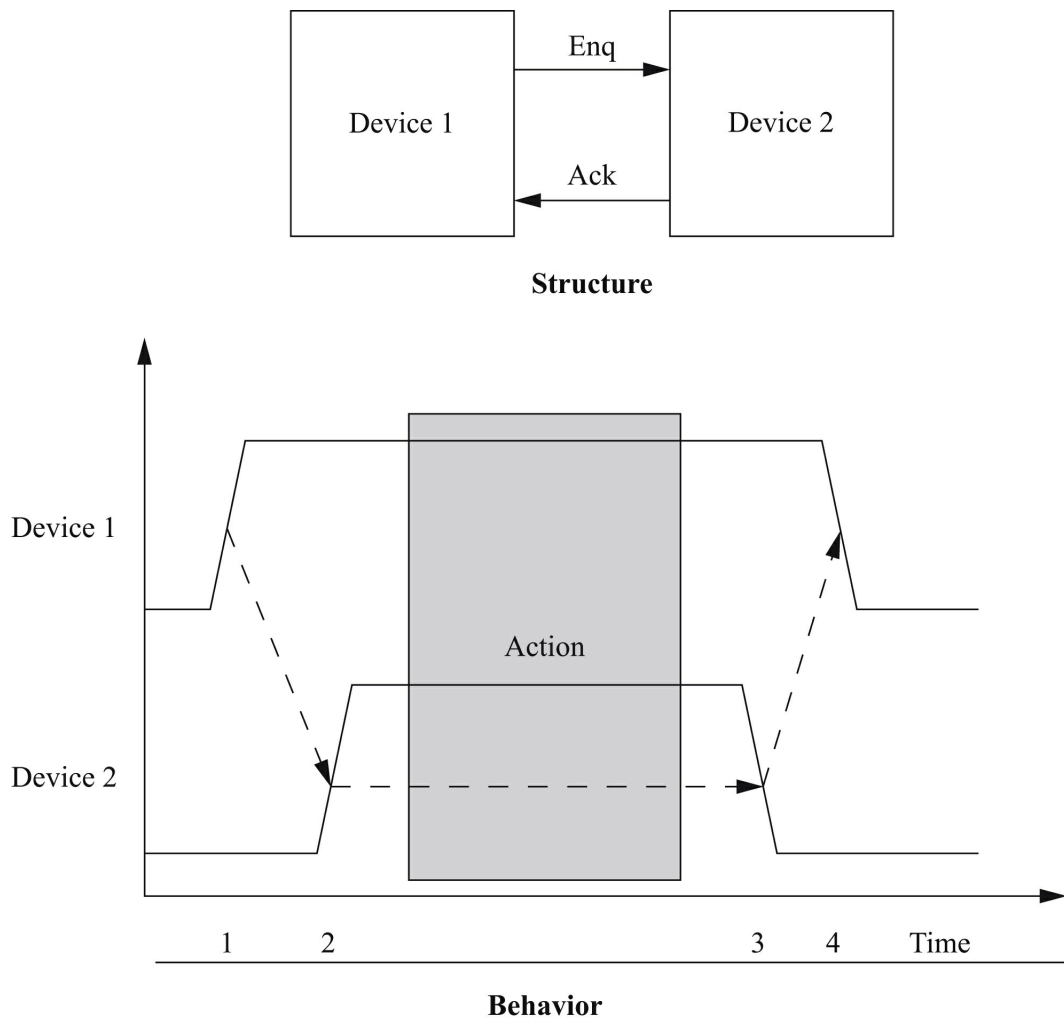
FIGURE 4.4 The four-cycle handshake.
