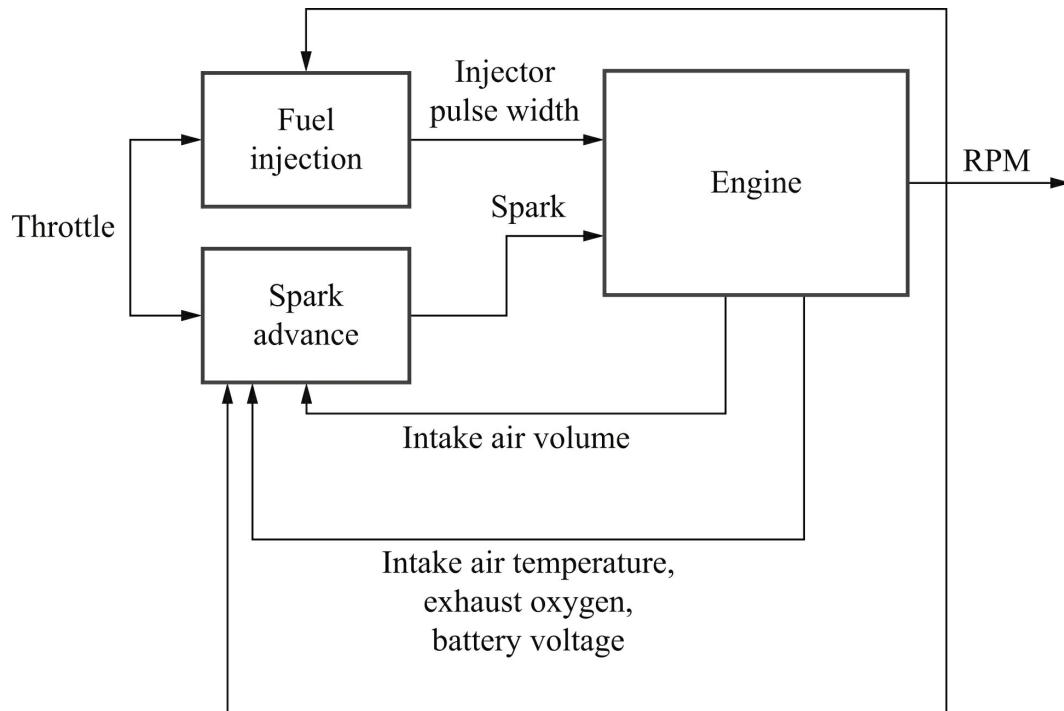
FIGURE 6.28 Engine block diagram.
