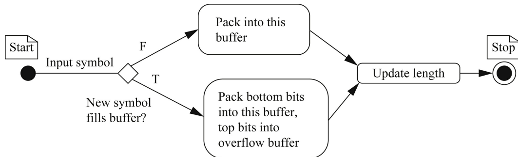
FIGURE 3.25 State diagram for insert behavior.
