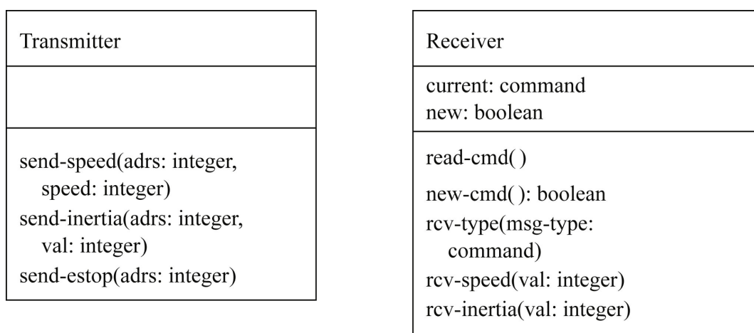
FIGURE 1.24 Class diagram for the Transmitter and Receiver .
