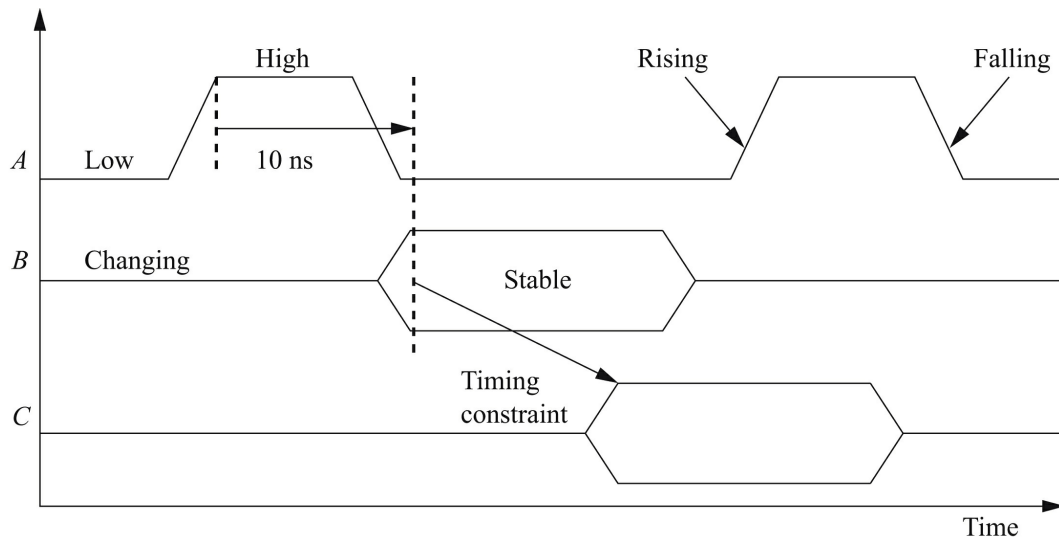
FIGURE 4.6 Timing diagram notation.
