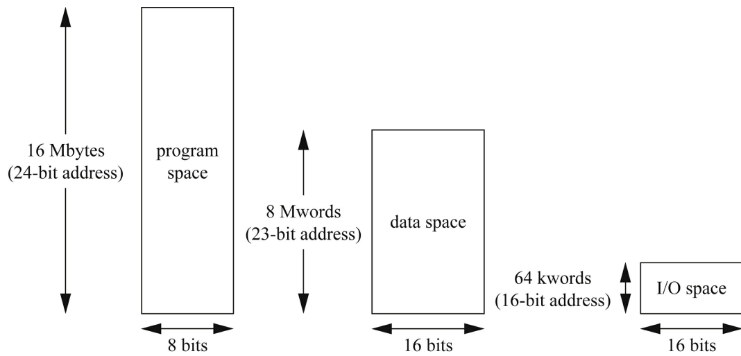
FIGURE 2.22 Address spaces in the TMS320C55x.
