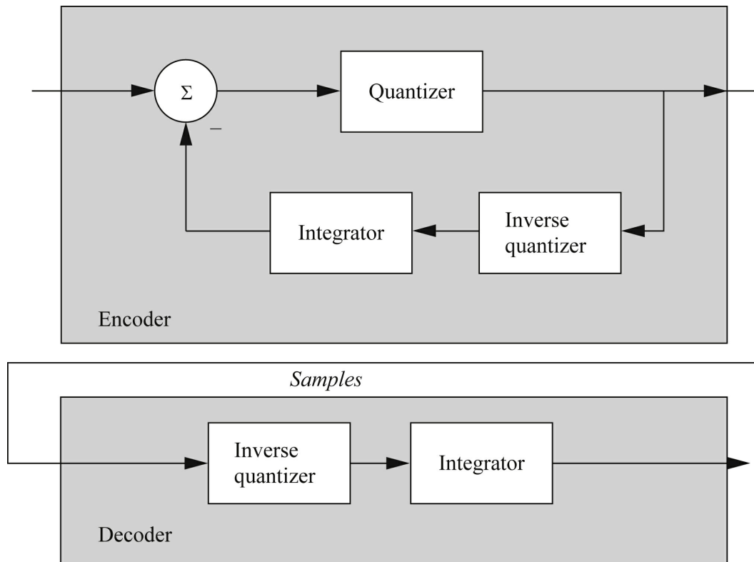
FIGURE 6.20 An ADPCM compression system.
