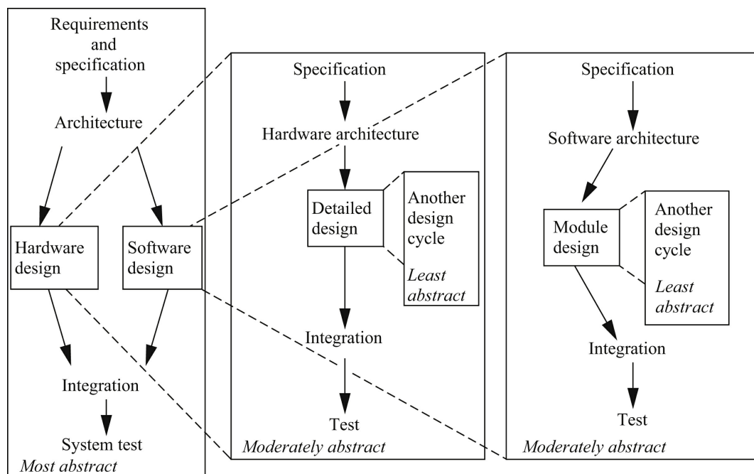
FIGURE 7.5 A hierarchical design flow for an embedded system.
