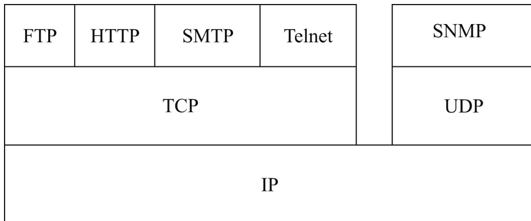
FIGURE 8.7 The Internet service stack.
