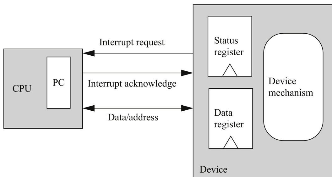
FIGURE 3.2 The interrupt mechanism.
