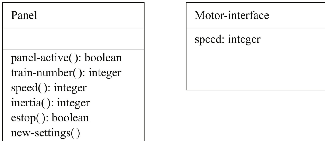
FIGURE 1.23 Class diagram for the panel and motor interface.
