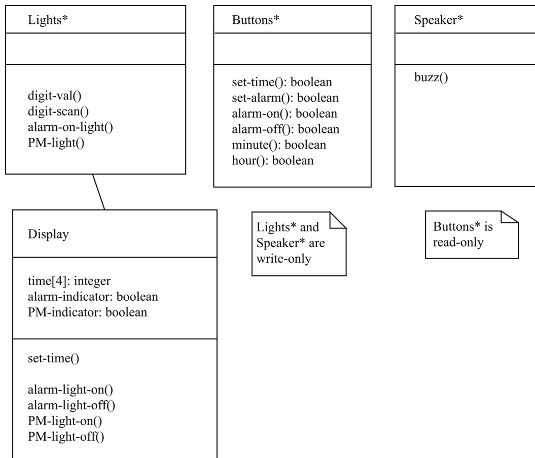
FIGURE 4.36 Details of user interface classes for the alarm clock.
