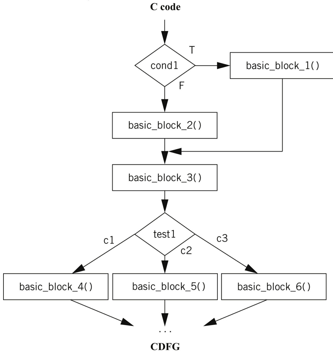
FIGURE 5.8 C code and its CDFG.
