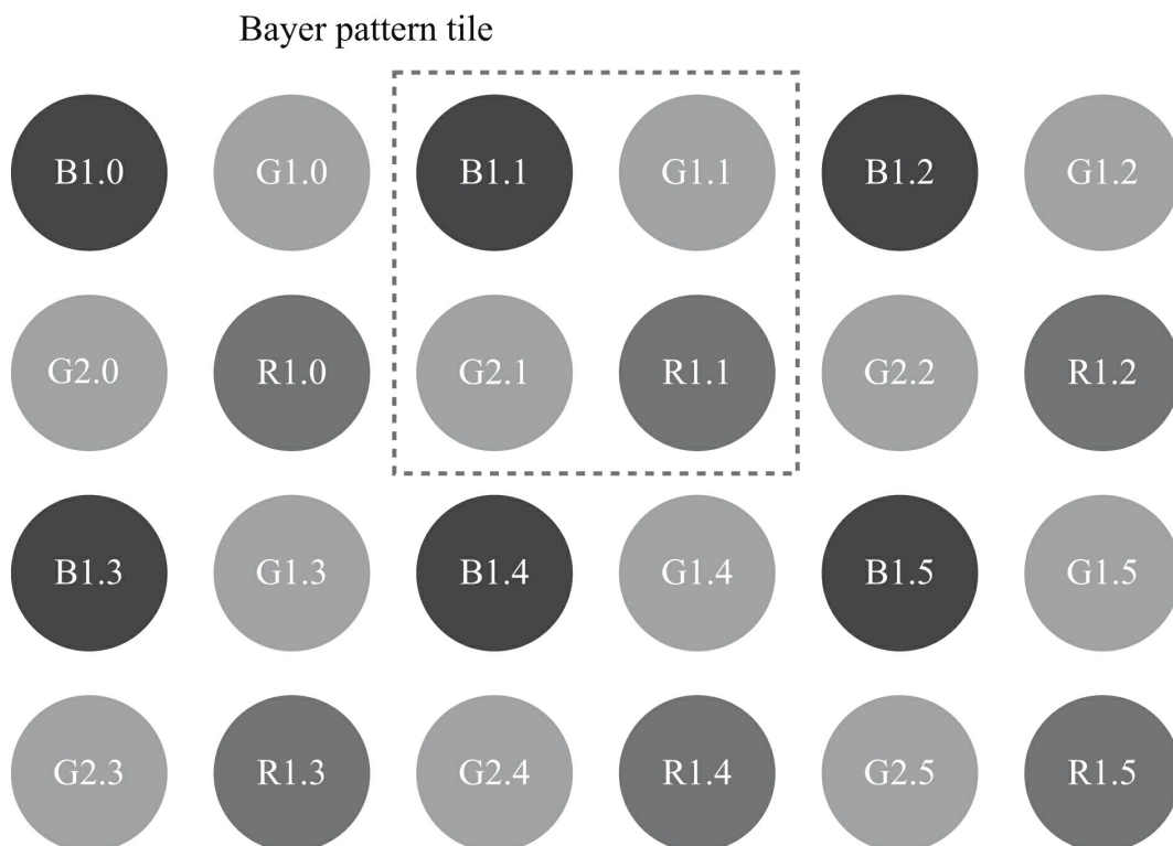
FIGURE 5.34 A color filter array arranged in a Bayer pattern.
