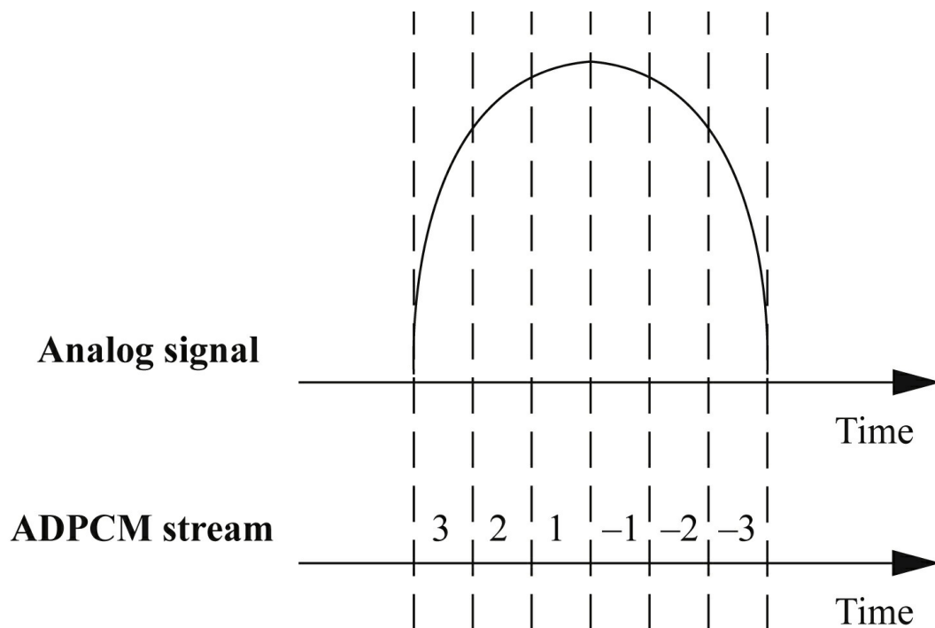
FIGURE 6.19 The ADPCM coding scheme.
