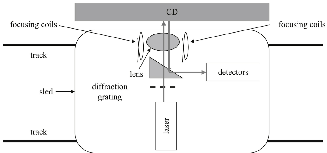
FIGURE 10.28 A compact disk mechanism.
