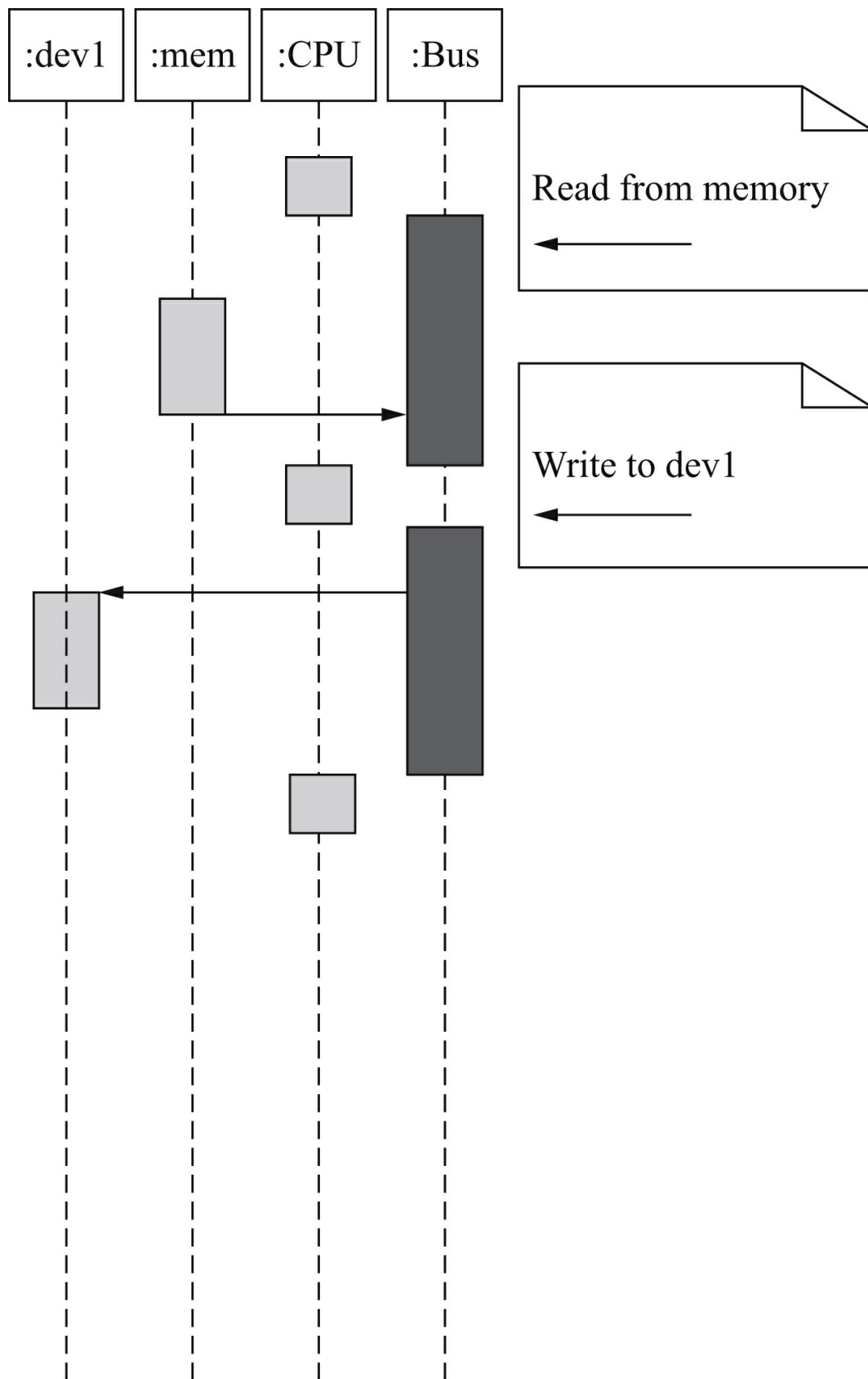
FIGURE 4.5 A typical sequence diagram for bus operations.
