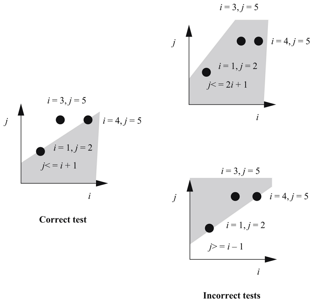
FIGURE 5.26 Domain testing for a pair of values.
