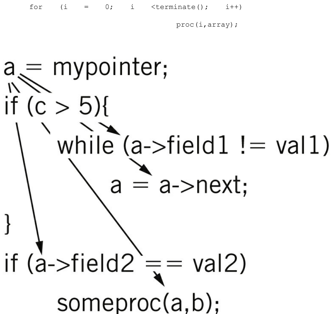
FIGURE 5.27 Definitions and uses of variables.
