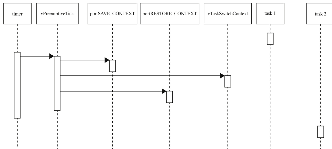
FIGURE 6.9 Sequence diagram for a FreeRTOS.org context switch.
