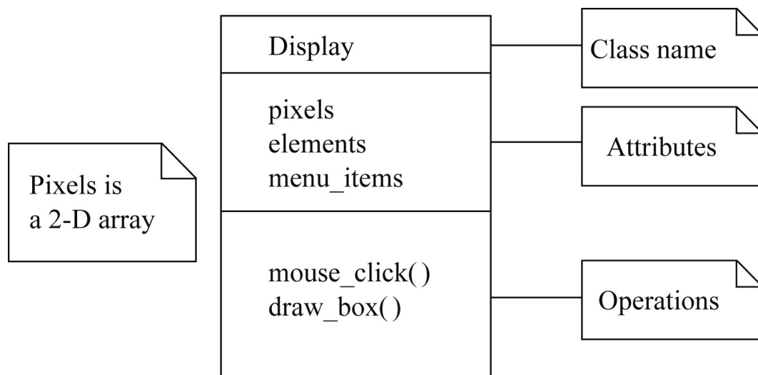
FIGURE 1.6 A class in UML notation.
