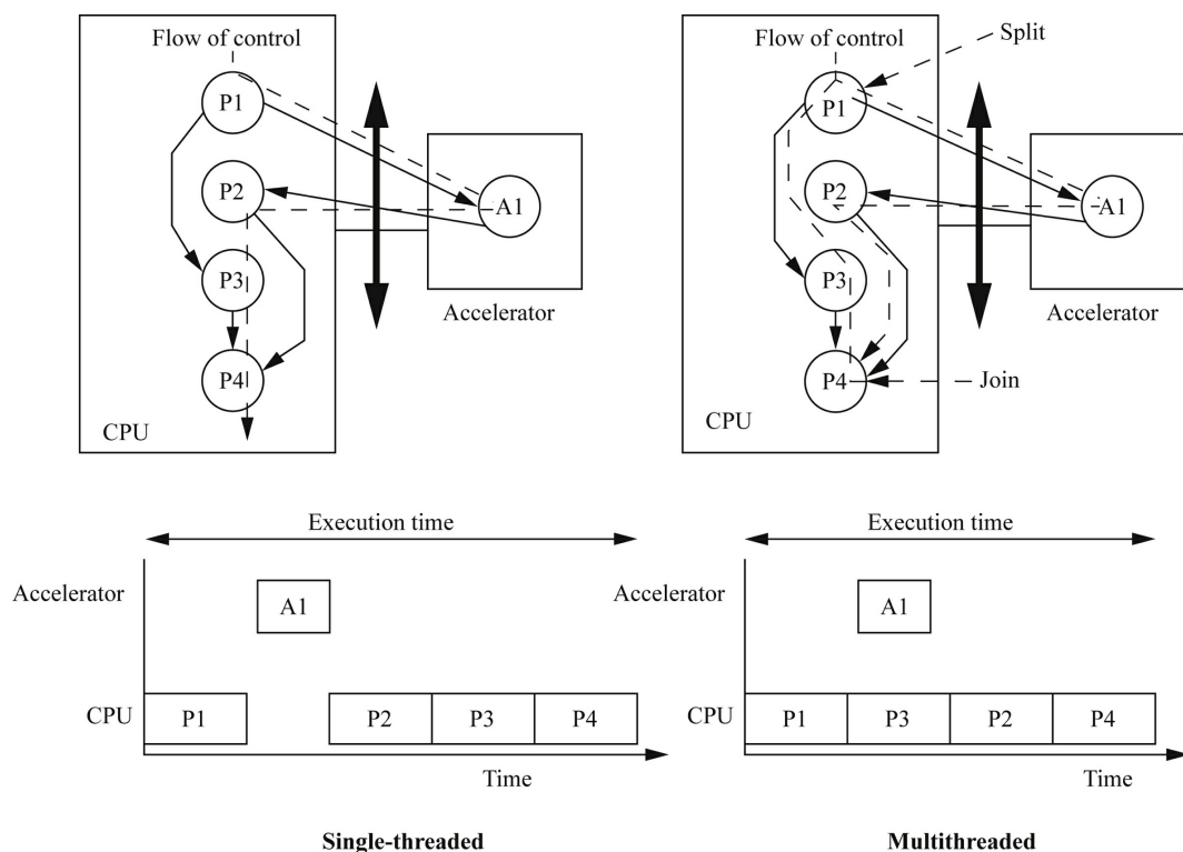
FIGURE 10.5 Single-threaded versus multithreaded control of an accelerator.
