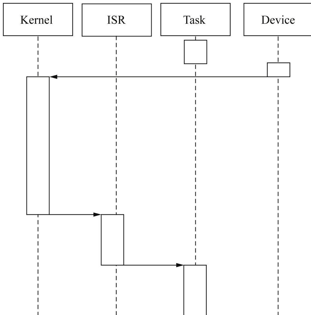
FIGURE 6.17 Sequence diagram for RTOS interrupt latency.
