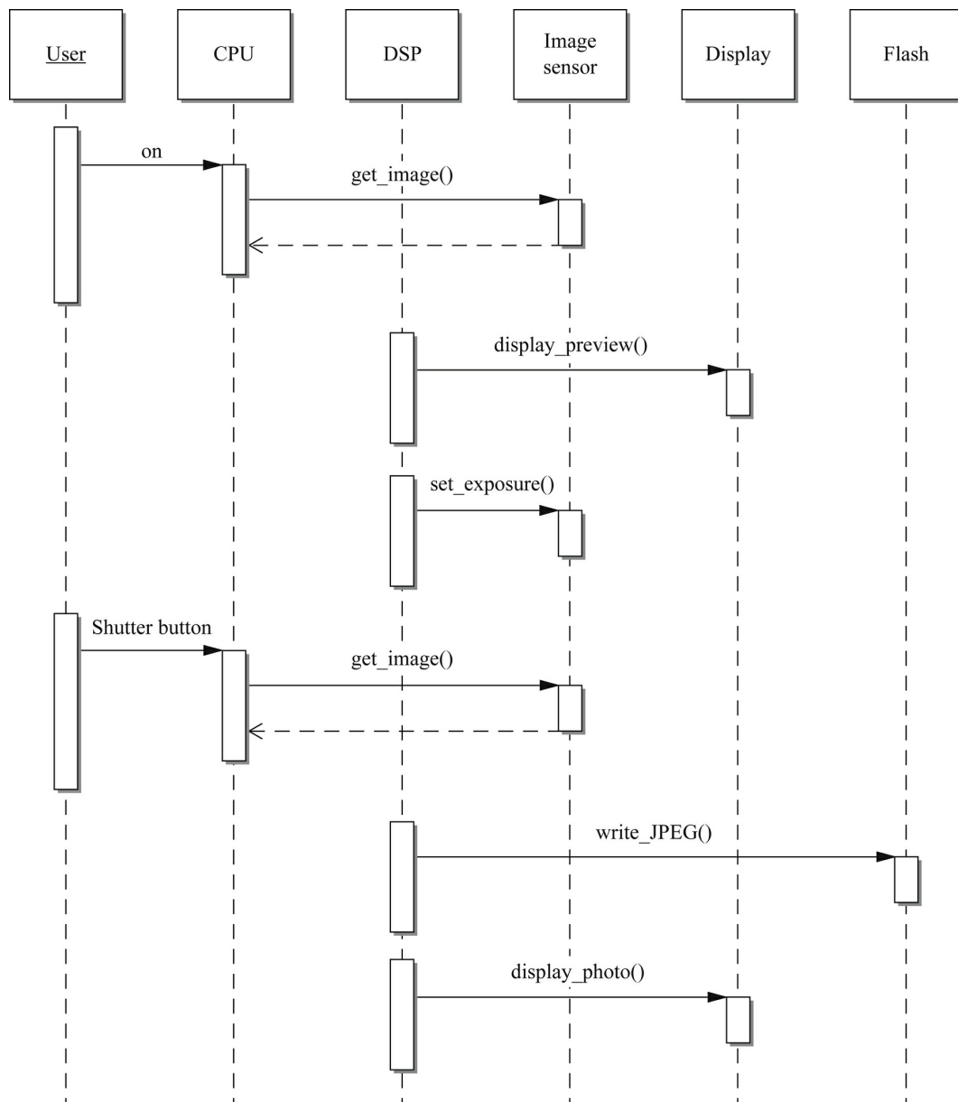
FIGURE 5.43 Sequence diagram for taking a picture with a digital still camera.
