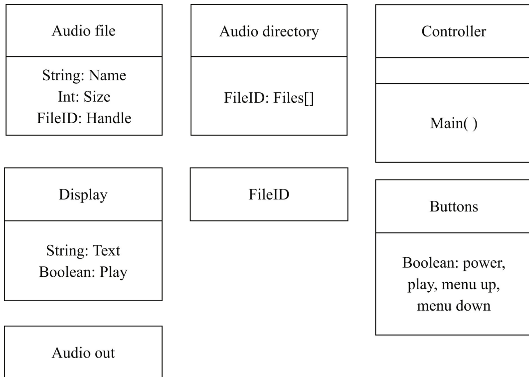
FIGURE 4.44 Classes in the audio player.
