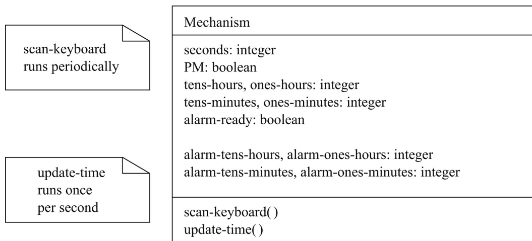
FIGURE 4.37 The Mechanism class.
