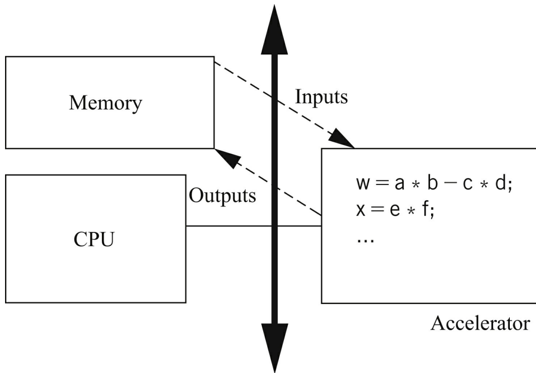
FIGURE 10.6 Components of execution time for an accelerator.
