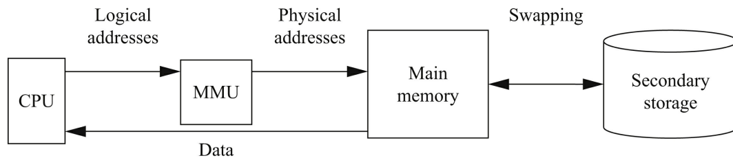
FIGURE 3.10 A virtually addressed memory system.
