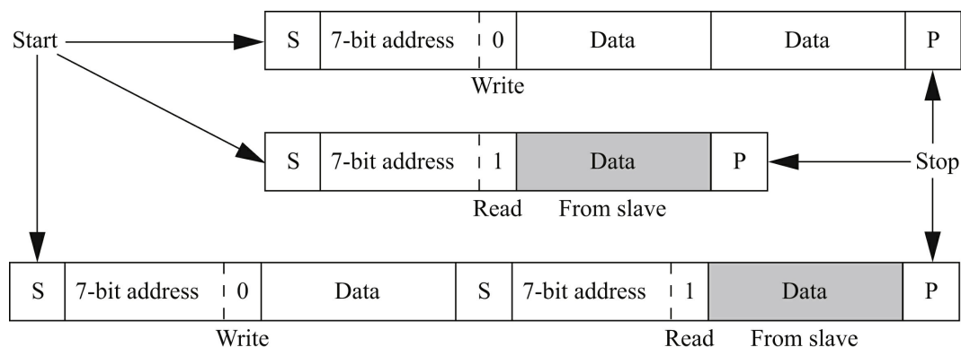
FIGURE 10.14 Typical bus transactions on the I 2 C bus.
