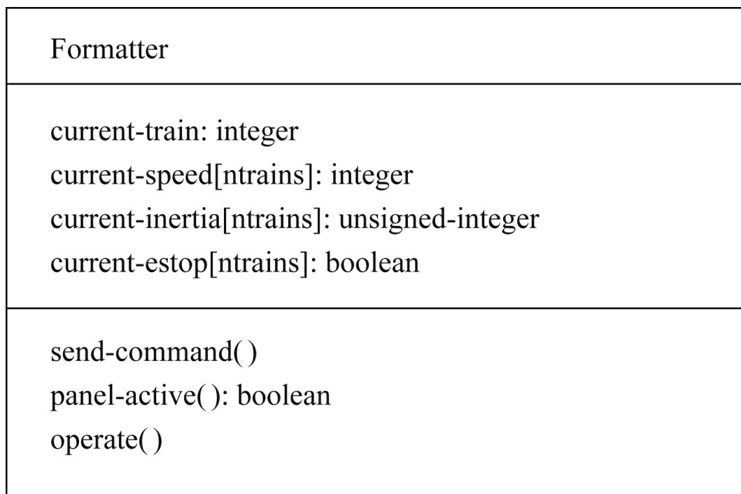
FIGURE 1.25 Class diagram for the Formatter class.
