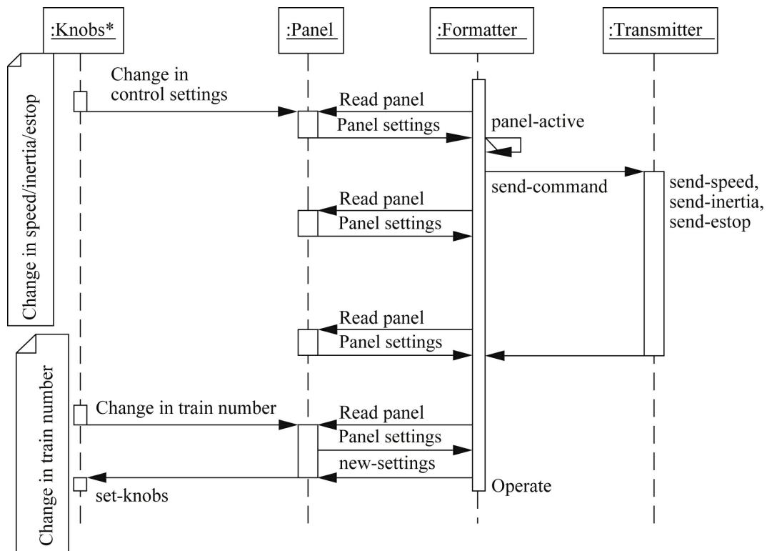
FIGURE 1.26 Sequence diagram for transmitting a control input.
