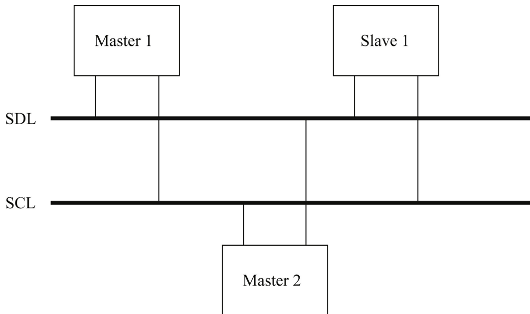
FIGURE 10.10 Structure of an I 2 C bus system.
