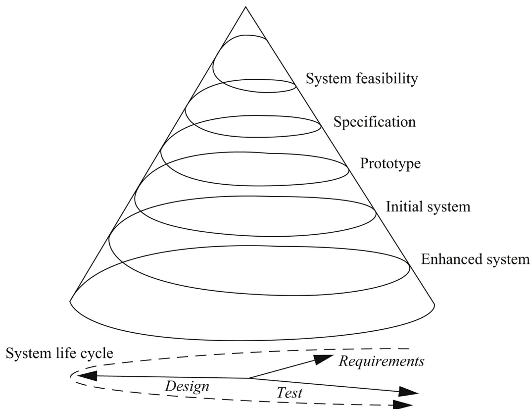
FIGURE 7.2 The spiral model of software design.
