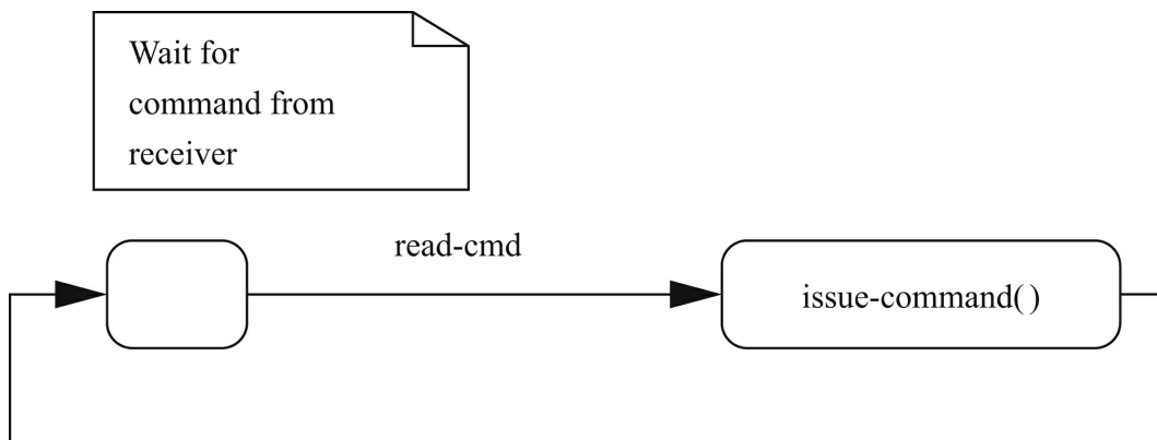
FIGURE 1.30 State diagram for the Controller operate behavior.
