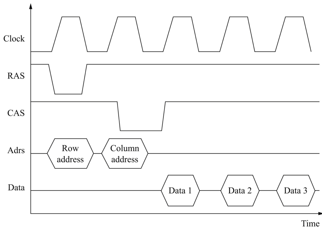
FIGURE 4.18 An SDRAM read operation.
