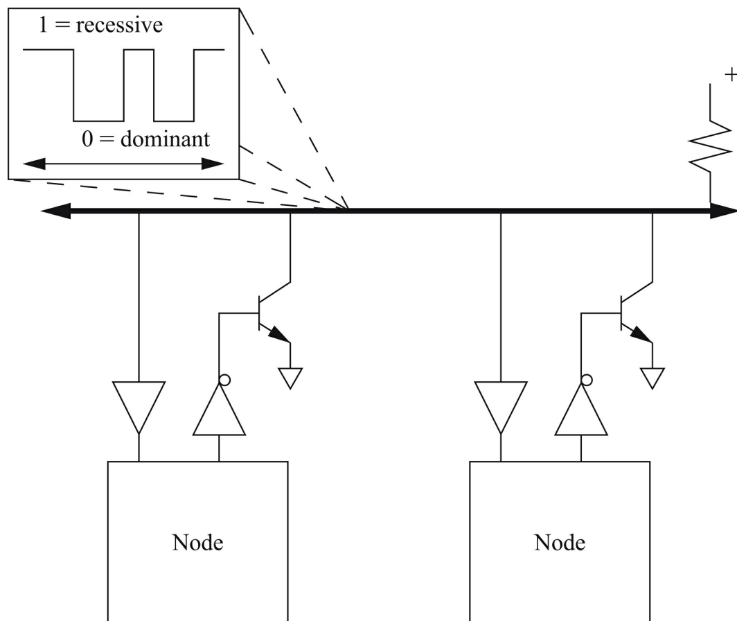
FIGURE 9.2 Physical and electrical organization of a CAN bus.
