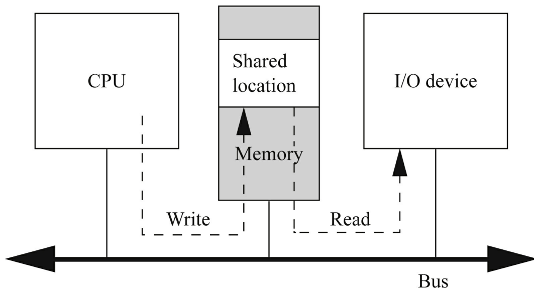
FIGURE 6.14 Shared memory communication implemented on a bus.
