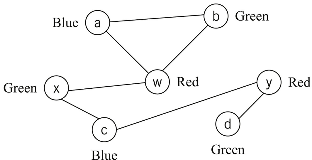
FIGURE 5.17 Using graph coloring to solve the problem of Example 5.5.
