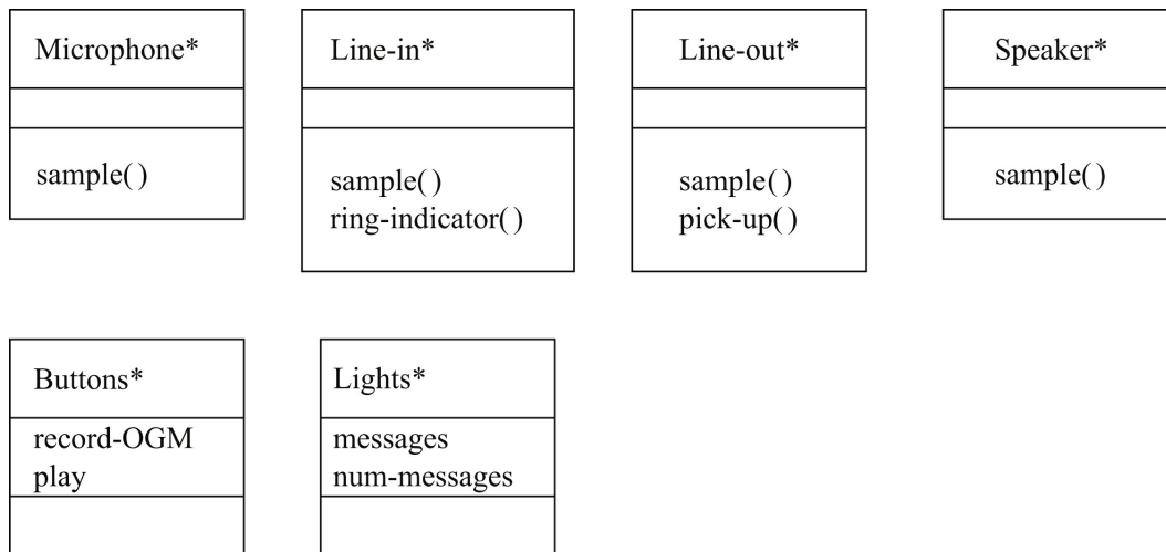
FIGURE 6.22 Physical class interfaces for the answering machine.
