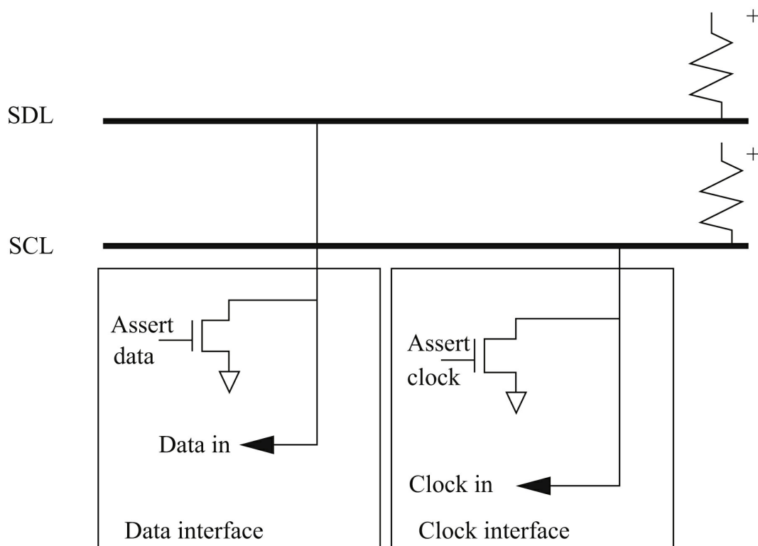
FIGURE 10.11 Electrical interface to the I 2 C bus.
