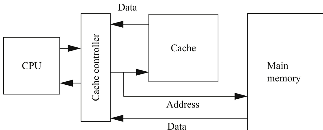
FIGURE 3.6 The cache in the memory system.
