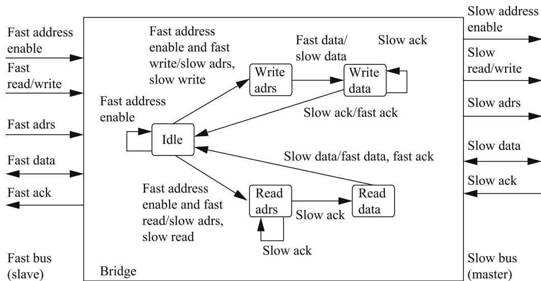
FIGURE 4.15 UML state diagram of bus bridge operation.
