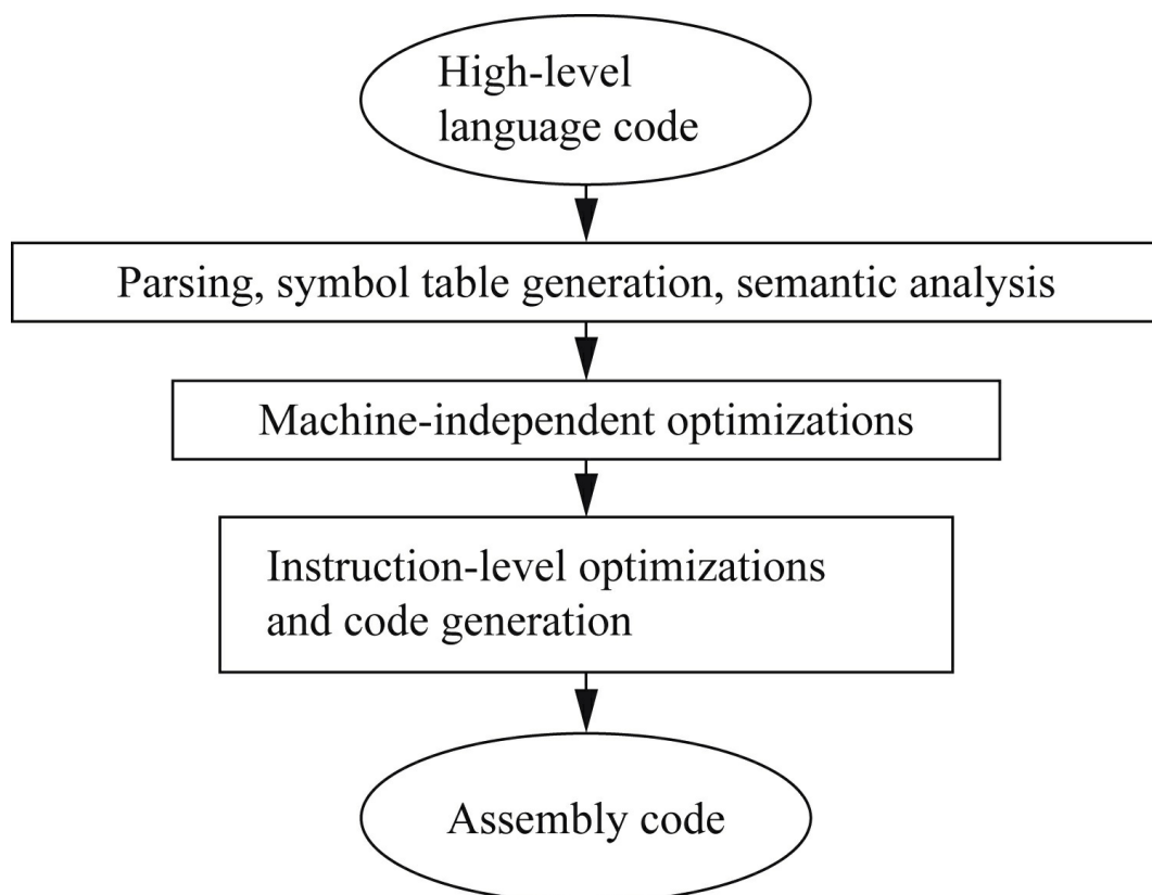
FIGURE 5.13 The compilation process.
