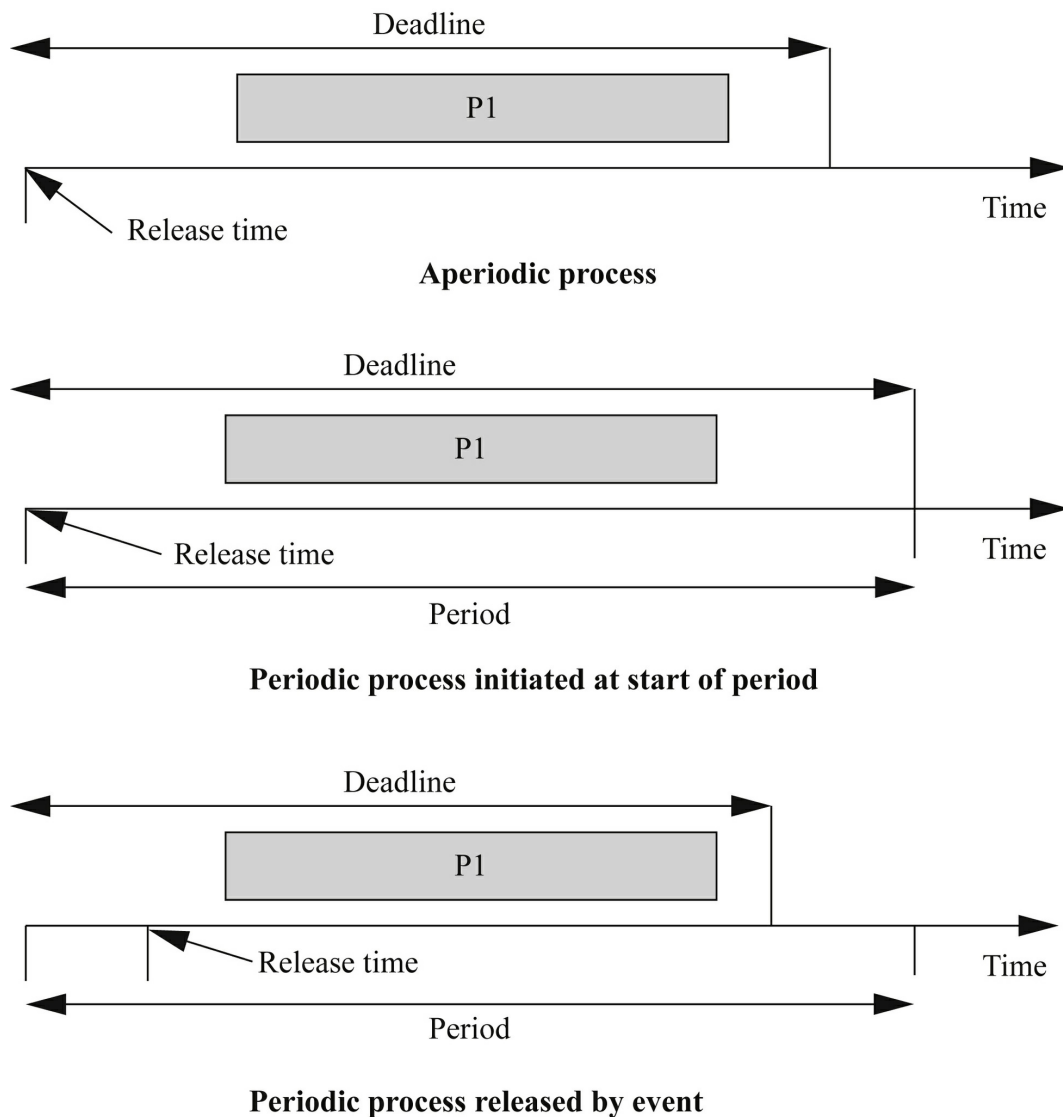
FIGURE 6.3 Example definitions of initiation times and deadlines.
