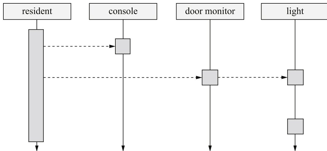
FIGURE 8.18 Light activation in the smart home.
