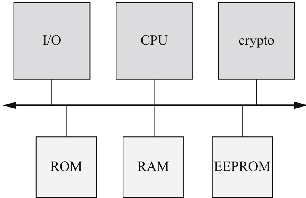
FIGURE 3.19 Architecture of a typical smart card.
