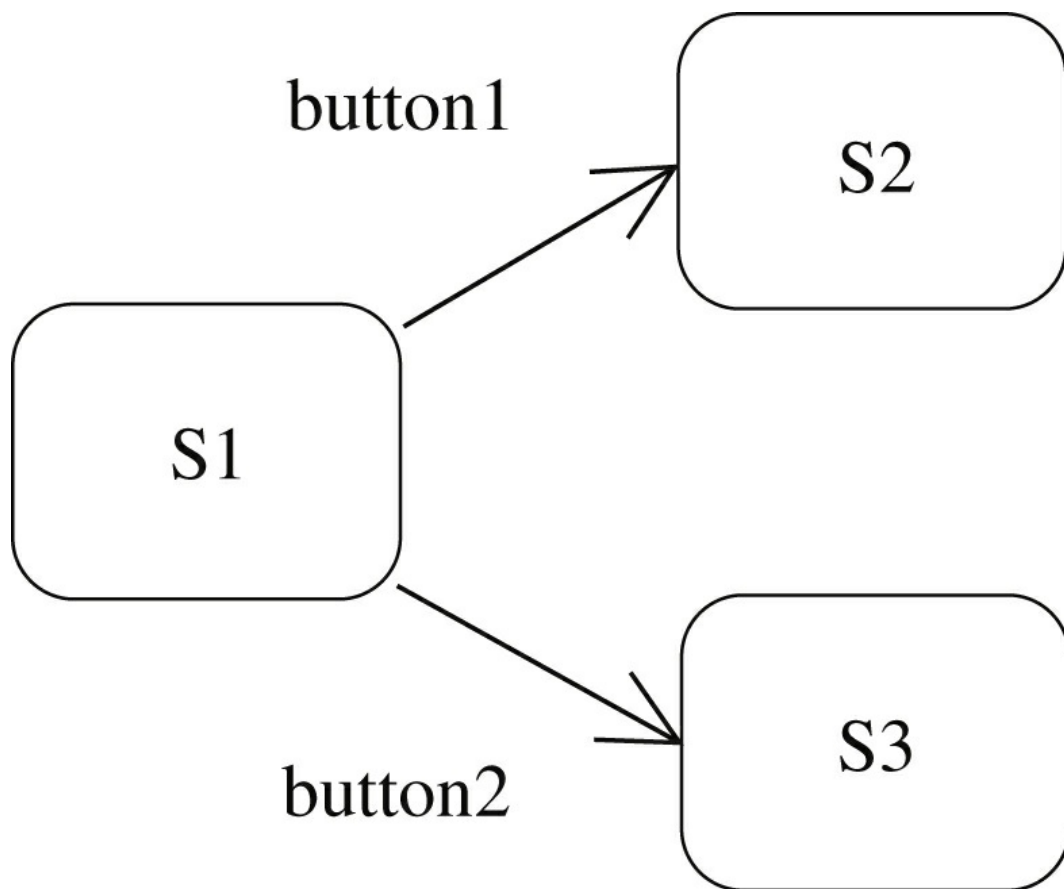
FIGURE 1.11 Event-driven events in UML state machines.
