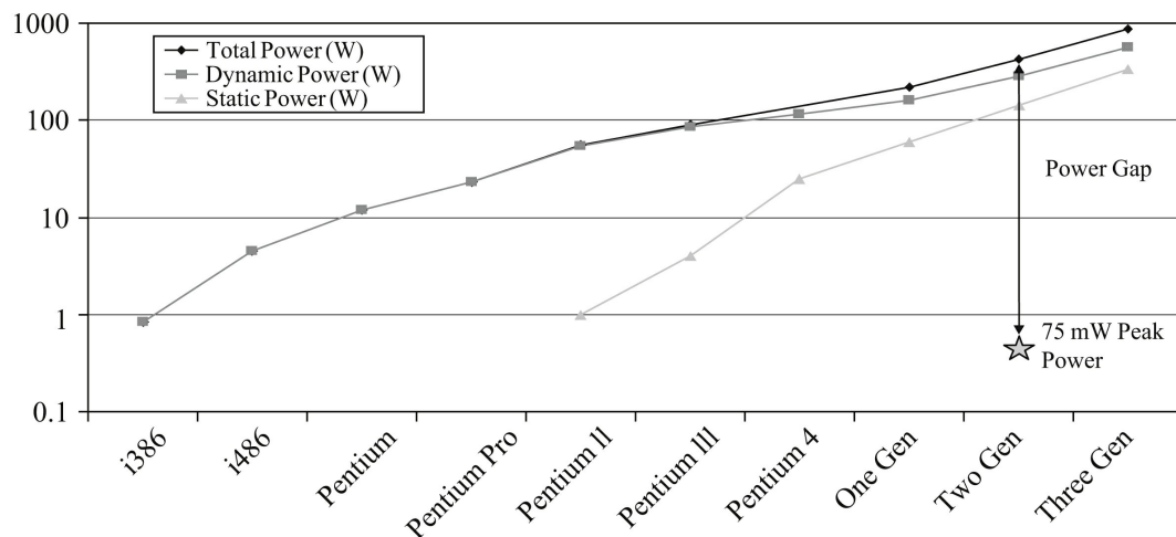
FIGURE 10.2 Power consumption trends for desktop processors [Aus04]. Copyright 2004 IEEE Computer Society.
