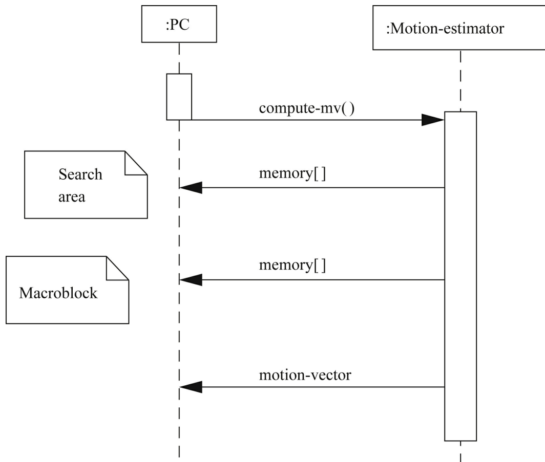
FIGURE 10.22 Sequence diagram for the video accelerator.
