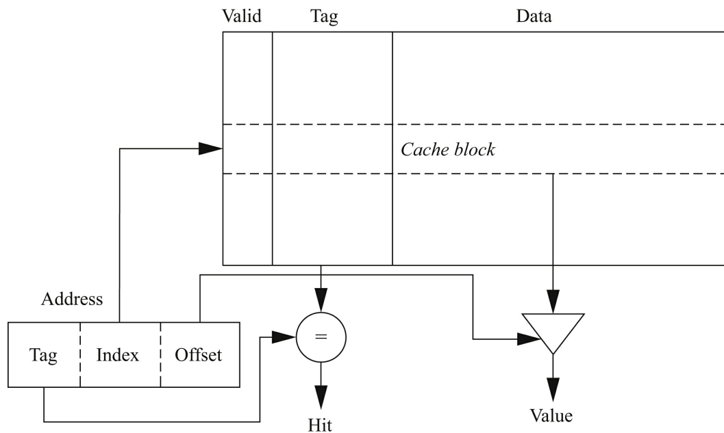
FIGURE 3.8 A direct-mapped cache.
