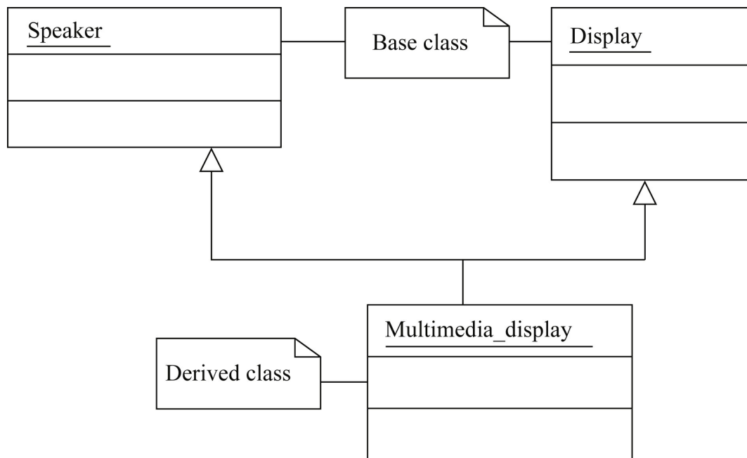
FIGURE 1.8 Multiple inheritance in UML.
