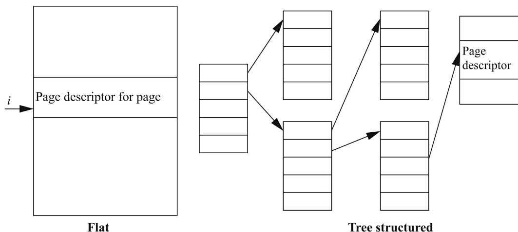
FIGURE 3.14 Alternative schemes for organizing page tables.
