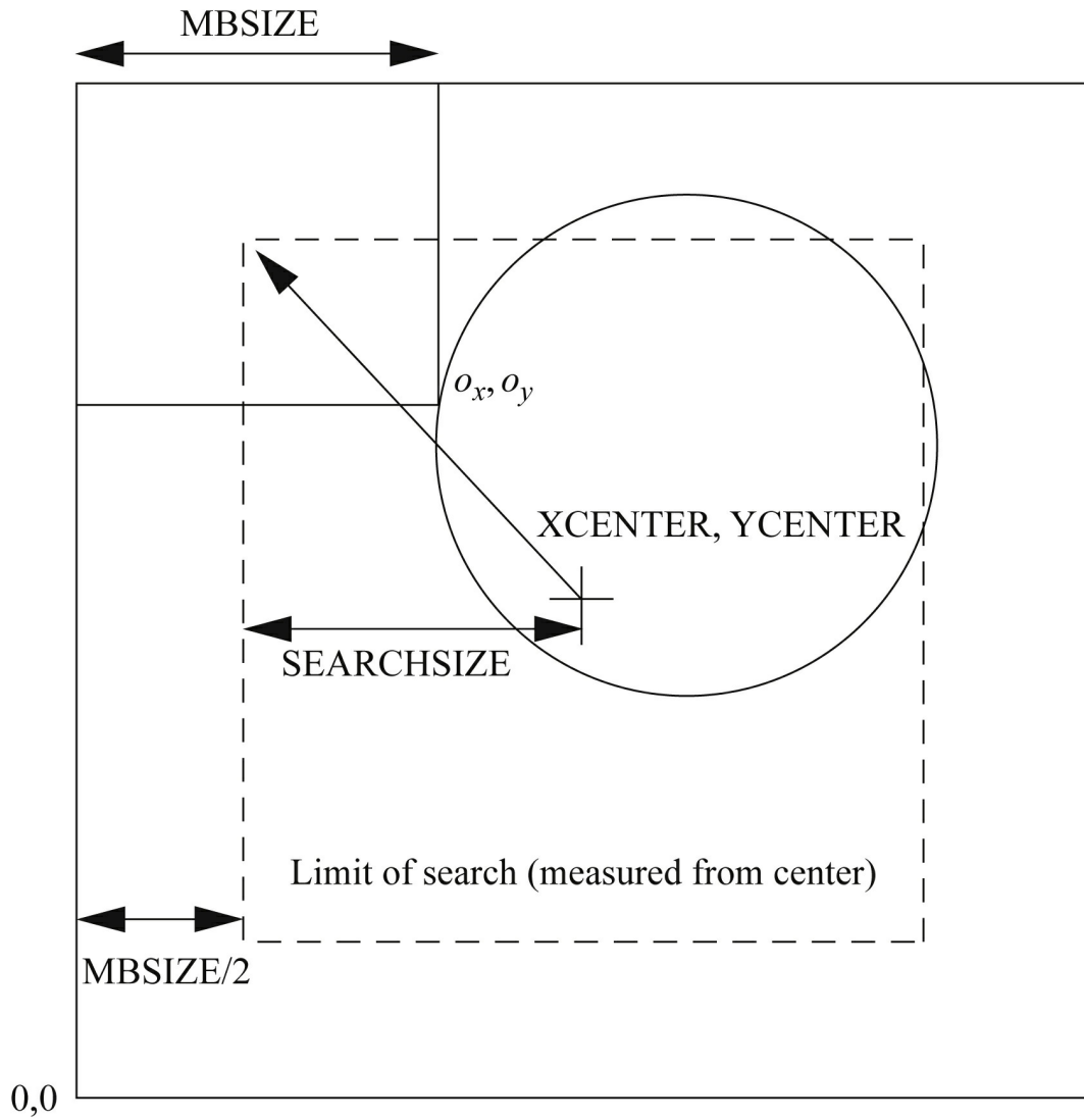
FIGURE 10.19 Block motion search parameters.
