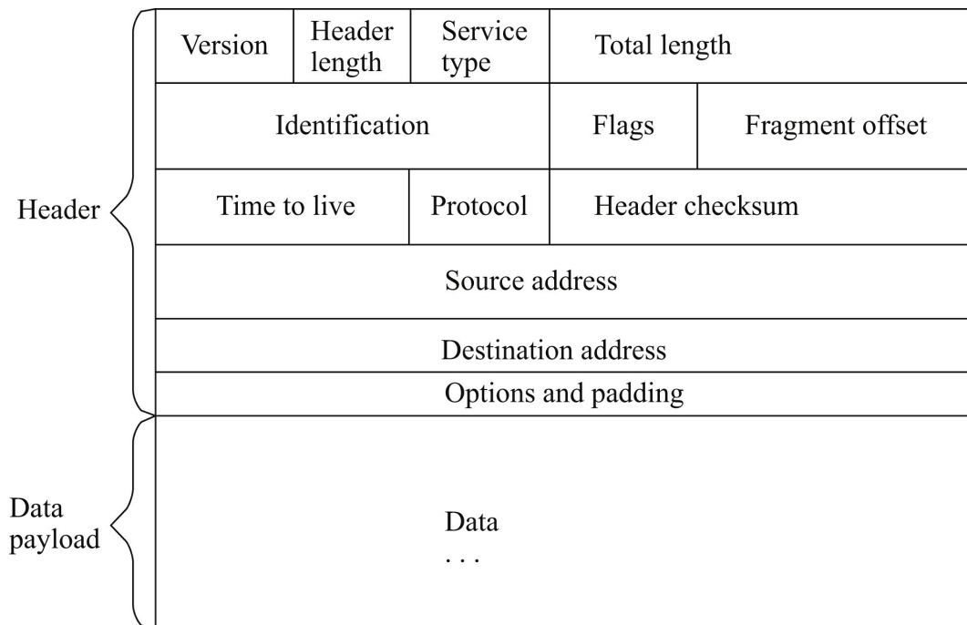
FIGURE 8.6 IP packet structure.
