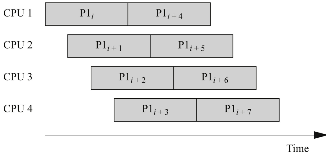
FIGURE 6.4 A sequence of processes with a high initiation rate.
