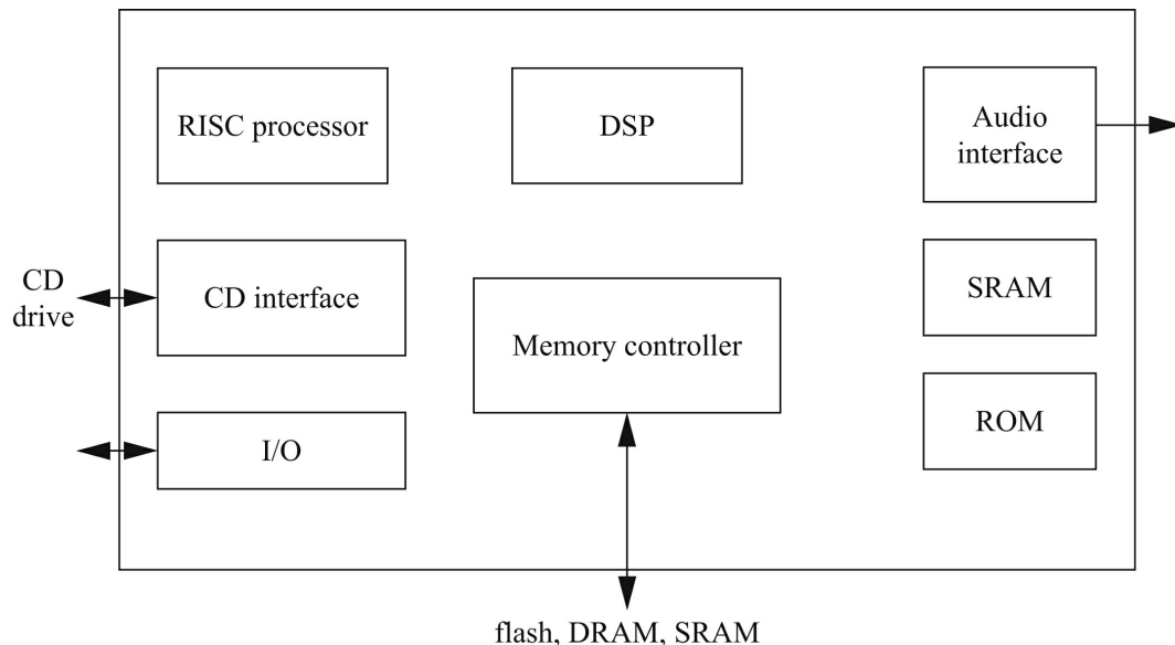
FIGURE 4.47 Architecture of a Cirrus audio processor for CD/MP3 players.
