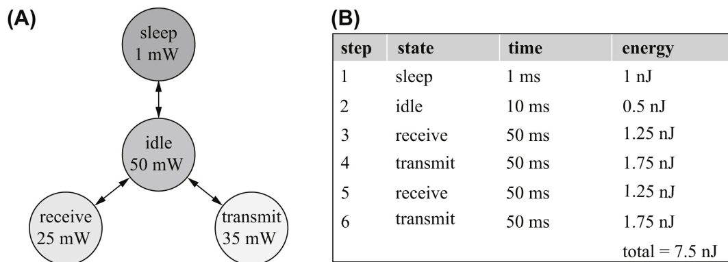
FIGURE 8.12 An example of radio energy consumption analysis. (a) Radio power state machine. (b) Use case-based energy analysis.
