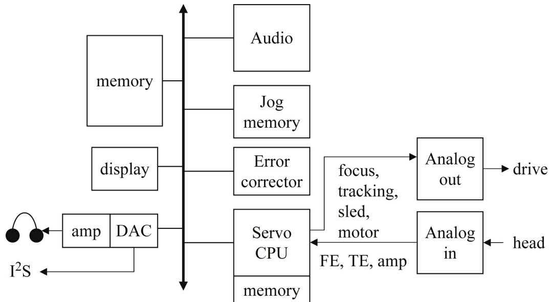
FIGURE 10.31 Computing platform for a CD player.
