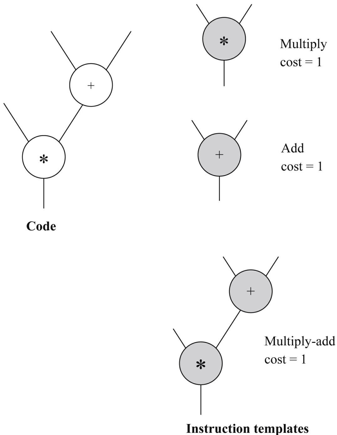
FIGURE 5.19 Code generation by template matching.
