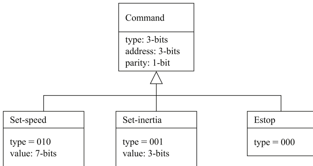
FIGURE 1.32 Refined class diagram for the train controller commands.
