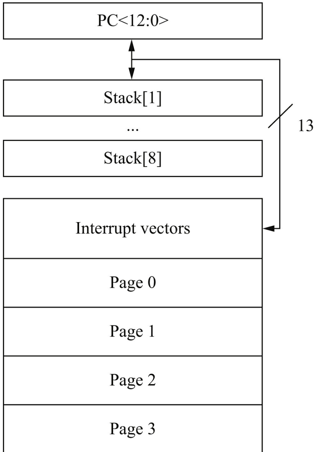
FIGURE 2.18 Instruction space for the PIC16F.
