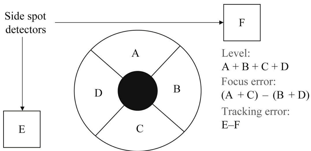
FIGURE 10.30 CD laser pickup regions.
