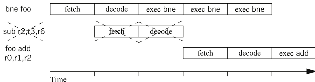
FIGURE 3.18 Pipelined execution of a branch in ARM.
