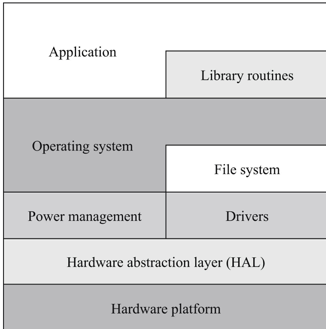
FIGURE 4.2 Software layer diagram for an embedded system.
