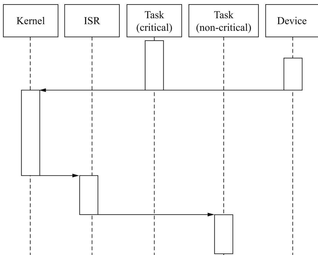
FIGURE 6.18 Interrupt latency during a critical section.
