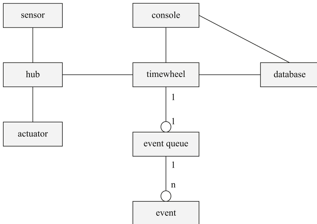
FIGURE 8.19 UML object diagram for smart home.
