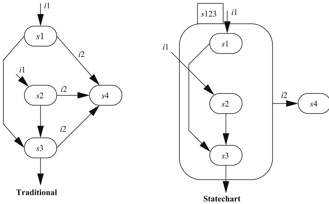
FIGURE 7.7 An OR state in Statecharts.
