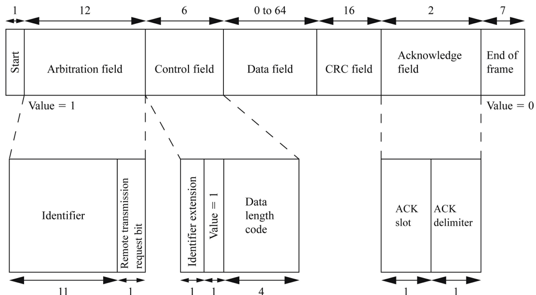
FIGURE 9.3 The CAN data frame format.
