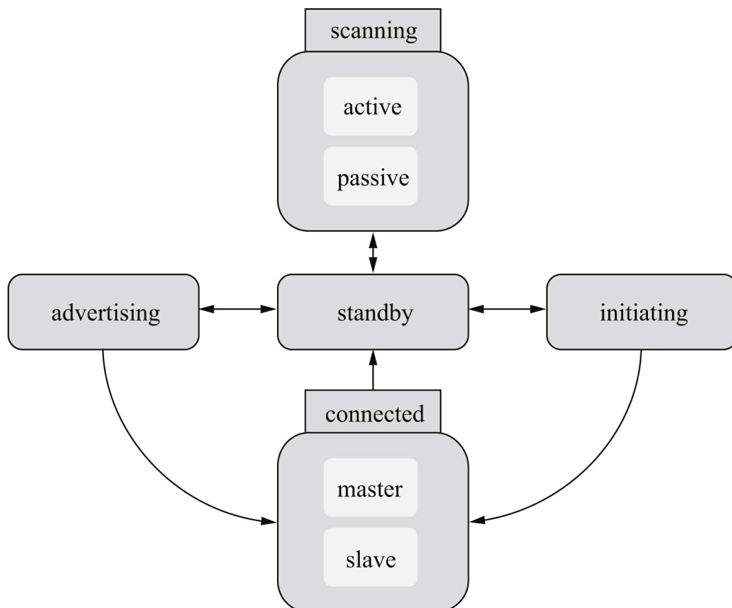
FIGURE 8.13 Bluetooth Low Energy link level state machine.
