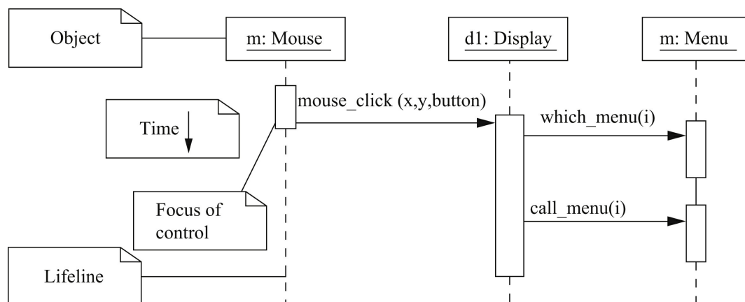
FIGURE 1.14 A sequence diagram in UML.
