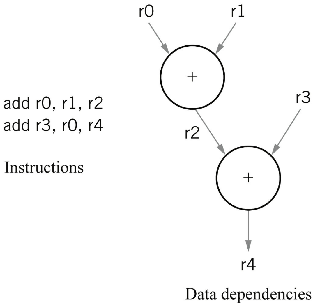
FIGURE 2.5 Data dependencies and order of instruction execution.
