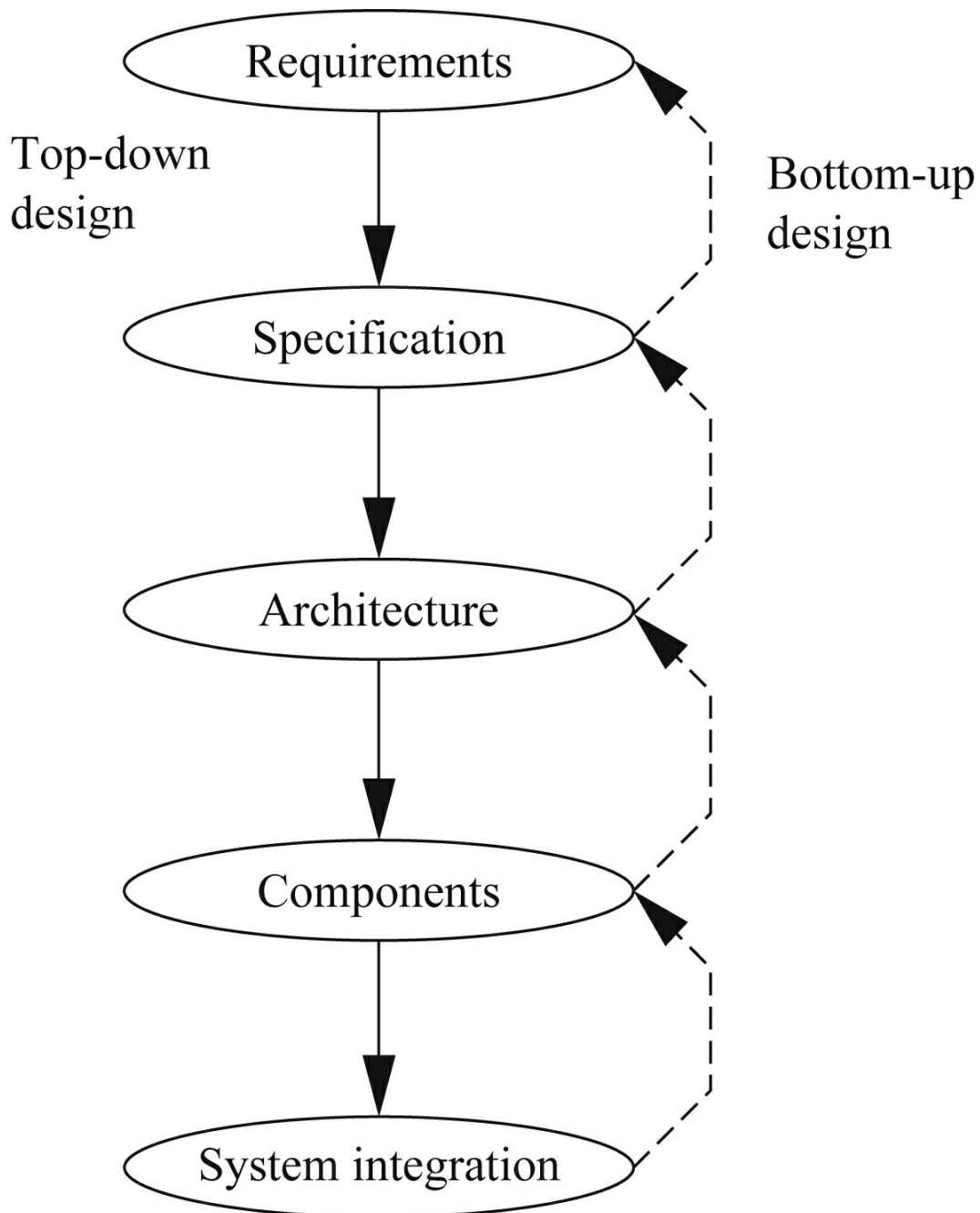
FIGURE 1.1 Major levels of abstraction in the design process.
