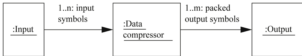
FIGURE 3.20 UML collaboration diagram for the data compressor.
