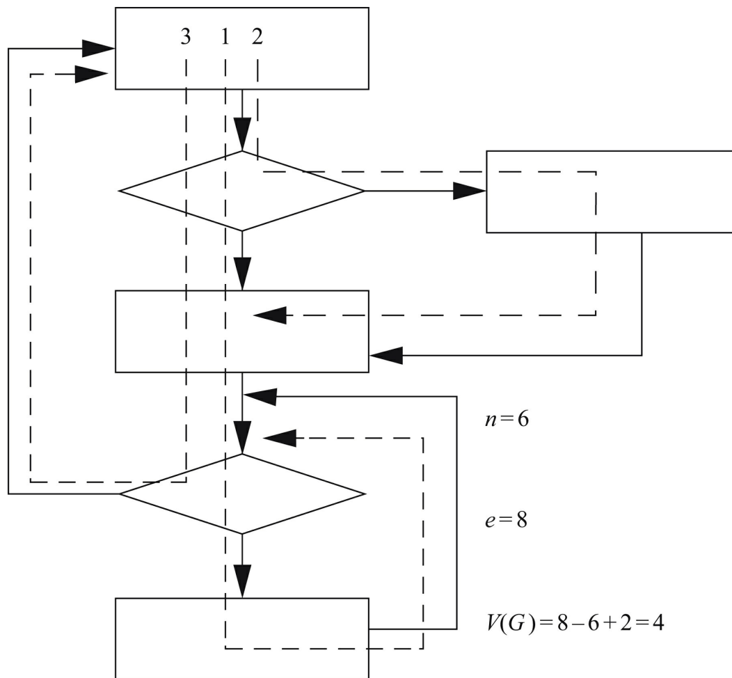
FIGURE 5.25 Cyclomatic complexity.
