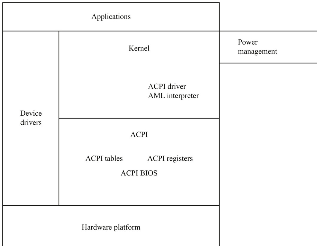
FIGURE 4.33 The Advanced Configuration and Power Interface and its relationship to a complete system.
