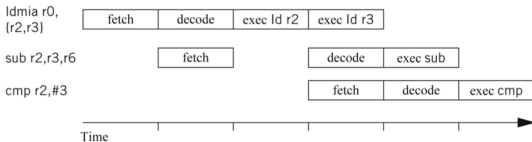
FIGURE 3.17 Pipelined execution of multicycle ARM instructions.
