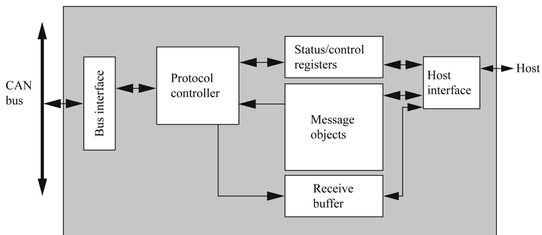
FIGURE 9.4 Architecture of a CAN controller.
