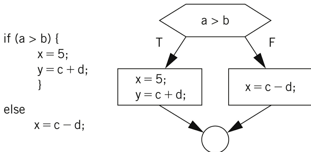
FIGURE 5.14 Flow of control in C and control flow diagrams.
