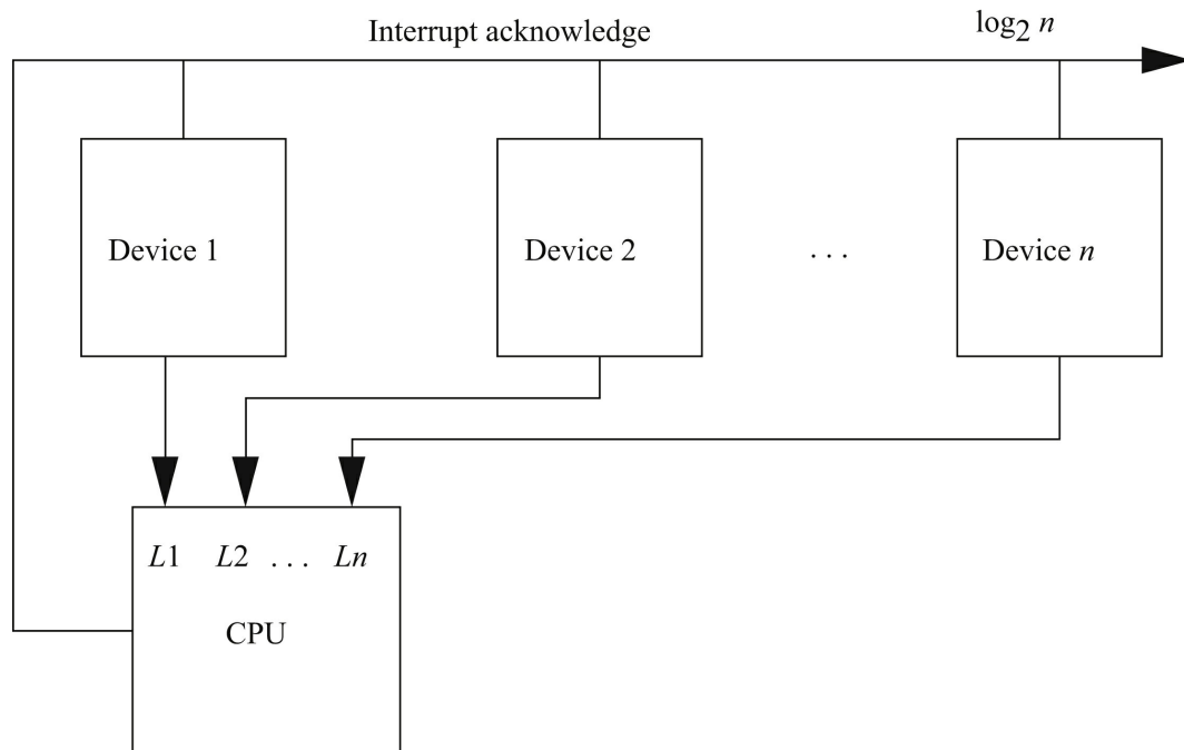
FIGURE 3.3 Prioritized device interrupts.
