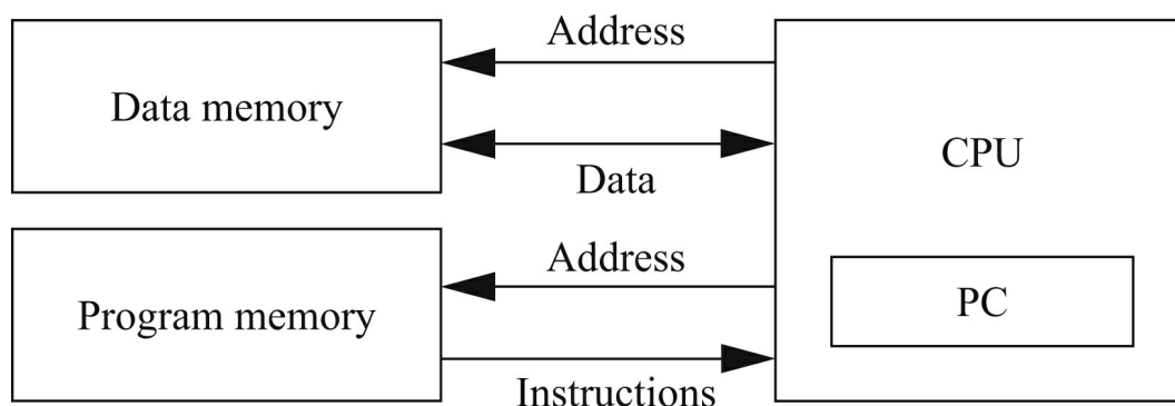
FIGURE 2.2 A Harvard architecture.
