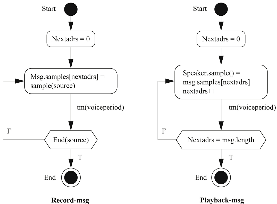
FIGURE 6.26 State diagrams for the record-msg and playback-msg behaviors.
