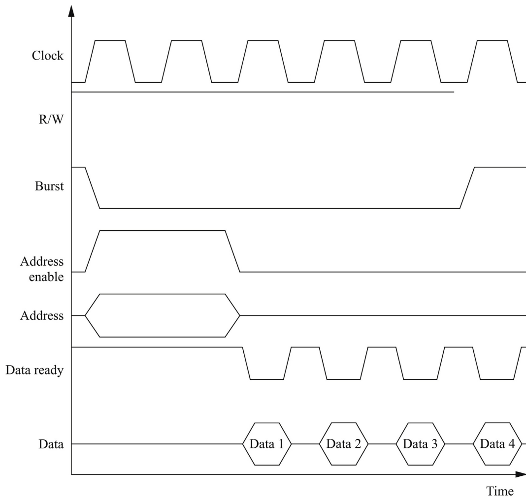
FIGURE 4.9 A burst read transaction.
