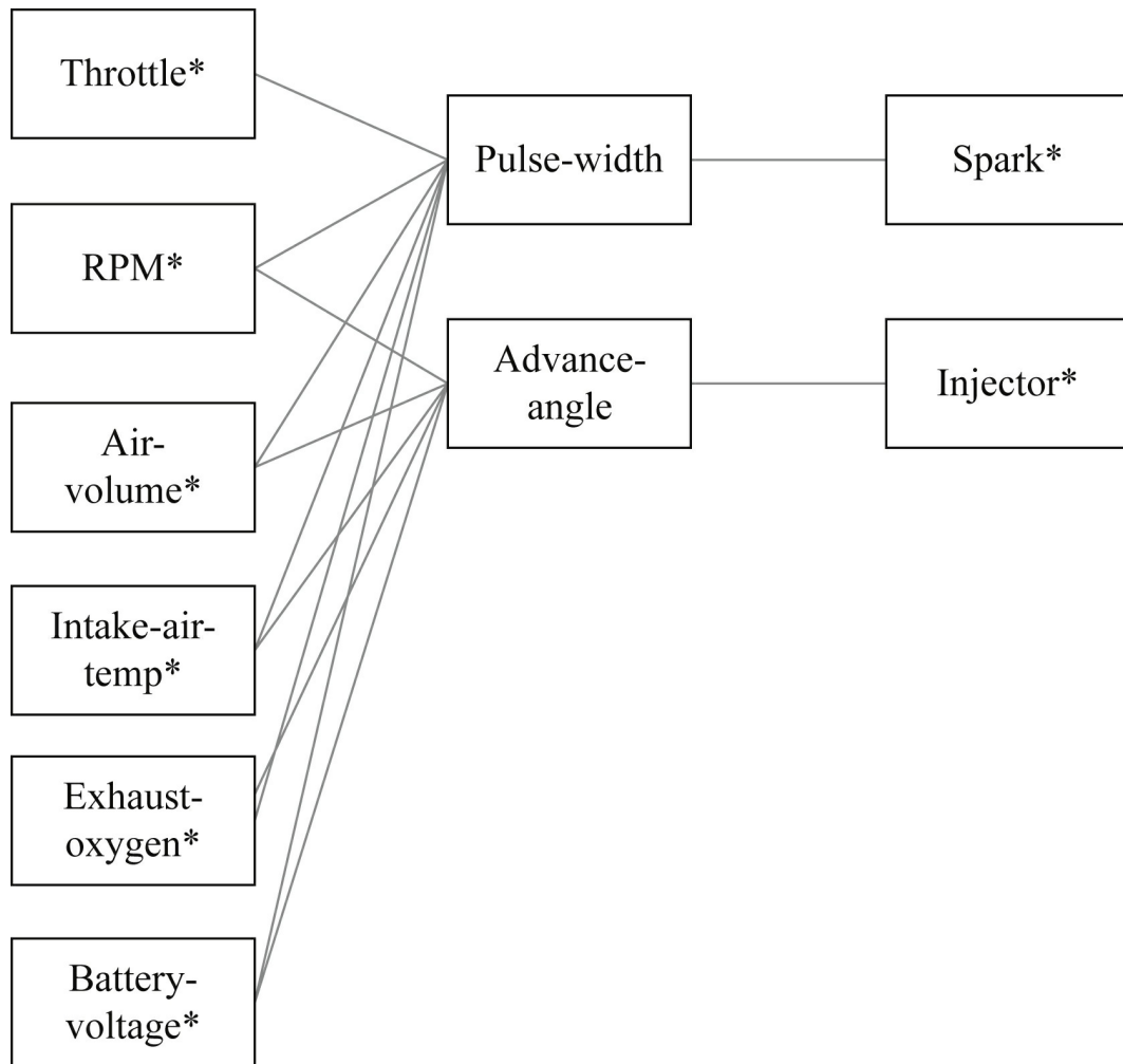
FIGURE 6.31 Class diagram for the engine controller.
