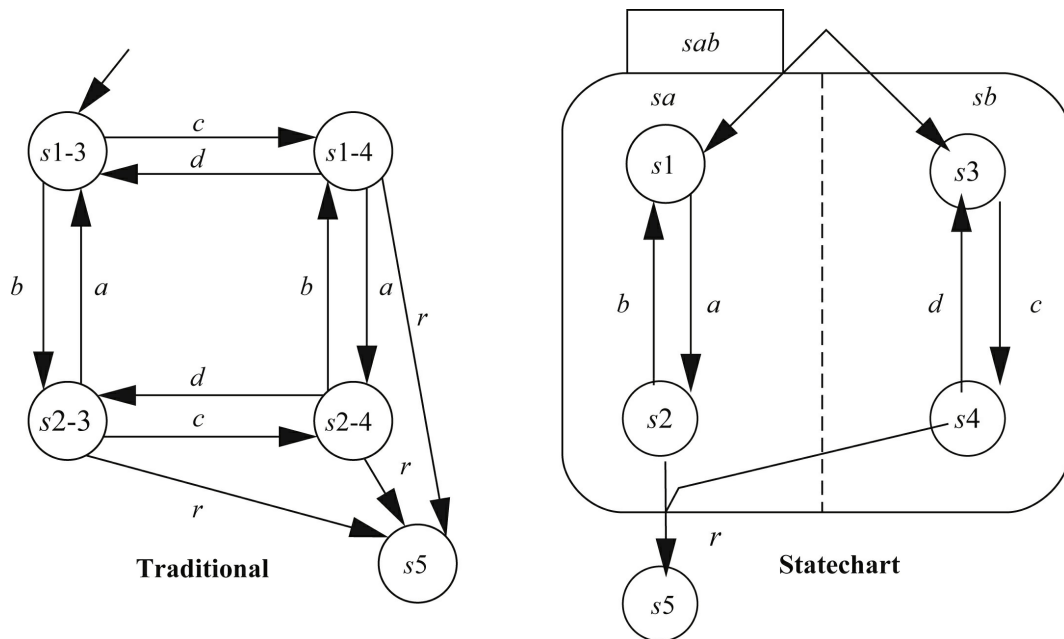
FIGURE 7.8 An AND state in Statecharts.
