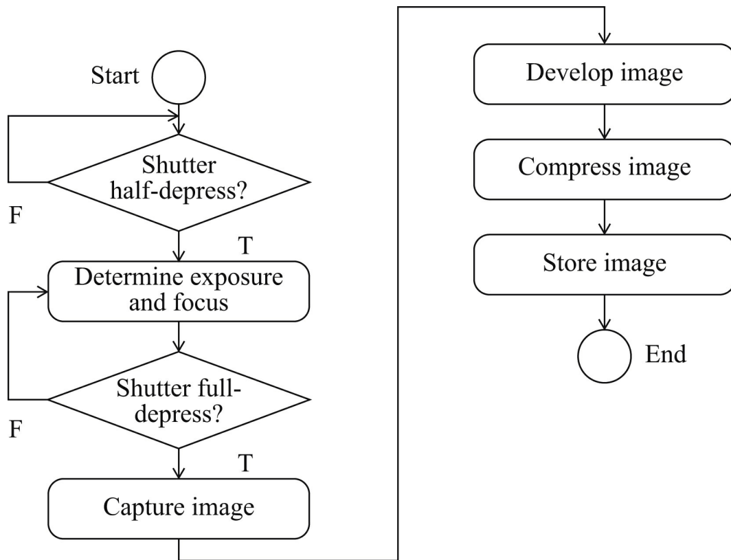
FIGURE 5.40 State diagram for picture taking.
