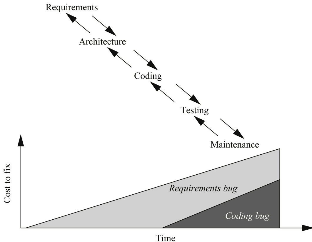
FIGURE 7.11 Long-lived bugs are more expensive to fix.
