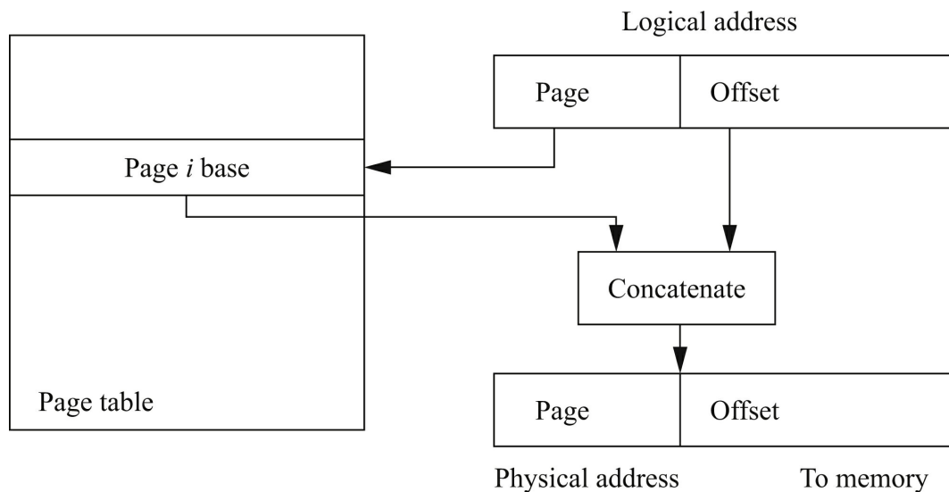
FIGURE 3.13 Address translation for a page.
