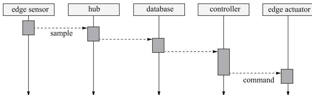
FIGURE 8.3 Use case for an IoT control system.
