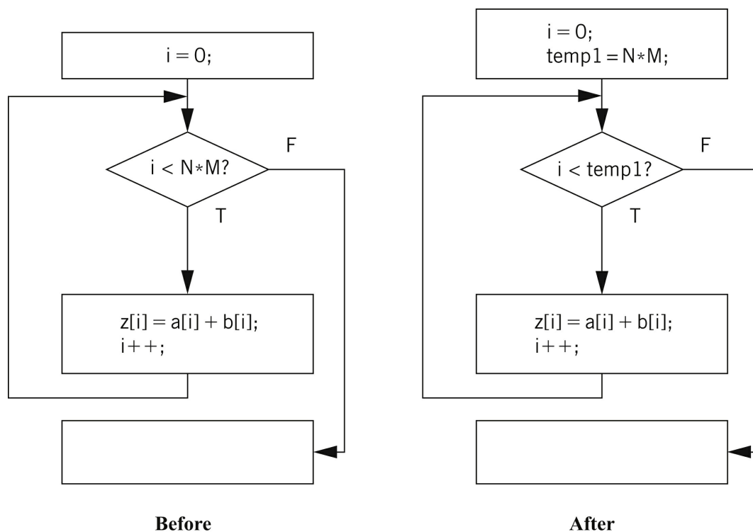
FIGURE 5.21 Code motion in a loop.
