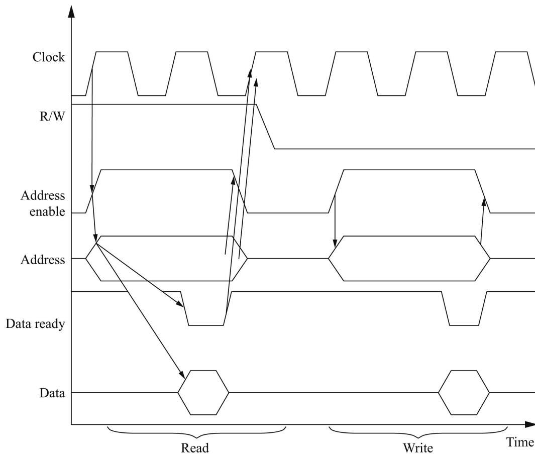
FIGURE 4.7 Timing diagram for read and write on the example bus.
