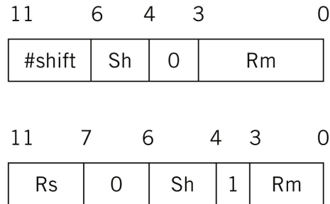
FIGURE 2.4 Format of an ARM data processing instruction.
