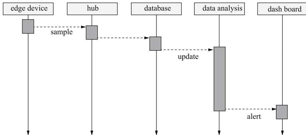
FIGURE 8.2 Use case for an IoT monitoring system.
