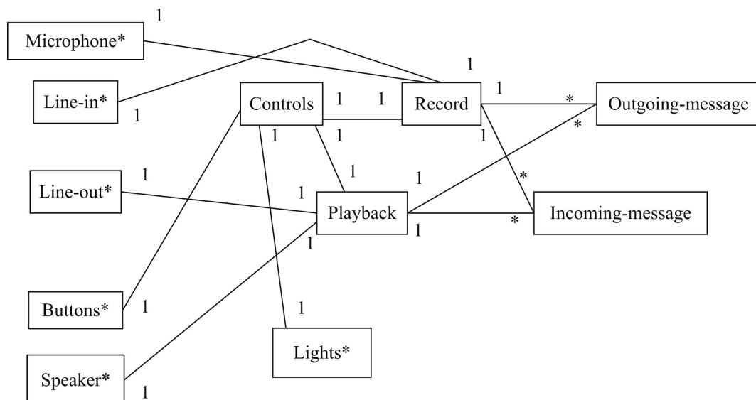
FIGURE 6.21 Class diagram for the answering machine.
