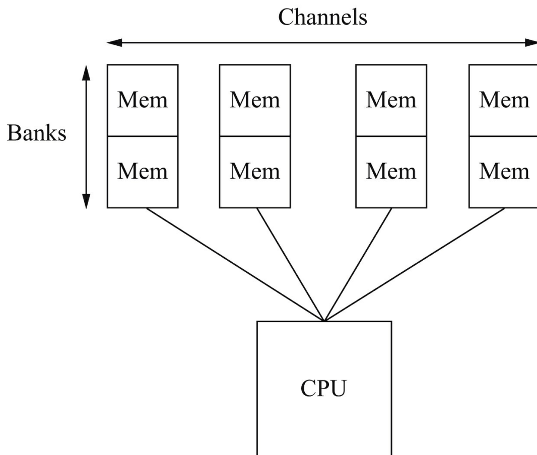
FIGURE 4.20 Channels and banks in a memory system.
