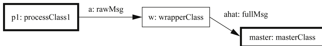
FIGURE 6.11 A collaboration diagram with active and normal objects.
