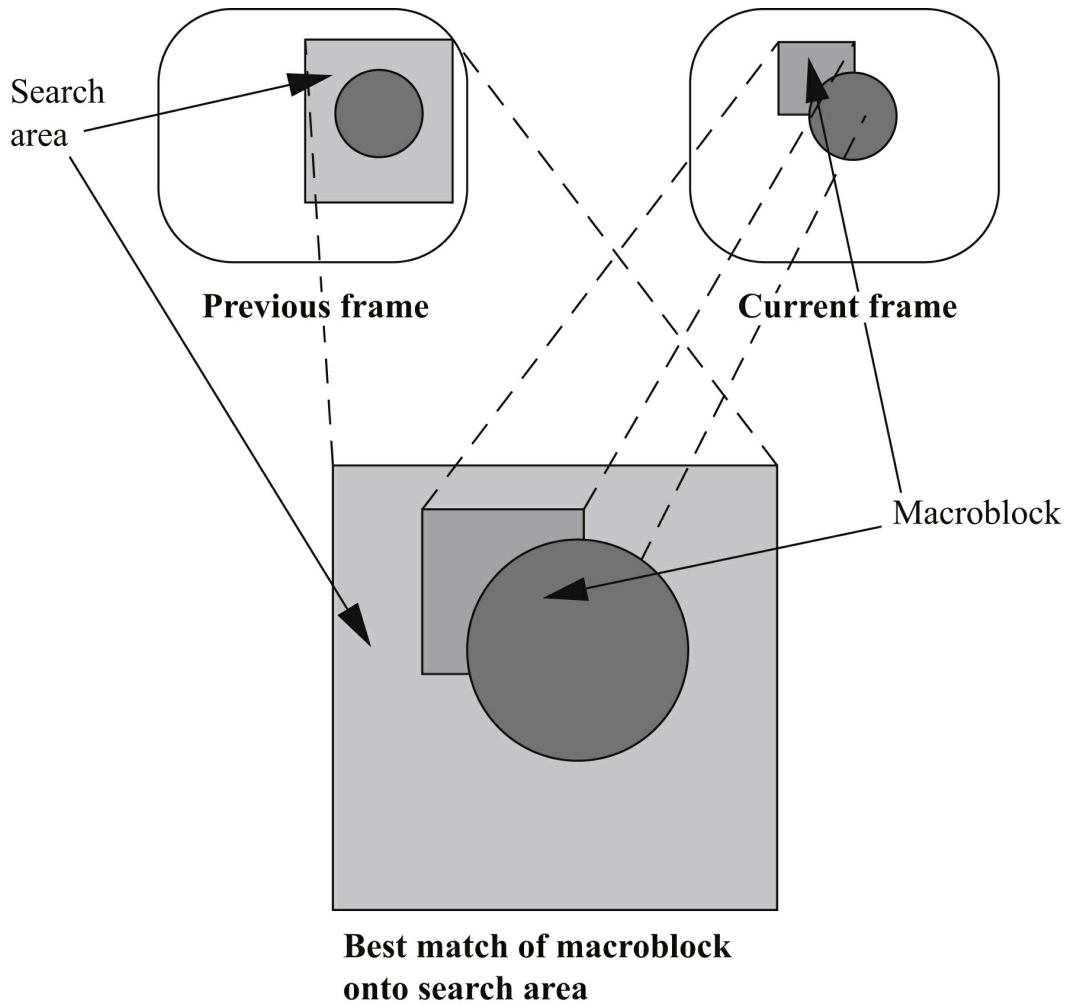
FIGURE 10.18 Block motion estimation.
