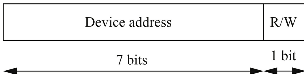
FIGURE 10.12 Format of an I 2 C address transmission.
