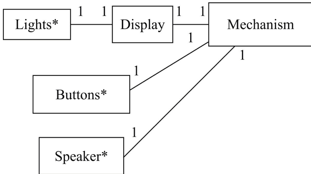
FIGURE 4.35 Class diagram for the alarm clock.
