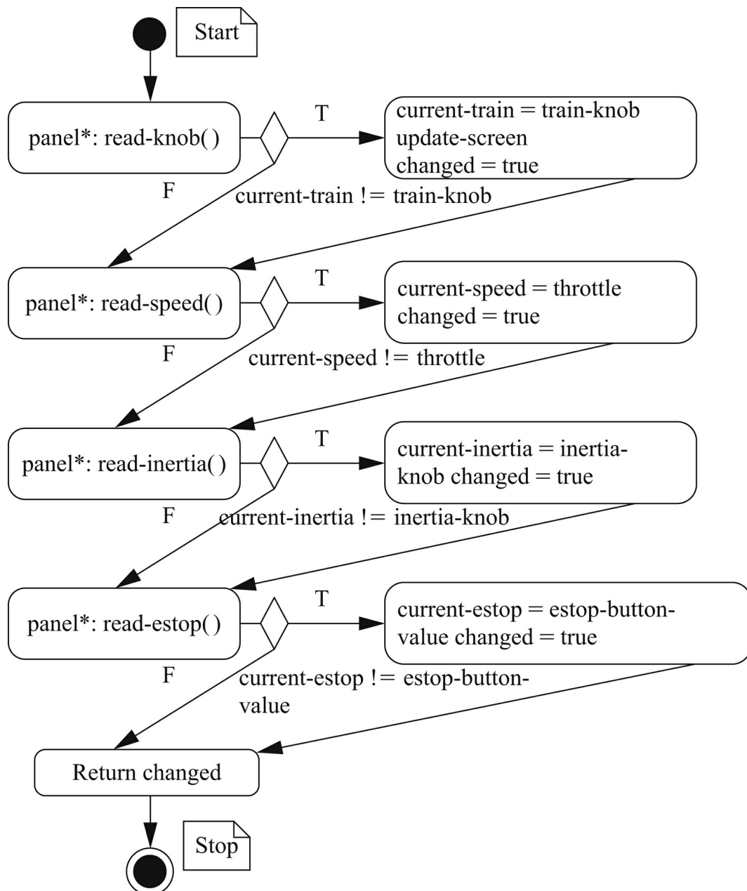
FIGURE 1.28 State diagram for the panel-active behavior.
