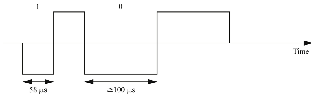
FIGURE 1.16 Bit encoding in DCC.
