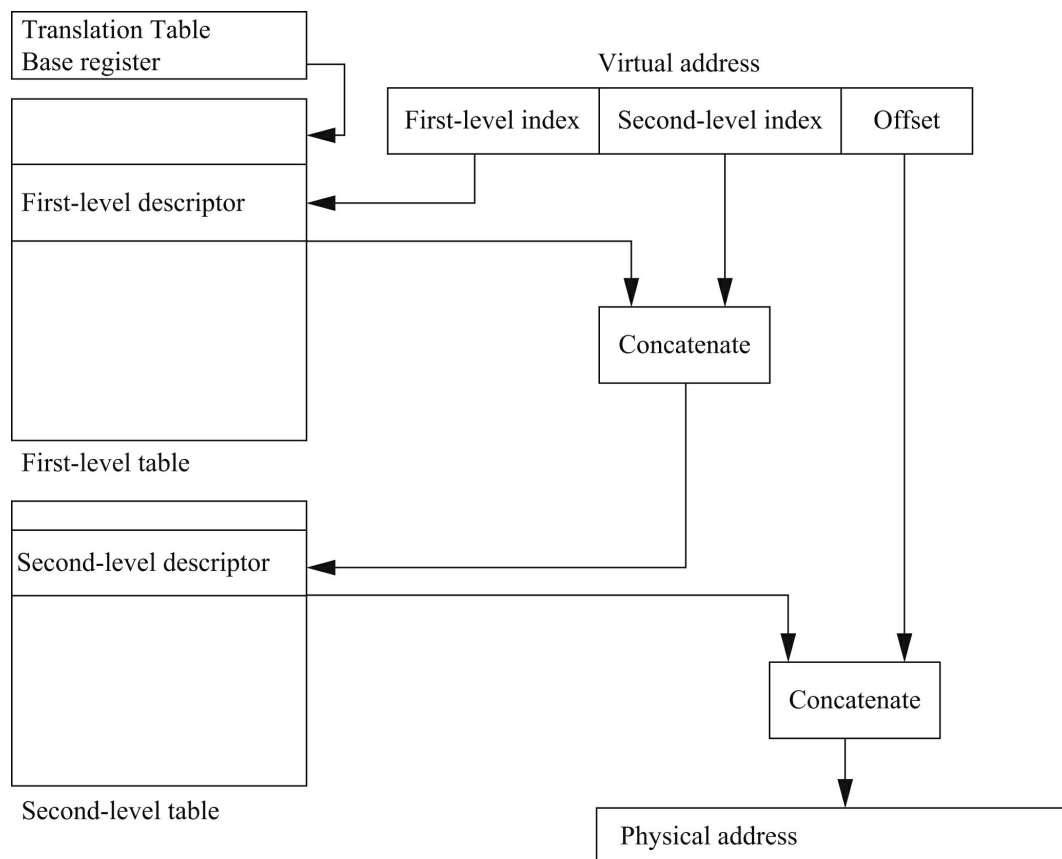
FIGURE 3.15 ARM two-stage address translation.
