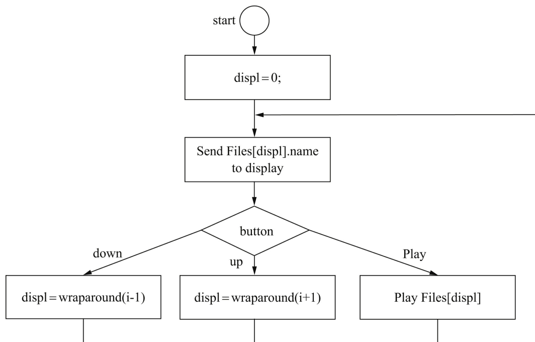
FIGURE 4.45 State diagram for file display and selection.
