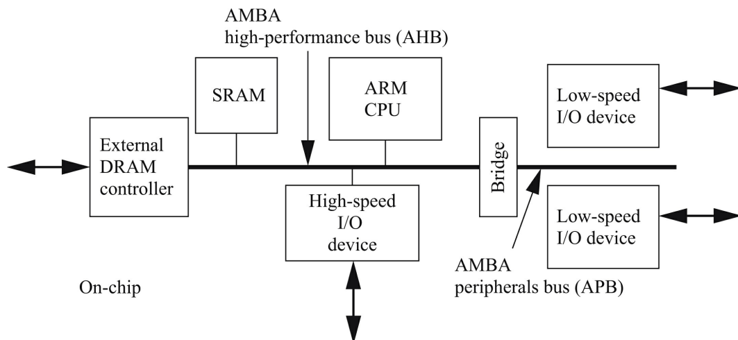
FIGURE 4.16 Elements of the ARM AMBA bus system.
