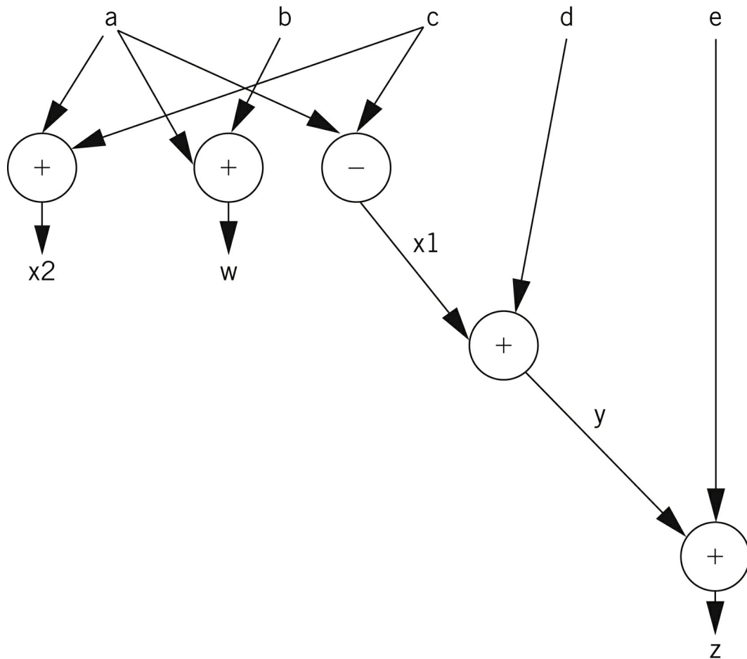
FIGURE 5.7 Standard data flow graph for our sample basic block.
