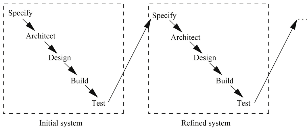
FIGURE 7.3 A successive refinement development model.
