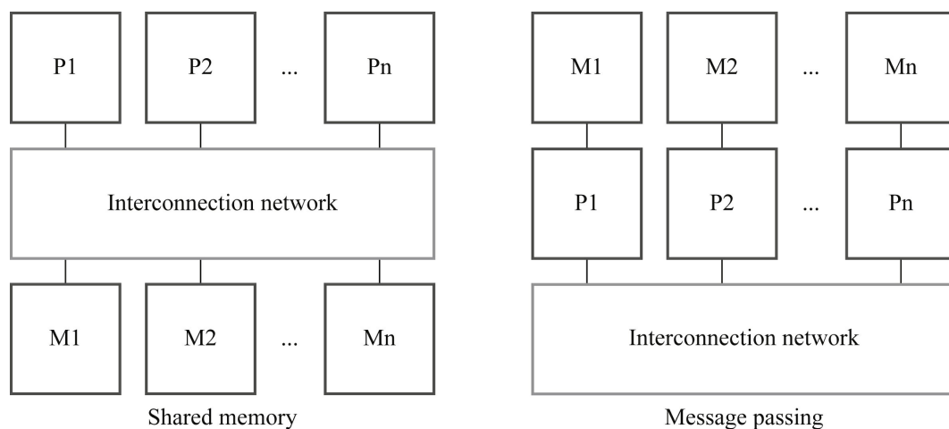
FIGURE 10.3 The two major multiprocessor architectures.
