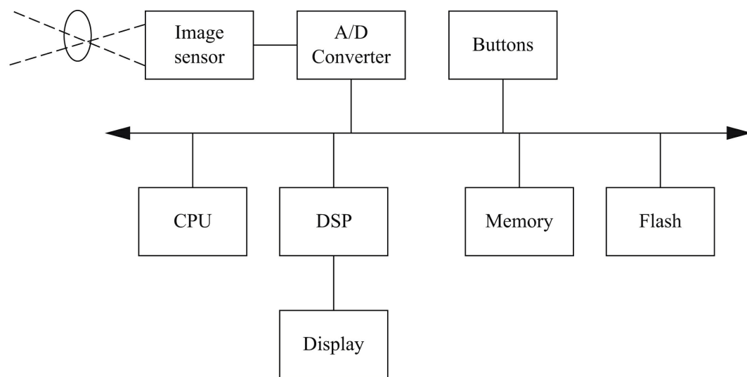
FIGURE 5.42 Computing platform for a digital still camera.
