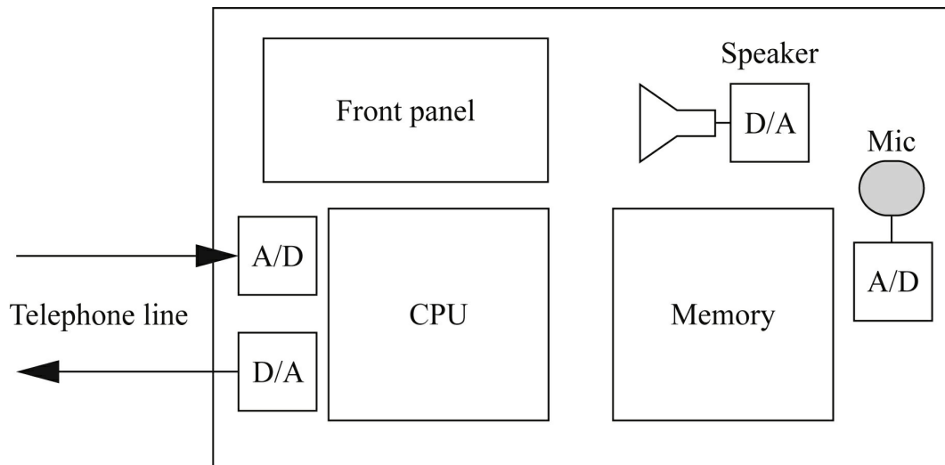
FIGURE 6.27 Hardware platform for the answering machine.
