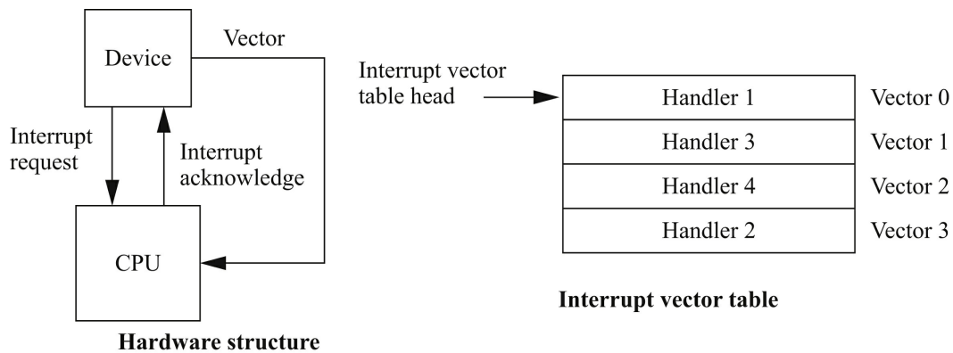
FIGURE 3.5 Interrupt vectors.
