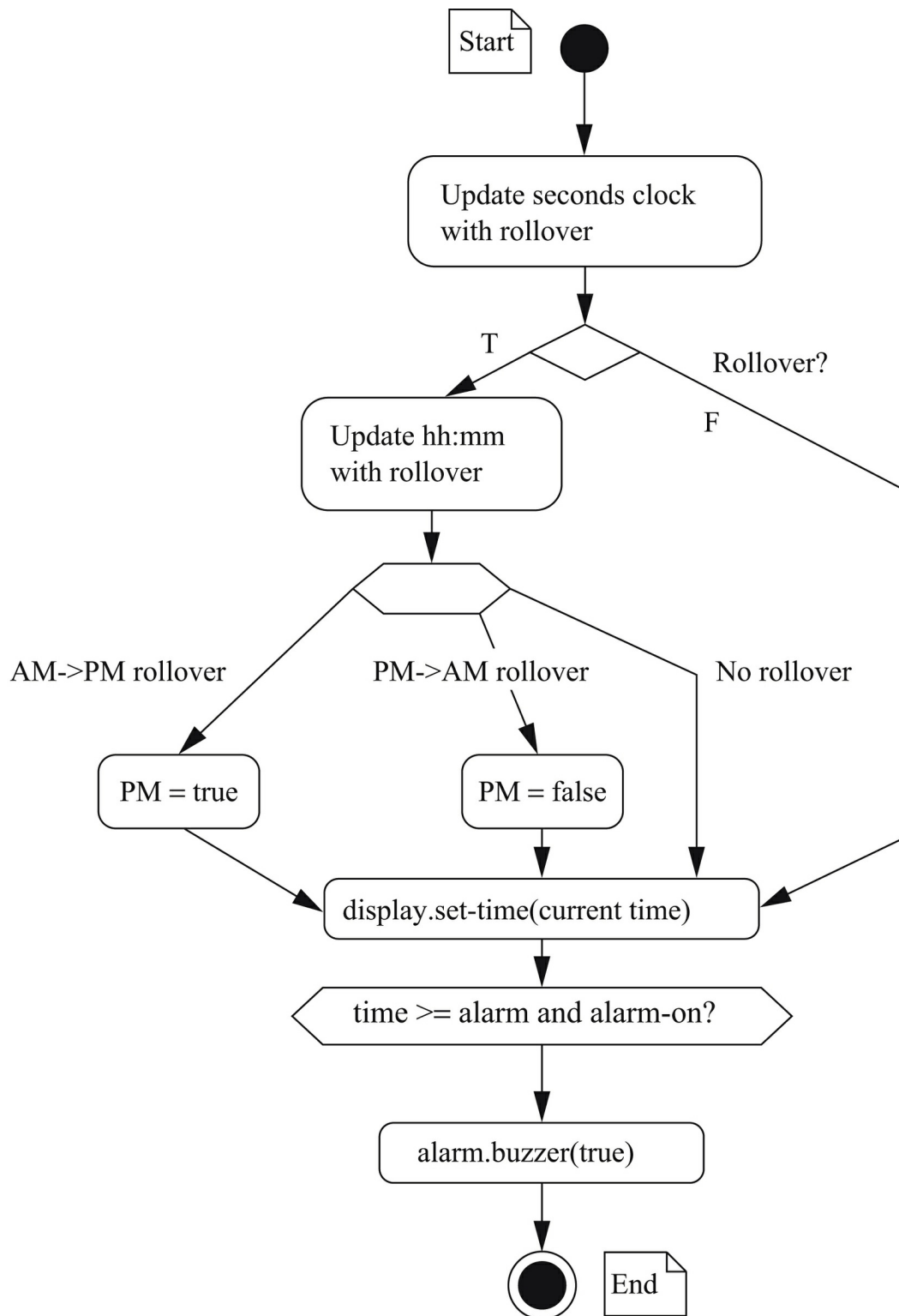
FIGURE 4.38 State diagram for update-time.
